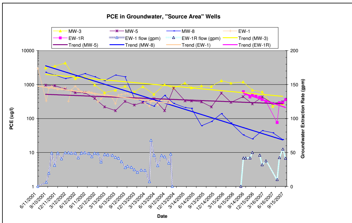
Figure 2. Historical PCE concentrations and trends in source area monitoring wells.
