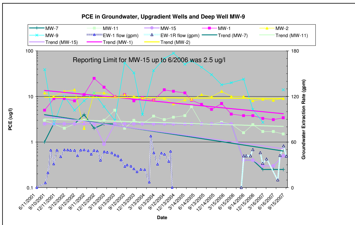
Figure 4. Historical PCE concentrations and trends in upgradient monitoring wells.
