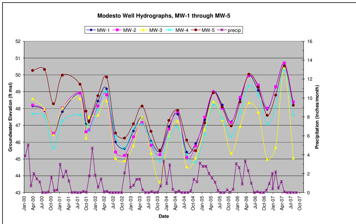
Figure 6. Select monitoring well hydrographs and monthly precipitation data.
