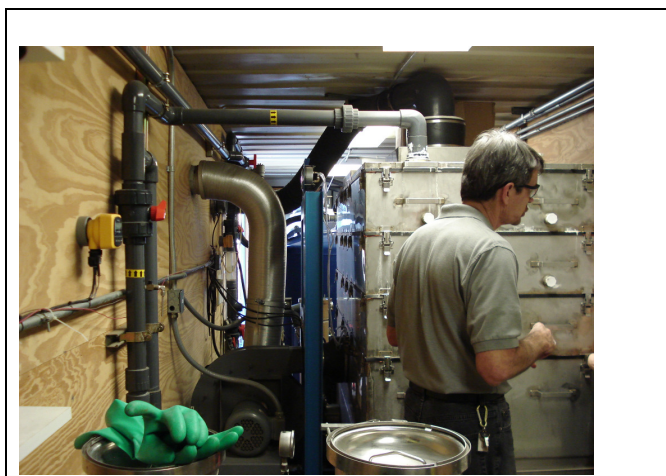
Photo 5. Air stripper inside GWTS unit.
