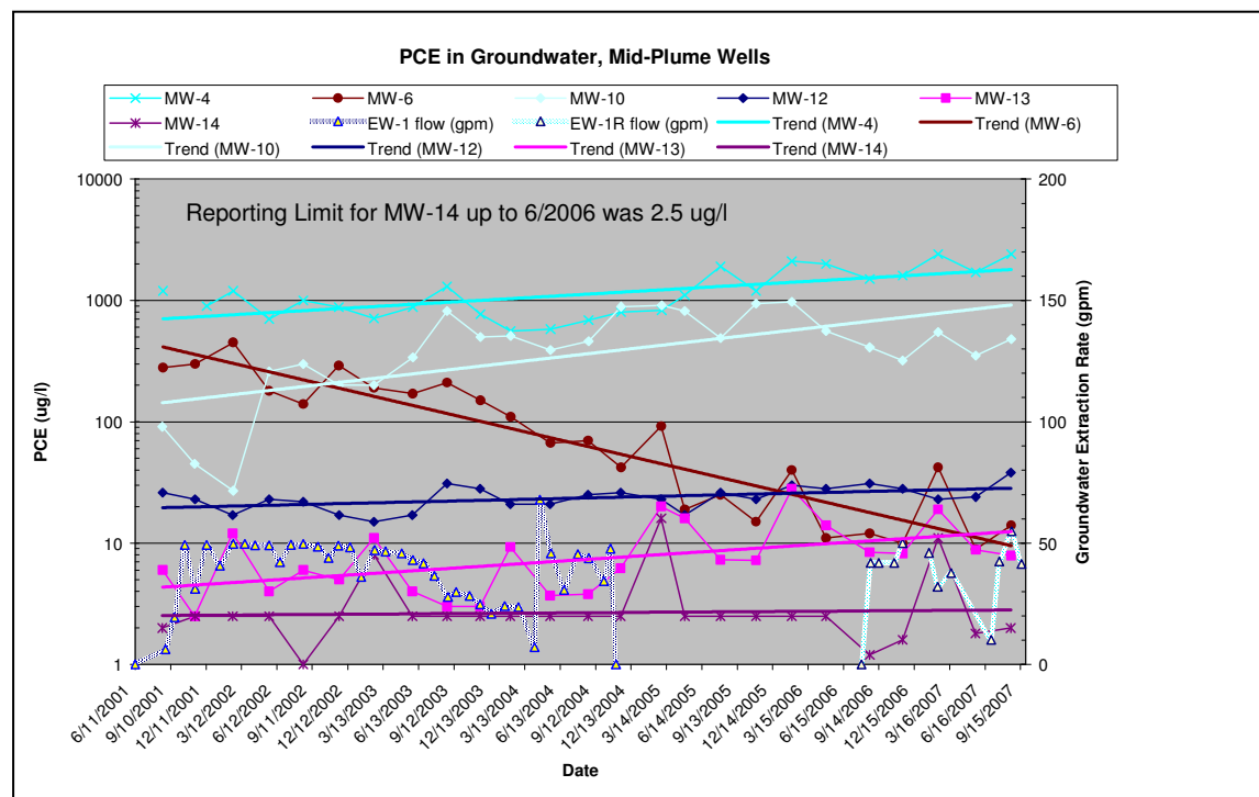
Figure 3. Historical PCE concentrations and trends in downgradient and side-gradient monitoring wells.
