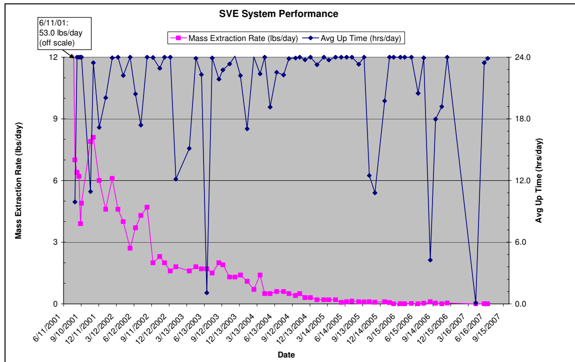
Figure 8. SVE system historical PCE mass extraction rate and operational data.
