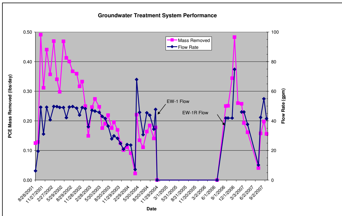
Figure 7. GWT system historical PCE mass extraction rate and operational data.
