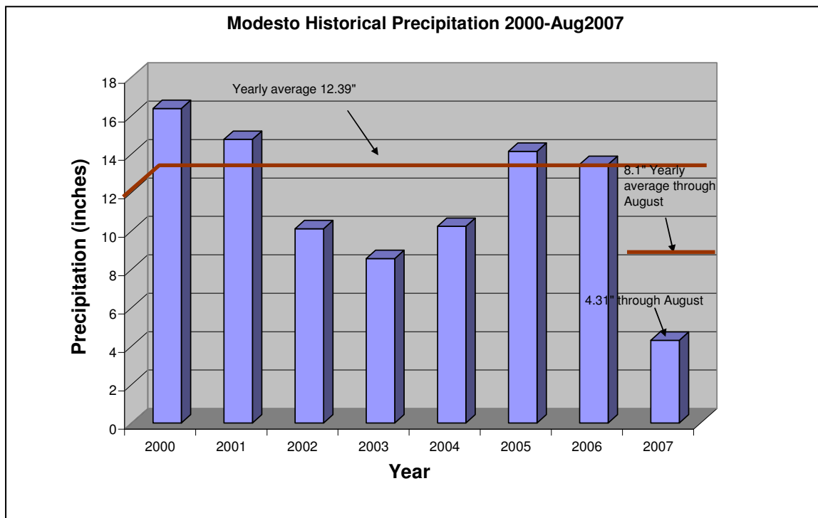
Figure 5. Historical annual precipitation for the Modesto Cooperative Weather Station compared to yearly average.
