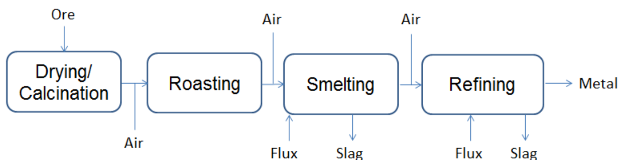
Exhibit 1.F.1. Simplified Flow Chart of Pyrometallurgical Processing 369
