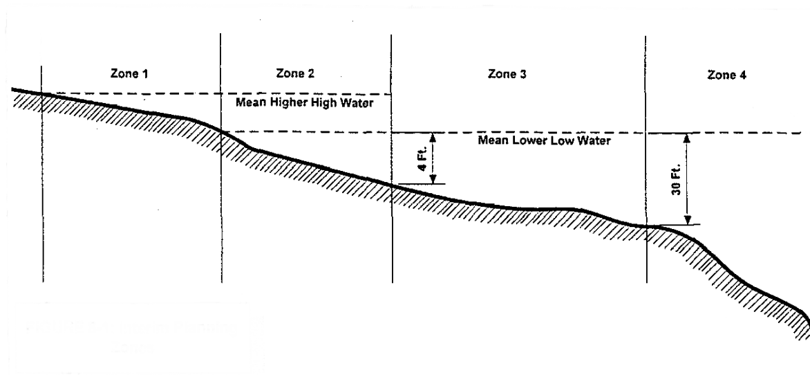
Figure 9-1. Example of Offshore Clearance Zones
