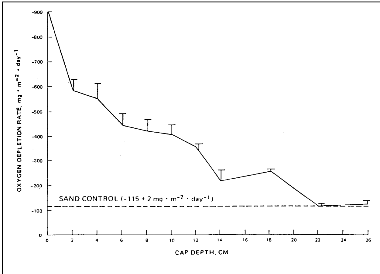
Figure C2. Typical results for effect of sand cap on oxygen command (Sturgis and Gunnison 1988)
