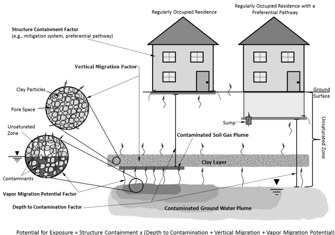
Figure 6. Potential for Exposure
