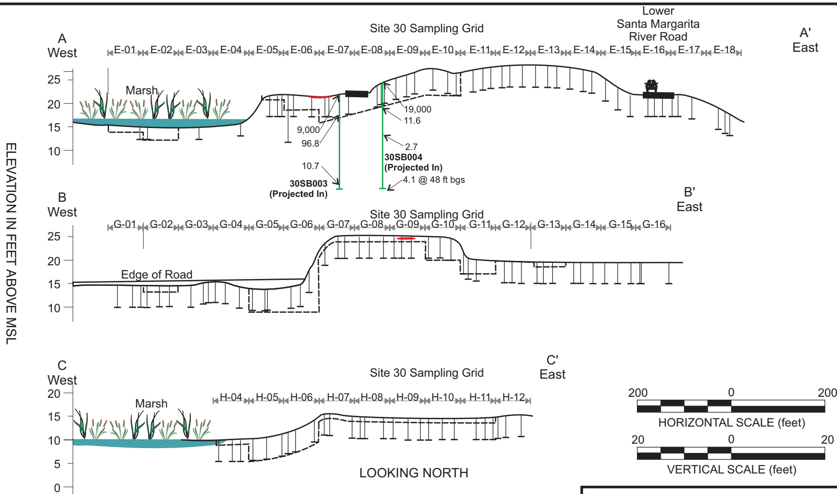
Figure 4-3 Site 30 Generalized Cross Sections
