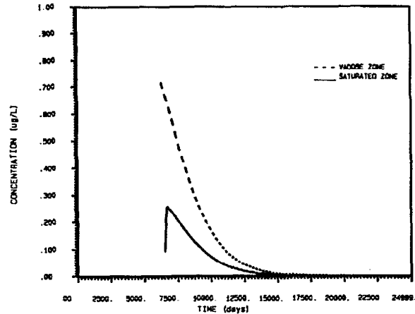
LIQUID PHASE CONCENTRATION VS TIME FOR VADOSE-ZONE AND SATURATED ZONE MODELS
