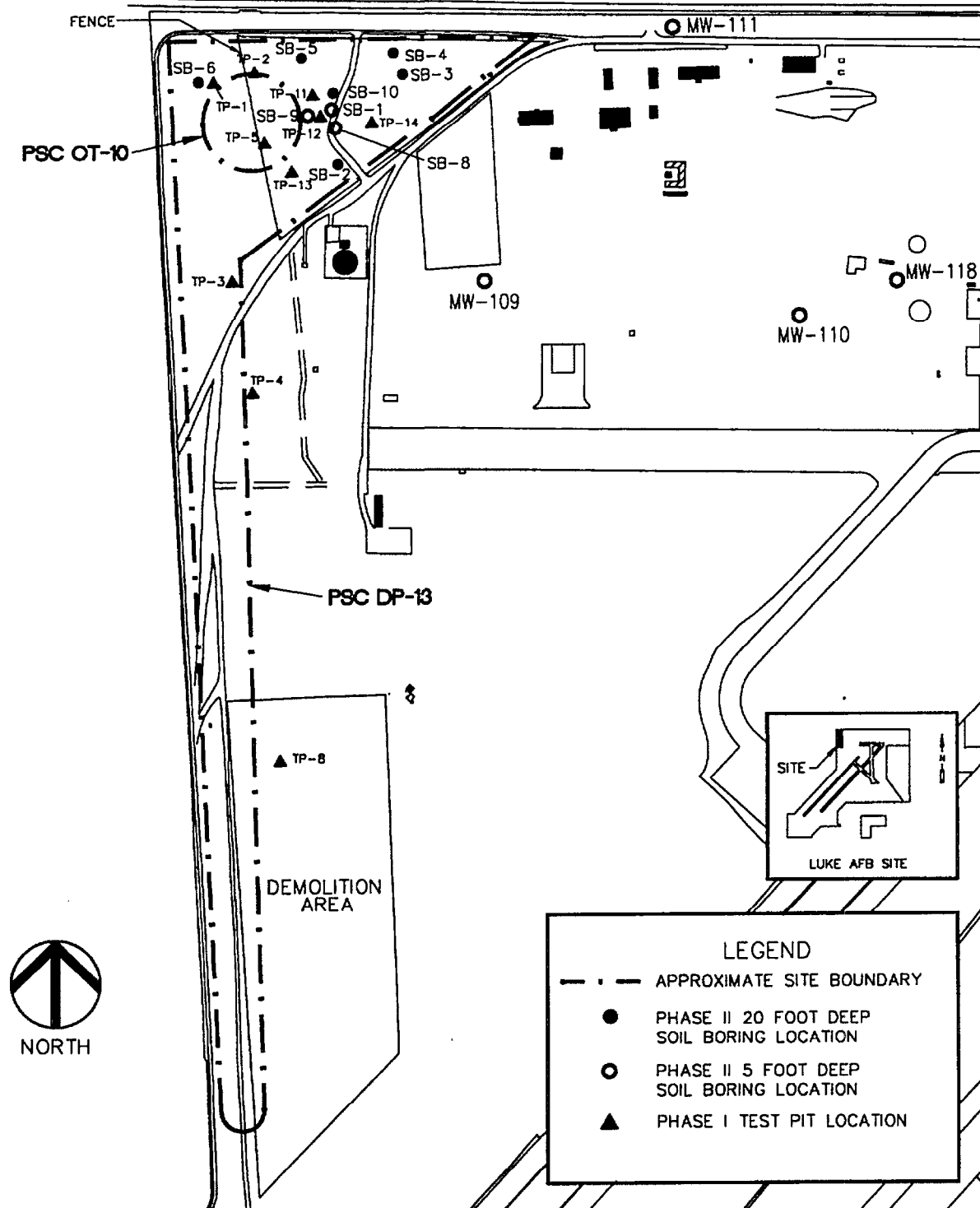
SITE DIAGRAM - PSCs OT-10 and DP-13 LOCATIONS OF SAMPLES WITH CONSTITUENTS OF CONCERN OPERABLE UNIT No.1, RECORD OF DECISION LUKE AIR FORCE BASE, ARIZONA
