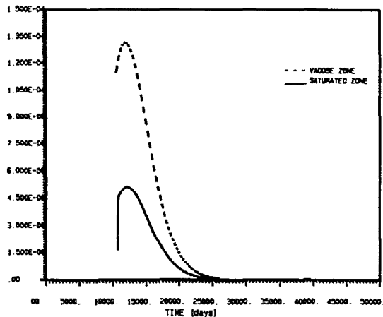
LIQUID PHASE CONCENTRATION VS TIME FOR VADOSE-ZONE AND SATURATED ZONE MODELS
