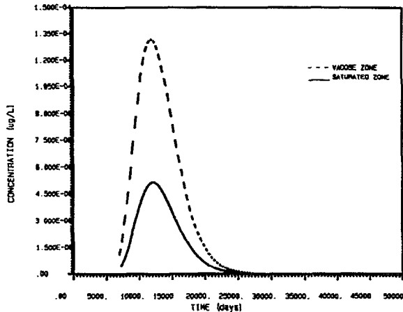
LIQUID PHASE CONCENTRATION VS TIME FOR VADOSE-ZONE AND SATURATED-ZONE MODELS
