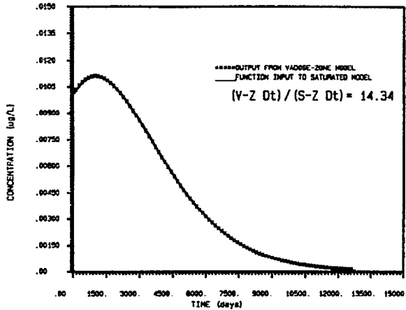
LIQUID PHASE CONCENTRATION VS TIME (CORRECTED TO INITIAL BREAKTHROUGH)
