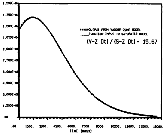
LIQUID PHASE CONCENTRATION VS TIME (CORRECTED TO INITIAL BREAKTHROUGH)
