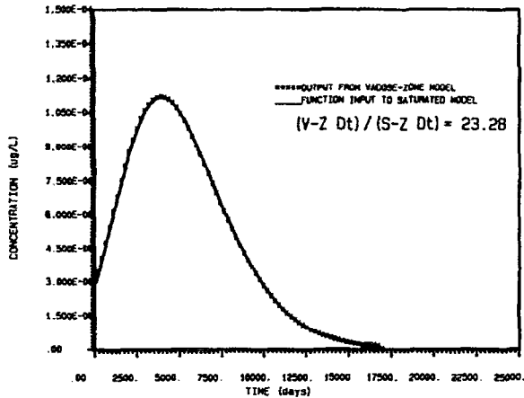
LIQUID PHASE CONCENTRATION VS TIME (CORRECTED TO INITIAL BREAKTHROUGH)
