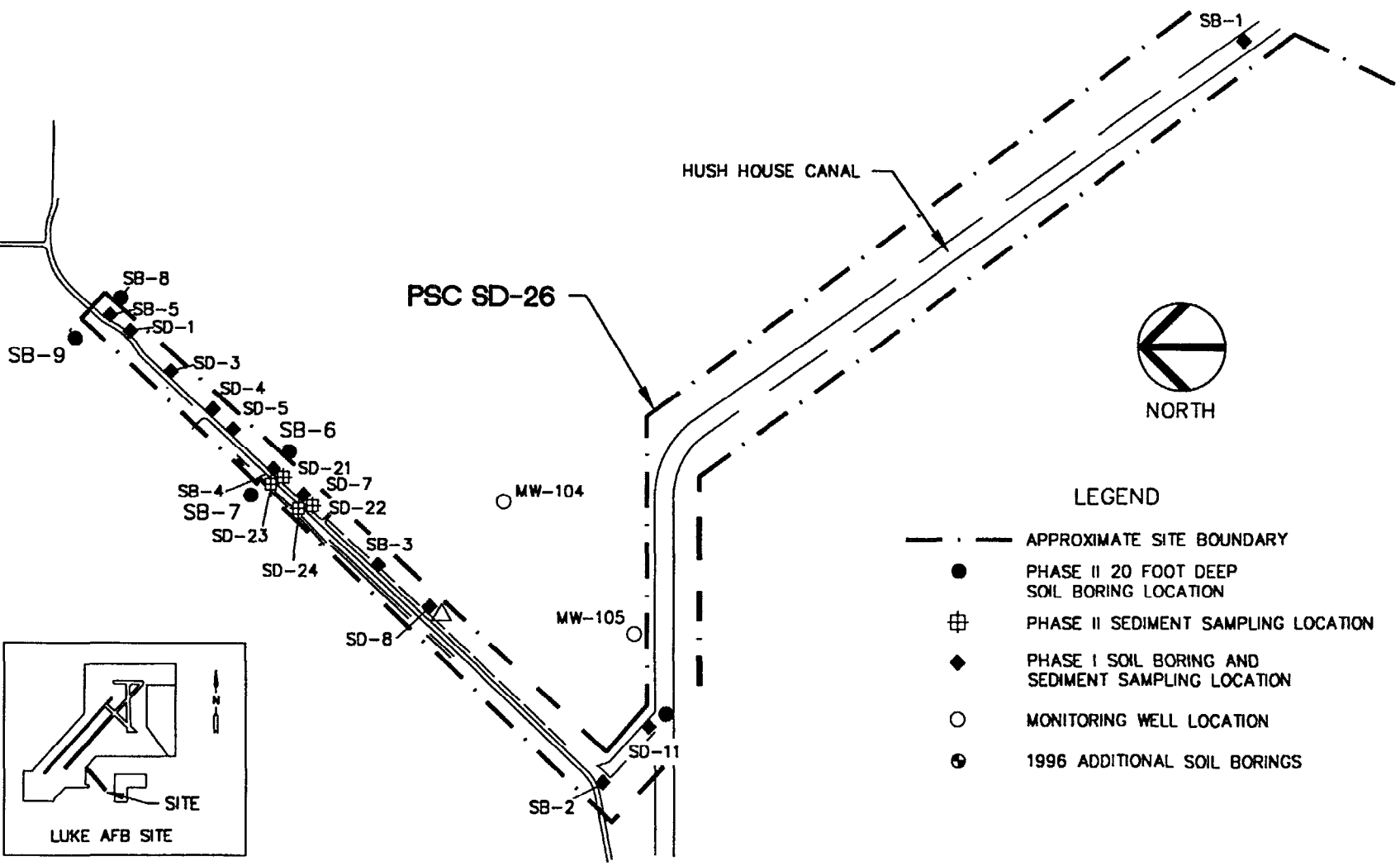
SITE DIAGRAM - PSC SD-26 LOCATIONS OF SAMPLES WITH CONSTITUENTS OF CONCERN OPERABLE UNIT No.1, RECORD OF DECISION LUKE AIR FORCE BASE, ARIZONA
