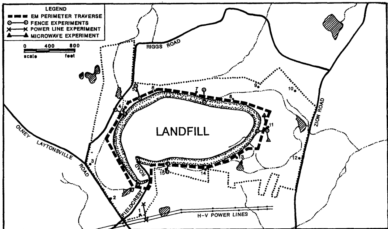
Figure 2-11. Surface geophysical EM-Conductivity) surveys were conducted periodically along transects between monitor wells encircling a sanitary landfill in Maryland to augment the leak detection monitoring network (from Rumbaugh et al., 1987).
