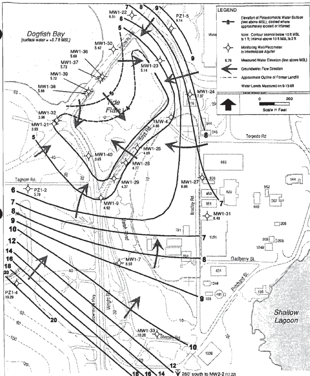
Figure 3-24 Water-level Contour Map Intermediate Aquifer - High Tide Round 5
