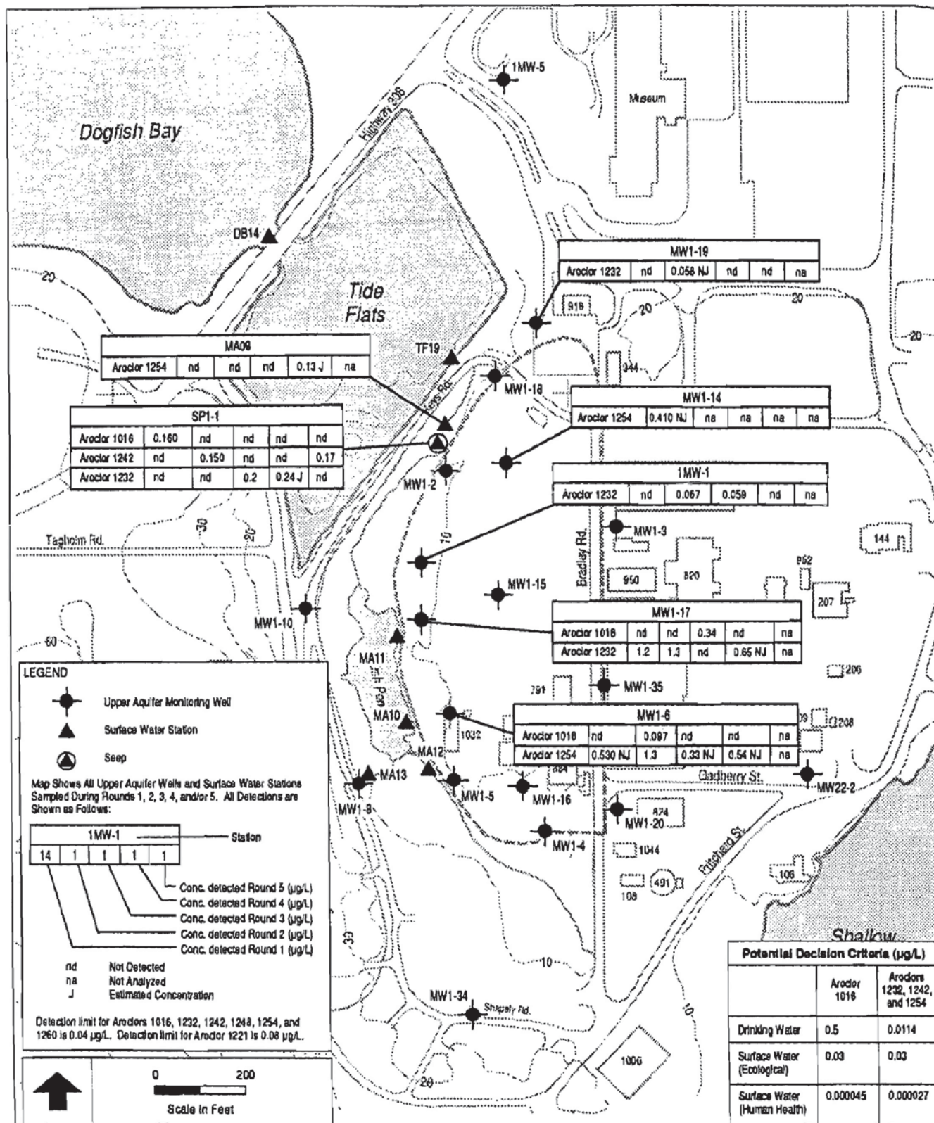
Figure 30 Distribution of Aroclors in Upper Aquifer and Surface Water
