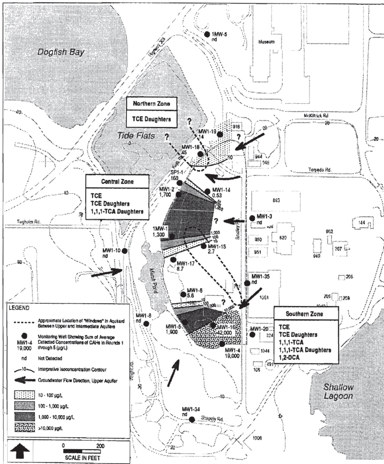
Figure 6-3 CAH Contaminant Zones in the Upper Aquifer
