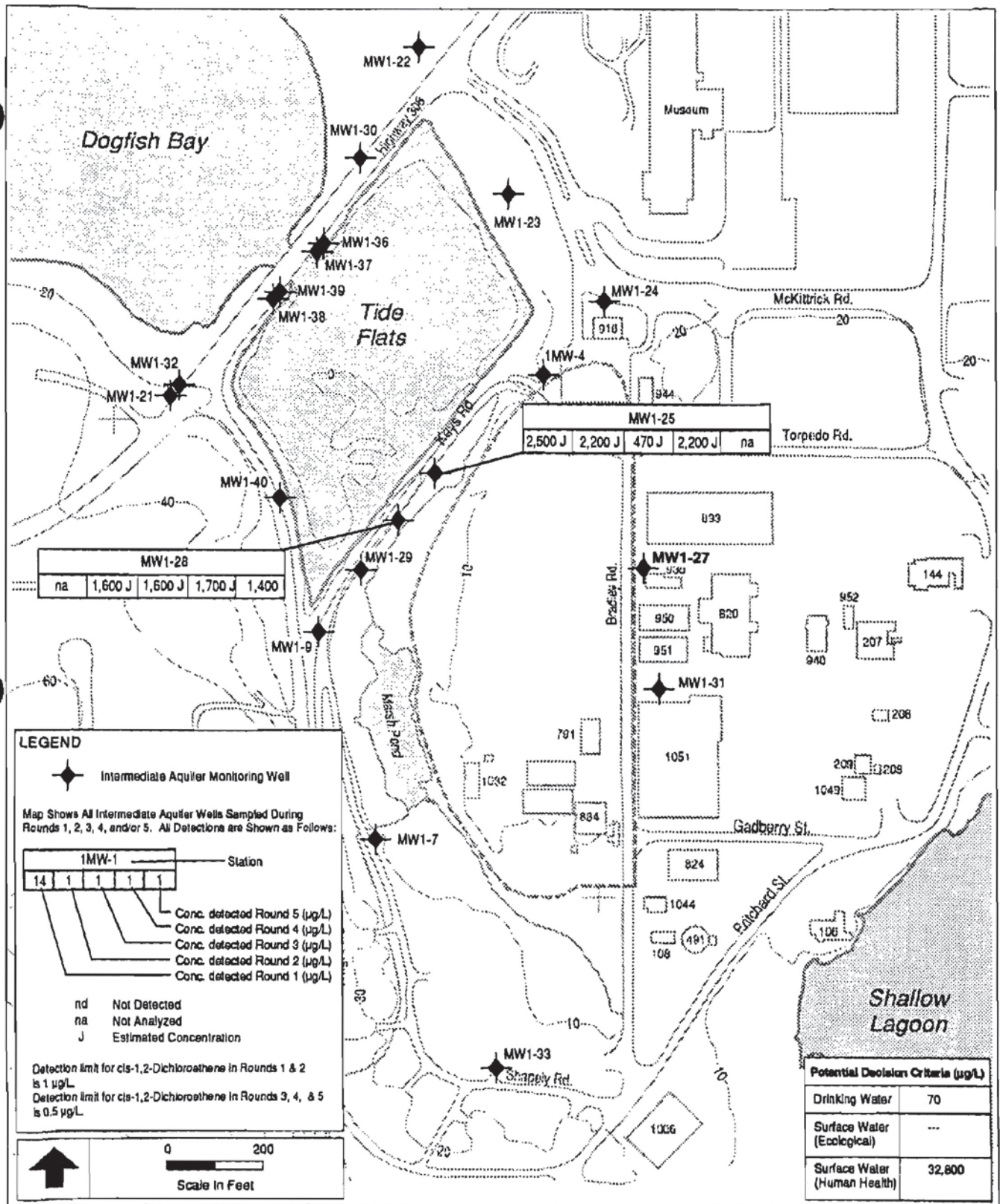
Figure 13 Distribution of cis-1,2-Dichloroethene in Intermediate Aquifer
