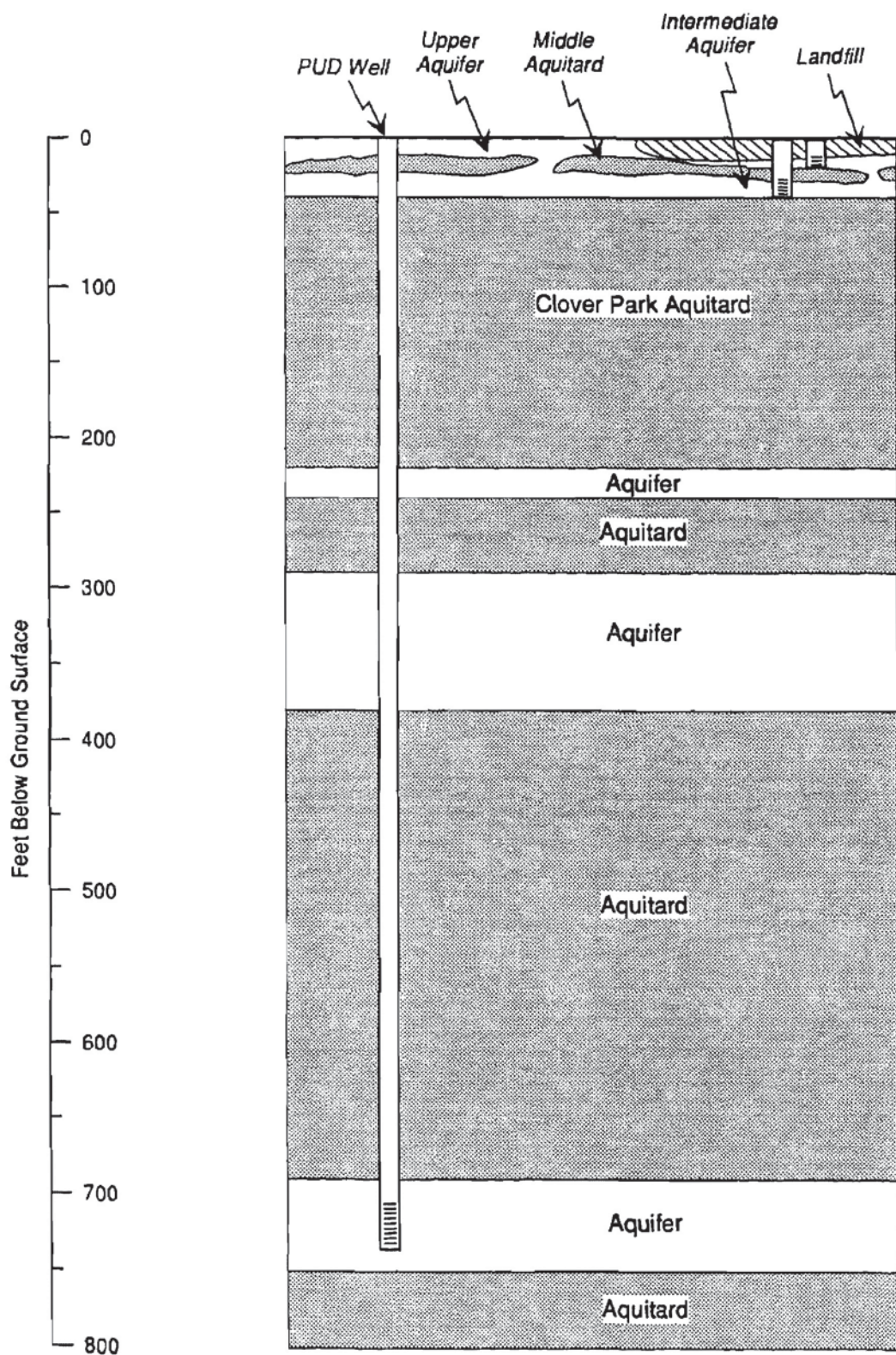
Figure 3 Generalized Hydrostratigraphy in Vicinity of OU 1
