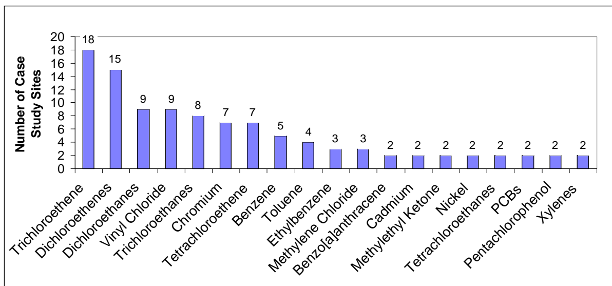
Exhibit 2-5: Specific Contaminants Treated at 28 Sites
