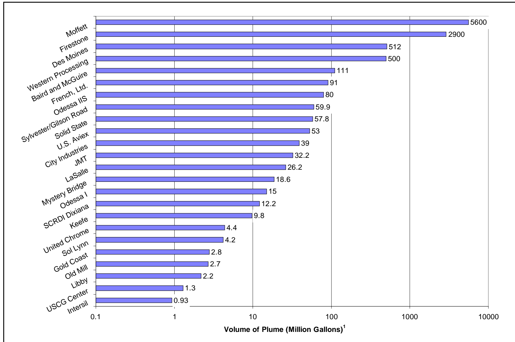
Exhibit 2-6: Initial Volume of Contaminated Groundwater Plumes at 24 Sites 1
