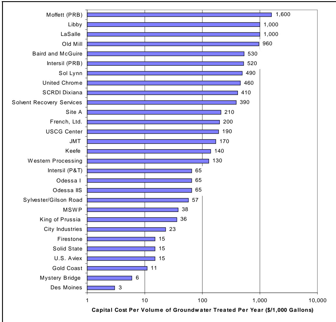
Exhibit 5-4: Capital Cost Per 1,000 Gallons of Groundwater Treated Per Year
