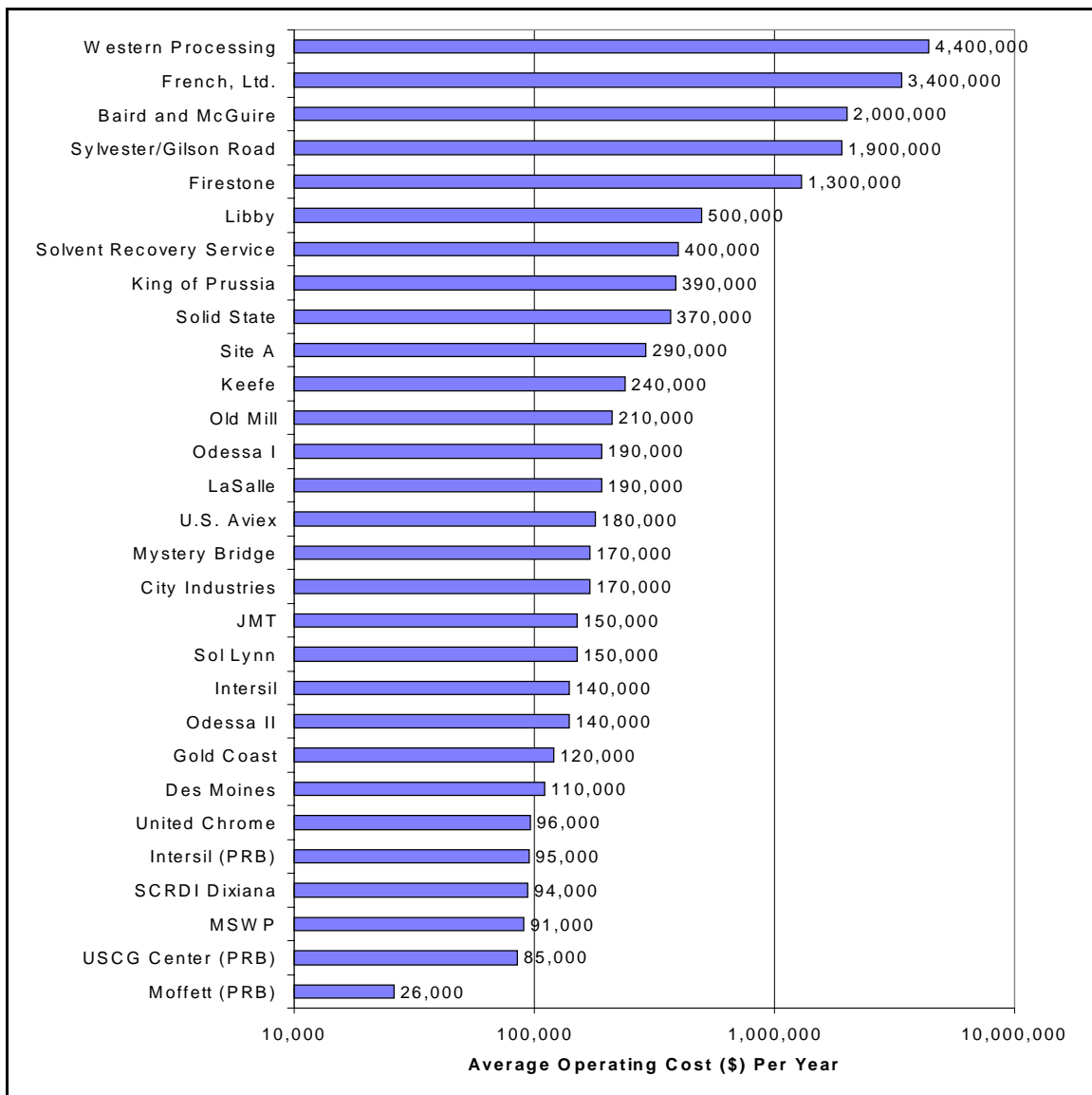
Exhibit 5-3: Average Operating Cost Per Year at 28 Sites
