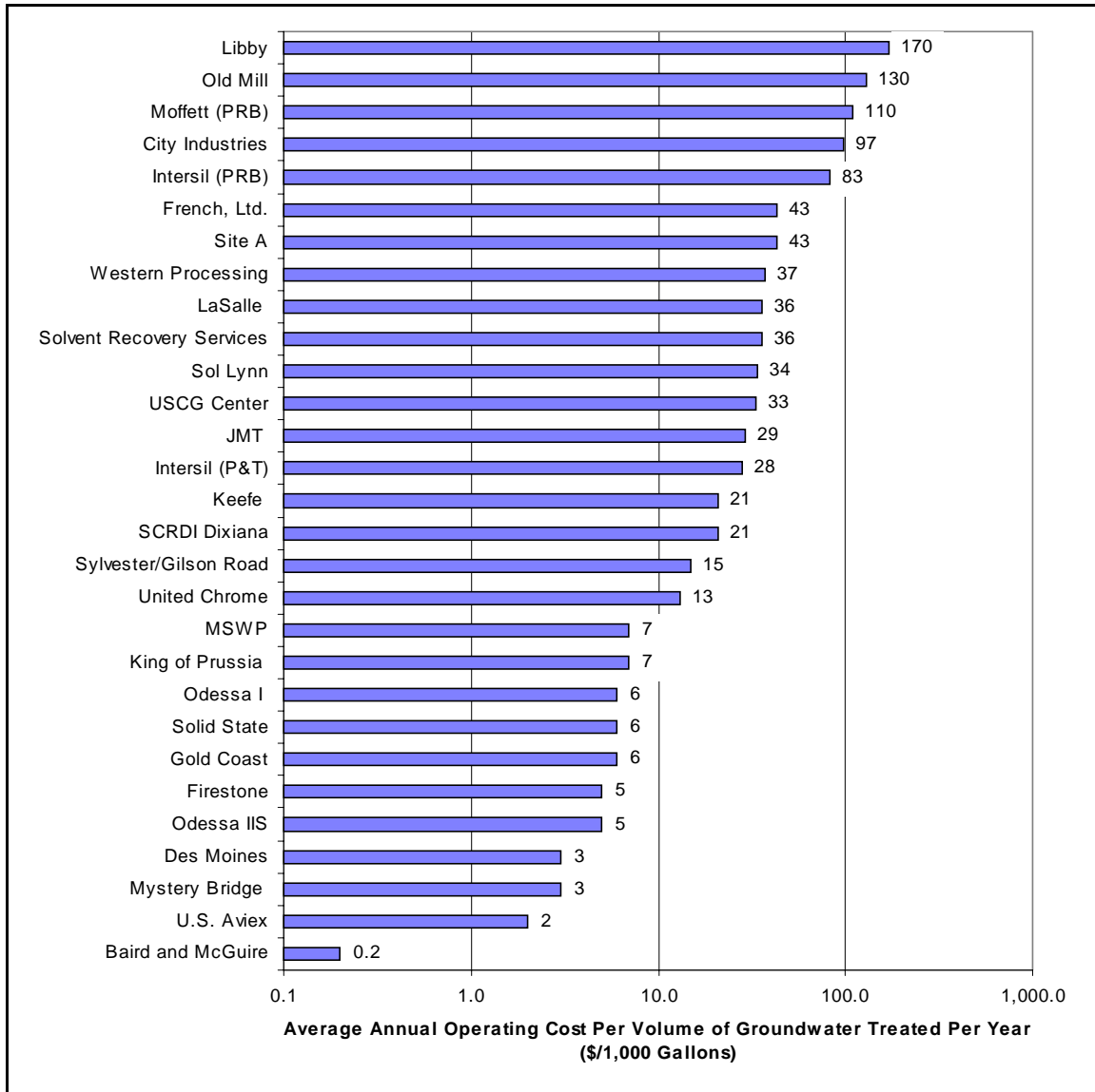
Exhibit 5-5: Average Annual Operating Cost per 1,000 Gallons of Groundwater Treated Per Year
