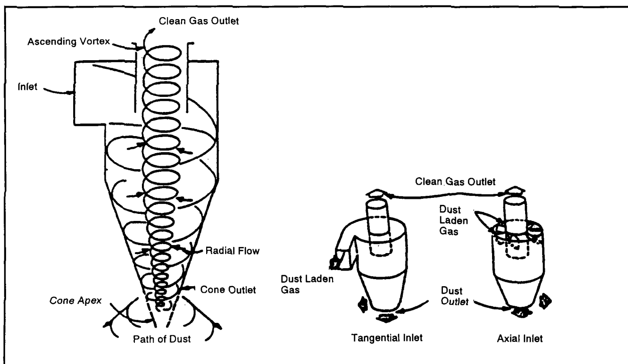
Figure 3: Typical Cyclone (adapted from EPA-530-R-94-014)
