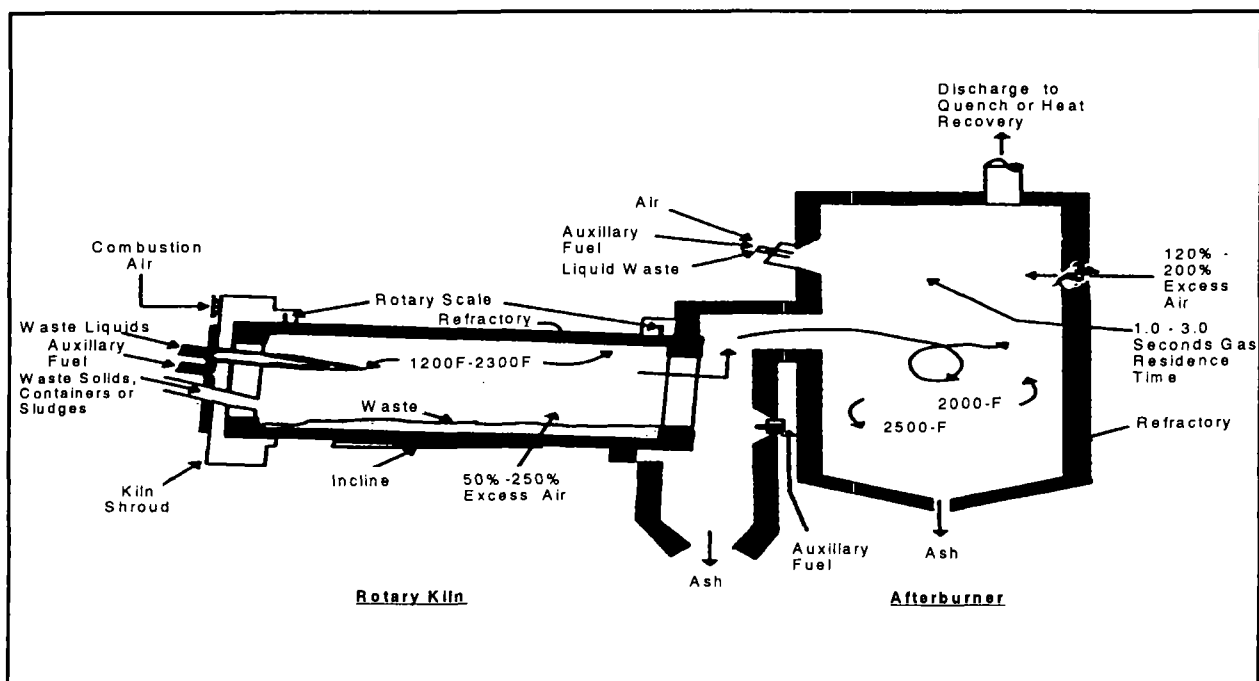
Figure 1 : Typical Rotary Kiln Incinerator (adapted from EPA-530-R-94-014)
