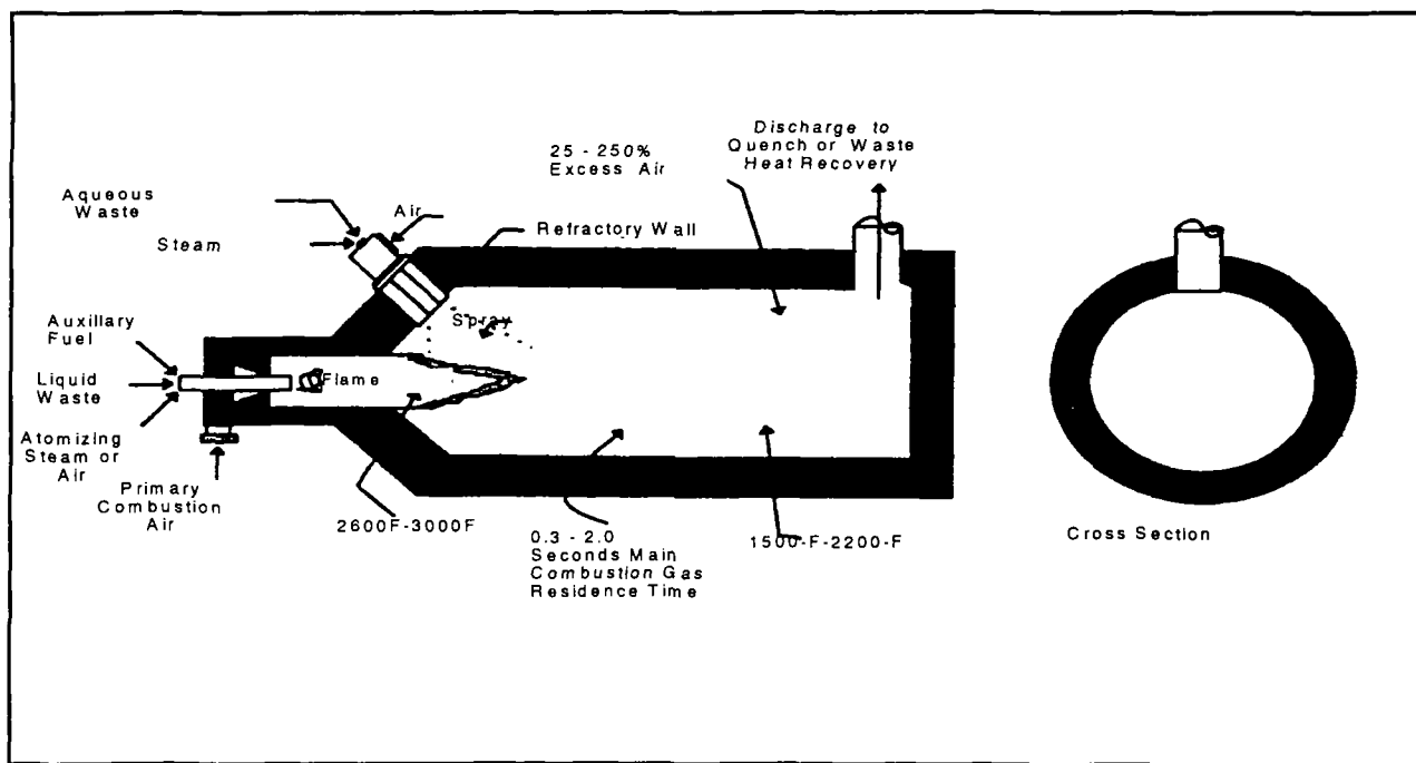
Figure 2: Typical Liquid Injection Incinerator (adapted from EPA-530-R-94-014)
