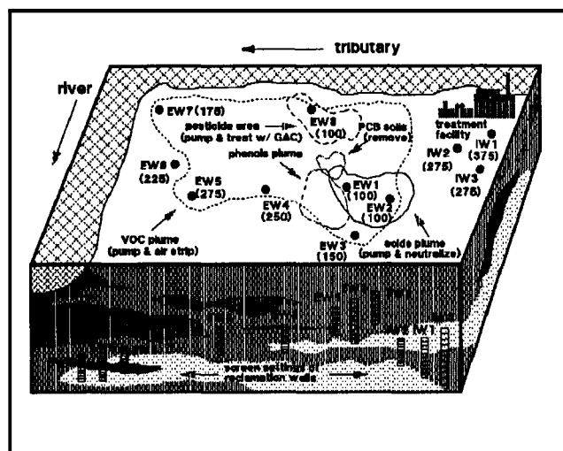
Figure 23. Moderate state-of-the-art remediation. Clusters of vertically-separated monitoring wells and an aquifer test are used to tailor the remedy to the site hydrogeology.
