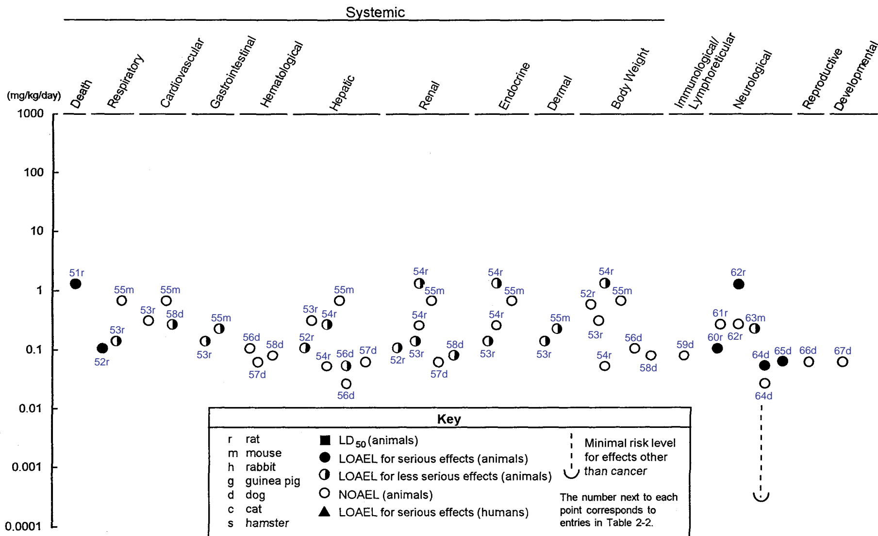
Figure 2-2. Levels of Significant Exposure to Endrin/Endrin Aldehyde - Oral (continued) Chronic ( \geq 365 days)
