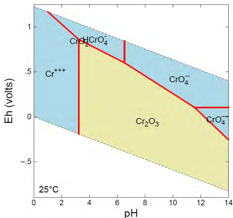
Figure 6-1. Pourbaix diagram for chromium. Prepared using Geochemist's Workbench Essentials version 8. Temperature = 25°C, Pressure = 1.013 bars, Chromium activity = 10 -6 .
