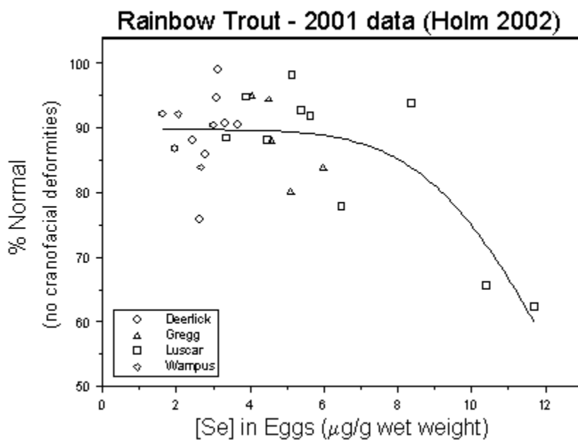
Holm Figure 5. Plot of percent normal (100 - percent total deformities) against selenium concentration in rainbow trout eggs ww, 2001 data. EC_{20} value at 10.4 \mu\text{g Se/g} egg ww.
