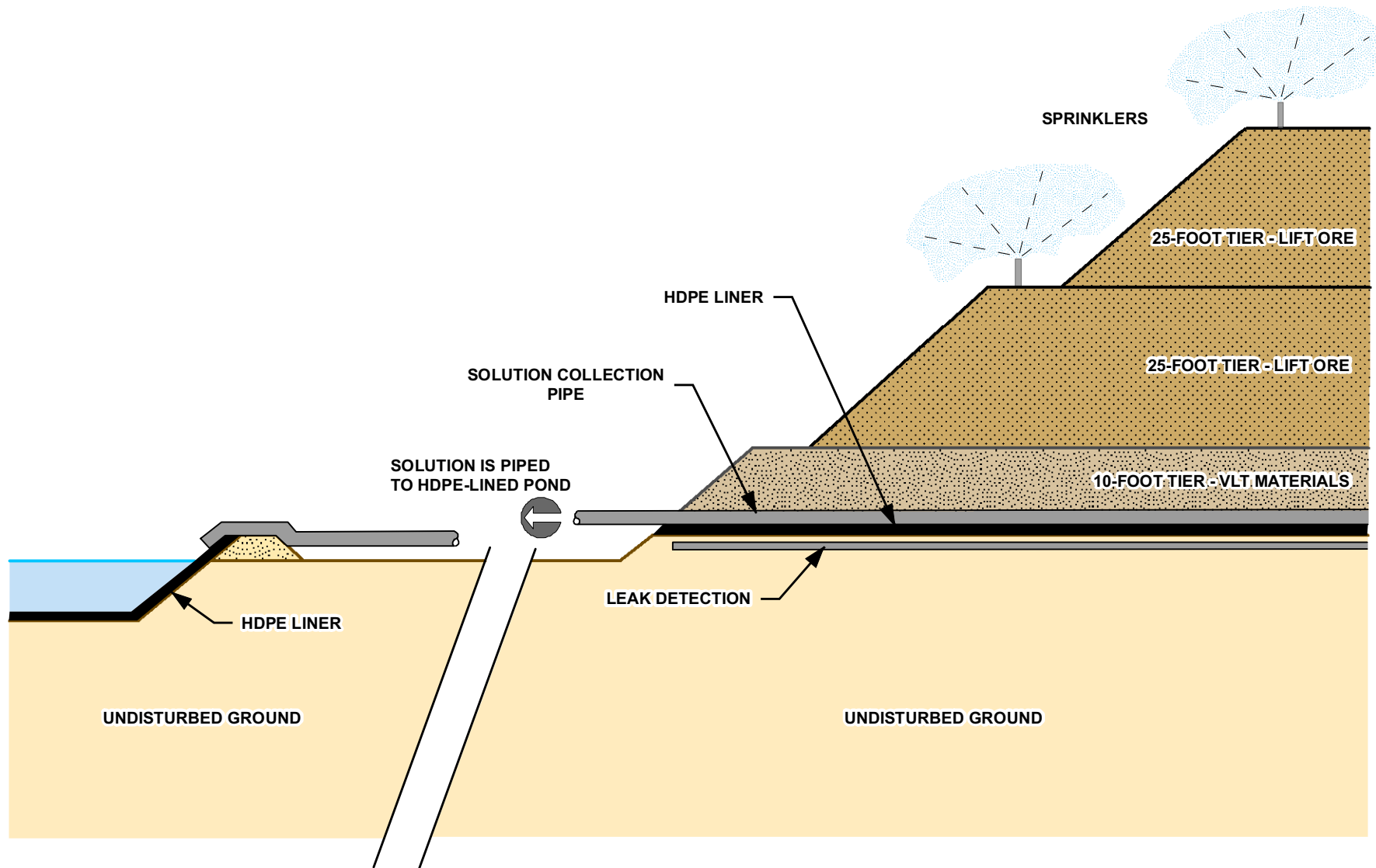
FIGURE 5-1 CONCEPTUAL ARIMETCO HEAP LEACH PAD CONDITIONS ANACONDA COPPER YERINGTON MINE
