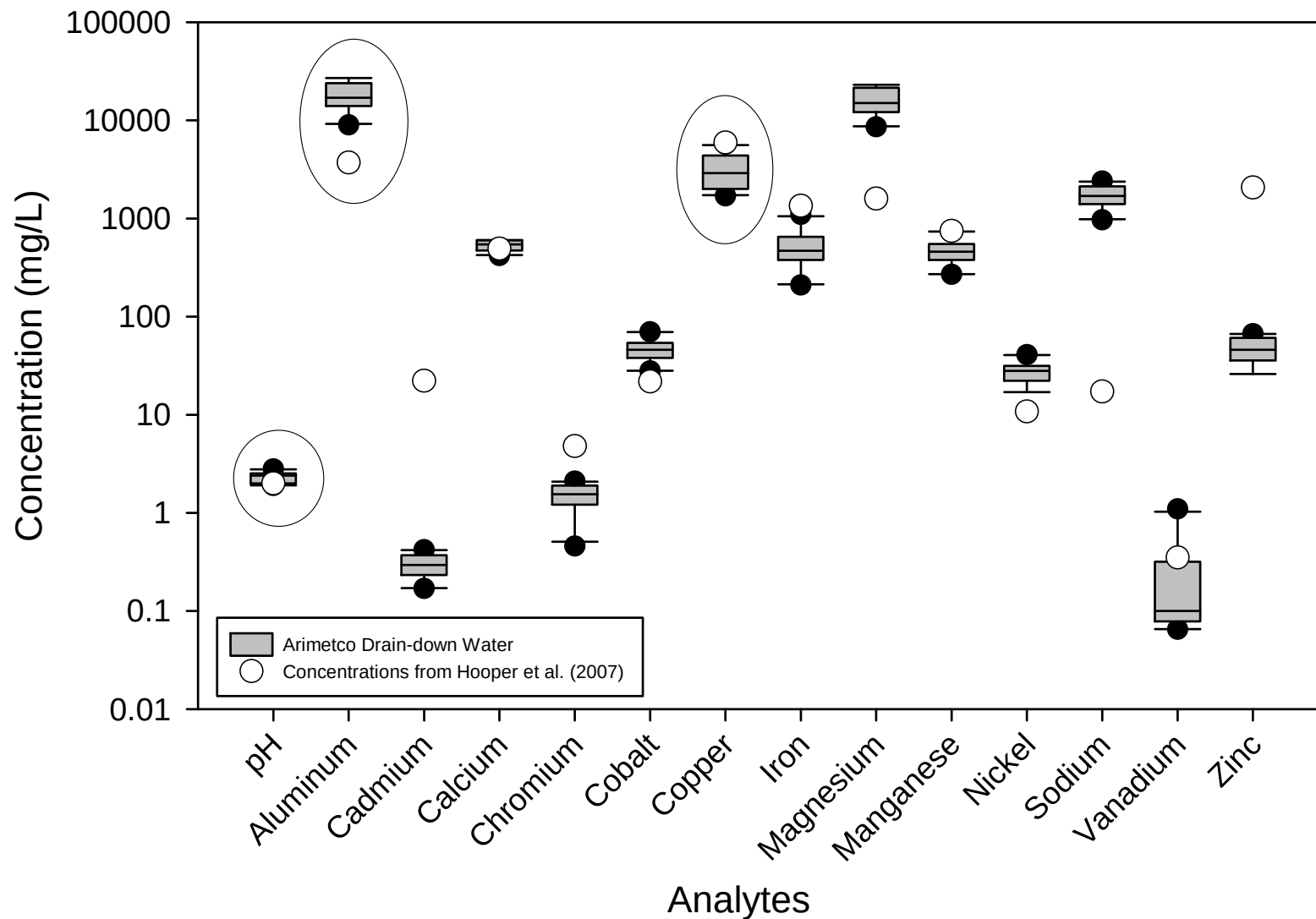
Figure 4-1. Comparison of analyte concentrations in drain-down water from Arimetco heap leach pads and synthetic acid-mine water used by Hooper et al. (2007) to evaluate acute toxicity to mallard ducks.
