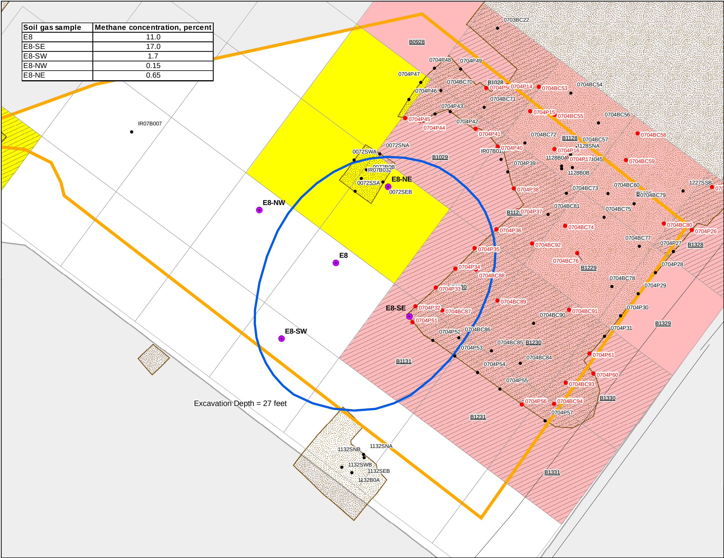
FIGURE 9-4 EXCAVATION AREA FOR METHANE SOURCE REMOVAL
