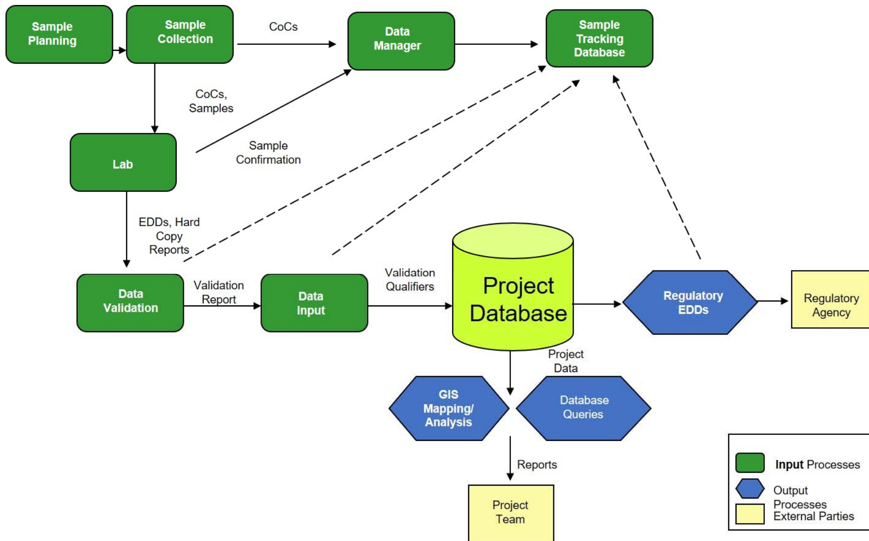
FIGURE 5.1 DATA MANAGEMENT FLOW DIAGRAM FOR LABORATORY ANALYTICAL DATA
