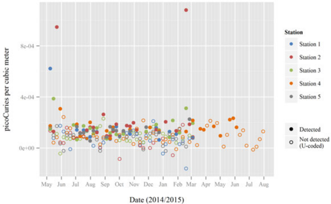
TIME SERIES PLOT OF URANIUM-238
