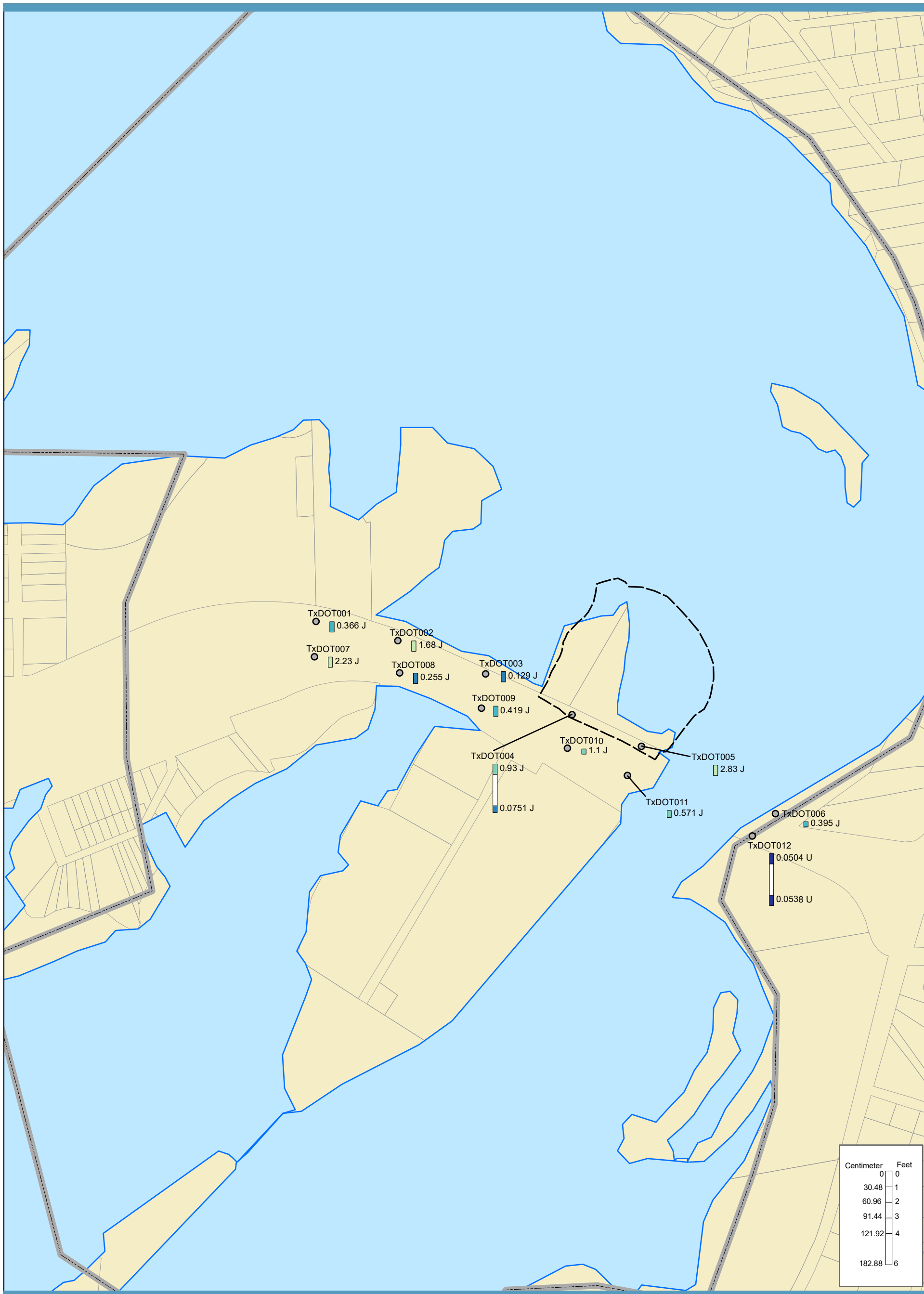
Figure 18 Distribution of TEQ P,M (ND = 1/2 DL) in Soils of the TxDOT Right-of-Way San Jacinto River Waste Pits Site
