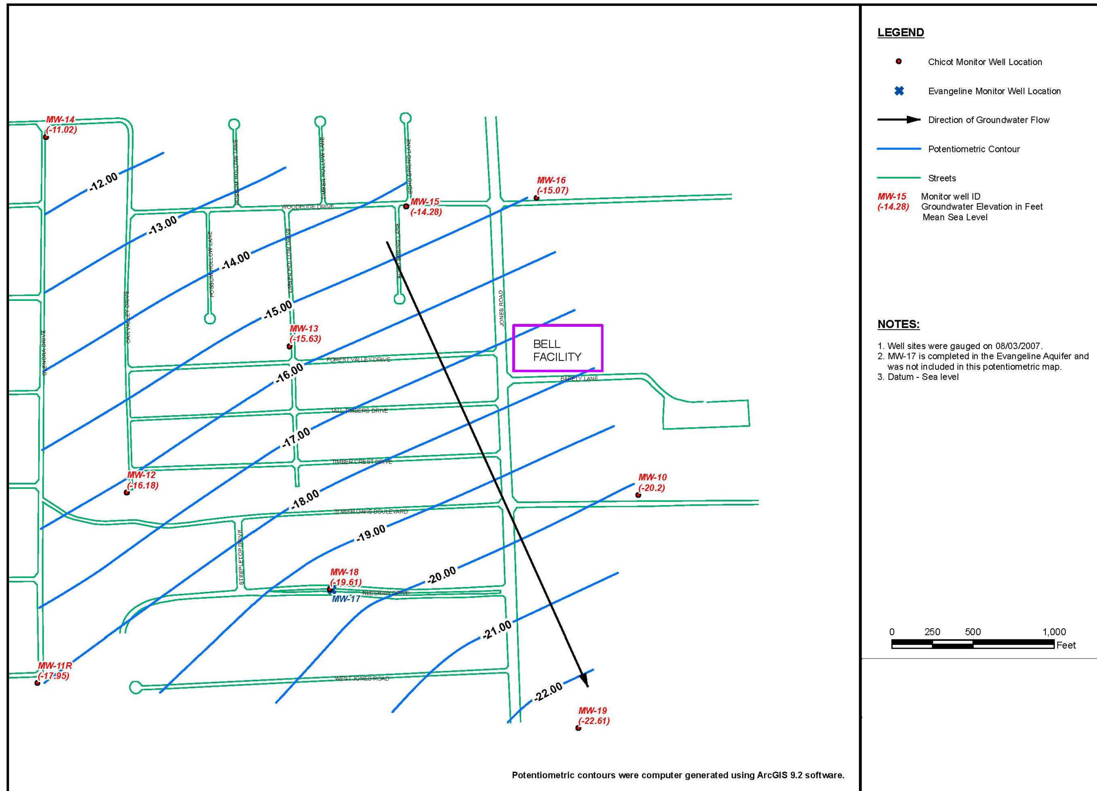
Figure 6 – Potentiometric Surface Map, Deep Groundwater Zone
