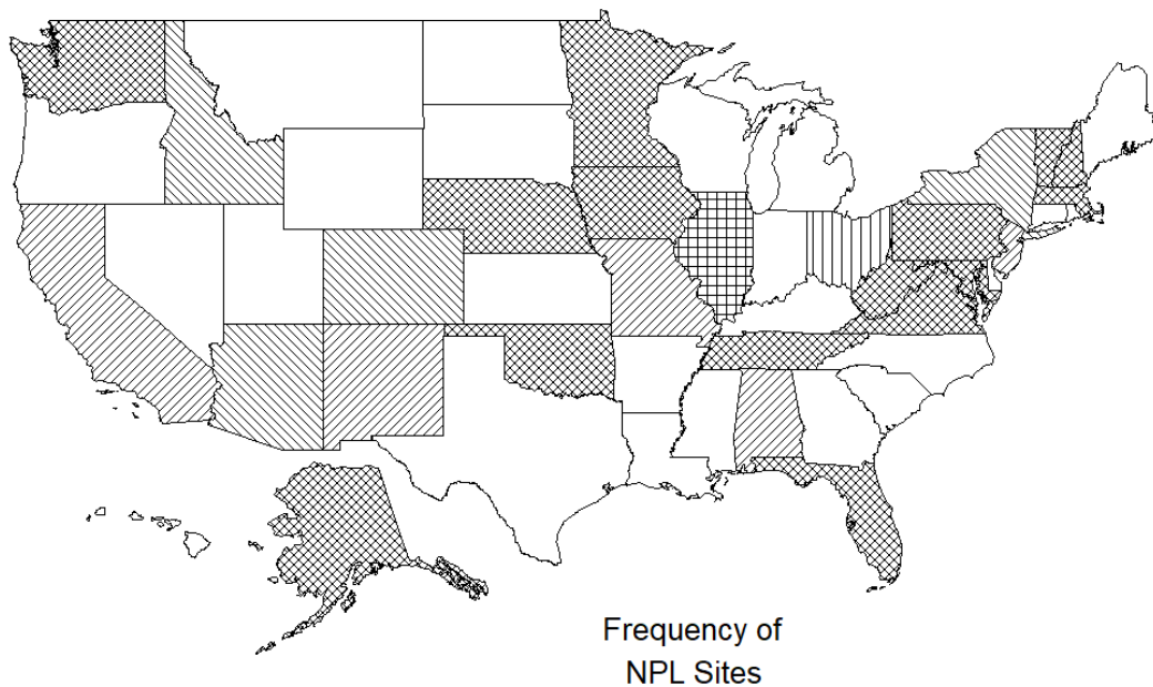
Figure 5-2. Number of NPL Sites with Lead Compound Contamination
