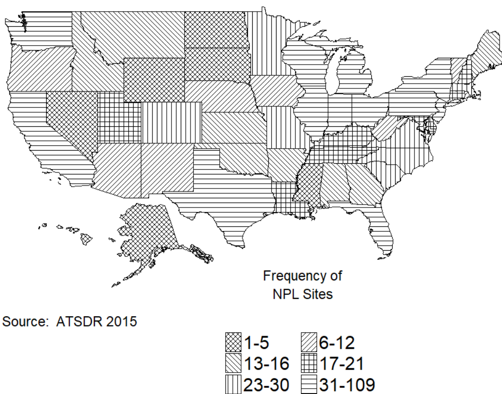
Figure 5-1. Number of NPL Sites with Lead Contamination
