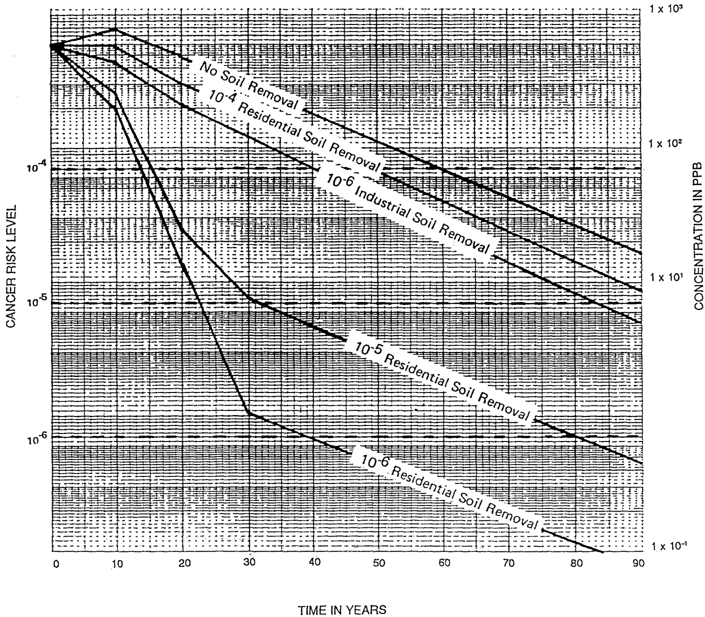
Figure 4-7. Time to achieve 10^{-4} to 10^{-6} risk level for a single-contaminant for ground water cleanup under various soil removal alternatives.
