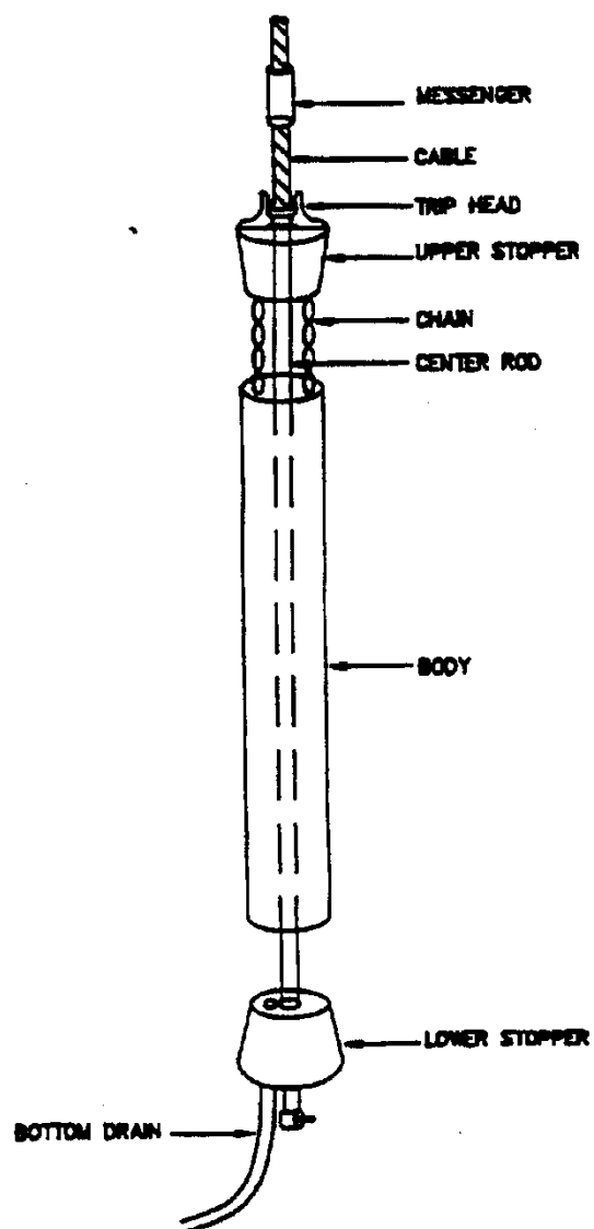
FIGURE 3 KEMMERER SAMPLER
