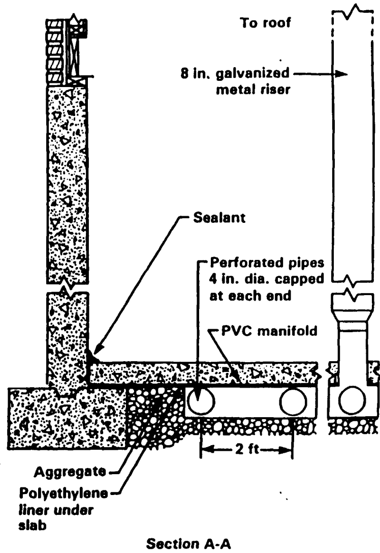
Figure 2-12. Passive Sub-slab Ventilation System
