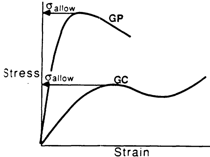
Figure 3-6. Crush strength of geopipe and geocomposite edge drain cores.
