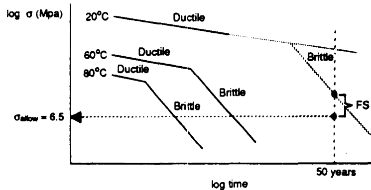
Figure 4-3. Rate process method for testing pipe.
