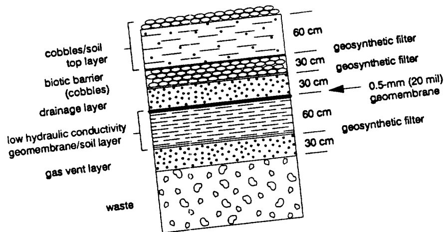
Figure 1-2. EPA-recommended landfill cover with options (1).
