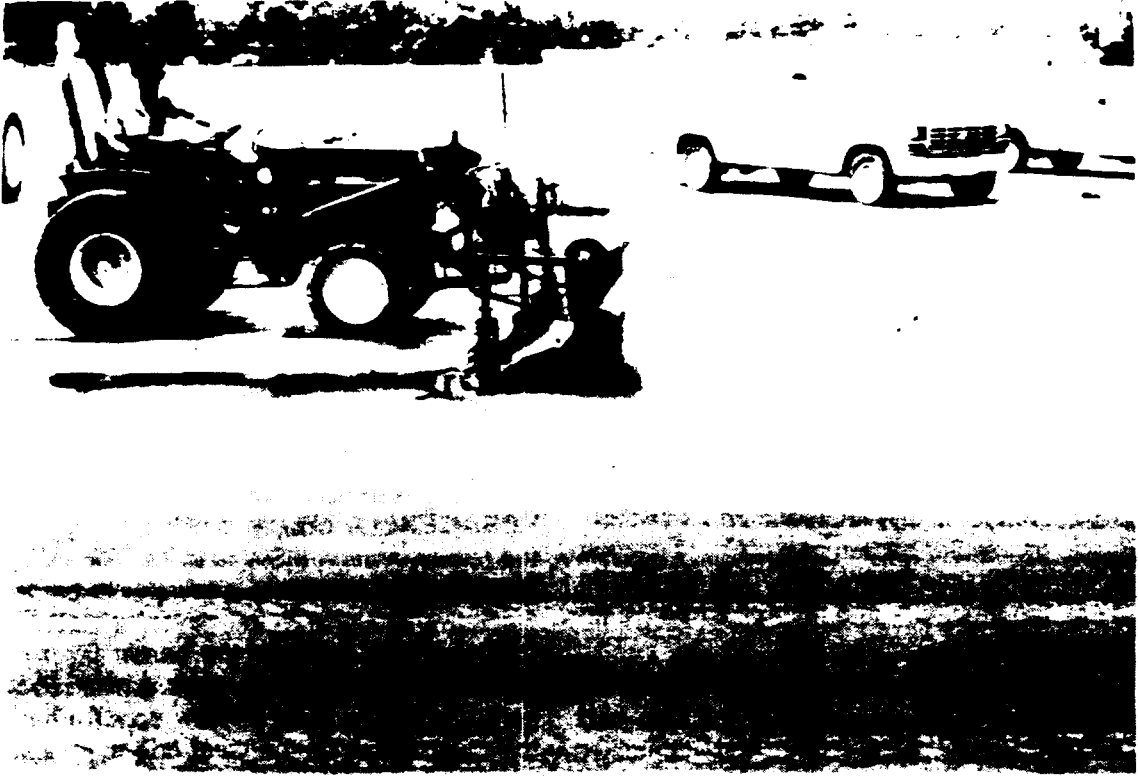
Figure 11-17a. Case 4—Placement of geotextile on asphalt emulsion.
