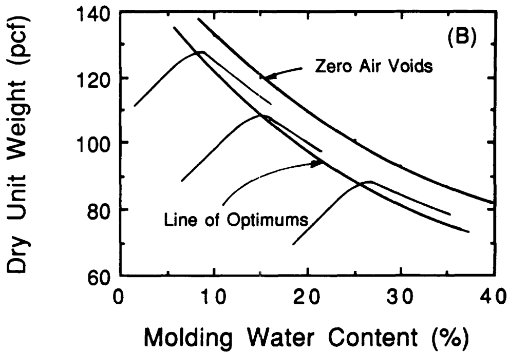
Figure 6-7. Possible approaches for specifying lower limit of Acceptable Zone: (A) minimum degree of saturation, S; and (B) line of optimums (5).
