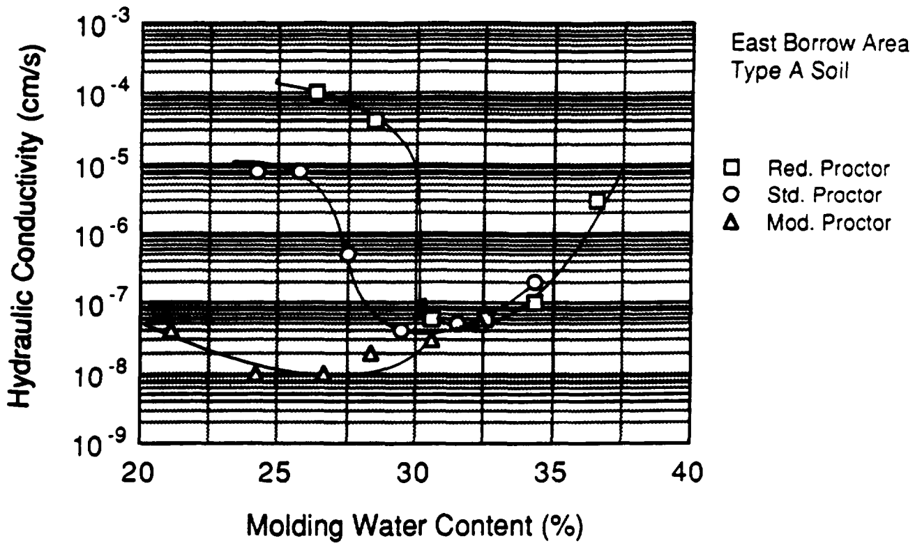
Figure 6-9. Hydraulic conductivity versus molding water content for Type A soil from East Borrow area at Oak Ridge Y-12 operations project (5).
