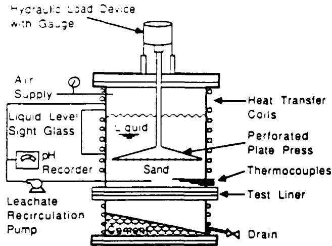
Figure 4-4. Rate process method for testing geomembranes.
