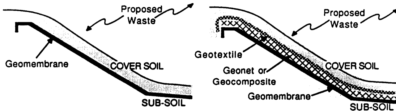
(c) Landfill Liner with Soil Above Geomembrane
