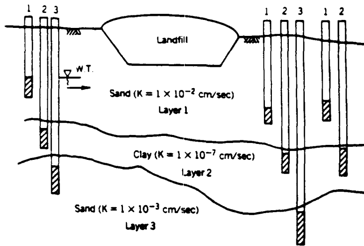
Figure 12-1. Monitoring well configuration.
