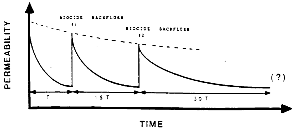
Figure 12-3. Impact of biological growth on filters.
