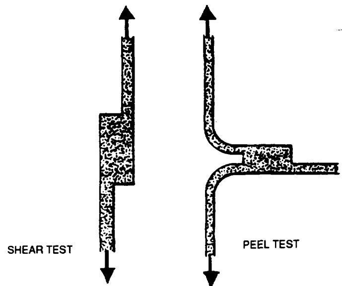
Figure 7-1. Shear and peel test for geomembrane seams.
