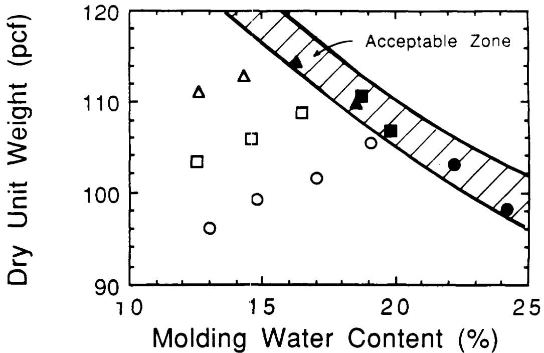
Figure 6-3. Compaction data for silty clay (6); solid symbols represent specimens with hydraulic conductivity less than or equal to 1 \times 10^{-7} cm/s and open symbols represent specimens with hydraulic conductivity > 1 \times 10^{-7} cm/s.
