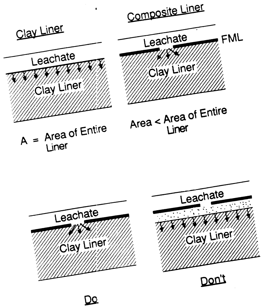
Figure 2-2. Soil liner and composite liner.
