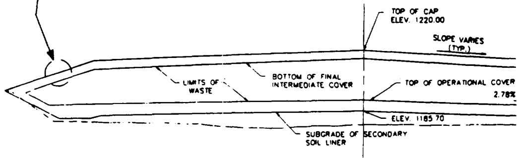
Figure 11-9. Case 2—Cap profile and geometry.
