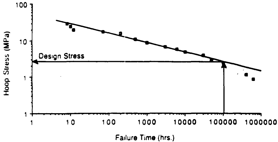
Figure 4-2. Stress limit testing for plastic pipe.
