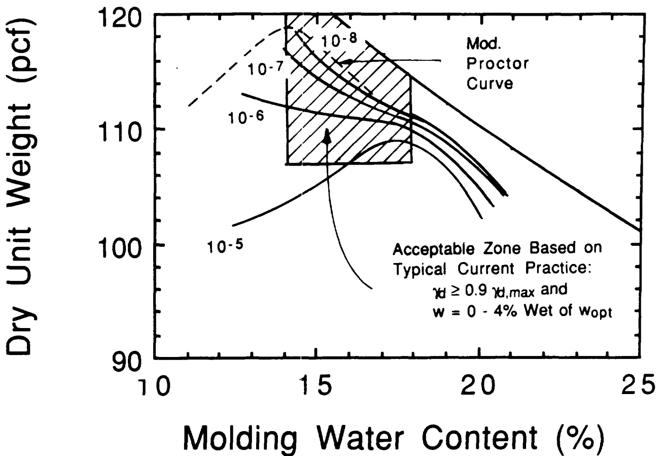
Figure 6-4. Contours of constant hydraulic conductivity for silty clay compacted with kneading compaction (6).
