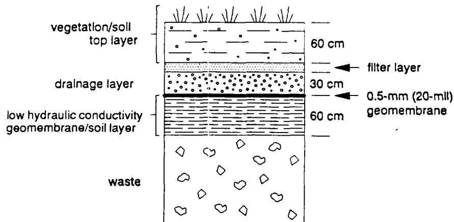
Figure 1-1. EPA-recommended landfill cover design (1).
