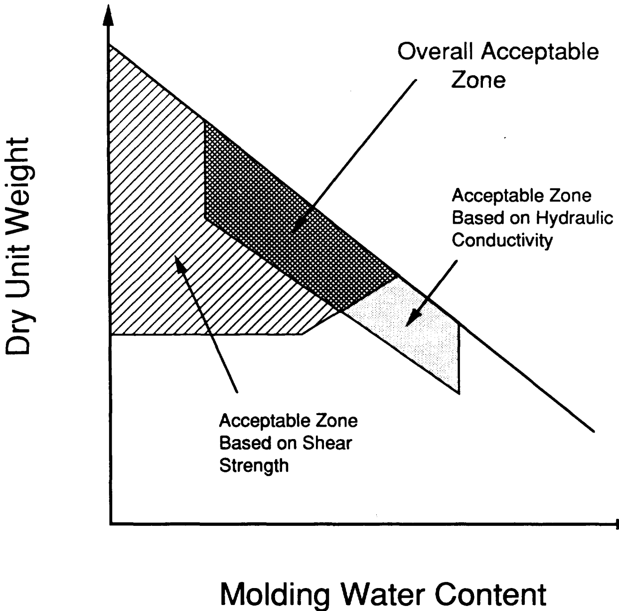
Figure 6-6. Use of hydraulic conductivity and shear strength data to define a single, overall acceptable zone (5).
