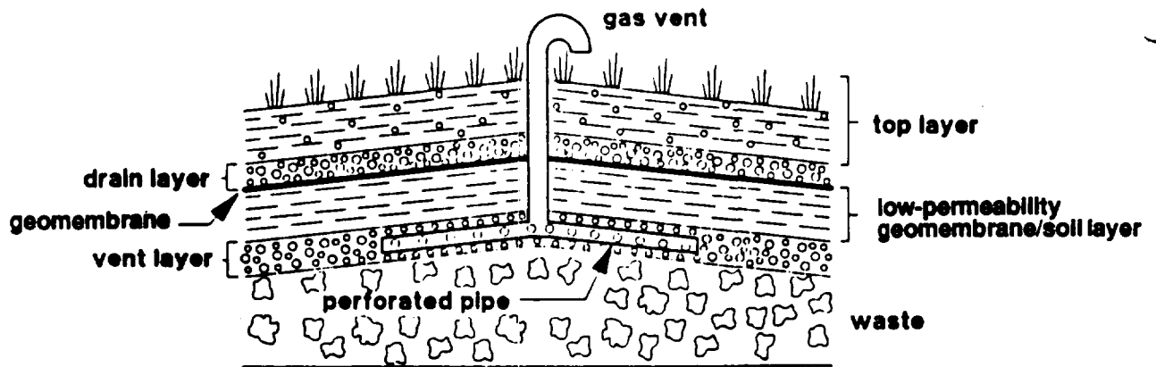
Figure 10-1. Cover with gas vent outlet and vent layer.
