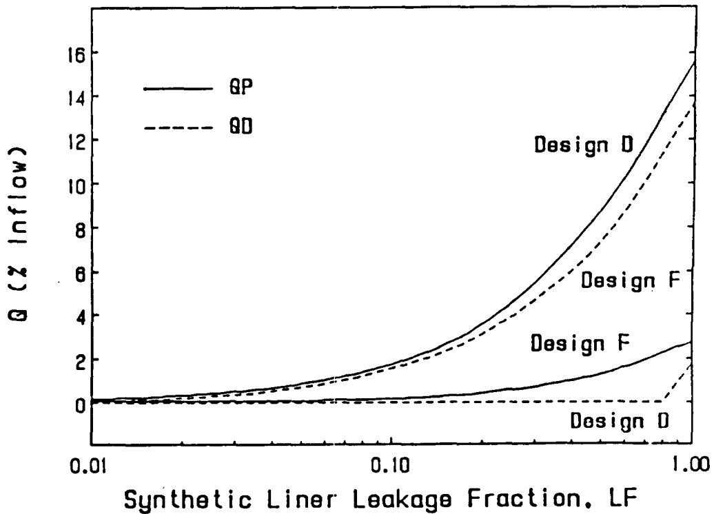
Figure 9-12. Percent of inflow to primary leachate collection layer discharging from leakage detection layer and bottom liner for double-liner systems D and F.
