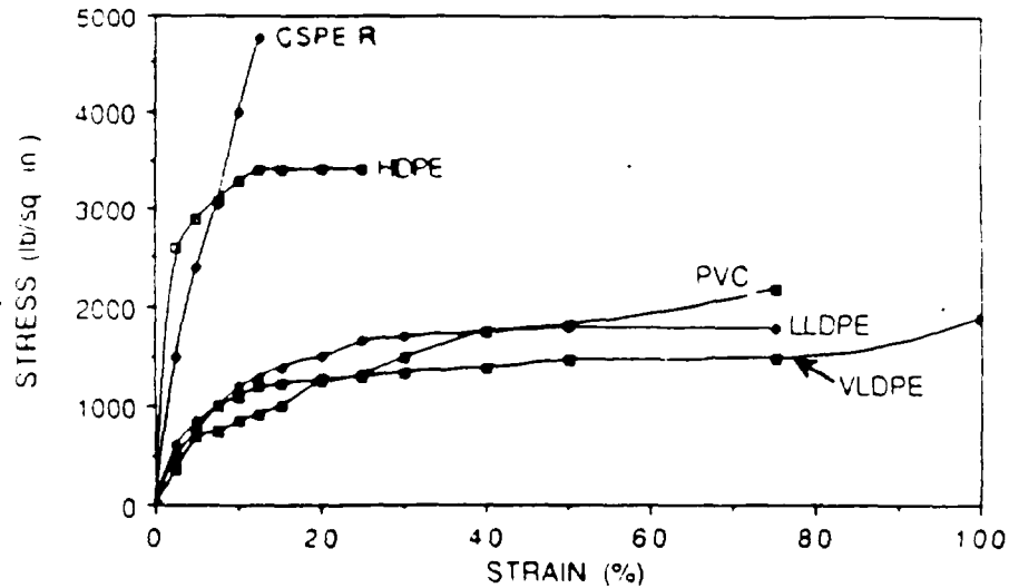
Figure 3-2. Response of common geomembranes to the three-dimensional geomembrane tension test.
