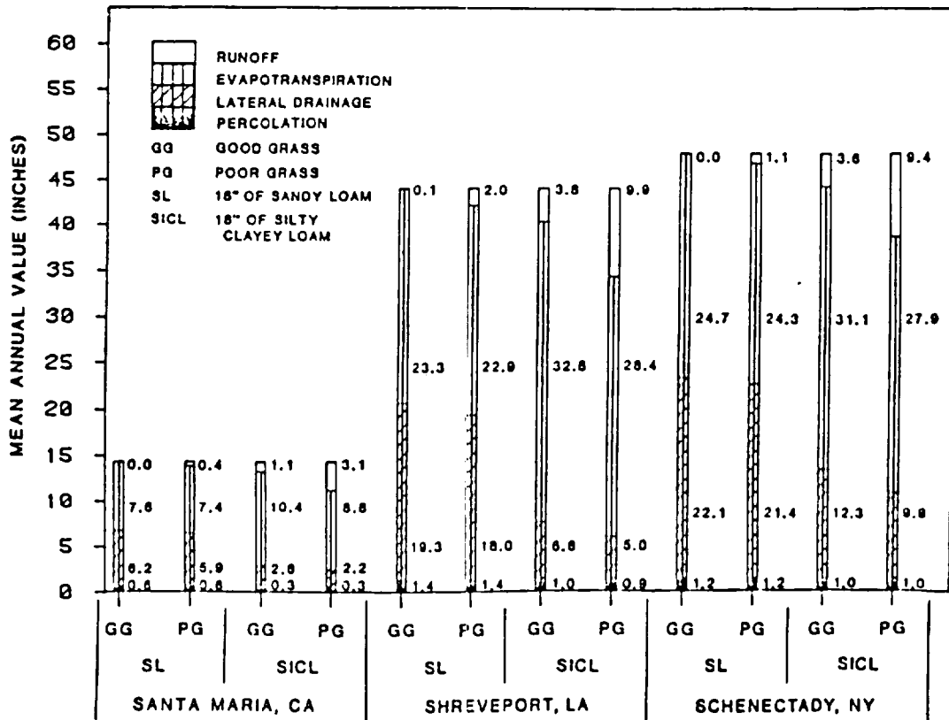
Figure 9-2. Bar graph for three-layer cover design showing effect of surface vegetation, topsoil type, and location.
