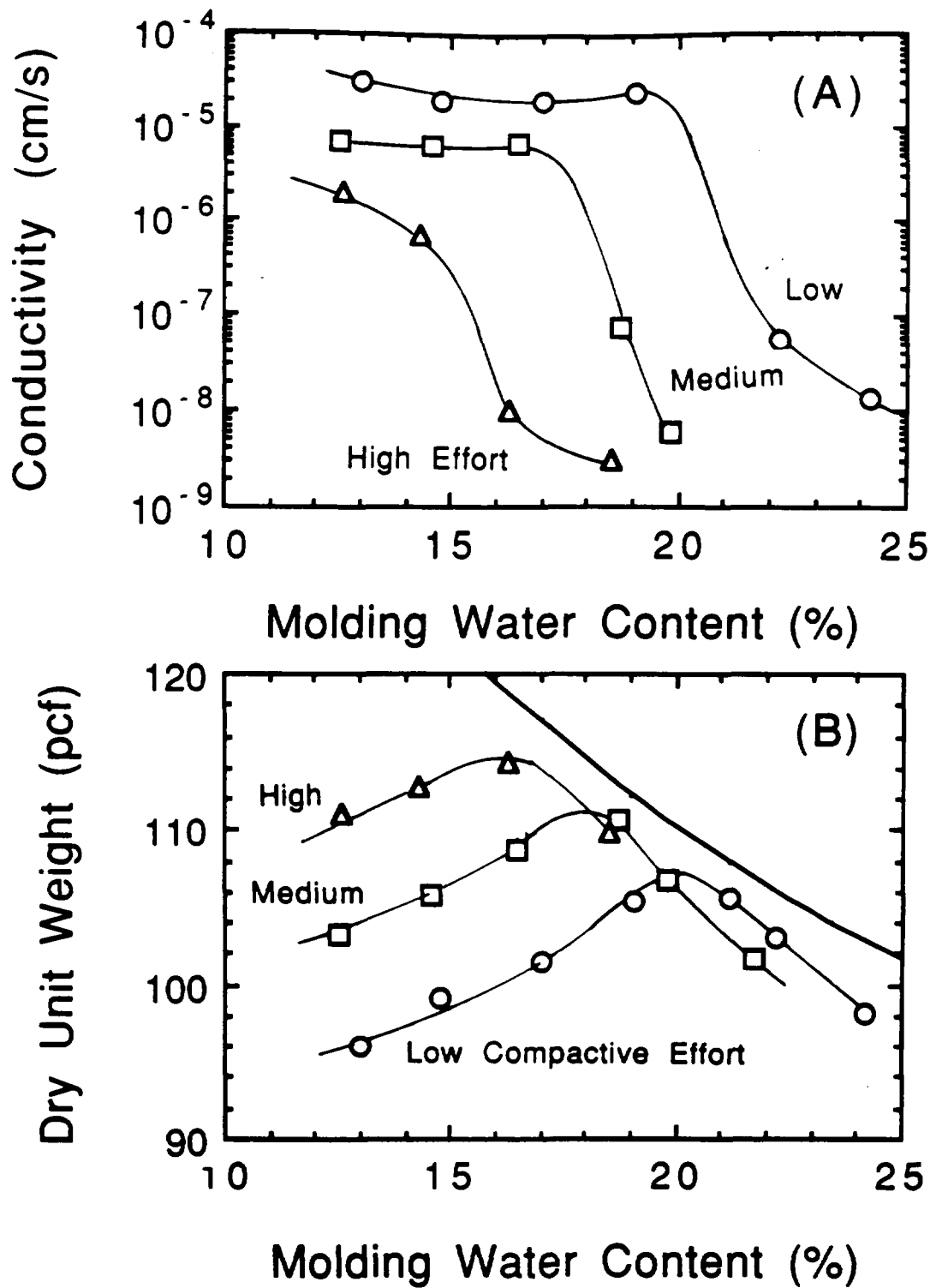
Figure 6-2. Data from Mitchell et al. for silty clay compacted with impact compaction (6).
