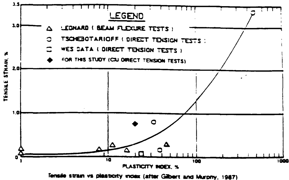
Figure 11-7. Case 1—Ultimate tensile strain in clays.
