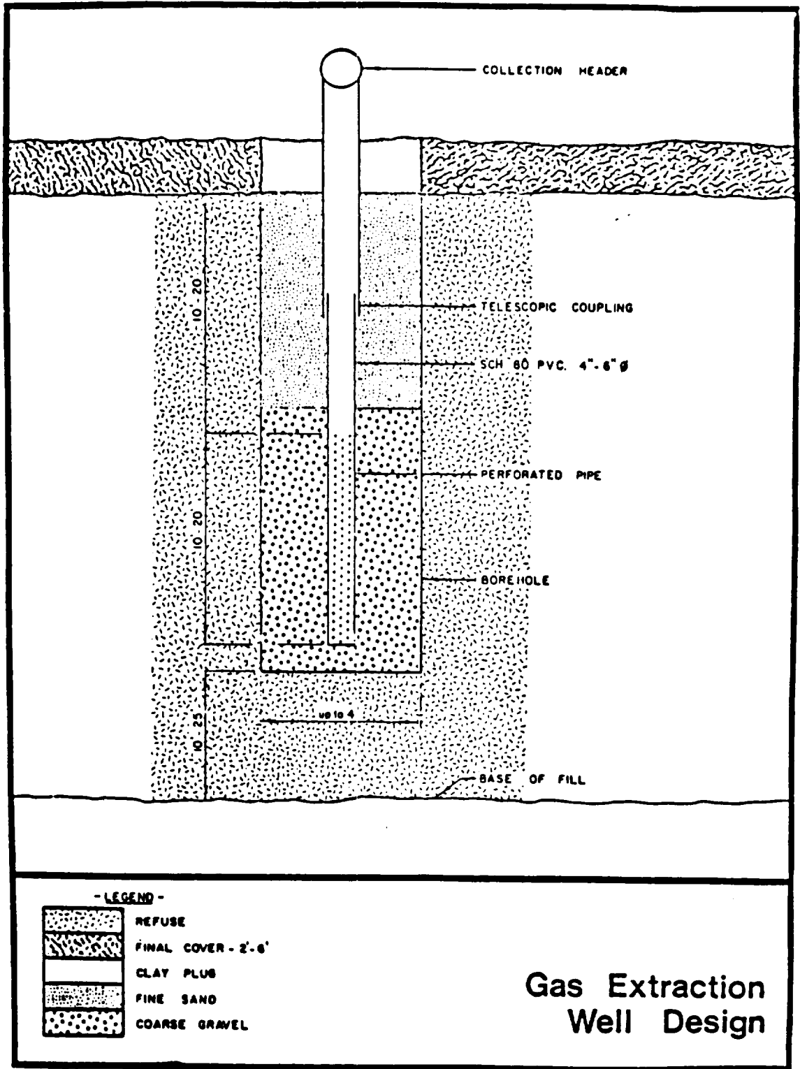
Figure 10-6. Gas extraction well design (6).
