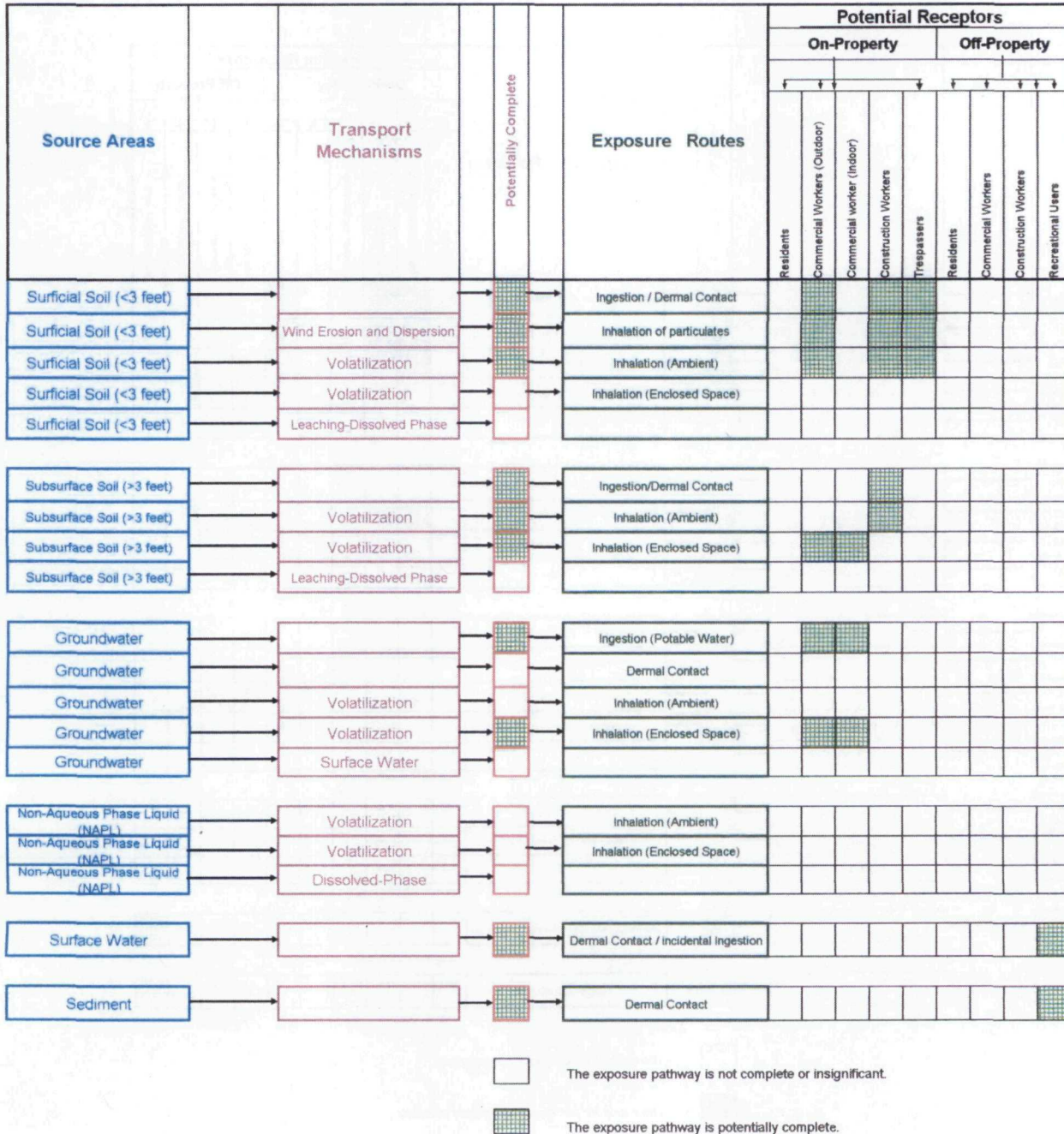
Figure 5 - Conceptual Site Model (cont.) Exposure Pathway Evaluation Flowchart - Future Land Use Honeywell Ironton Tar Plant Ironton, Ohio
