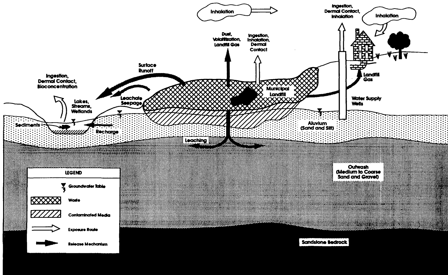
Figure 3-1 CONCEPTUAL SITE MODEL EXAMPLE LANDFILL SITE
