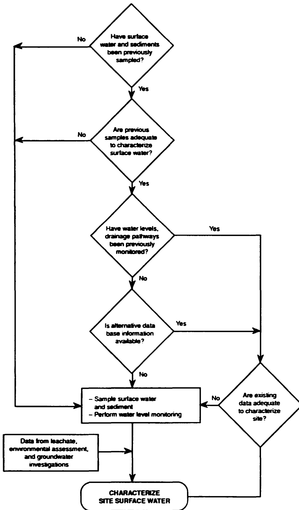
Figure 3-6 LOGIC DIAGRAM FOR SURFACE WATER/ SEDIMENT SAMPLING NEAR MUNICIPAL LANDFILL
