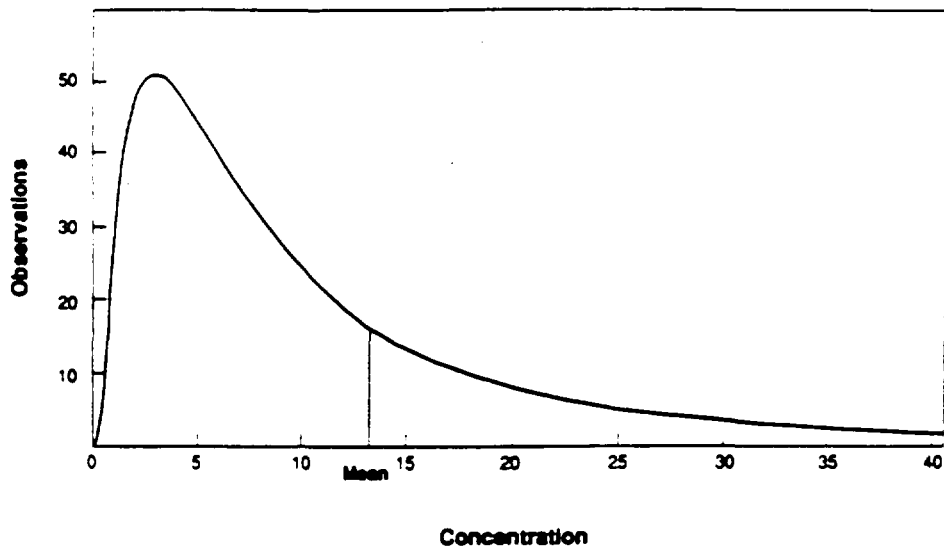
Highlight 3 EXAMPLE OF A LOGNORMAL DISTRIBUTION
