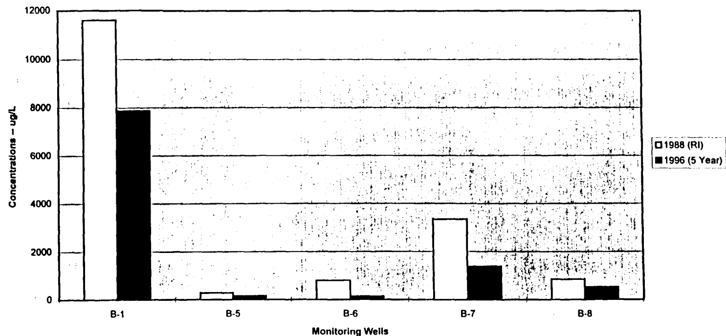
Manganese Concentration Trend In Monitoring Wells
