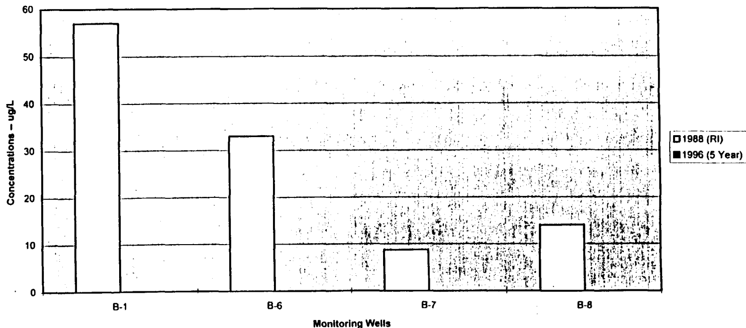
Vanadium Concentration Trend In Monitoring Wells
