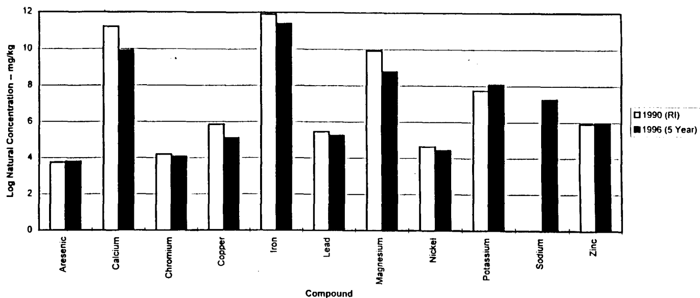
Inorganic Trend In Quarry Sediment
