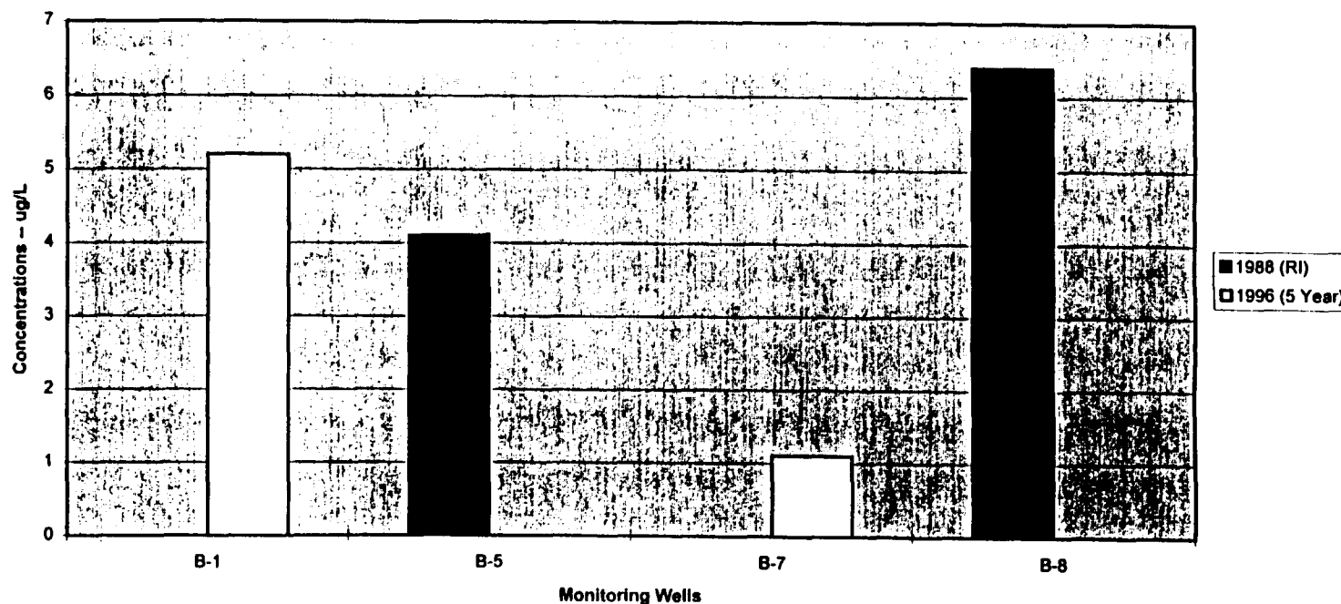
Cadmium Concentration Trend In Monitoring Wells
