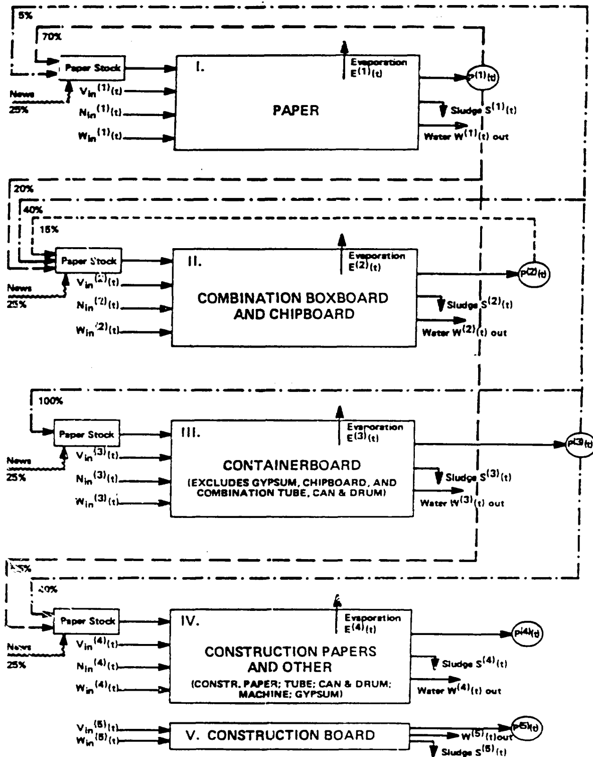
Figure 5-4. SCHEMATIC OF SECOND ORDER MODEL
