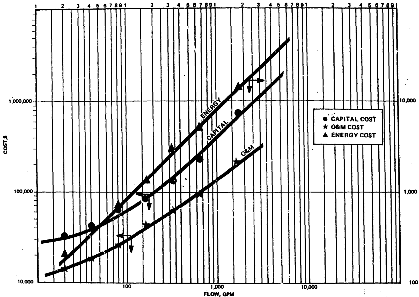
Figure 4-2. CARBON ABSORPTION WASTEWATER TREATMENT SYSTEM COSTS
