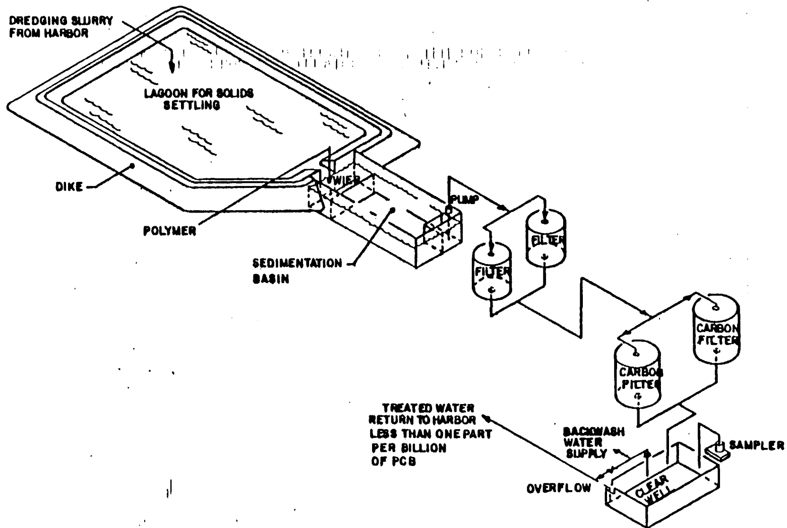
FIGURE V-4: PROPOSED TREATMENT SYSTEM FOR EXCESS WATER
