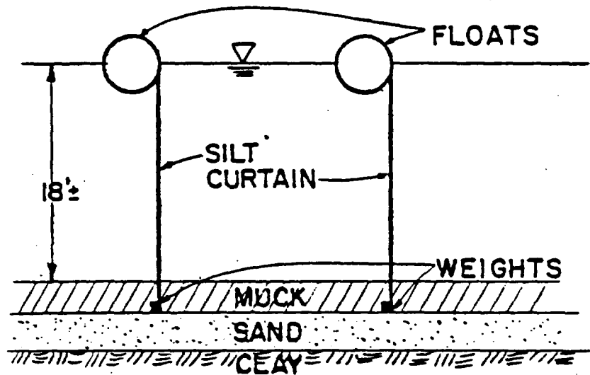
SECTION A-A ELEVATION OF DUAL CURTAIN
