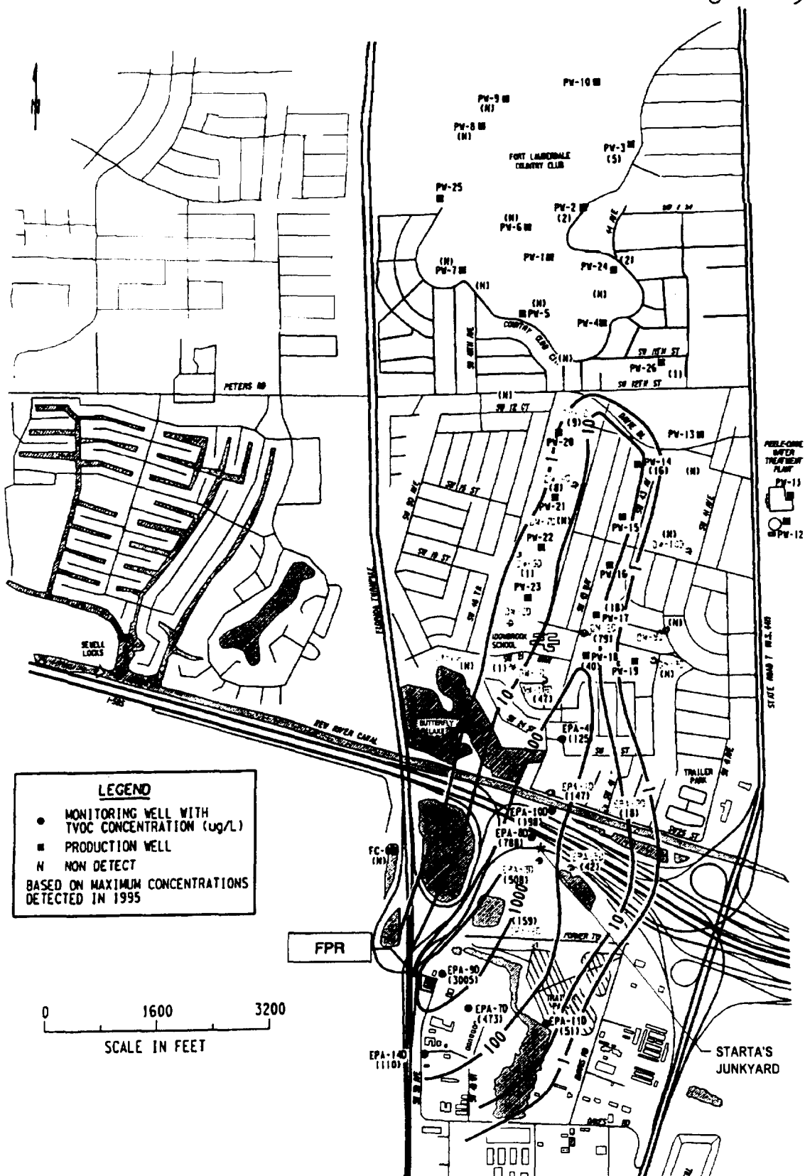
Figure 1-4 TVOC Plume in Deep Aquifer - 1995 Florida Petroleum Reprocessors, Davie, Florida
