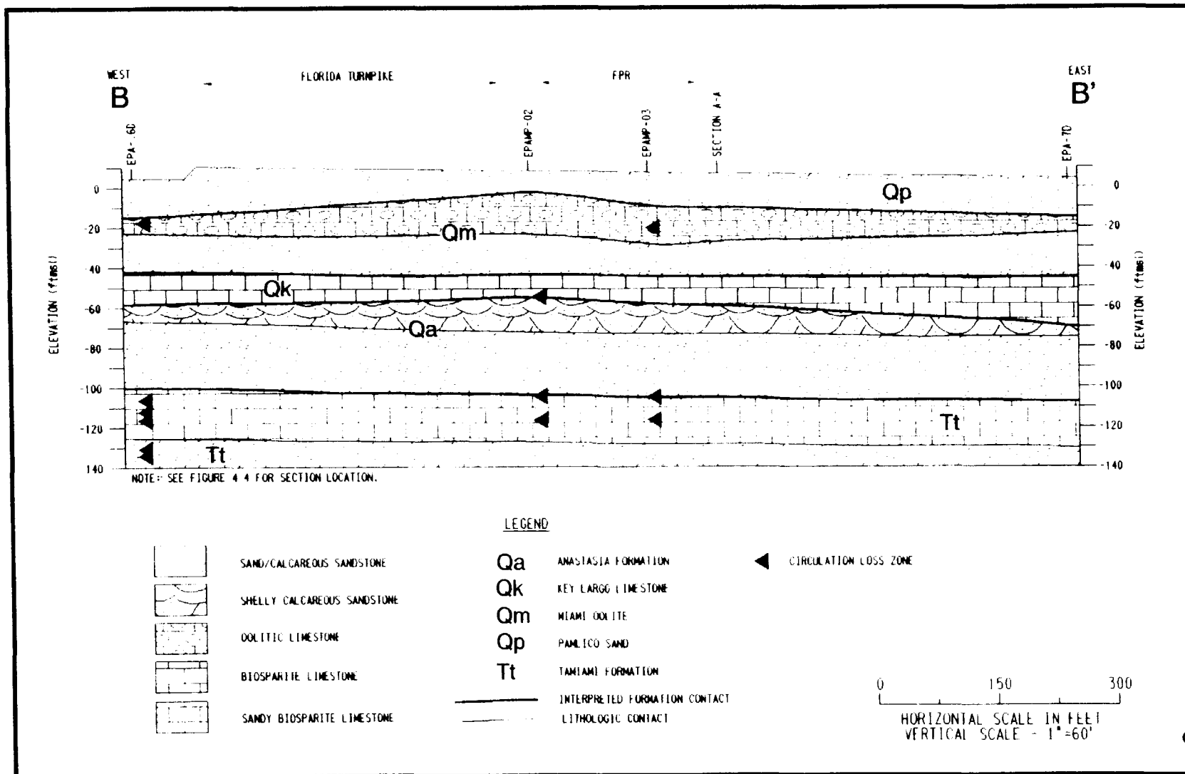
Figure 4-2 Generalized Geologic Cross-Section B-B' Florida Petroleum Reprocessors, Davie, Florida
