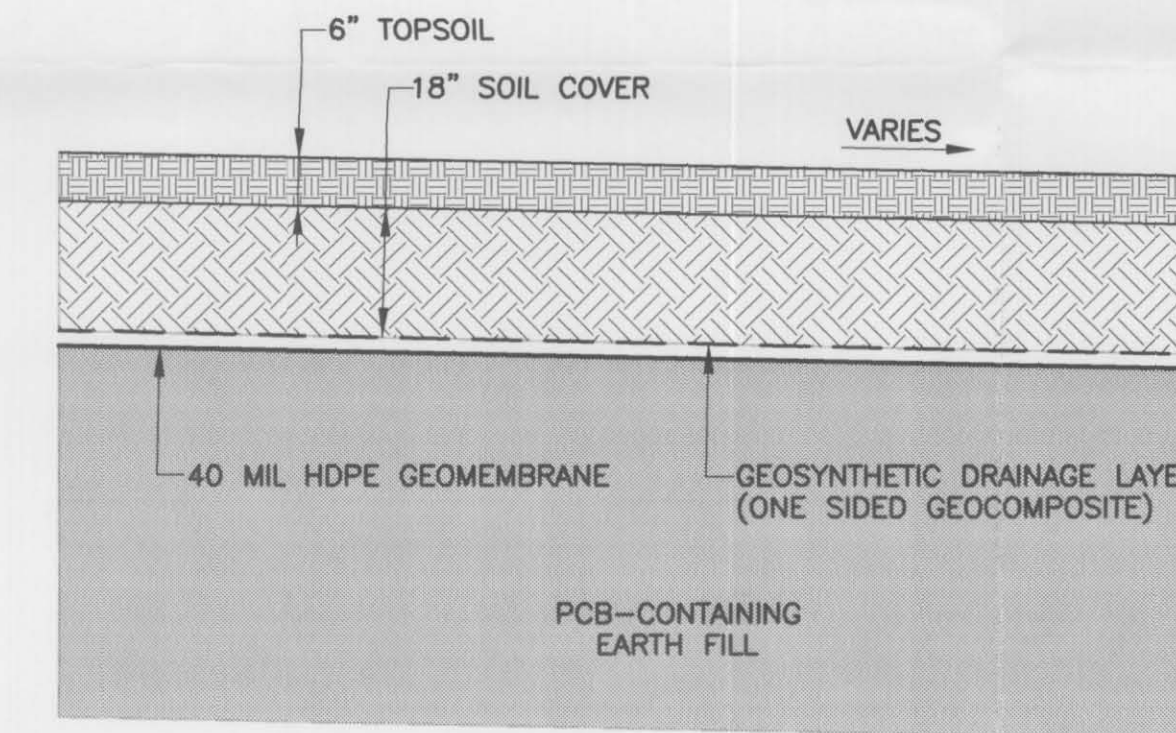
3 6 TYPICAL COVER SYSTEM DETAIL
