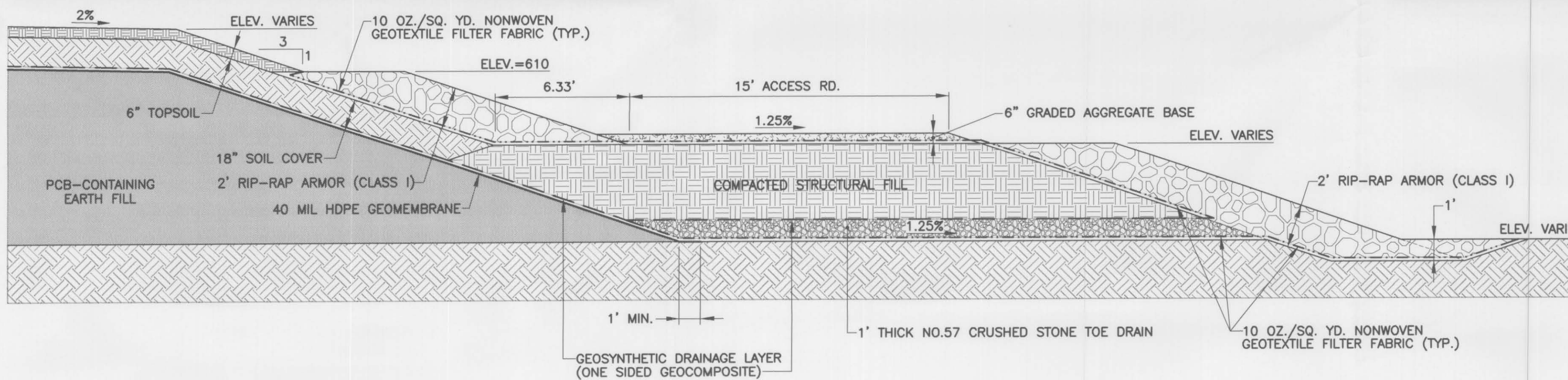
2 6 TYPICAL ACCESS ROAD SECTION
