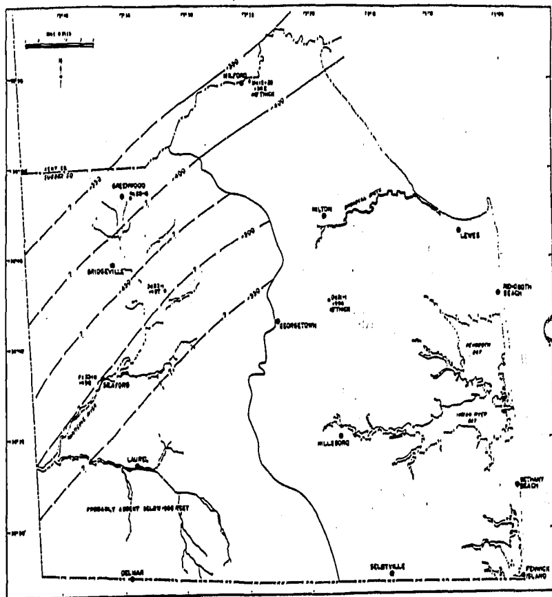
FIGURE 7. STRUCTURAL MAP OF THE TOP OF THE CHESWOLD AQUIFER (SEA LEVEL DATUM).
