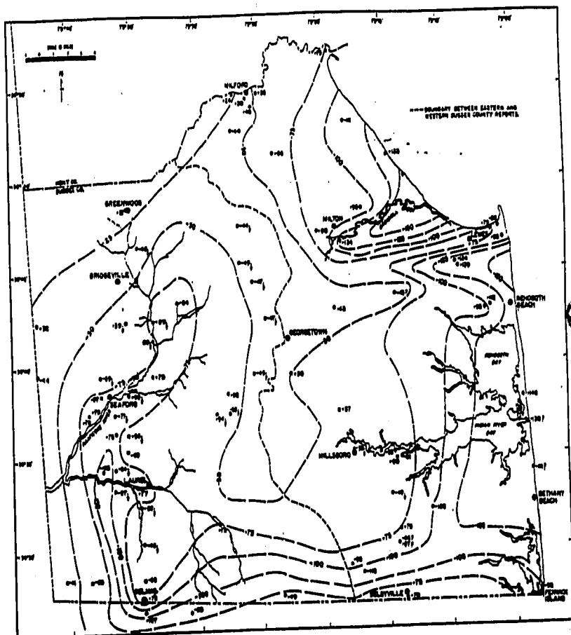
FIGURE 9. STRUCTURAL MAP OF THE BASE OF THE COLUMBIA GROUP.
