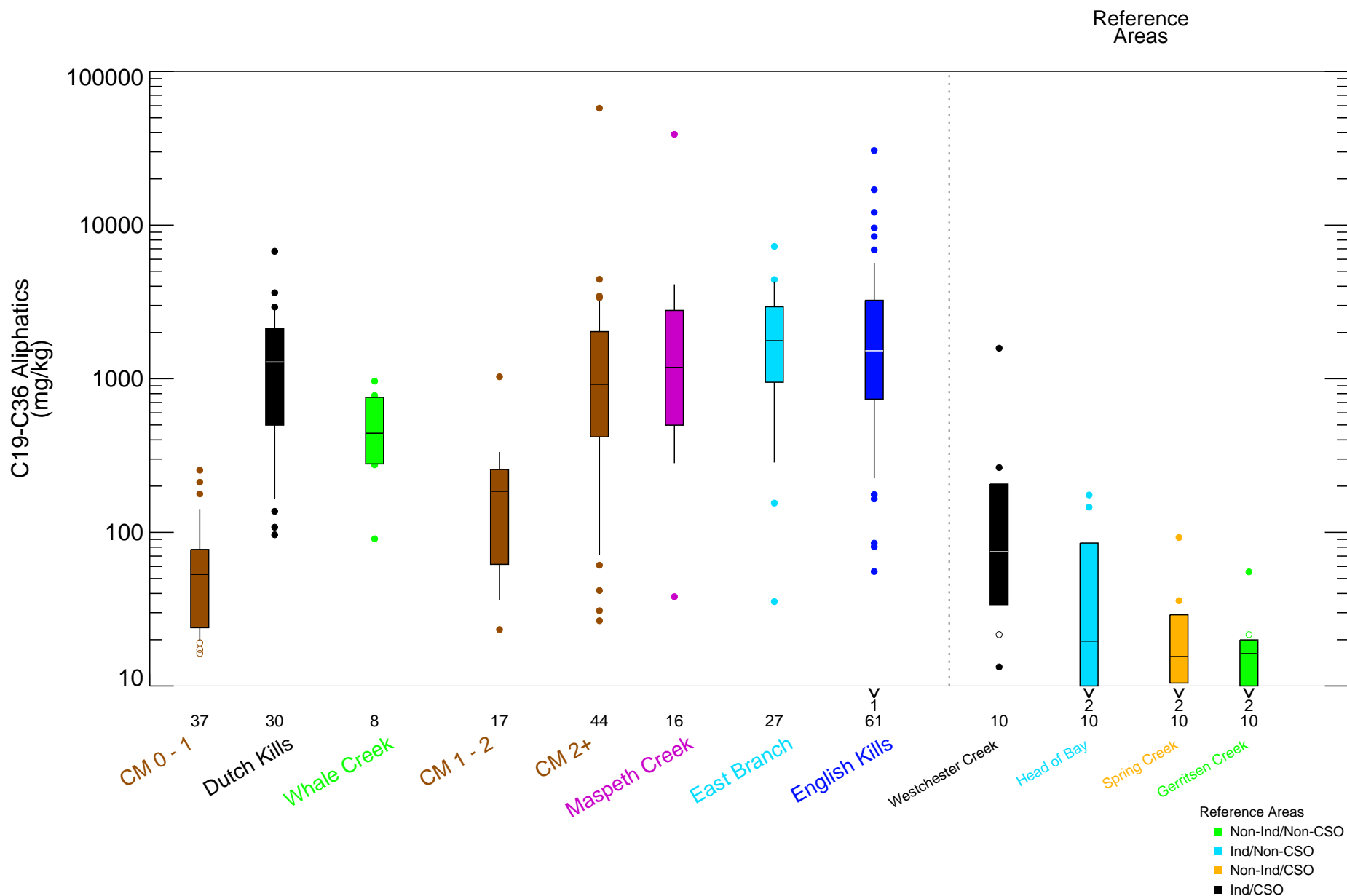
Figure 4-23 C19-C36 Aliphatics in Surface Sediment - Box Plots by Location Remedial Investigation Report Newtown Creek RI/FS
