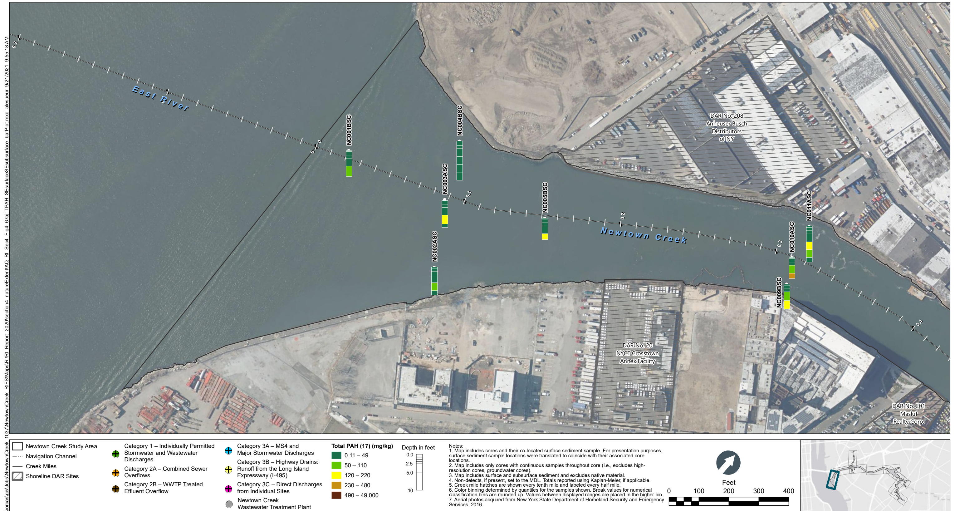
Figure 4-67a Total PAH (17) in Surface and Subsurface Sediment Bar Plots by Depth – Plan View of Newtown Creek CM 0 to 0.4 Remedial Investigation Report Newtown Creek RI/FS
