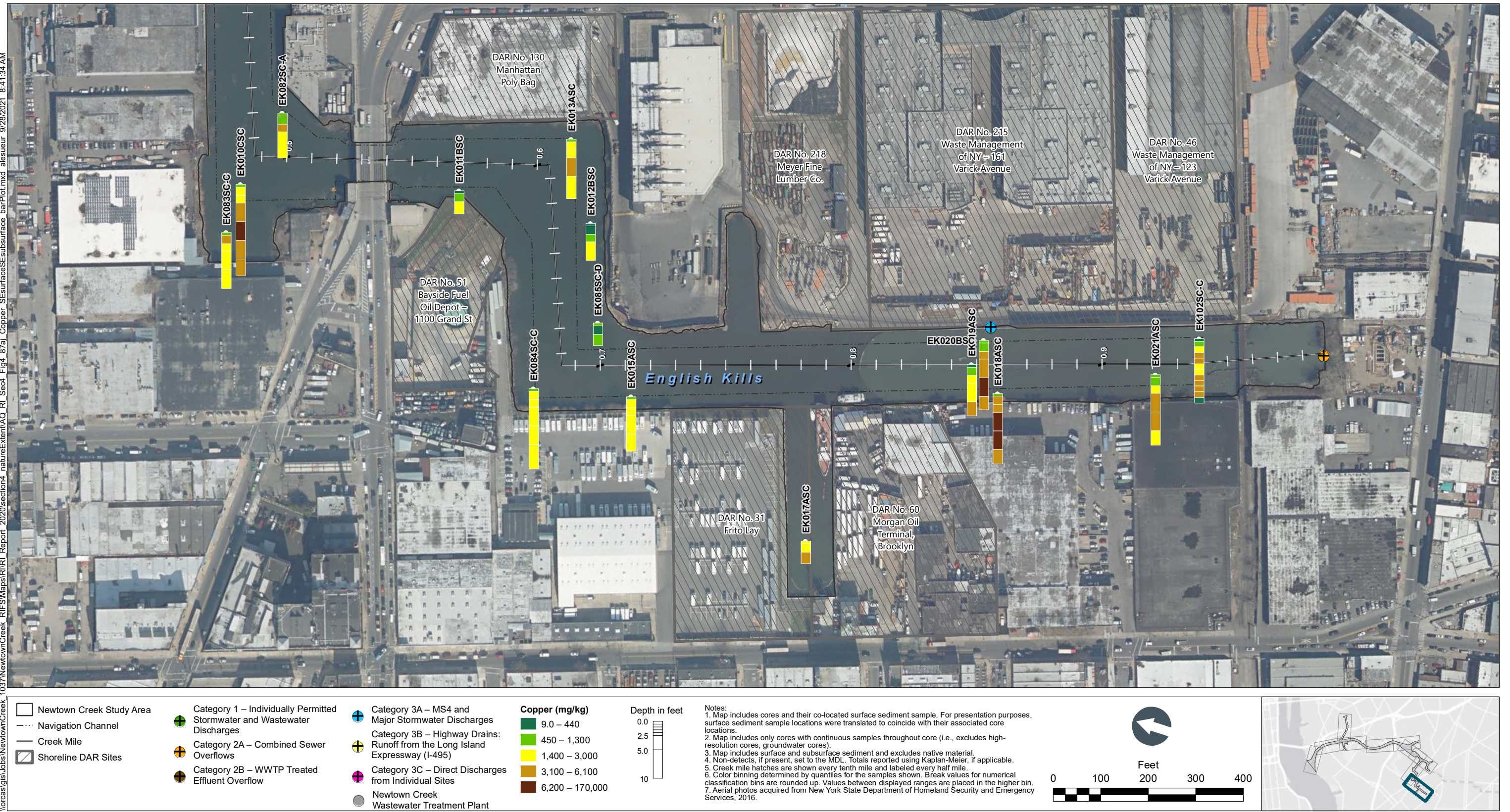
Figure 4-87j Copper in Surface and Subsurface Sediment Bar Plots by Depth – Plan View of English Kills CM 0.5 to 0.9 Remedial Investigation Report Newtown Creek RI/FS
