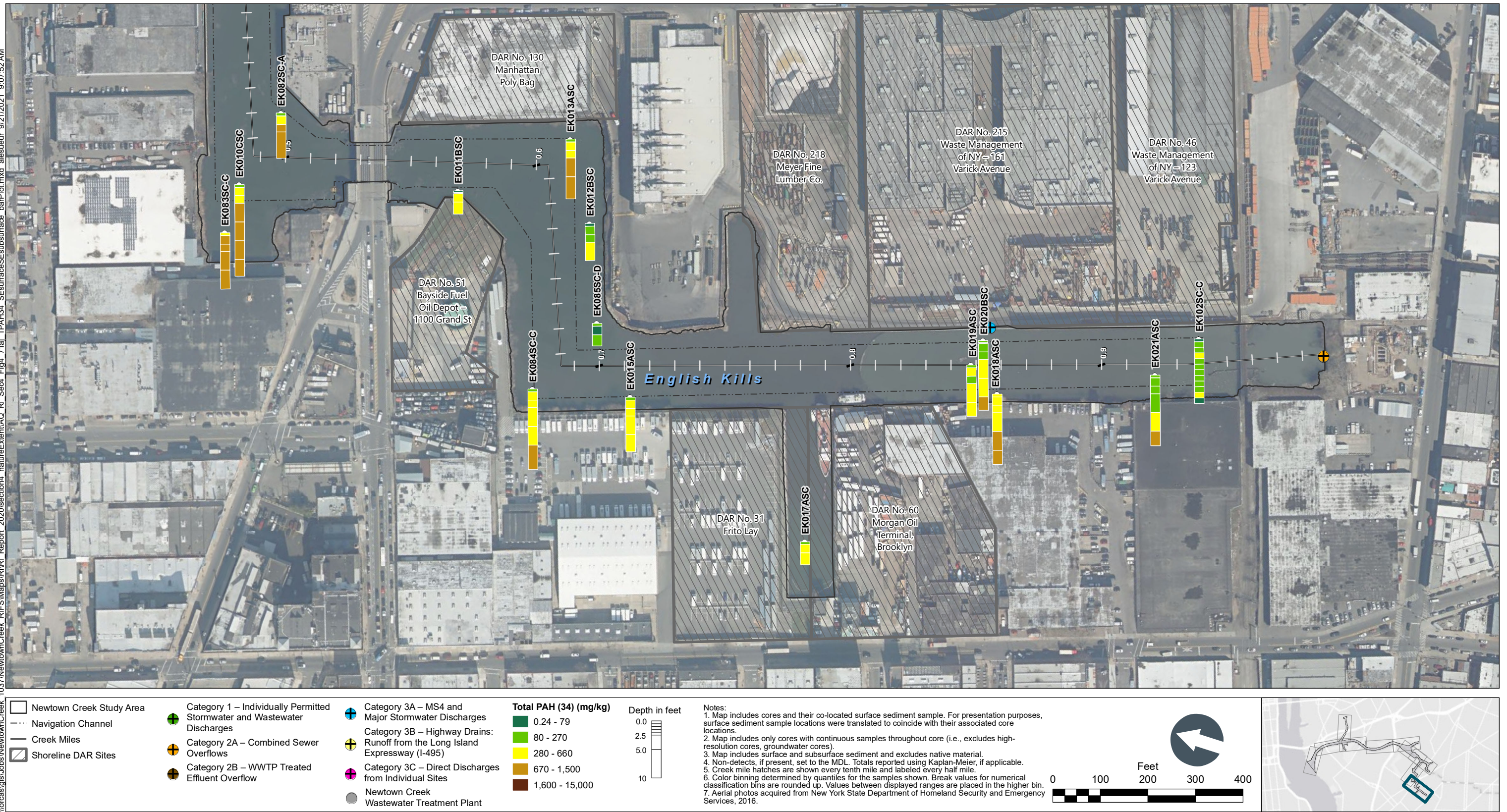
Figure 4-71j Total PAH (34) in Surface and Subsurface Sediment Bar Plots by Depth – Plan View of English Kills CM 0.5 to 0.9 Remedial Investigation Report Newtown Creek RI/FS
