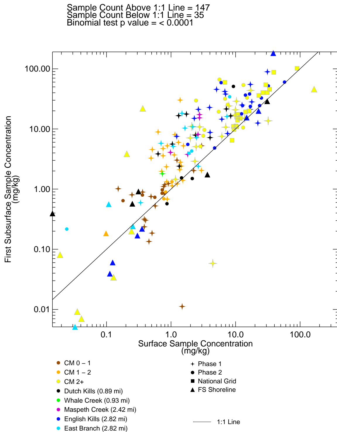
Figure 4-96 Total PCBs in Surface Sediment versus Total PCBs in First Subsurface Interval – Cross Plot Remedial Investigation Report Newtown Creek RI/FS
