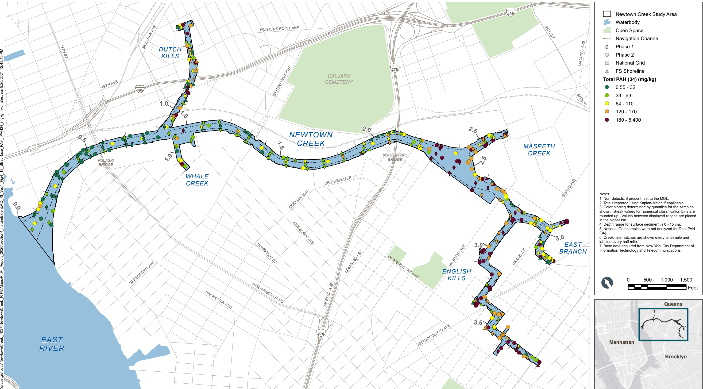
Figure 4-18 Total PAH (34) in Surface Sediment – Plan View Remedial Investigation Report Newtown Creek RI/FS
