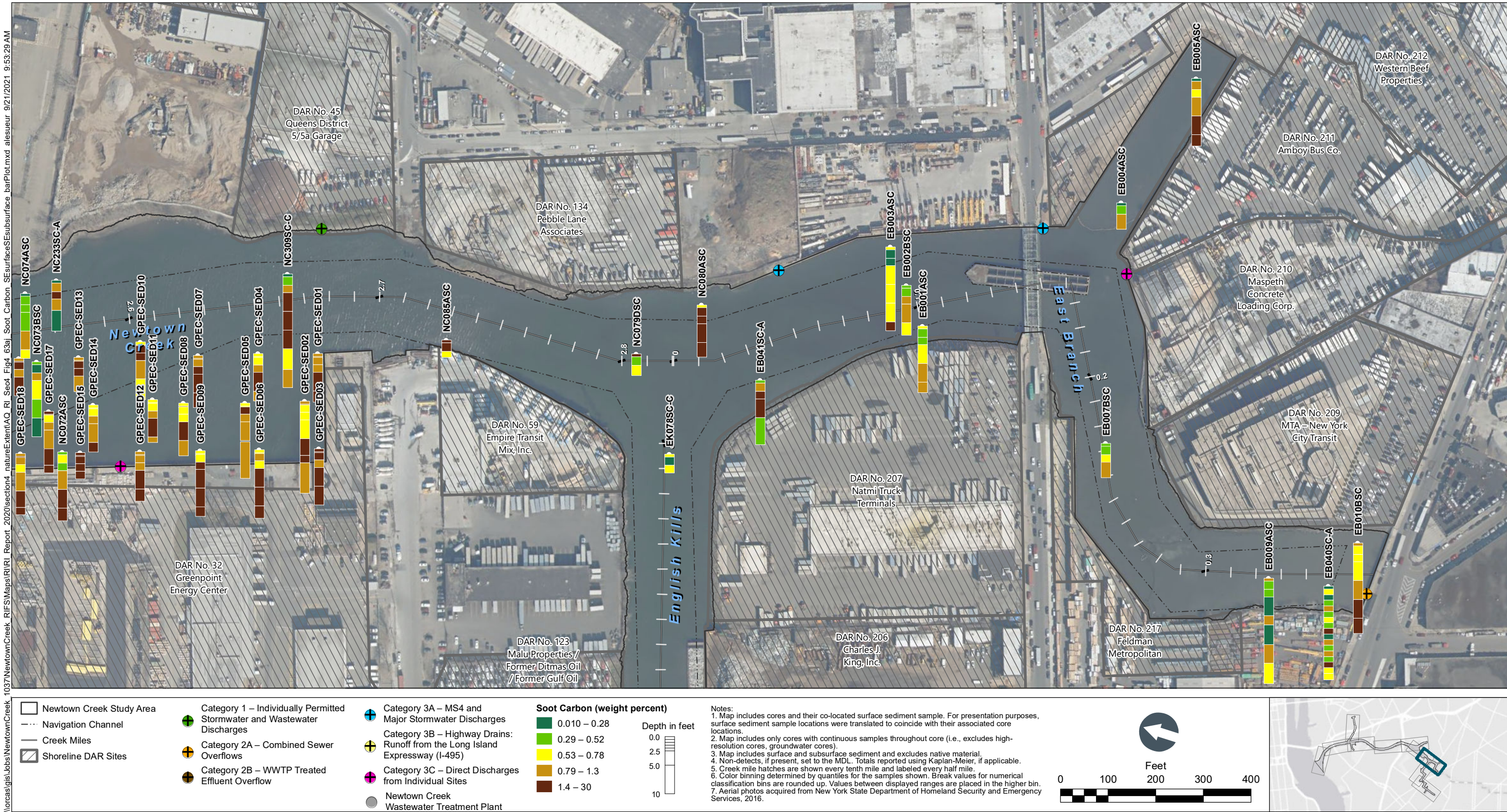
Figure 4-63h Percent Soot Carbon in Surface and Subsurface Sediment Bar Plots by Depth – Plan View of East Branch and Newtown Creek CM 2.6 to 2.8 Remedial Investigation Report Newtown Creek RI/FS
