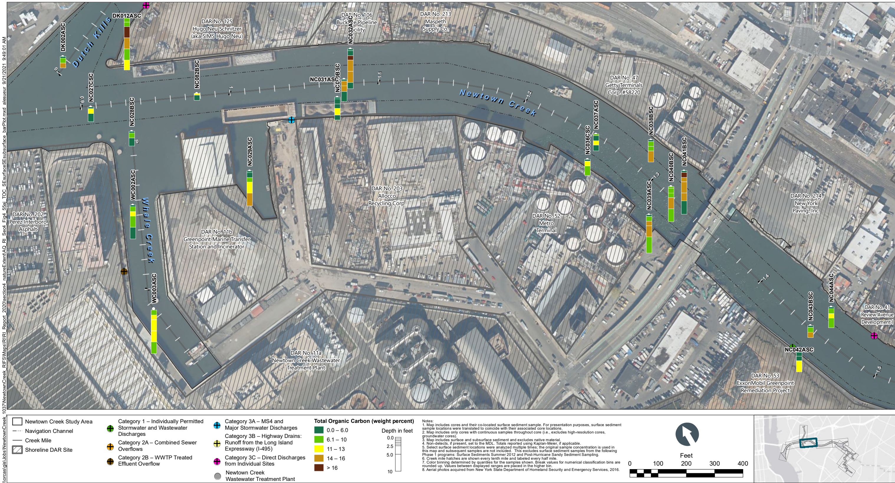
Figure 4-55c TOC in Surface and Subsurface Sediment Bar Plots by Depth – Plan View of Whale Creek and Newtown Creek CM 0.9 to 1.5 Remedial Investigation Report Newtown Creek RI/FS
