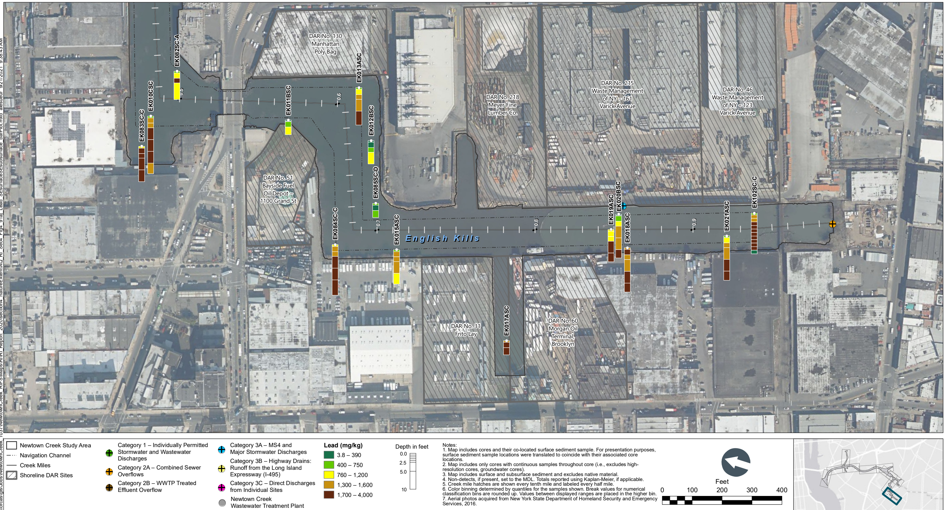
Figure 4-91j Lead in Surface and Subsurface Sediment Bar Plots by Depth – Plan View of English Kills CM 0.5 to 0.9 Remedial Investigation Report Newtown Creek RI/FS
