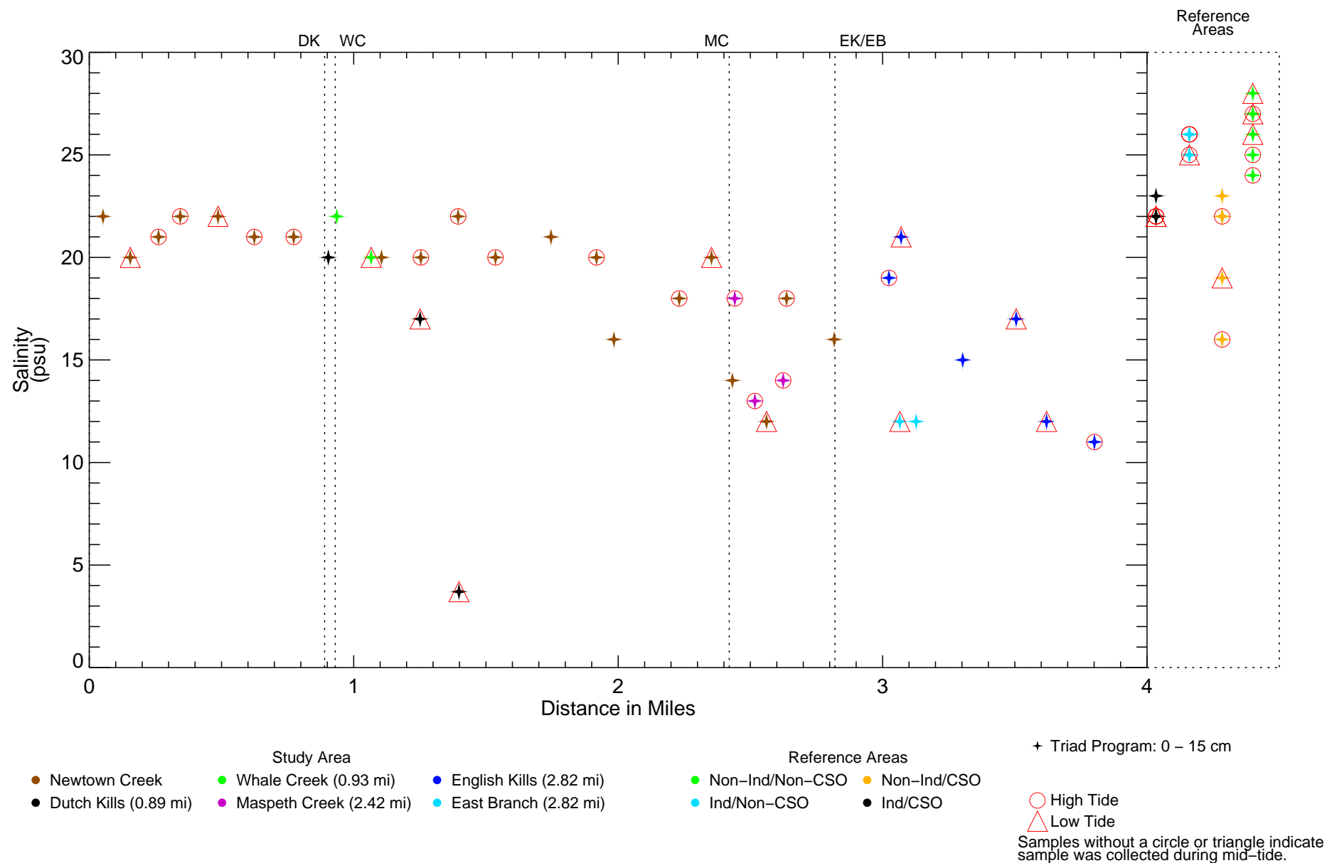
Figure 4-195 Salinity in Shallow Porewater – Longitudinal Profile Remedial Investigation Report Newtown Creek RI/FS
