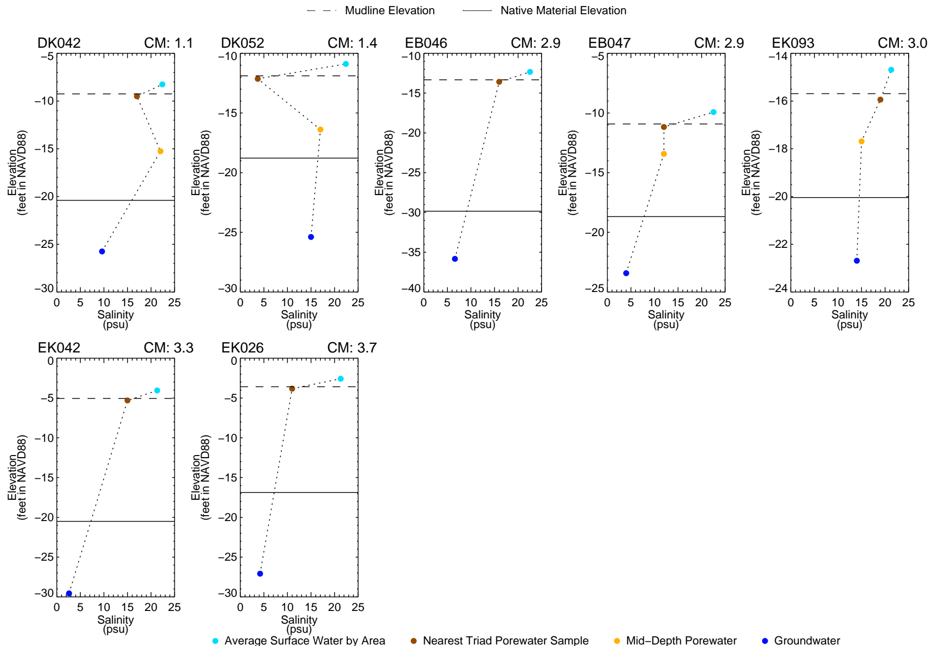
Figure 4-231b Salinity in Porewater and Groundwater – Depth Profiles for Dutch Kills, East Branch, and English Kills Remedial Investigation Report Newtown Creek RI/FS
