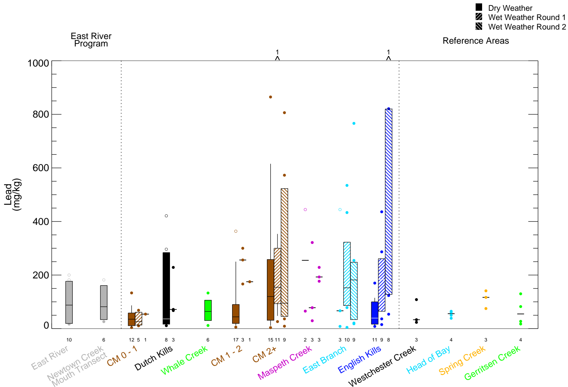
Figure 4-193 Calculated Particulate Phase Lead in Surface Water During Dry and Wet Weather Sampling Events - Box Plots Remedial Investigation Report Newtown Creek RI/FS
