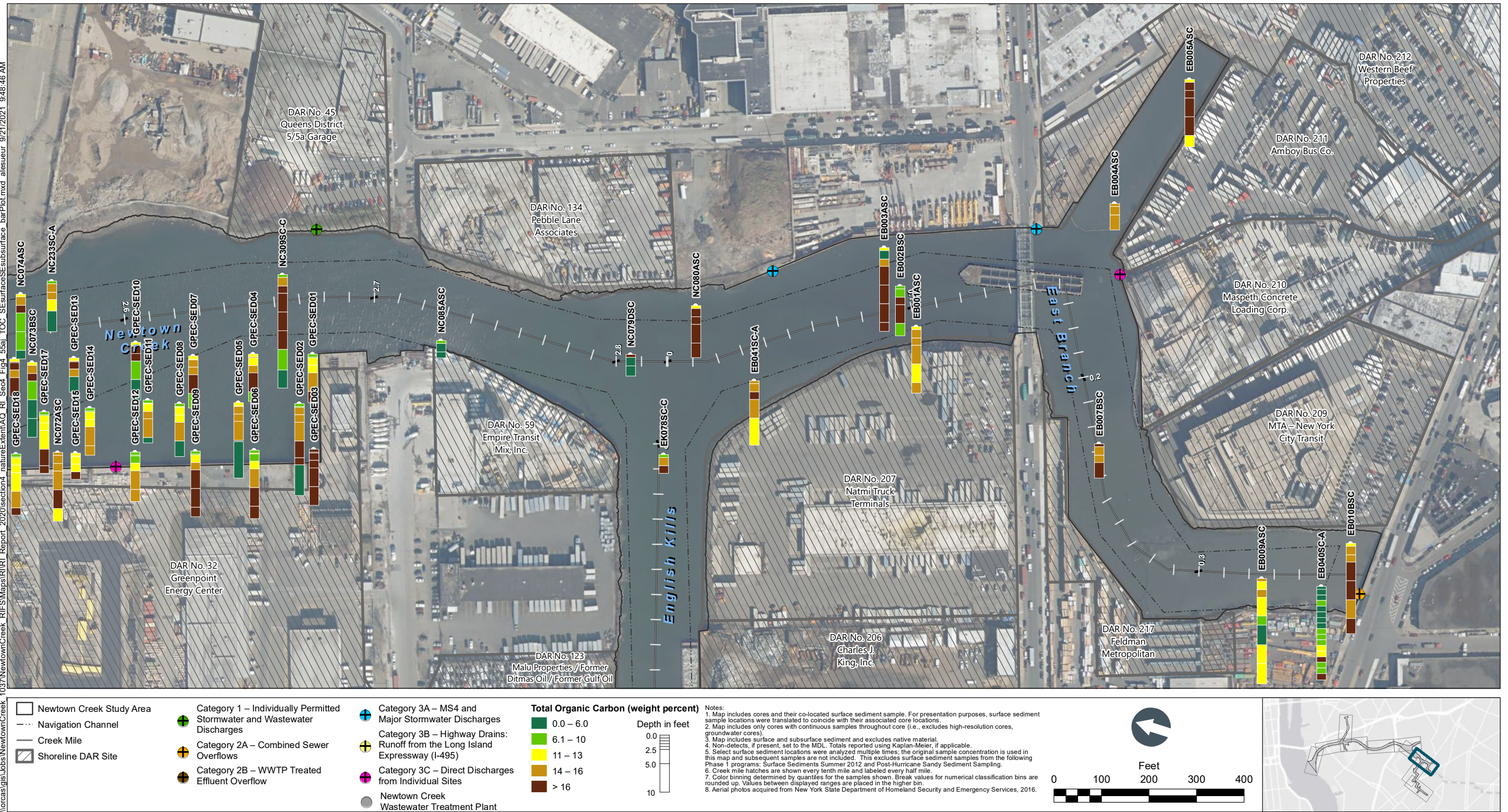
Figure 4-55h TOC in Surface and Subsurface Sediment Bar Plots by Depth – Plan View of East Branch and Newtown Creek CM 2.6 to 2.8 Remedial Investigation Report Newtown Creek RI/FS
