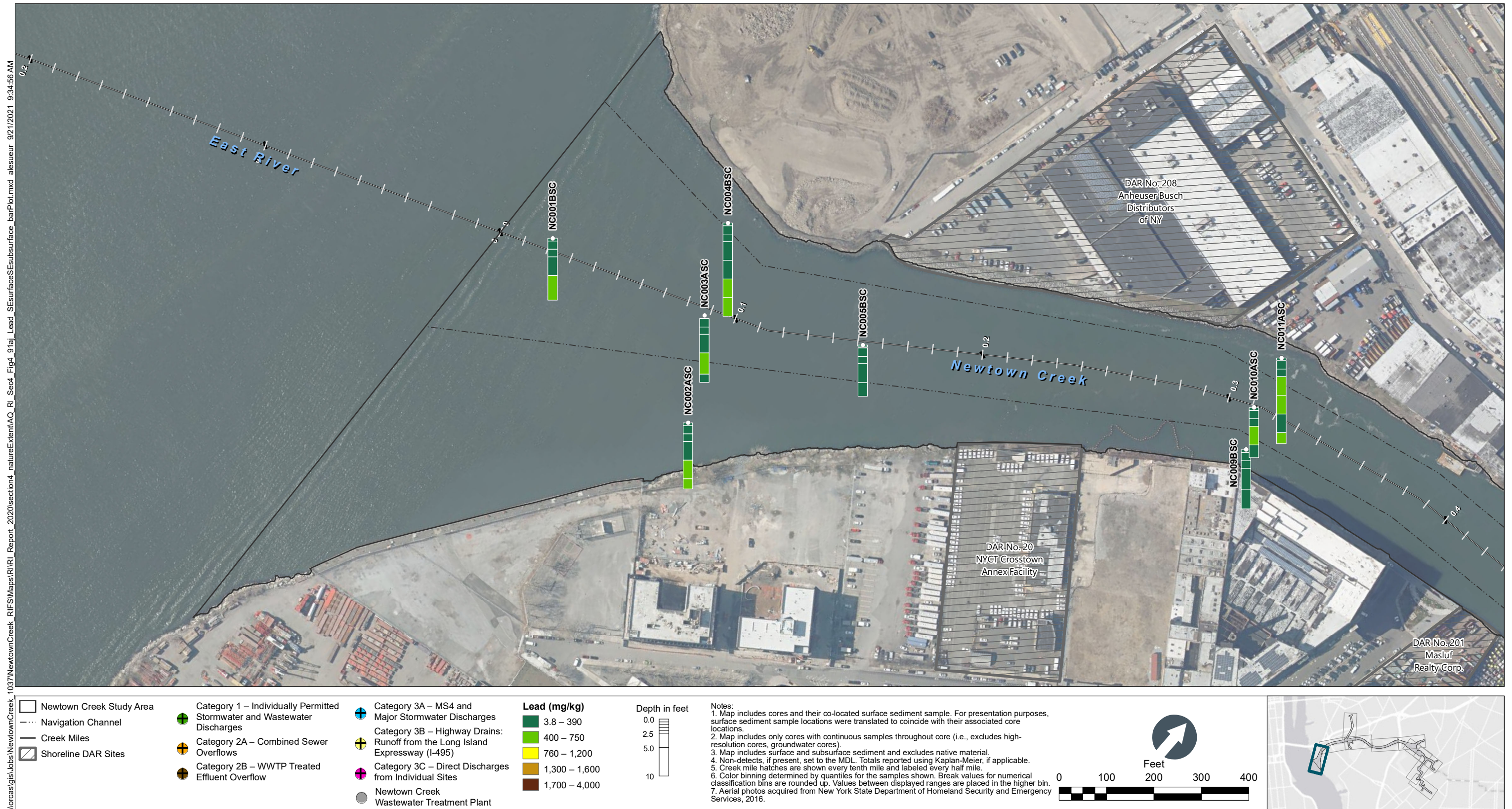
Figure 4-91a Lead in Surface and Subsurface Sediment Bar Plots by Depth – Plan View of Newtown Creek CM 0 to 0.4 Remedial Investigation Report Newtown Creek RI/FS
