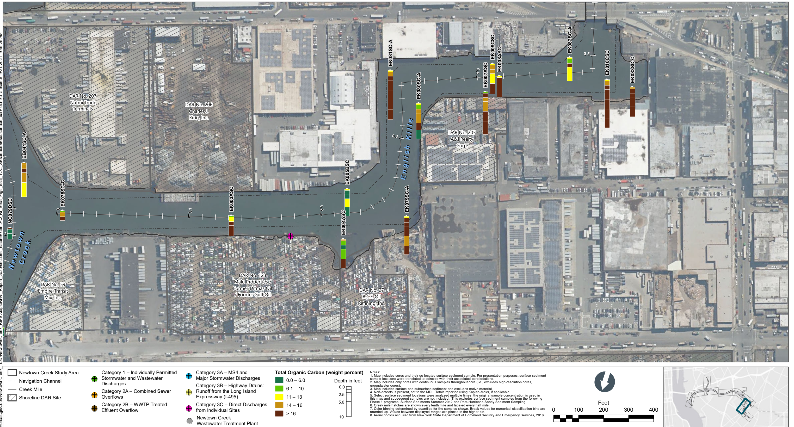
Figure 4-55i TOC in Surface and Subsurface Sediment Bar Plots by Depth – Plan View of English Kills CM 0 to 0.5 Remedial Investigation Report Newtown Creek RI/FS
