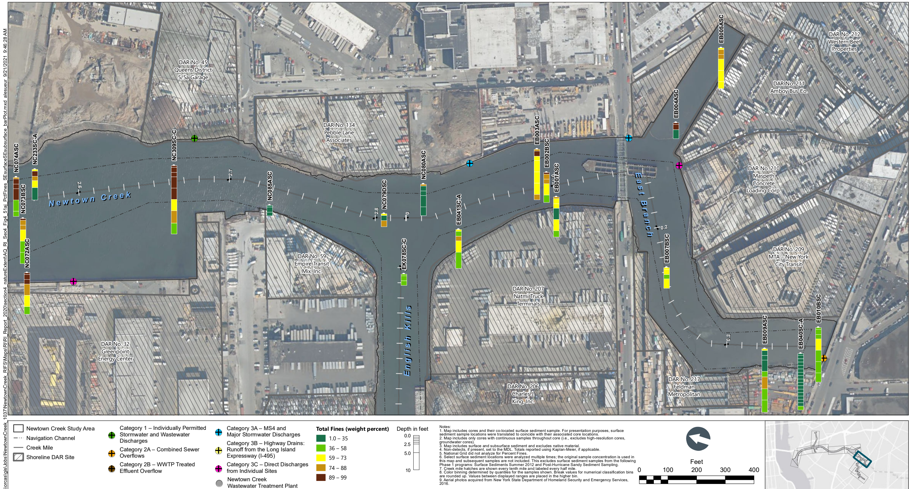
Figure 4-51h Total Percent Fines in Surface and Subsurface Sediment Bar Plots by Depth – Plan View of East Branch and Newtown Creek CM 2.6 to 2.8 Remedial Investigation Report Newtown Creek RI/FS
