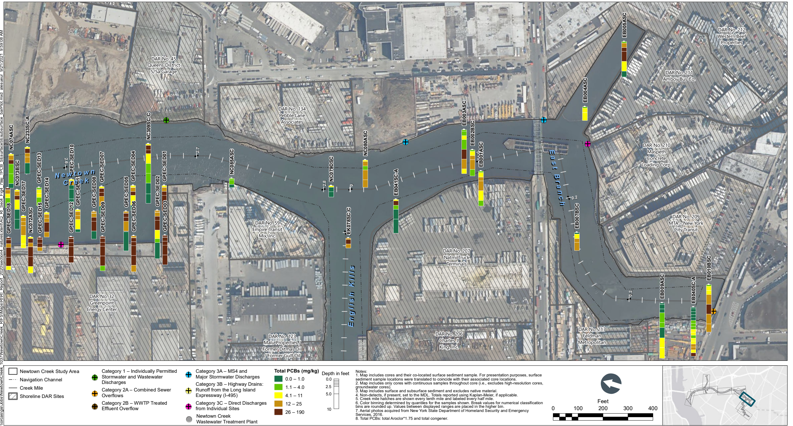
Figure 4-79h Total PCBs in Surface and Subsurface Sediment Bar Plots by Depth – Plan View of East Branch and Newtown Creek CM 2.6 to 2.8 Remedial Investigation Report Newtown Creek RI/FS
