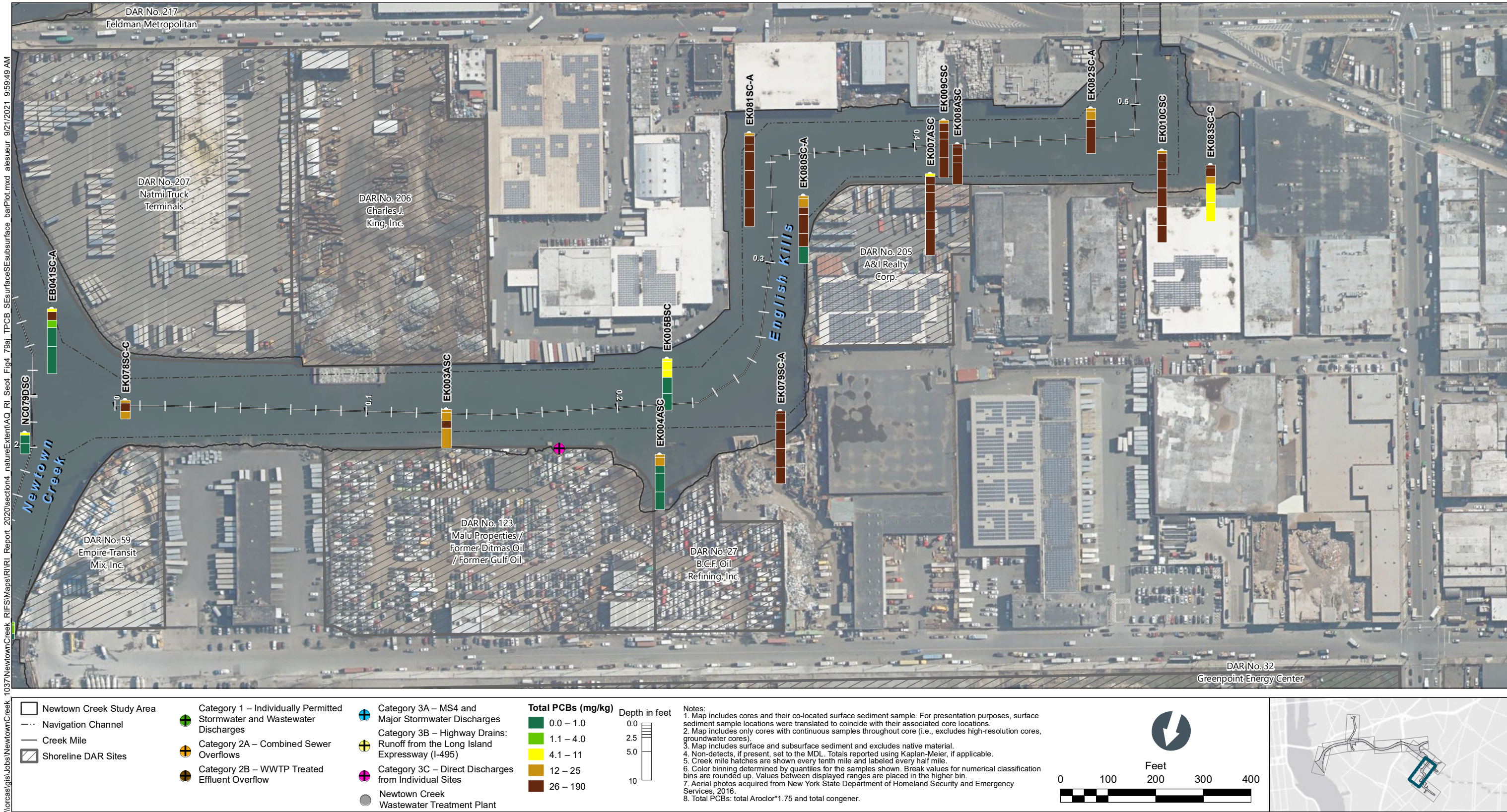
Figure 4-79i Total PCBs in Surface and Subsurface Sediment Bar Plots by Depth – Plan View of English Kills CM 0 to 0.5 Remedial Investigation Report Newtown Creek RI/FS
