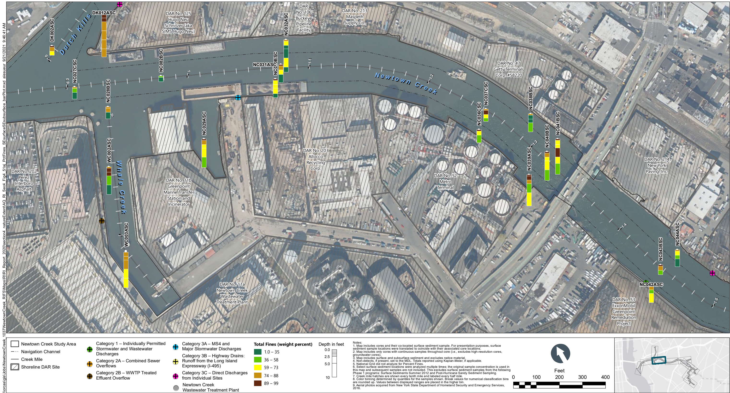
Figure 4-51c Total Percent Fines in Surface and Subsurface Sediment Bar Plots by Depth – Plan View of Whale Creek and Newtown Creek CM 0.9 to 1.5 Remedial Investigation Report Newtown Creek RI/FS
