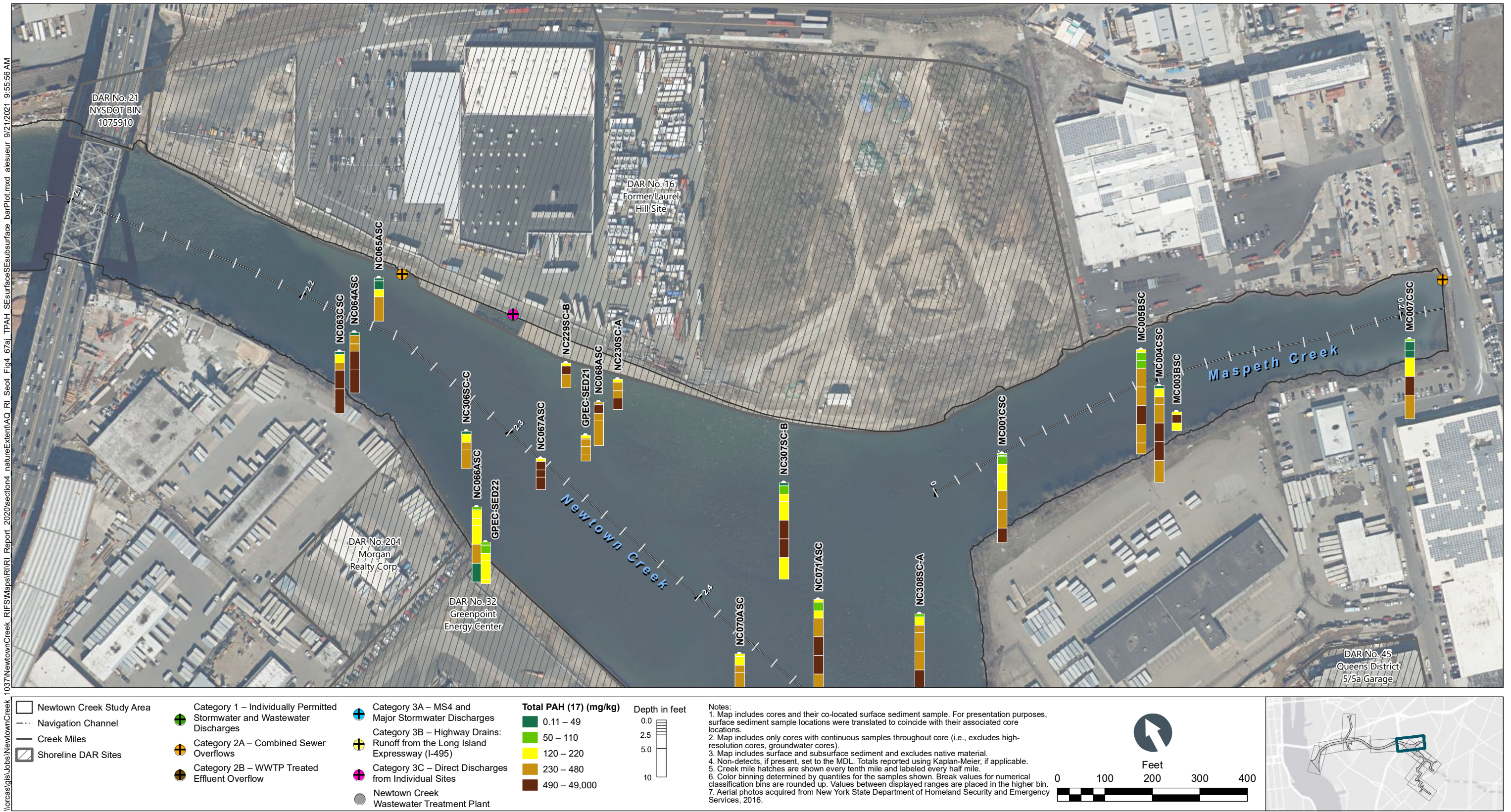
Figure 4-67f Total PAH (17) in Surface and Subsurface Sediment Bar Plots by Depth – Plan View of Maspeth Creek and Newtown Creek CM 2.1 to 2.4 Remedial Investigation Report Newtown Creek RI/FS
