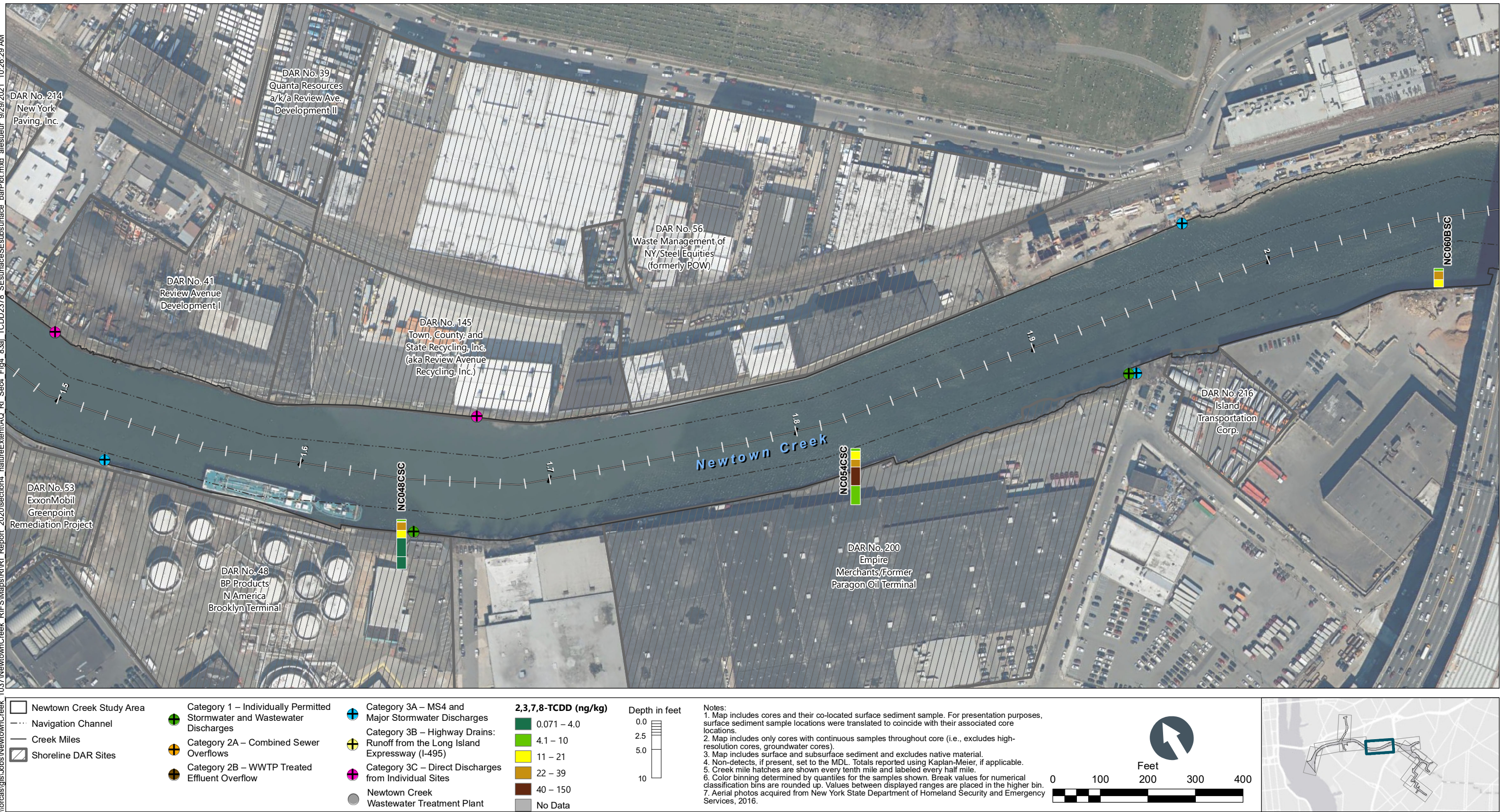
Figure 4-83e 2,3,7,8-TCDD in Surface and Subsurface Sediment Bar Plots by Depth – Plan View of Newtown Creek CM 1.5 to 2.0 Remedial Investigation Report Newtown Creek RI/FS
