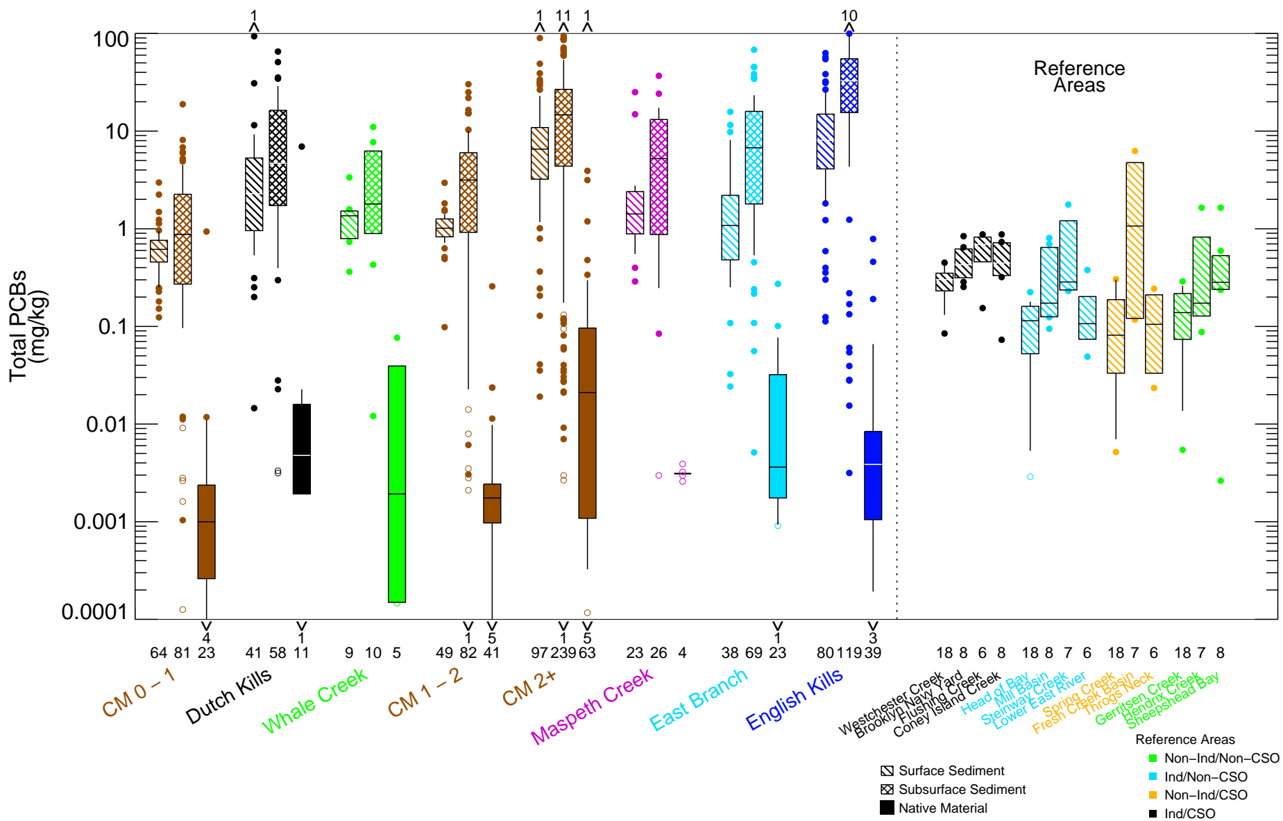
Figure 4-76 Total PCBs in Surface Sediment, Subsurface Sediment, and Native Material – Box Plots by Location Remedial Investigation Report Newtown Creek RI/FS
