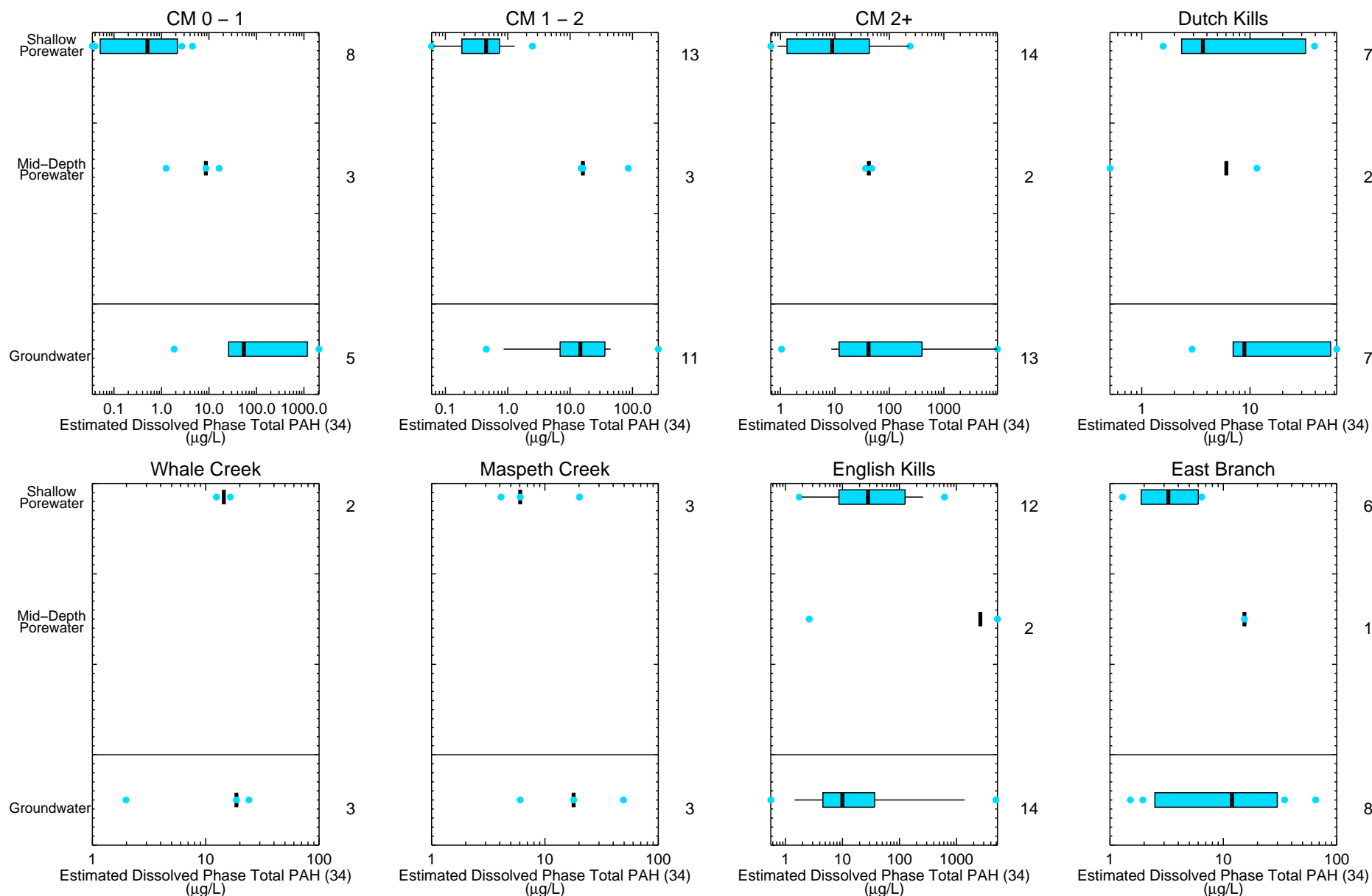
Figure 4-242b Estimated Dissolved Phase (Method 2) Total PAH (34) in Porewater and Groundwater – Box Plot Depth Profiles Remedial Investigation Report Newtown Creek RI/FS
