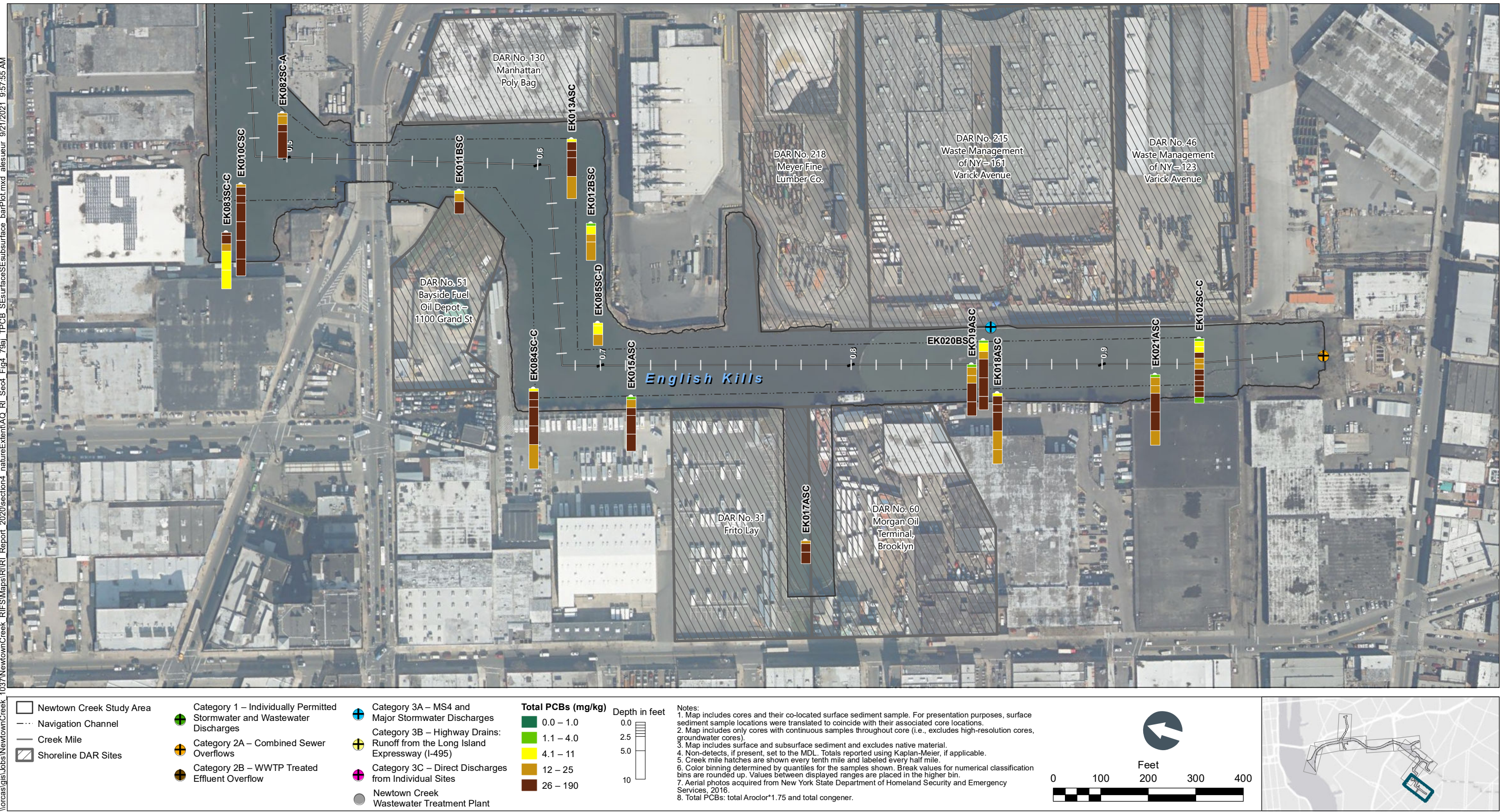
Figure 4-79j Total PCBs in Surface and Subsurface Sediment Bar Plots by Depth – Plan View of English Kills CM 0.5 to 0.9 Remedial Investigation Report Newtown Creek RI/FS
