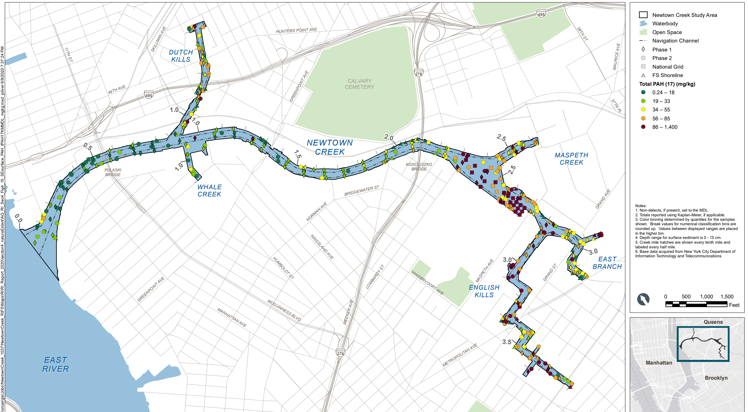
Figure 4-15 Total PAH (17) in Surface Sediment – Plan View Remedial Investigation Report Newtown Creek RI/FS
