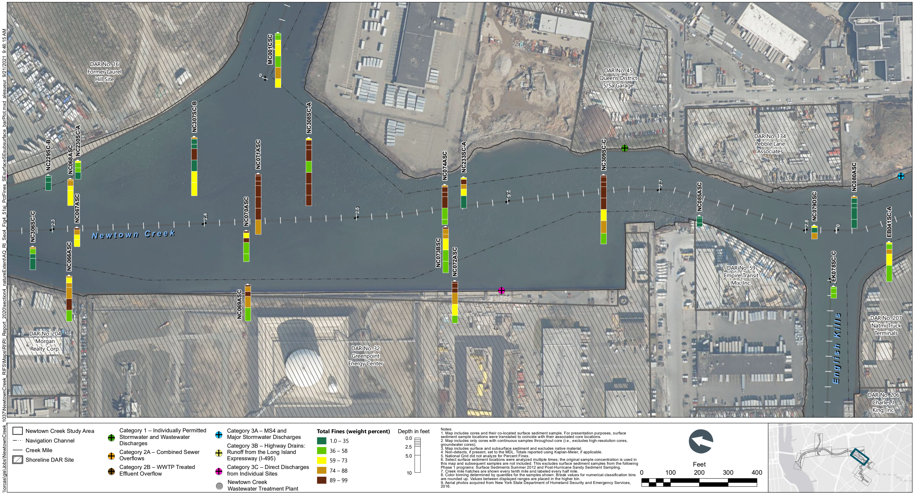
Figure 4-51g Total Percent Fines in Surface and Subsurface Sediment Bar Plots by Depth – Plan View of Newtown Creek CM 2.3 to 2.8 Remedial Investigation Report Newtown Creek RI/FS
