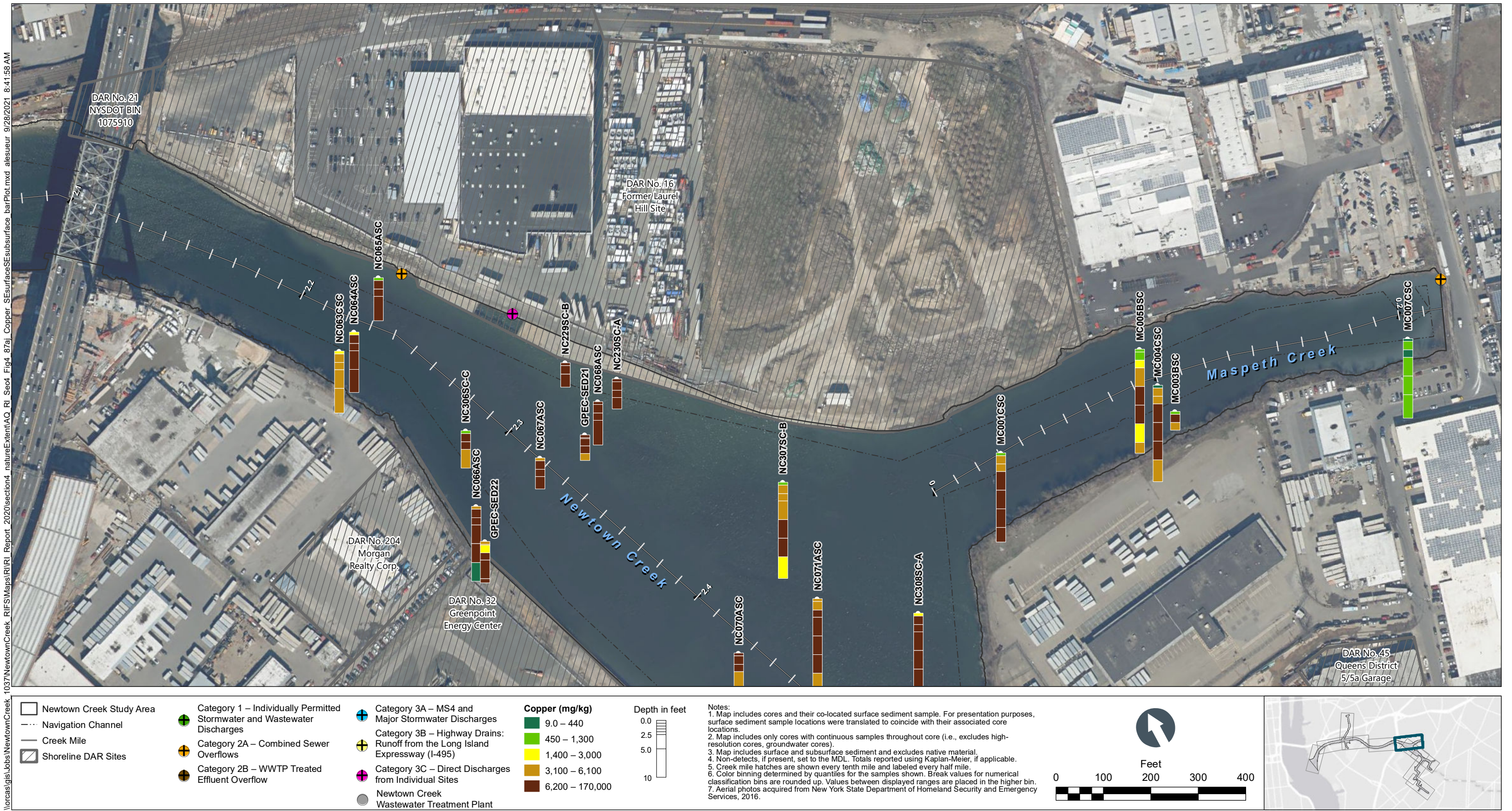
Figure 4-87f Copper in Surface and Subsurface Sediment Bar Plots by Depth – Plan View of Maspeth Creek and Newtown Creek CM 2.1 to 2.4 Remedial Investigation Report Newtown Creek RI/FS
