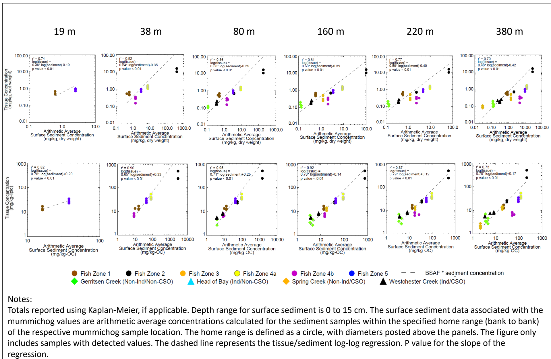
Figure 6-49 Total PCBs in Mummichog Whole Body versus Sediment – Cross Plots Remedial Investigation Report Newtown Creek RI/FS
