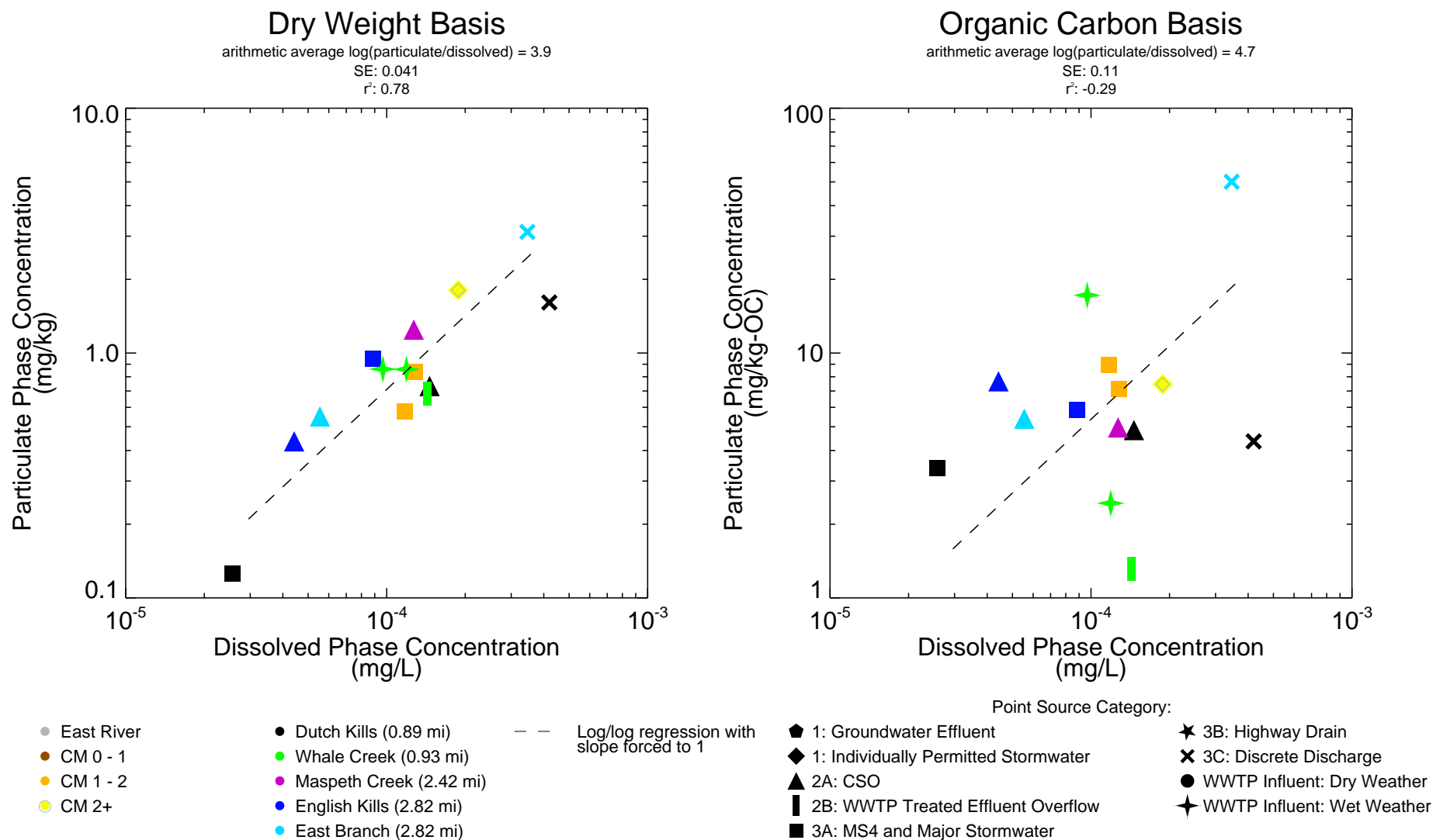
Figure 6-11c Point Source Particulate Phase versus Dissolved Phase for C3-Naphthalenes - Cross Plots Remedial Investigation Report Newtown Creek RI/FS
