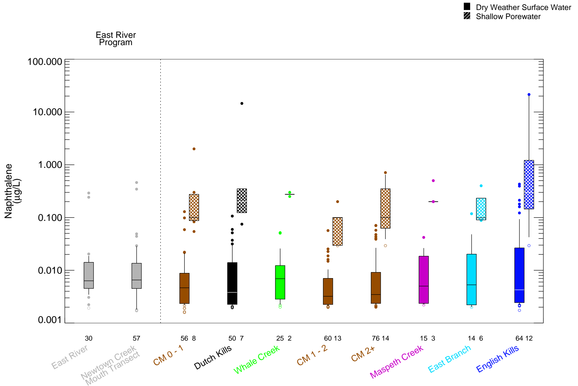
Figure 6-24b Dissolved Phase Naphthalene in Surface Water Dry Weather and Shallow Porewater - Box Plots Remedial Investigation Report Newtown Creek RI/FS
