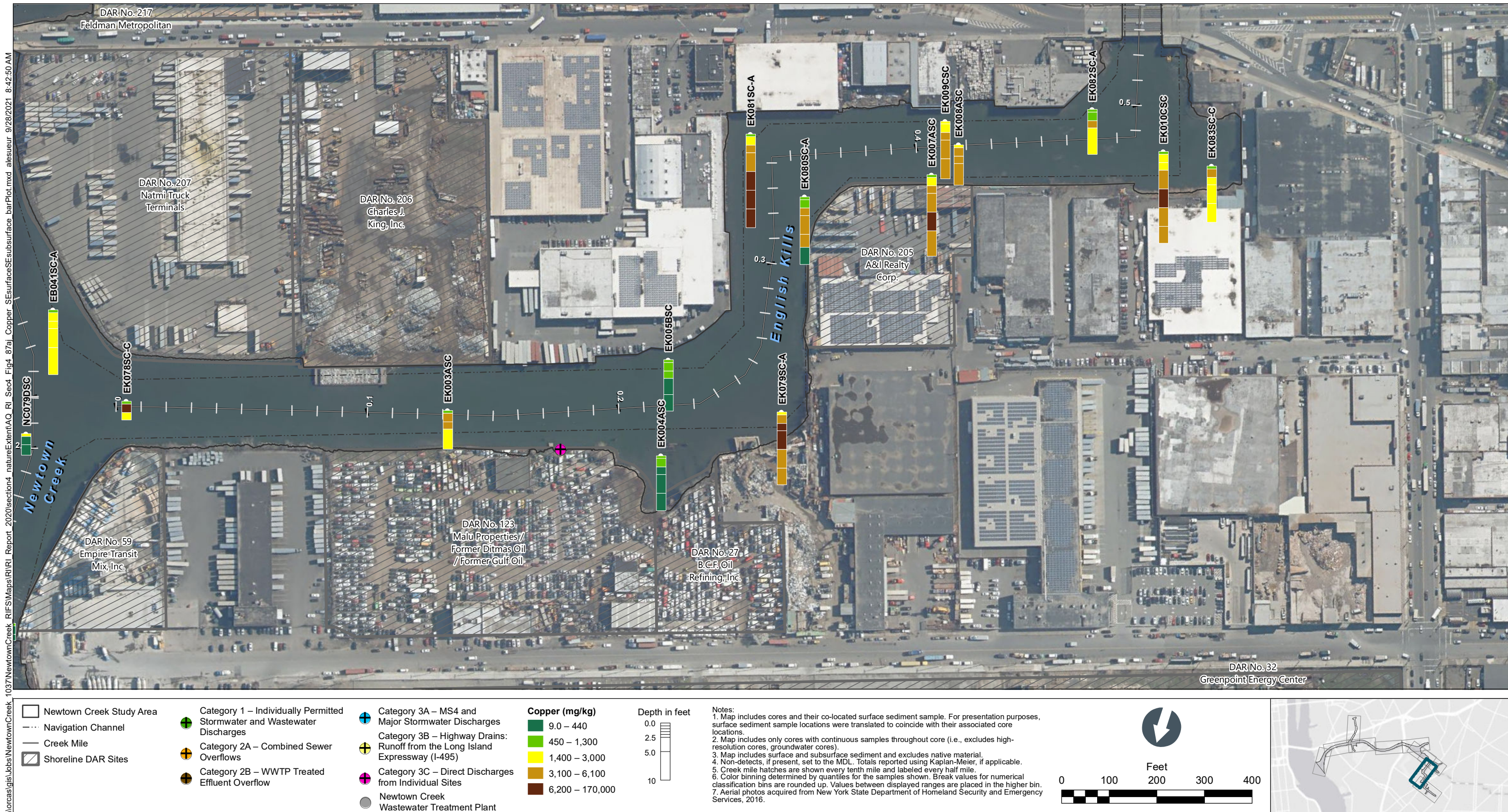
Figure 4-87i Copper in Surface and Subsurface Sediment Bar Plots by Depth – Plan View of English Kills CM 0 to 0.5 Remedial Investigation Report Newtown Creek RI/FS
