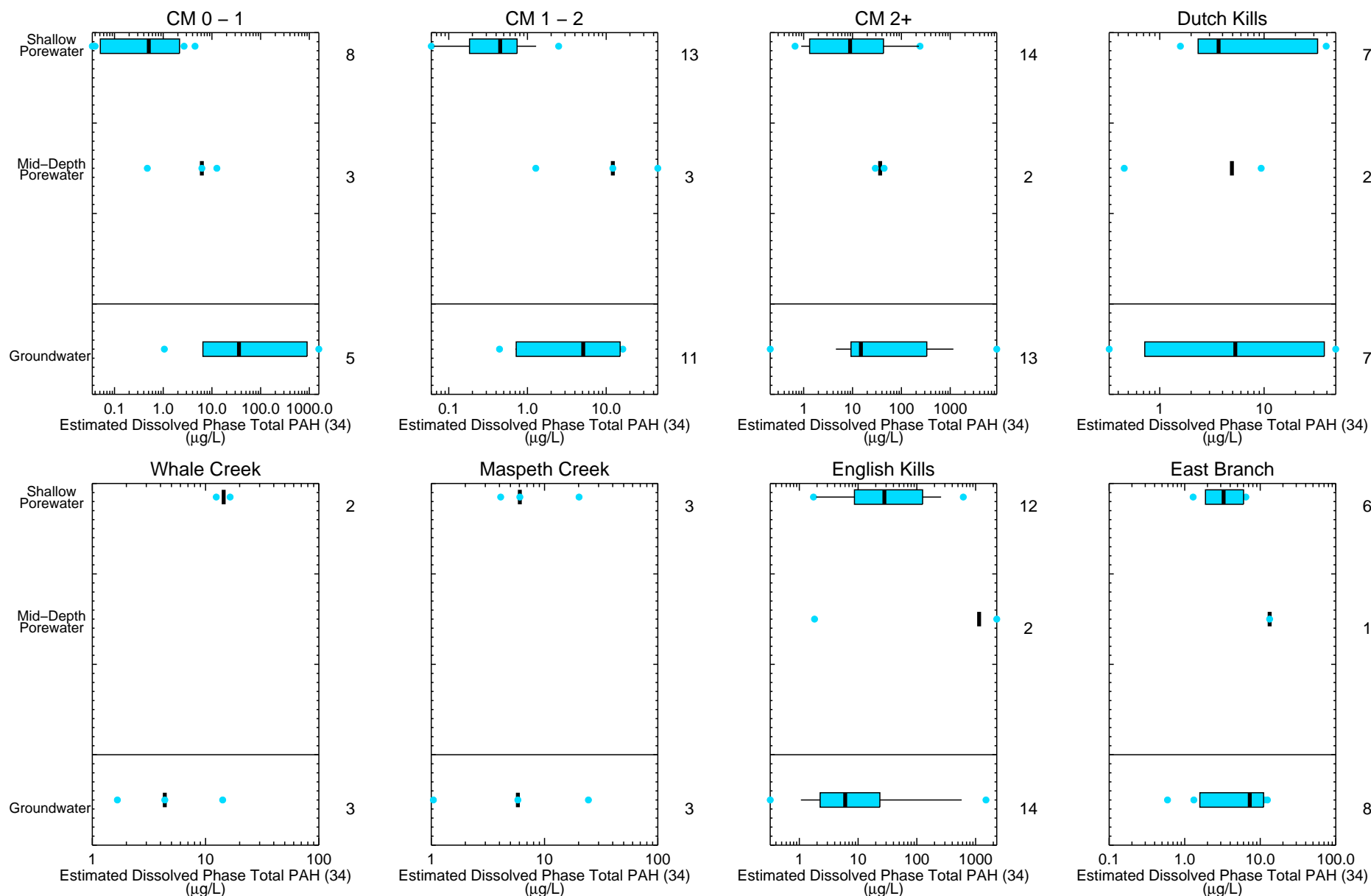
Figure 4-242a Estimated Dissolved Phase (Method 1) Total PAH (34) in Porewater and Groundwater – Box Plot Depth Profiles Remedial Investigation Report Newtown Creek RI/FS
