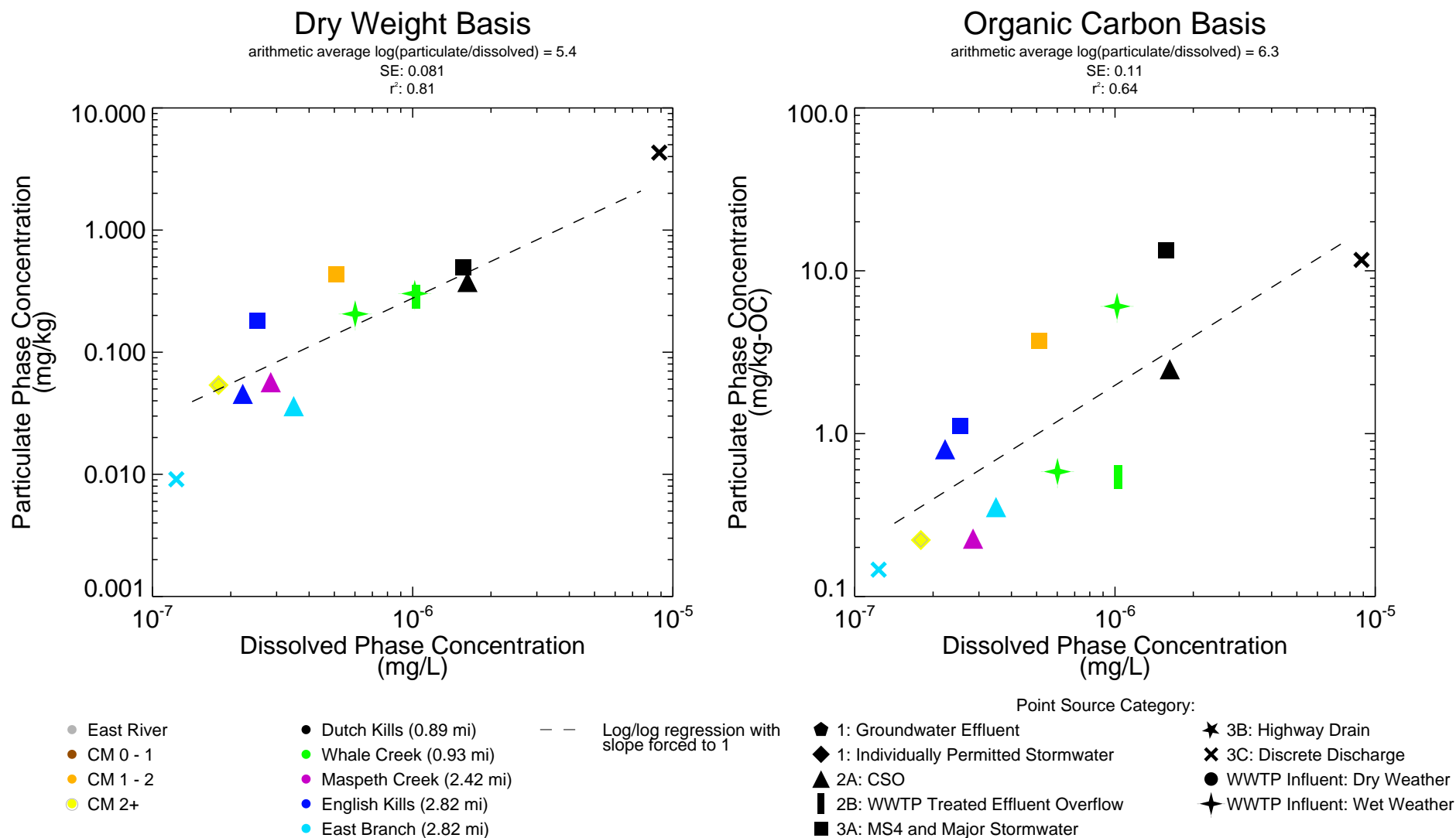
Figure 6-12e Point Source Particulate Phase versus Dissolved Phase for Total Pentachlorobiphenyl Homologs - Cross Plots Remedial Investigation Report Newtown Creek RI/FS
