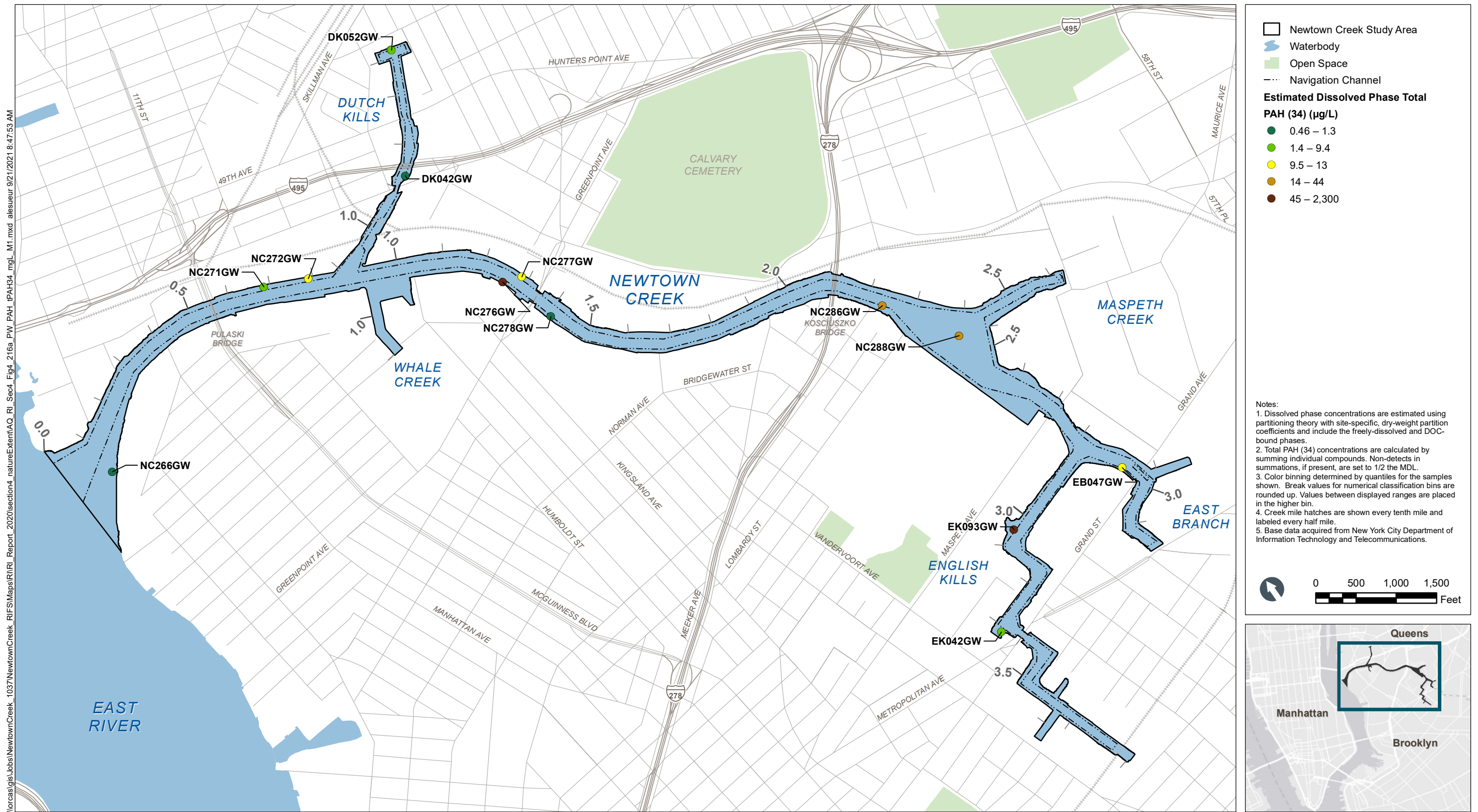
Figure 4-216a Estimated Dissolved Phase (Method 1) Total PAH (34) in Mid-Depth Porewater – Plan View Remedial Investigation Report Newtown Creek RI/FS
