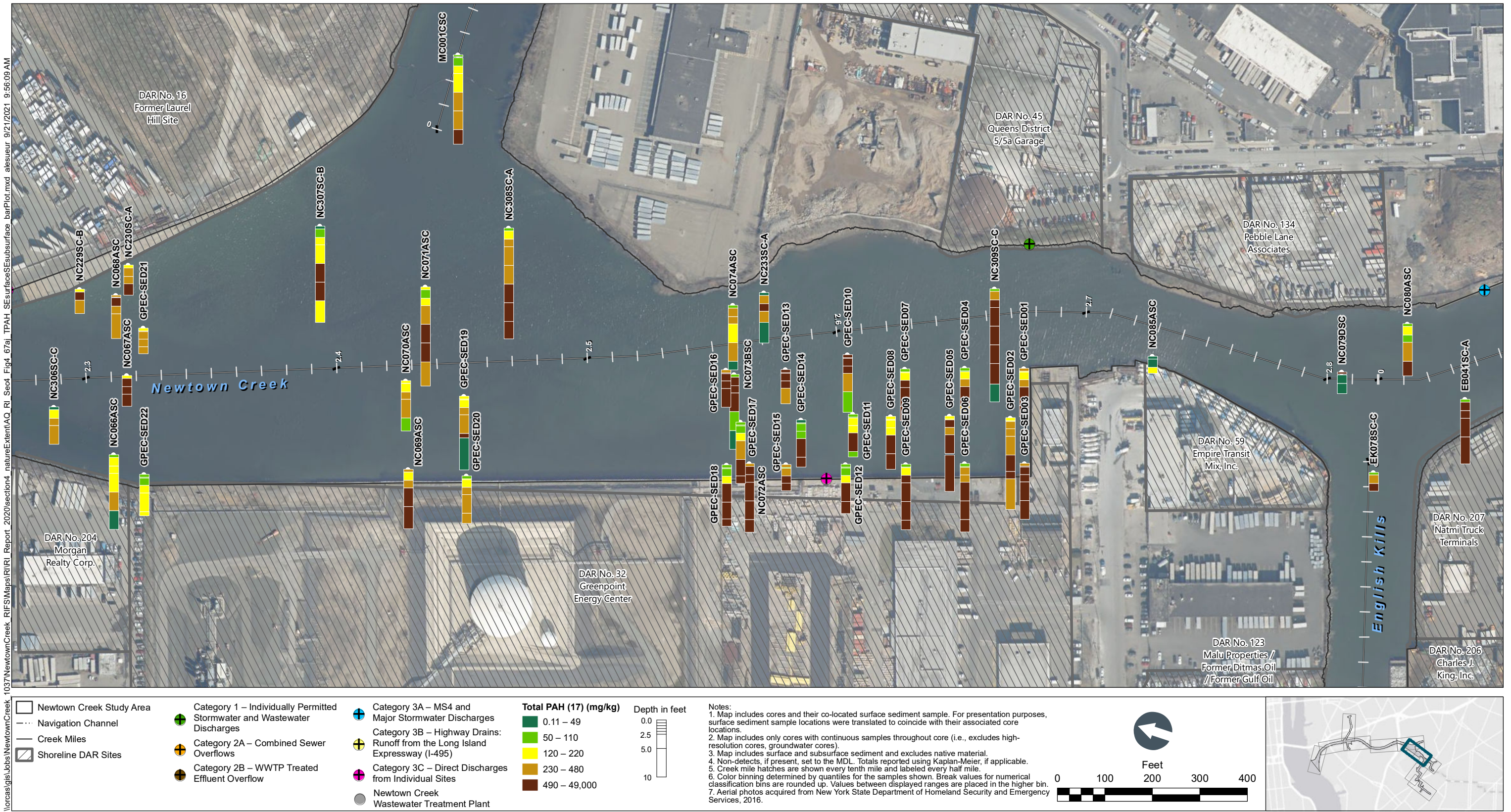
Figure 4-67g Total PAH (17) in Surface and Subsurface Sediment Bar Plots by Depth – Plan View of Newtown Creek CM 2.3 to 2.8 Remedial Investigation Report Newtown Creek RI/FS
