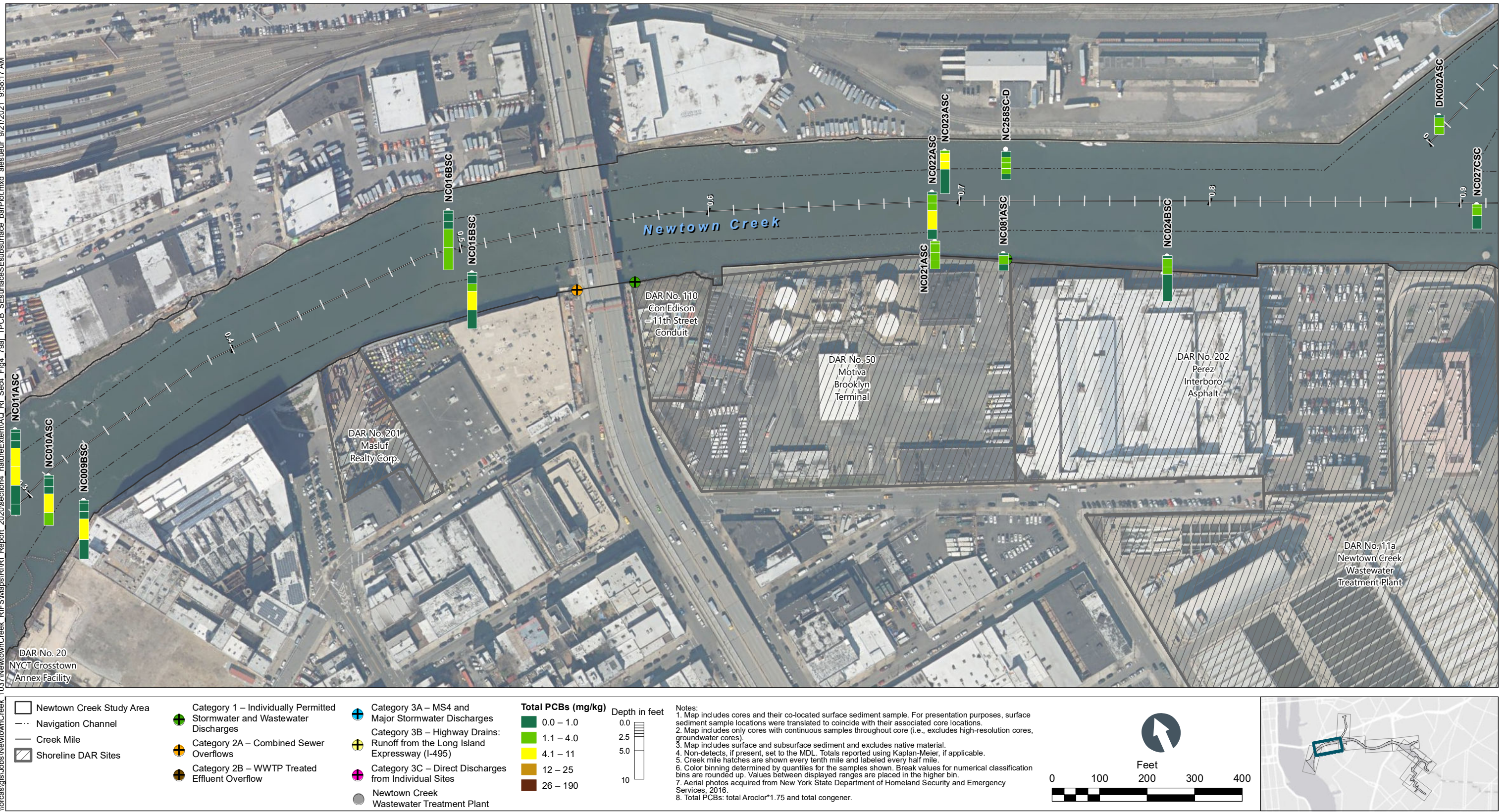
Figure 4-79b Total PCBs in Surface and Subsurface Sediment Bar Plots by Depth – Plan View of Newtown Creek CM 0.3 to 0.9 Remedial Investigation Report Newtown Creek RI/FS
