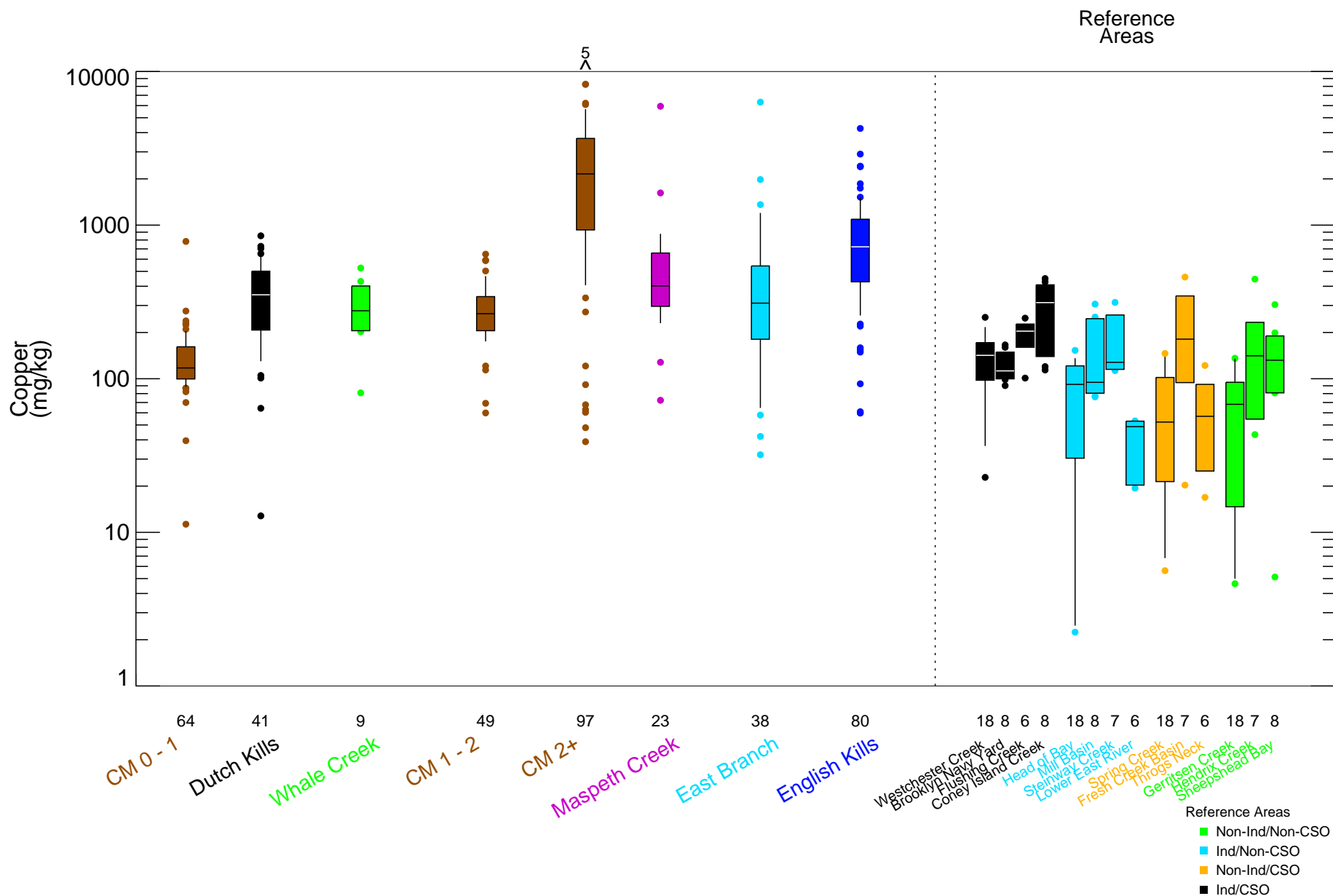
Figure 8-11 Copper in Surface Sediment - Box Plots by Location Remedial Investigation Report Newtown Creek RI/FS
