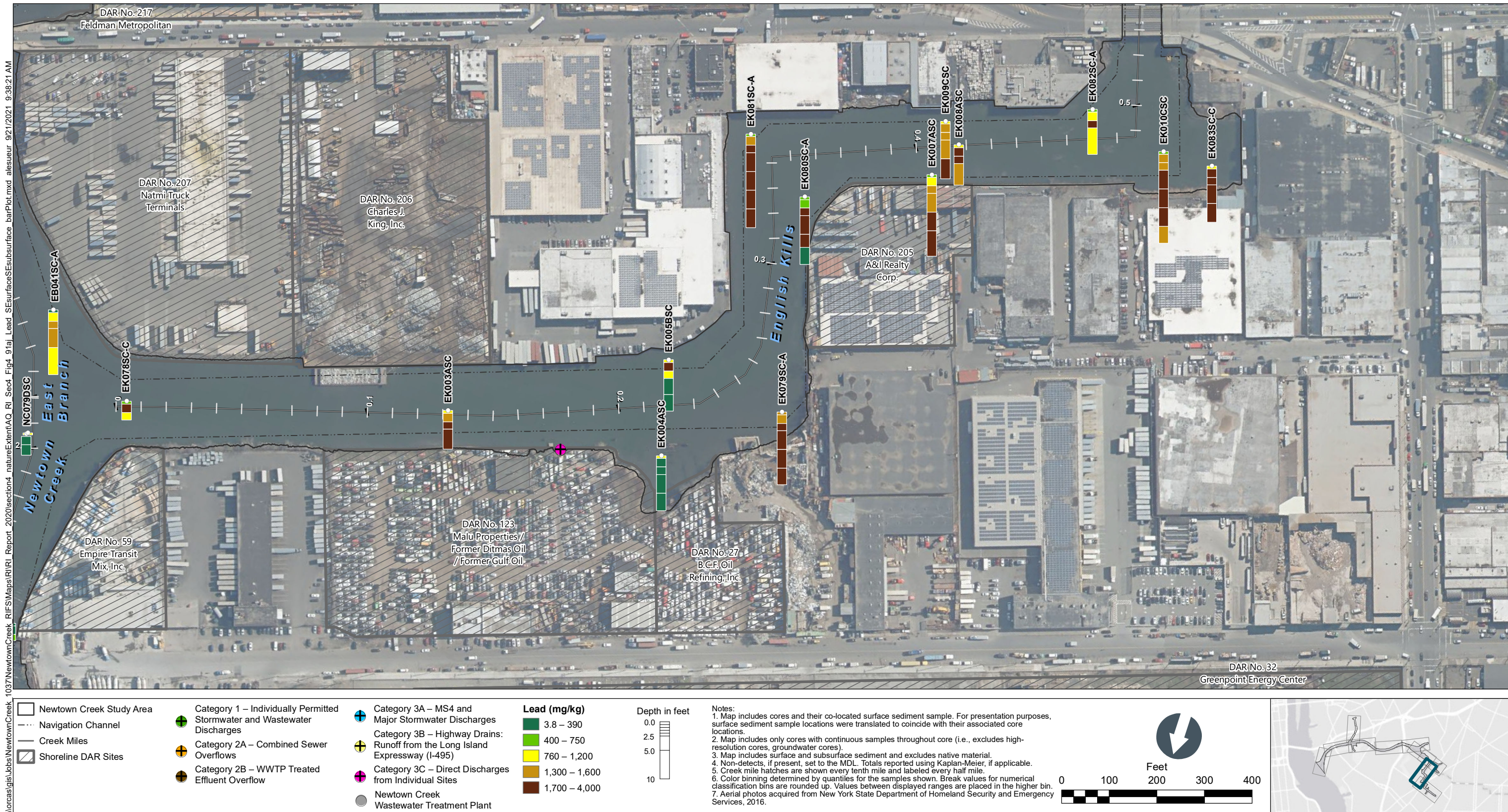
Figure 4-91i Lead in Surface and Subsurface Sediment Bar Plots by Depth – Plan View of English Kills CM 0 to 0.5 Remedial Investigation Report Newtown Creek RI/FS
