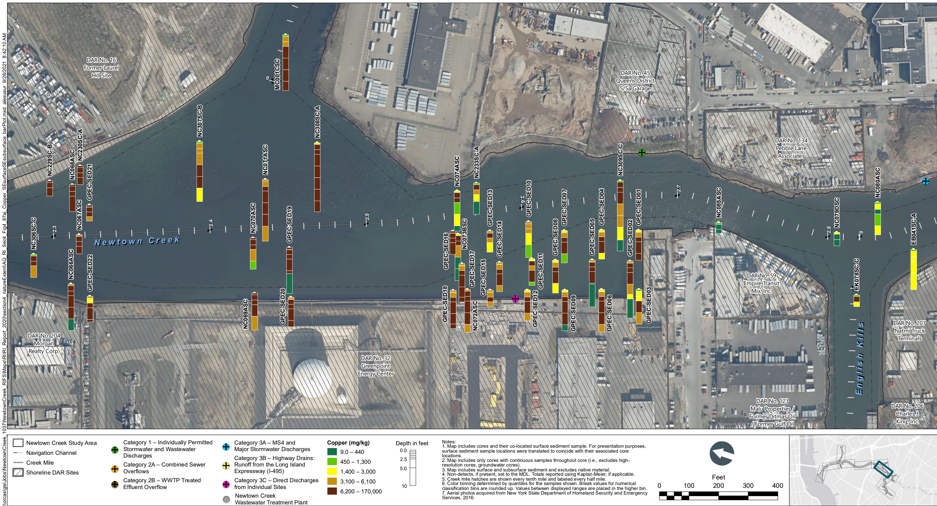
Figure 4-87g Copper in Surface and Subsurface Sediment Bar Plots by Depth – Plan View of Newtown Creek CM 2.3 to 2.8 Remedial Investigation Report Newtown Creek RI/FS
