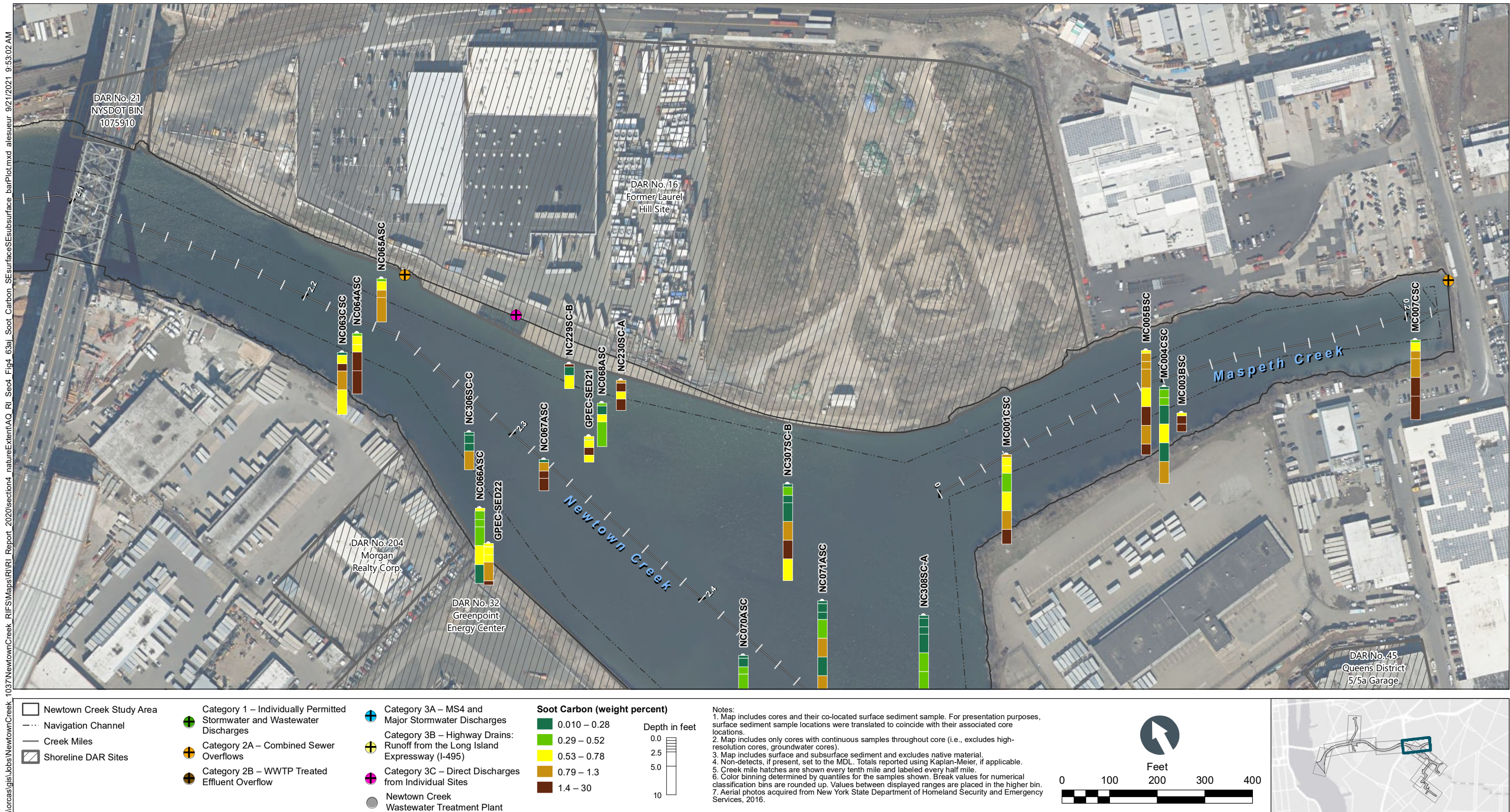
Figure 4-63f Percent Soot Carbon in Surface and Subsurface Sediment Bar Plots by Depth – Plan View of Maspeth Creek and Newtown Creek CM 2.1 to 2.4 Remedial Investigation Report Newtown Creek RI/FS
