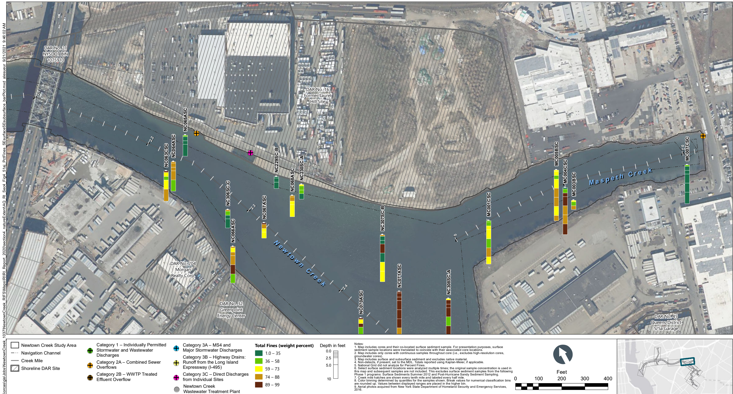
Figure 4-51f Total Percent Fines in Surface and Subsurface Sediment Bar Plots by Depth – Plan View of Maspeth Creek and Newtown Creek CM 2.1 to 2.4 Remedial Investigation Report Newtown Creek RI/FS
