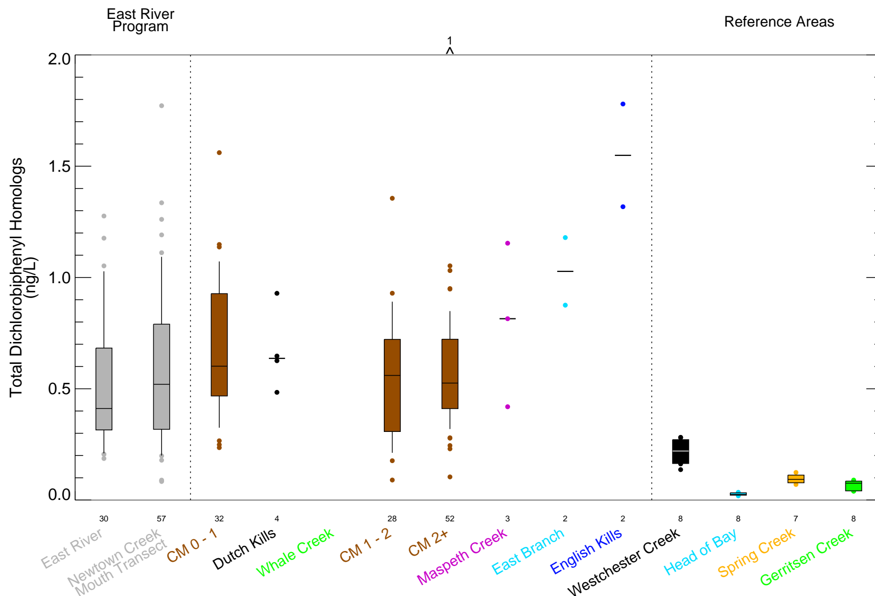
Figure 6-32a Total Dichlorobiphenyl Homologs in Surface Water During Dry Weather Sampling Events - Box Plots by Location Remedial Investigation Report Newtown Creek RI/FS
