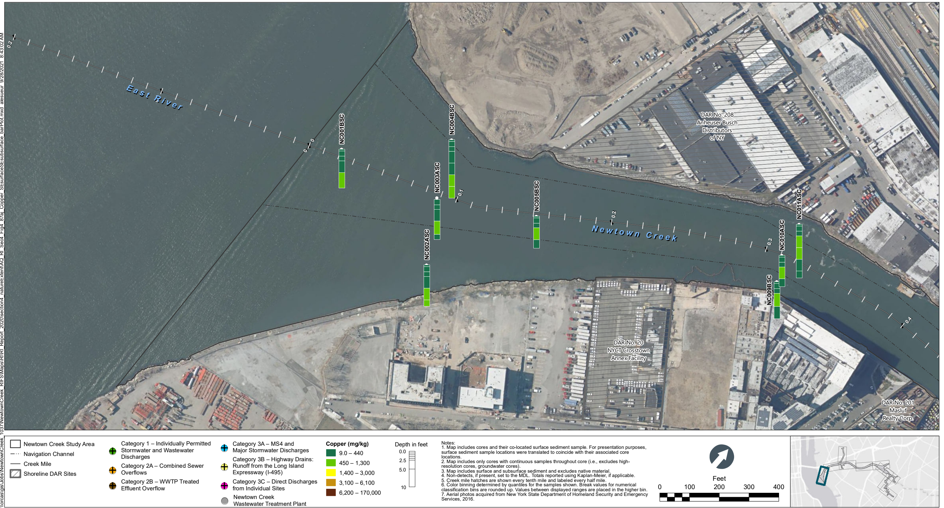
Figure 4-87a Copper in Surface and Subsurface Sediment Bar Plots by Depth – Plan View of Newtown Creek CM 0 to 0.4 Remedial Investigation Report Newtown Creek RI/FS
