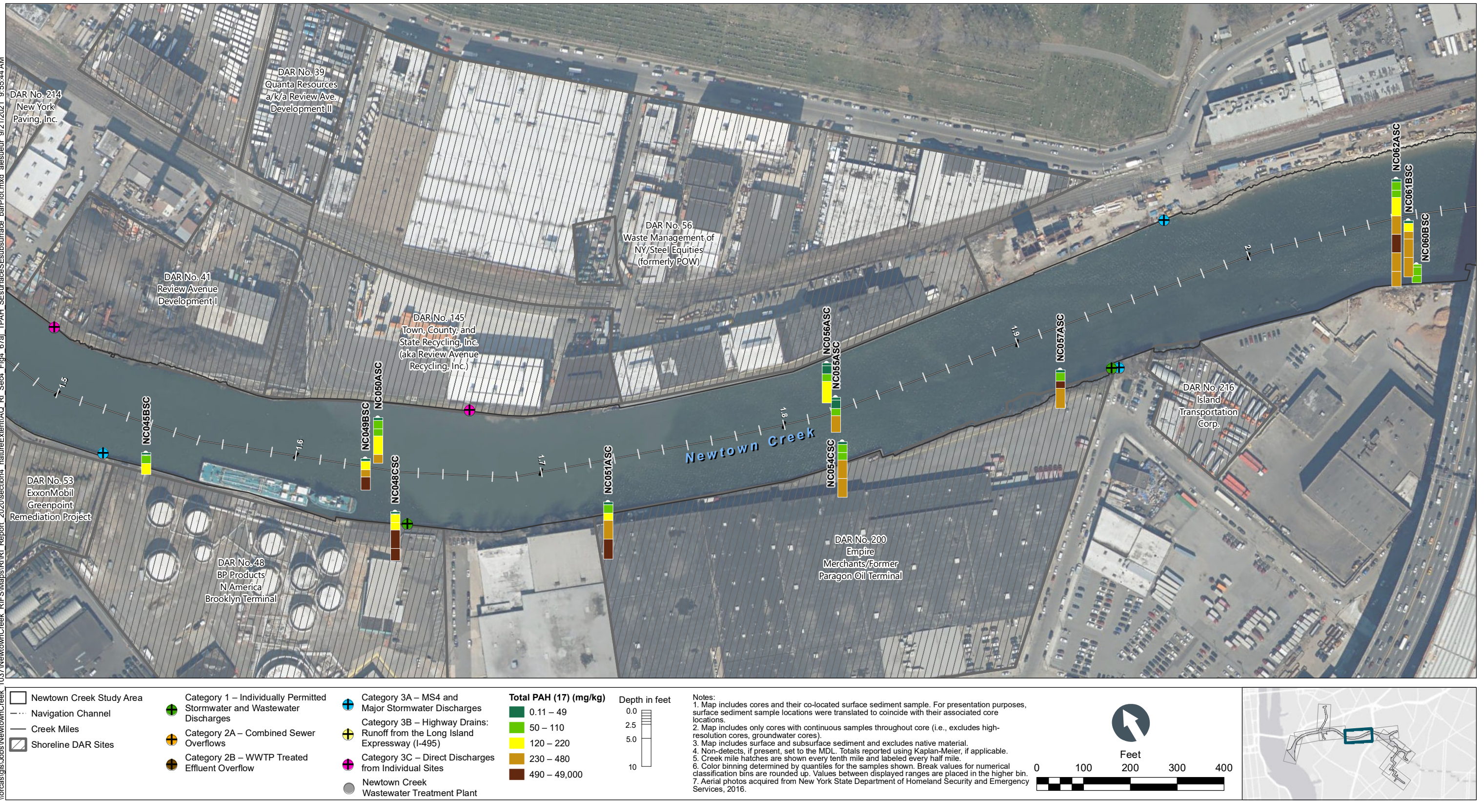
Figure 4-67e Total PAH (17) in Surface and Subsurface Sediment Bar Plots by Depth – Plan View of Newtown Creek CM 1.5 to 2.0 Remedial Investigation Report Newtown Creek RI/FS
