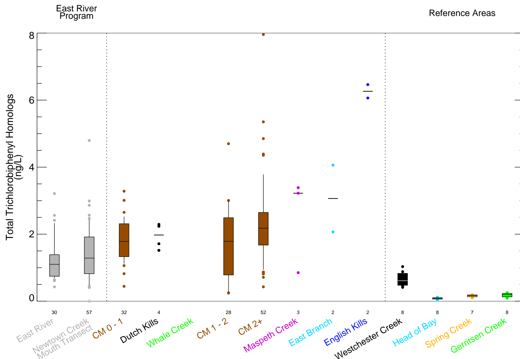
Figure 6-32b Total Trichlorobiphenyl Homologs in Surface Water During Dry Weather Sampling Events - Box Plots by Location Remedial Investigation Report Newtown Creek RI/FS
