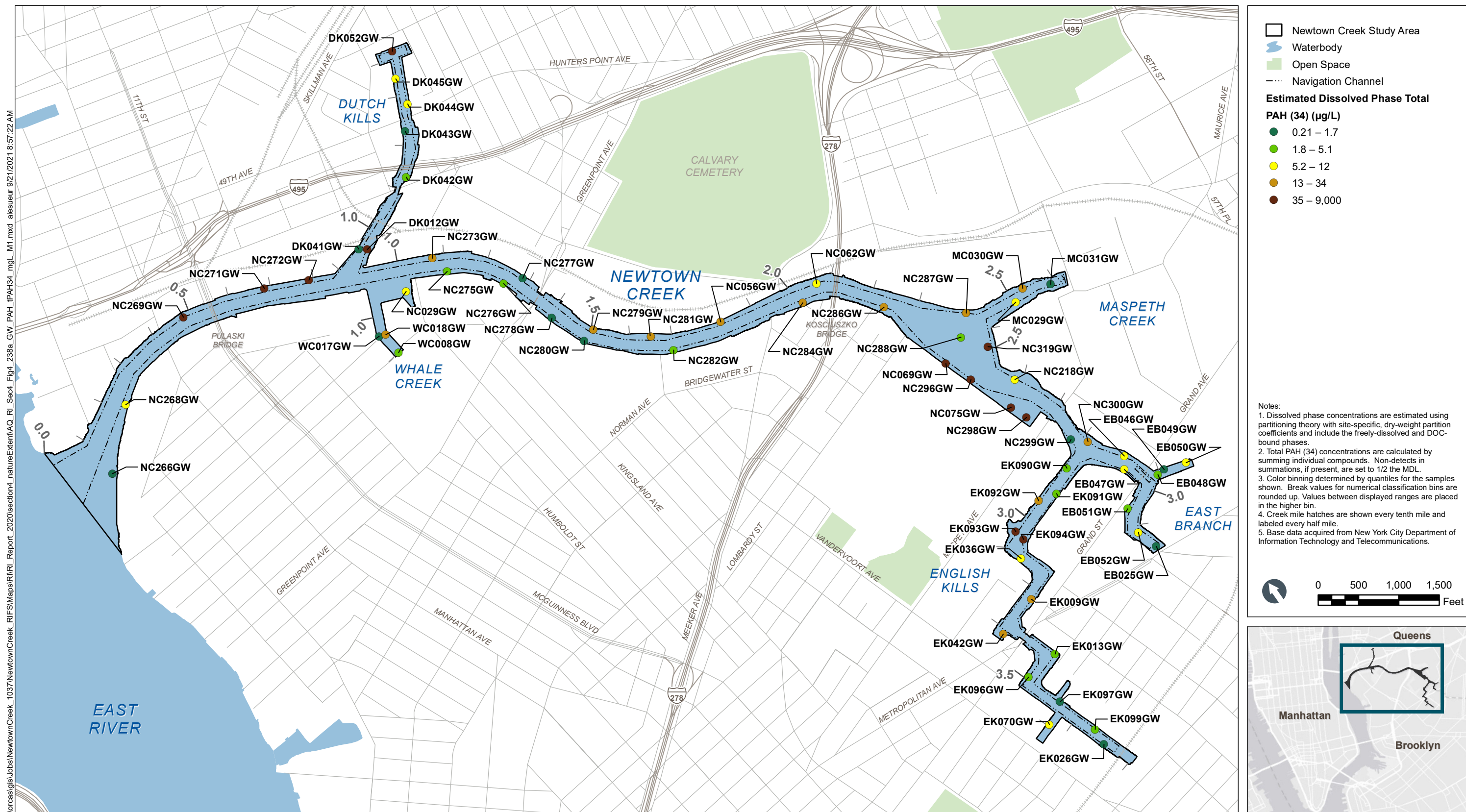
Figure 4-238a Estimated Dissolved Phase (Method 1) Total PAH (34) in Groundwater – Plan View Remedial Investigation Report Newtown Creek RI/FS
