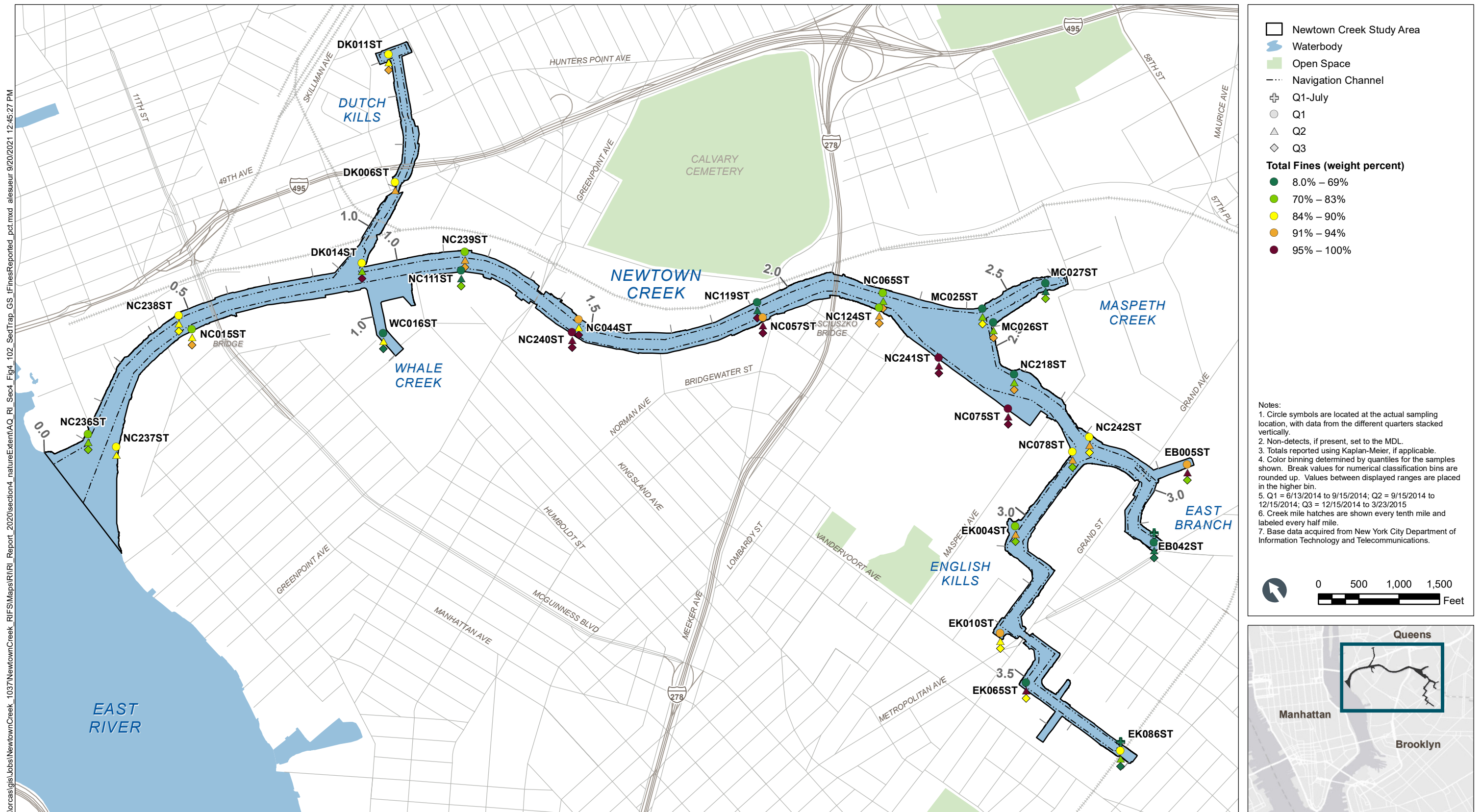
Figure 4-102 Spatial Pattern of Percent Fines in Sediment Traps – Plan View Remedial Investigation Report Newtown Creek RI/FS
