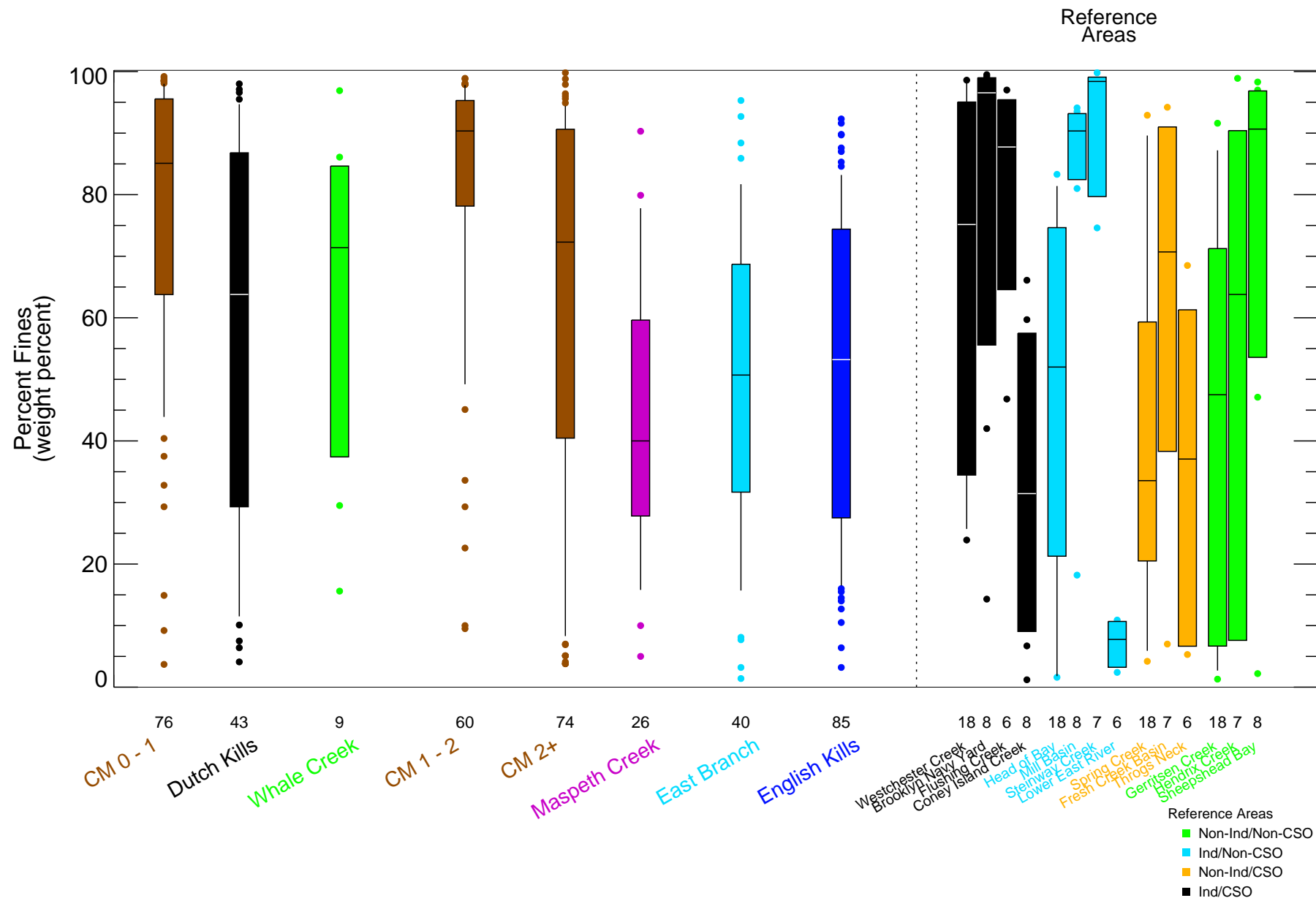
Figure 4-6 Percent Fines in Surface Sediment - Box Plots by Location Remedial Investigation Report Newtown Creek RI/FS
