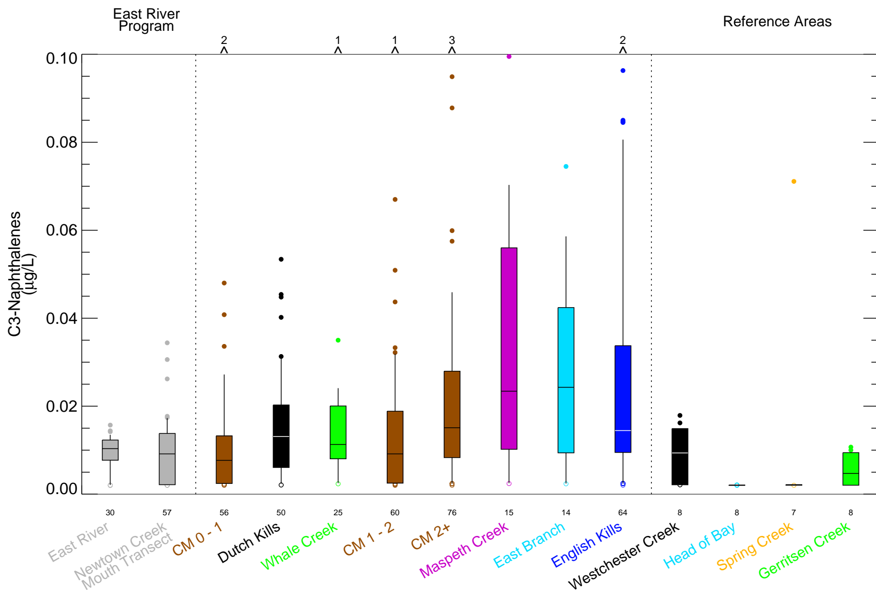
Figure 6-31e C3-Naphthalenes in Surface Water During Dry Weather Sampling Events - Box Plots by Location Remedial Investigation Report Newtown Creek RI/FS
