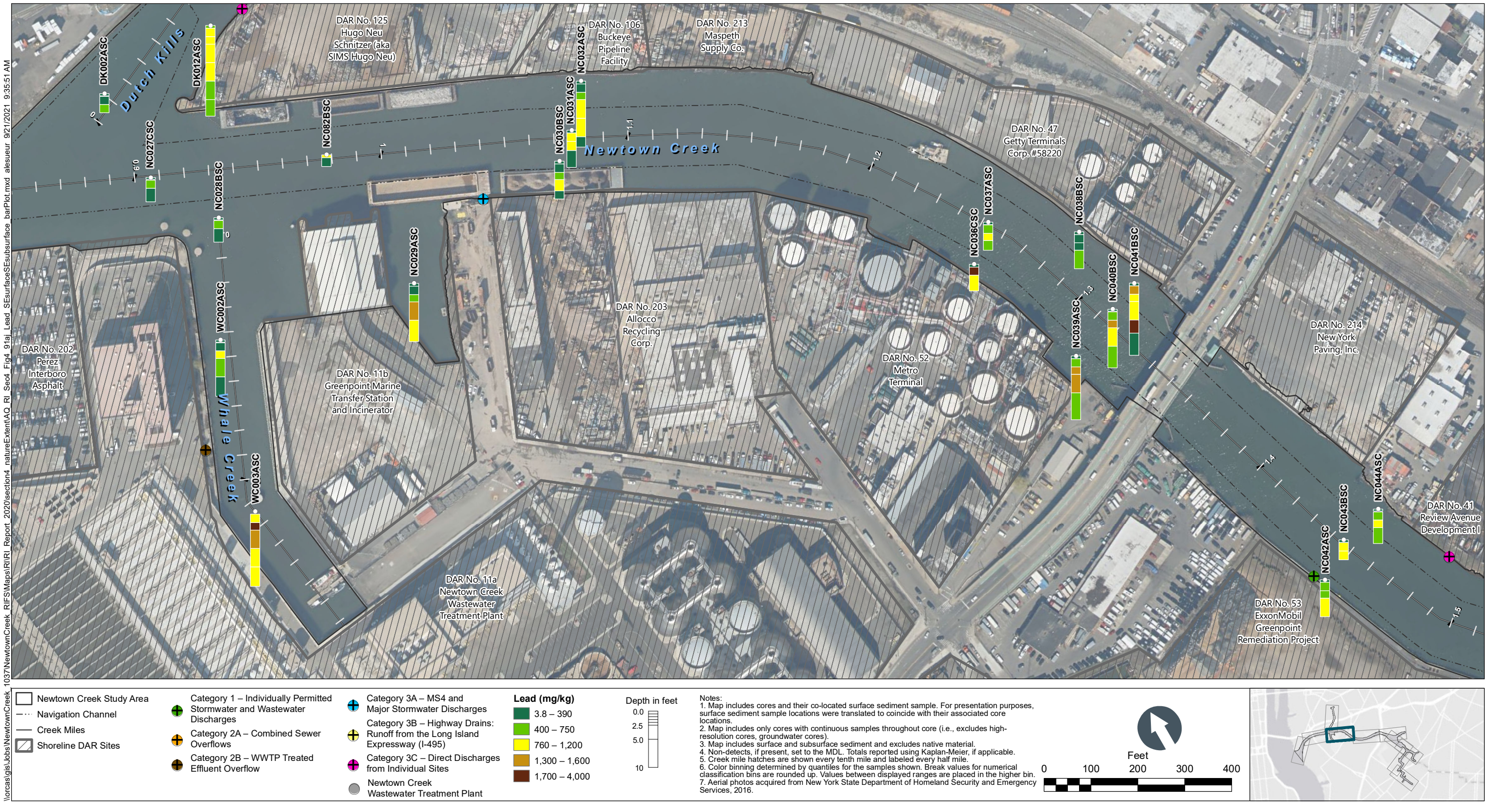
Figure 4-91c Lead in Surface and Subsurface Sediment Bar Plots by Depth – Plan View of Whale Creek and Newtown Creek CM 0.9 to 1.5 Remedial Investigation Report Newtown Creek RI/FS
