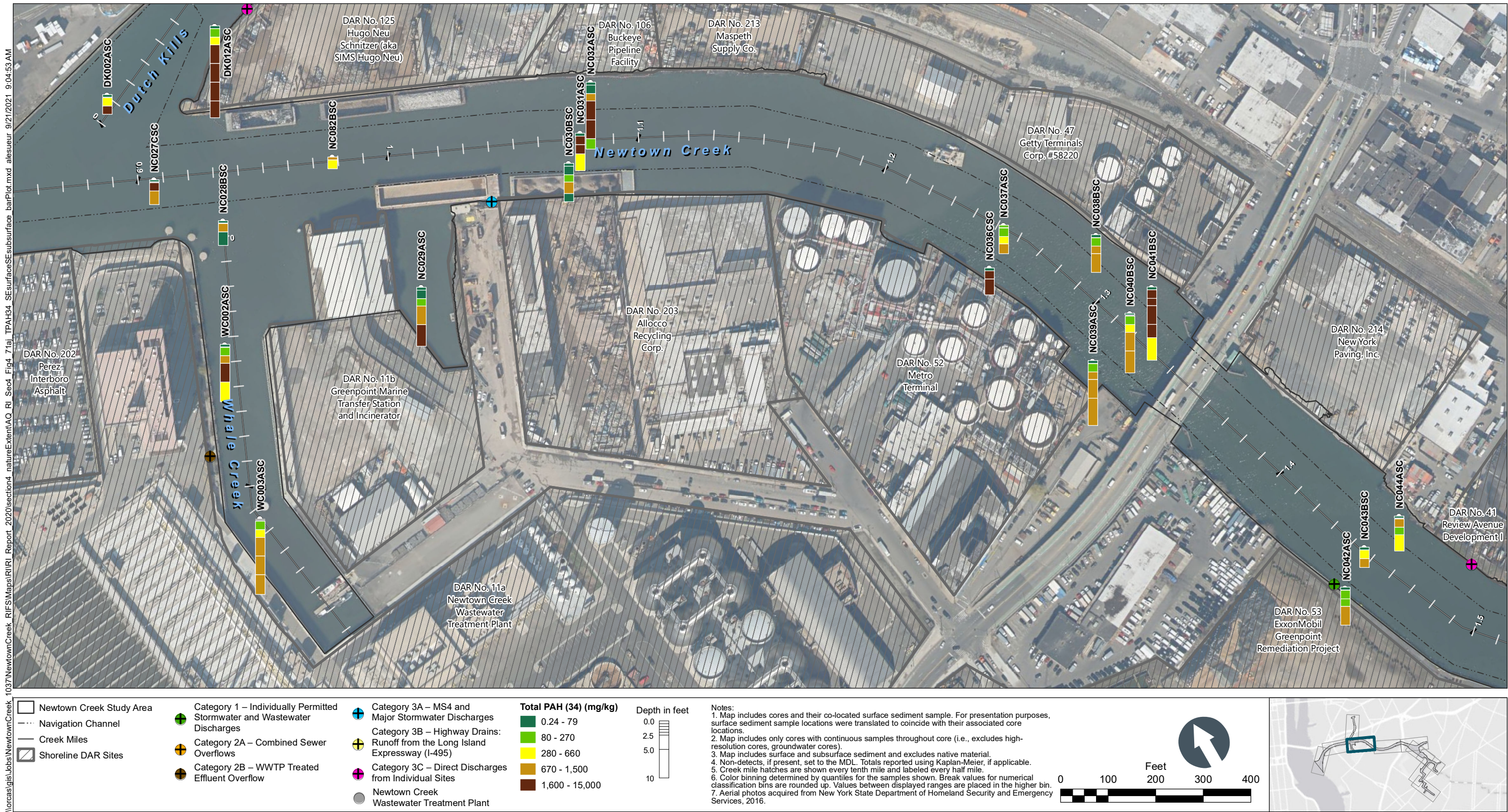
Figure 4-71c Total PAH (34) in Surface and Subsurface Sediment Bar Plots by Depth – Plan View of Whale Creek and Newtown Creek CM 0.9 to 1.5 Remedial Investigation Report Newtown Creek RI/FS
