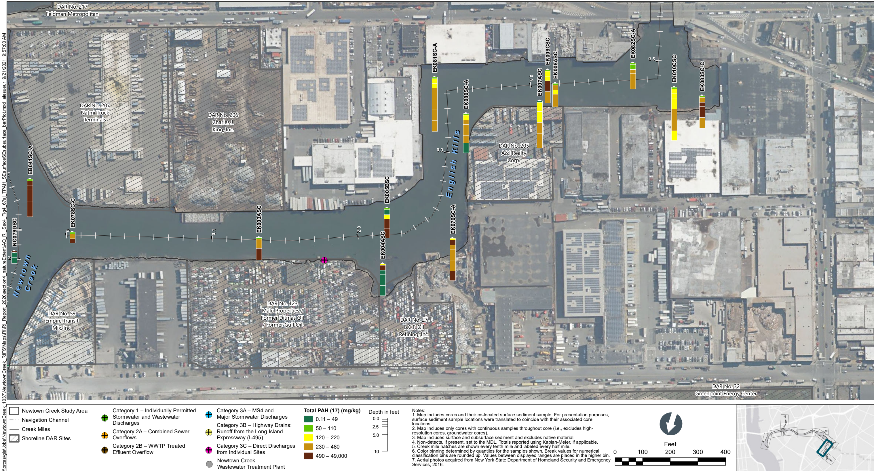
Figure 4-67i Total PAH (17) in Surface and Subsurface Sediment Bar Plots by Depth – Plan View of English Kills CM 0 to 0.5 Remedial Investigation Report Newtown Creek RI/FS
