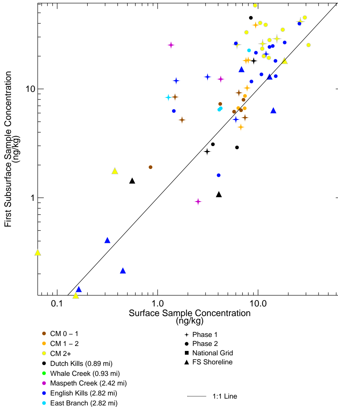
Figure 4-97 2,3,7,8-TCDD in Surface Sediment versus 2,3,7,8-TCDD in First Subsurface Interval – Cross Plot Remedial Investigation Report Newtown Creek RI/FS
