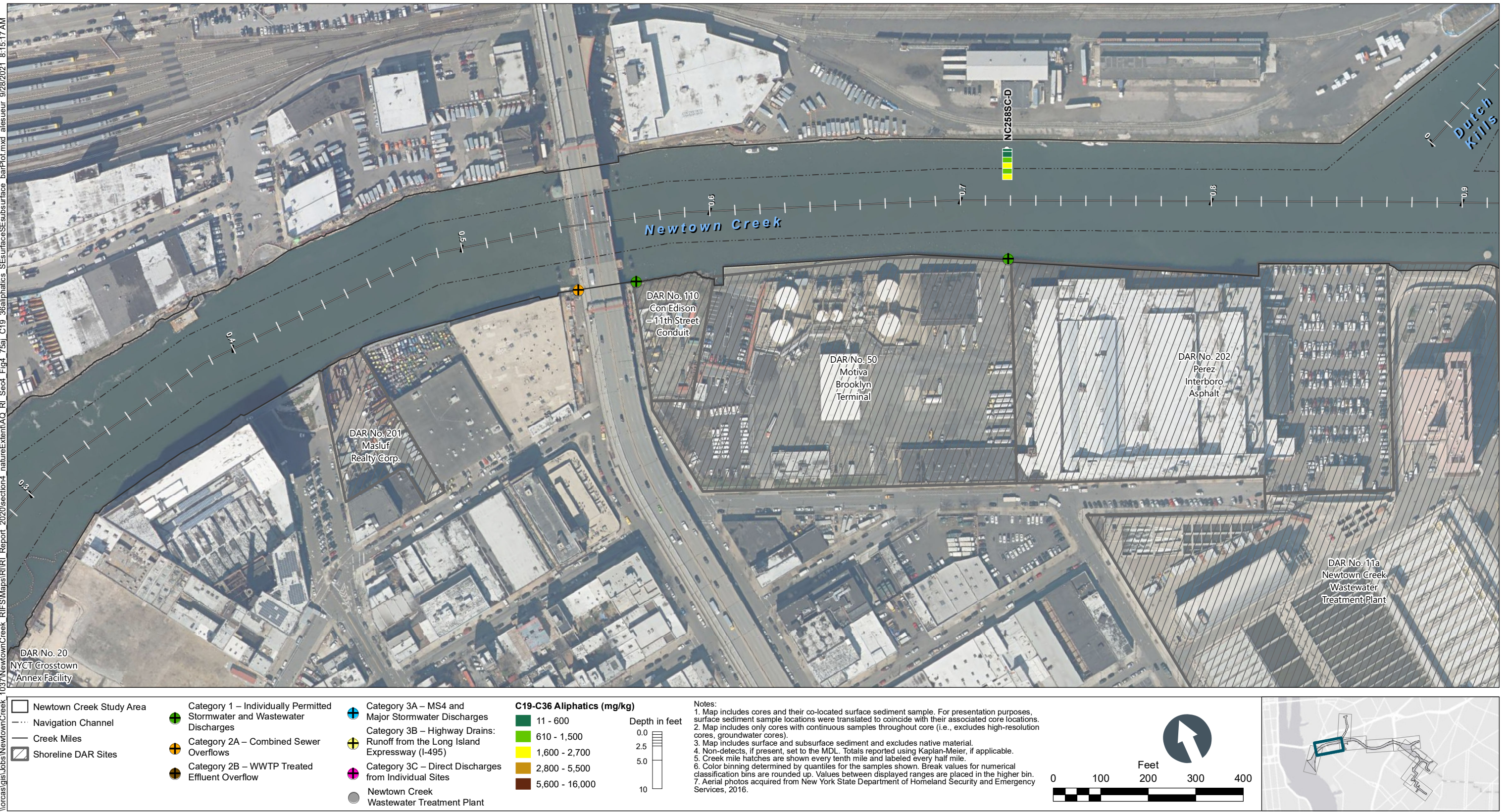
Figure 4-75b C19-C36 Aliphatics in Surface and Subsurface Sediment Bar Plots by Depth – Plan View of Newtown Creek CM 0.3 to 0.9 Remedial Investigation Report Newtown Creek RI/FS
