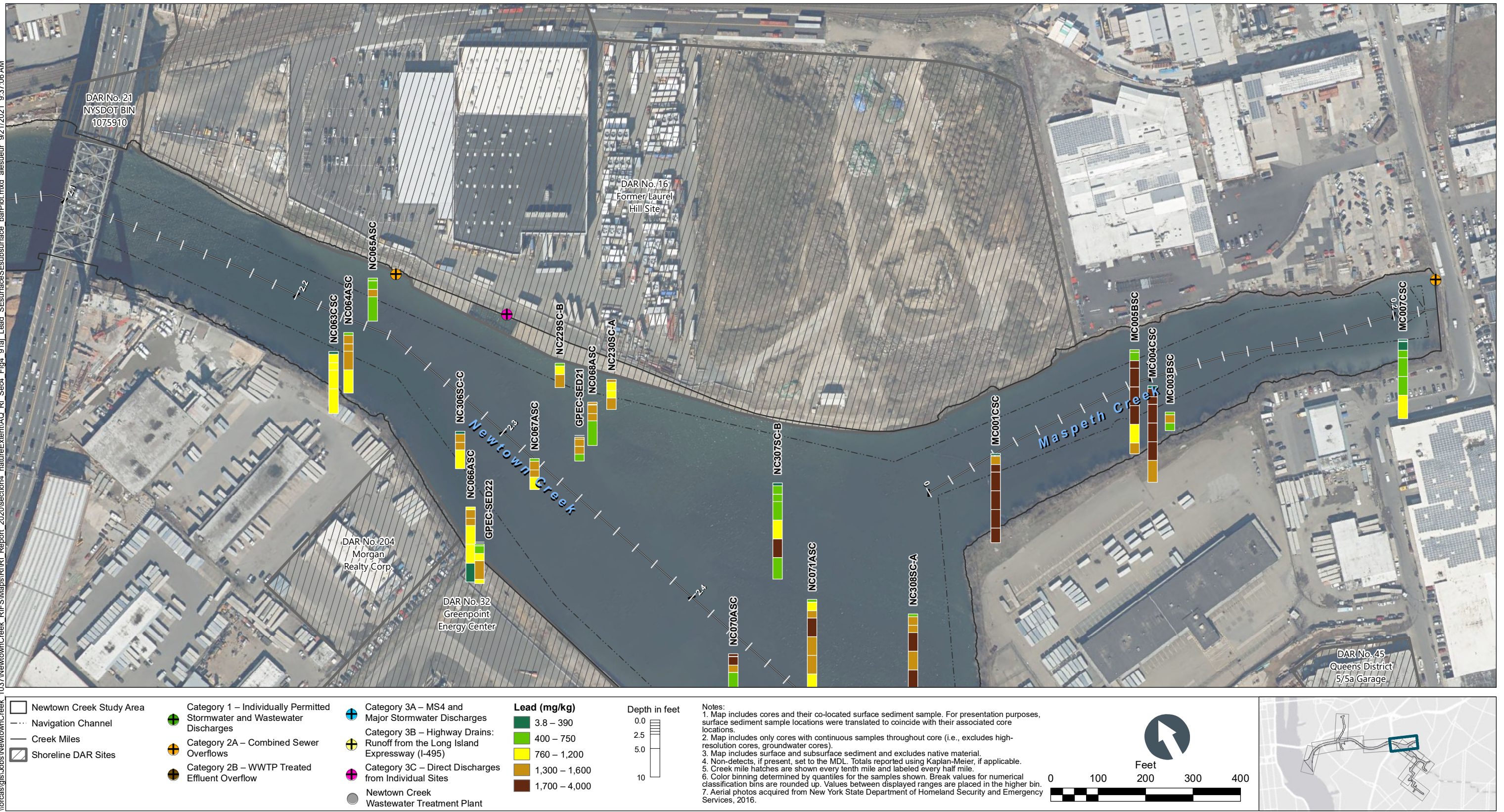
Figure 4-91f Lead in Surface and Subsurface Sediment Bar Plots by Depth – Plan View of Maspeth Creek and Newtown Creek CM 2.1 to 2.4 Remedial Investigation Report Newtown Creek RI/FS
