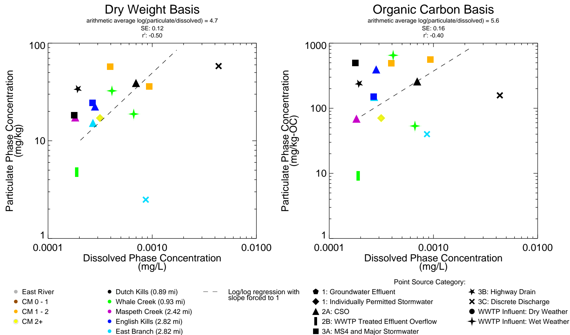
Figure 6-11a Point Source Particulate Phase versus Dissolved Phase for Total PAH (17) - Cross Plots Remedial Investigation Report Newtown Creek RI/FS
