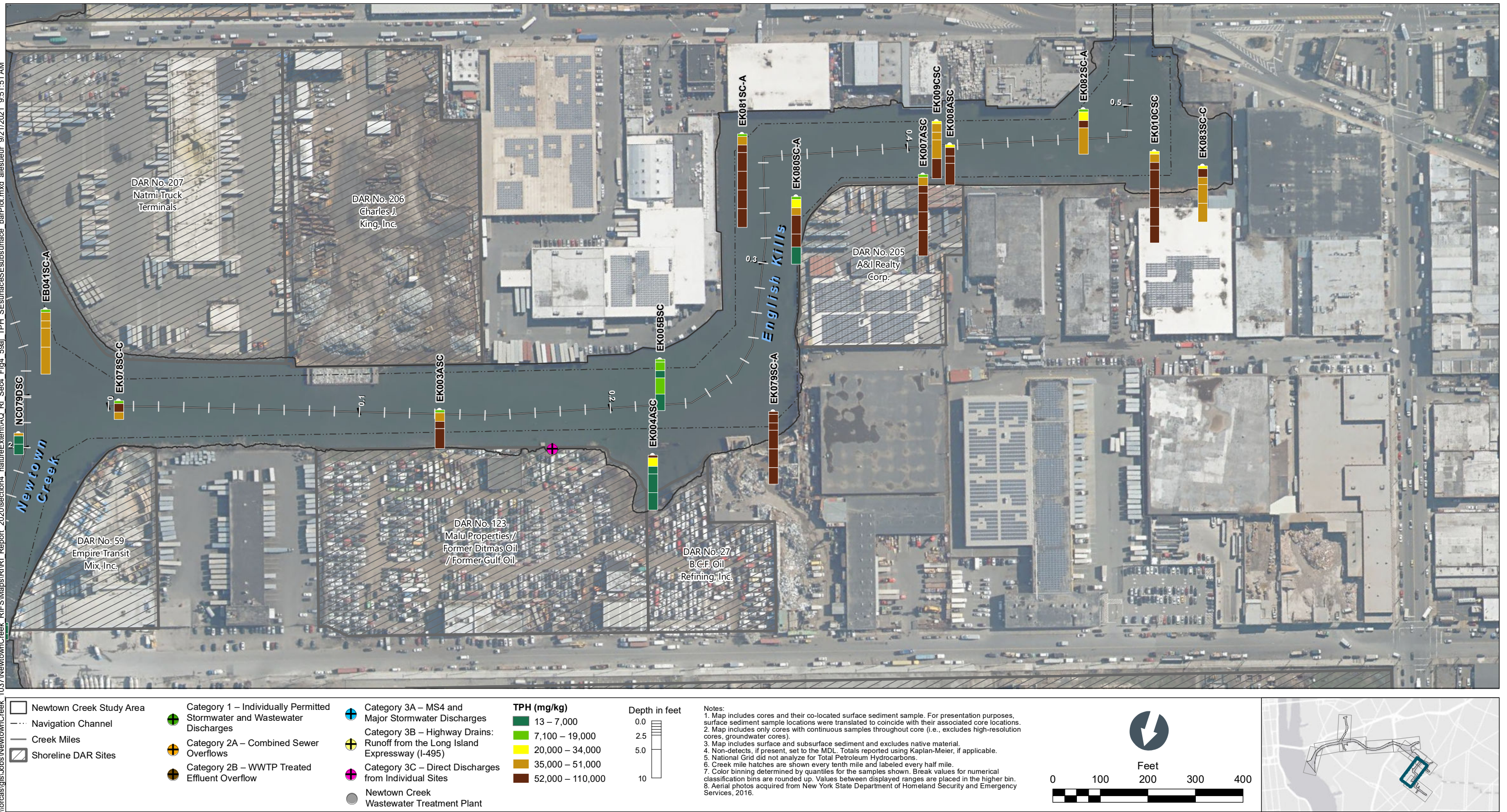
Figure 4-59i TPH in Surface and Subsurface Sediment Bar Plots by Depth – Plan View of English Kills CM 0 to 0.5 Remedial Investigation Report Newtown Creek RI/FS
