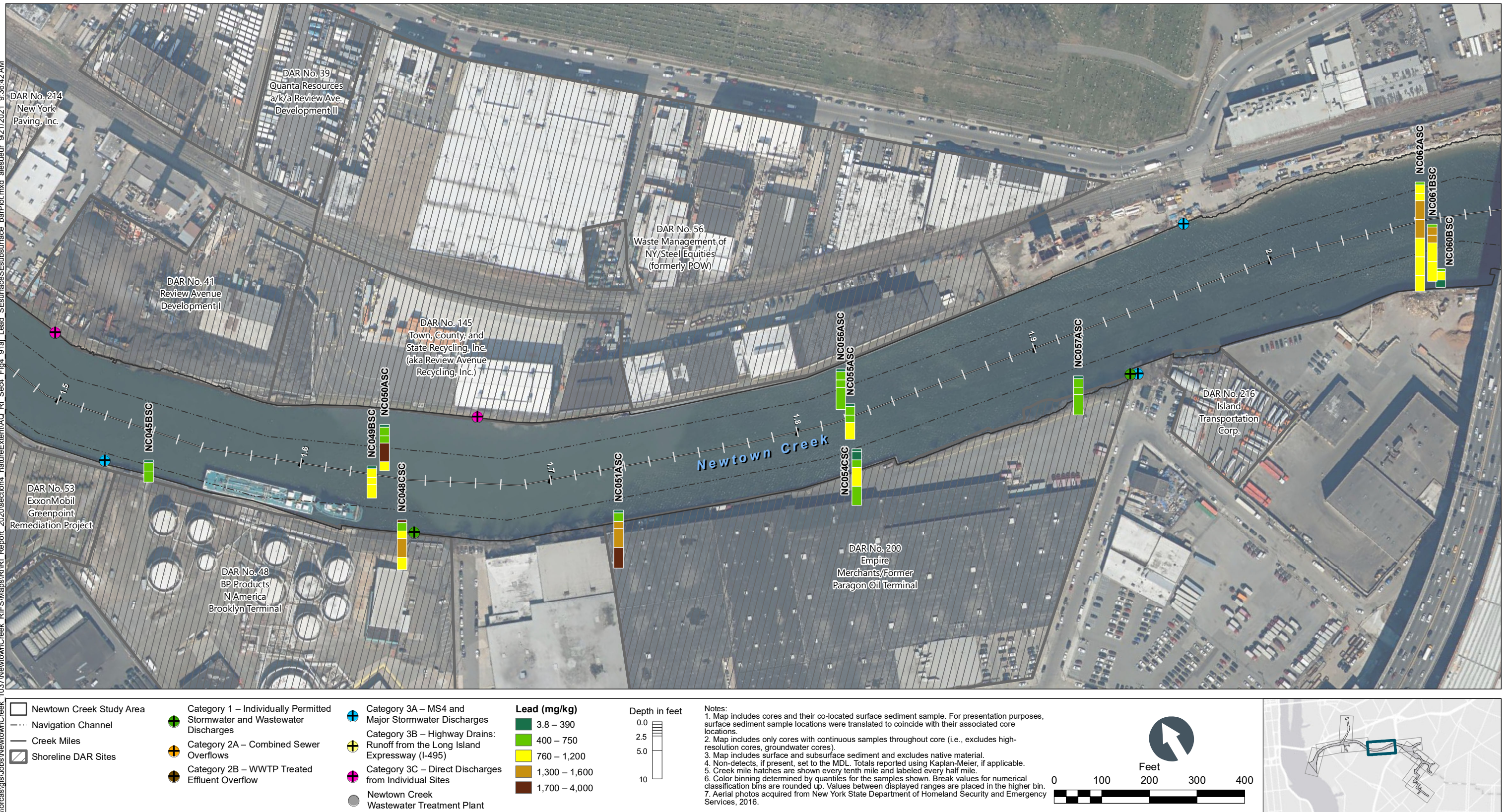
Figure 4-91e Lead in Surface and Subsurface Sediment Bar Plots by Depth – Plan View of Newtown Creek CM 1.5 to 2.0 Remedial Investigation Report Newtown Creek RI/FS
