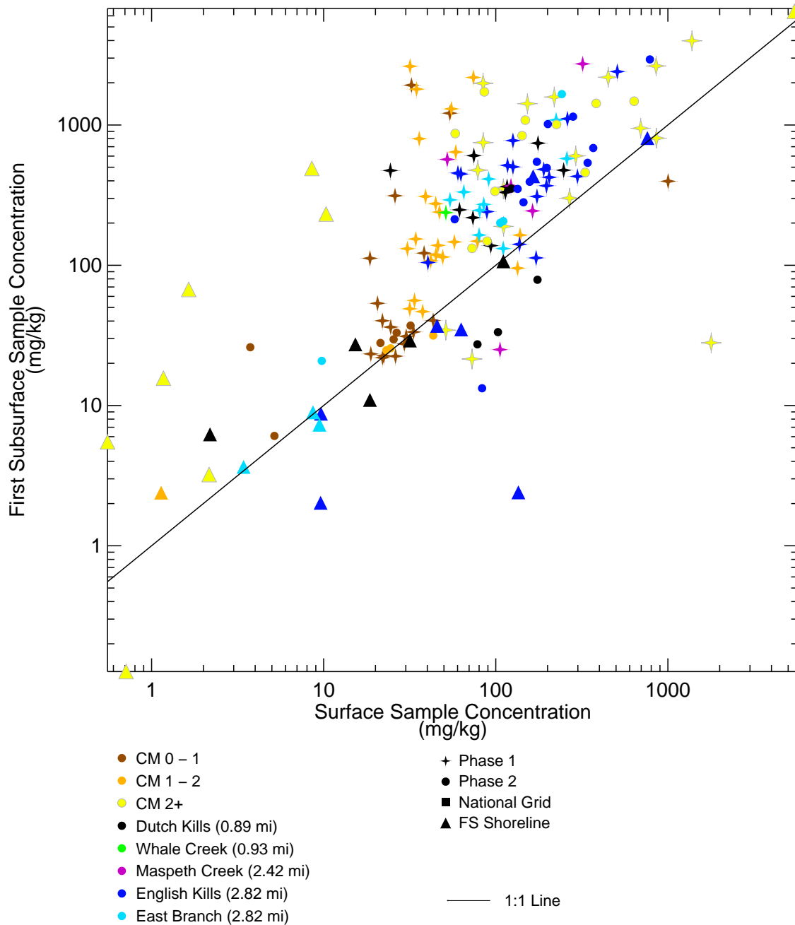
Figure 4-94 Total PAH (34) in Surface Sediment versus Total PAH (34) in First Subsurface Interval – Cross Plot Remedial Investigation Report Newtown Creek RI/FS
