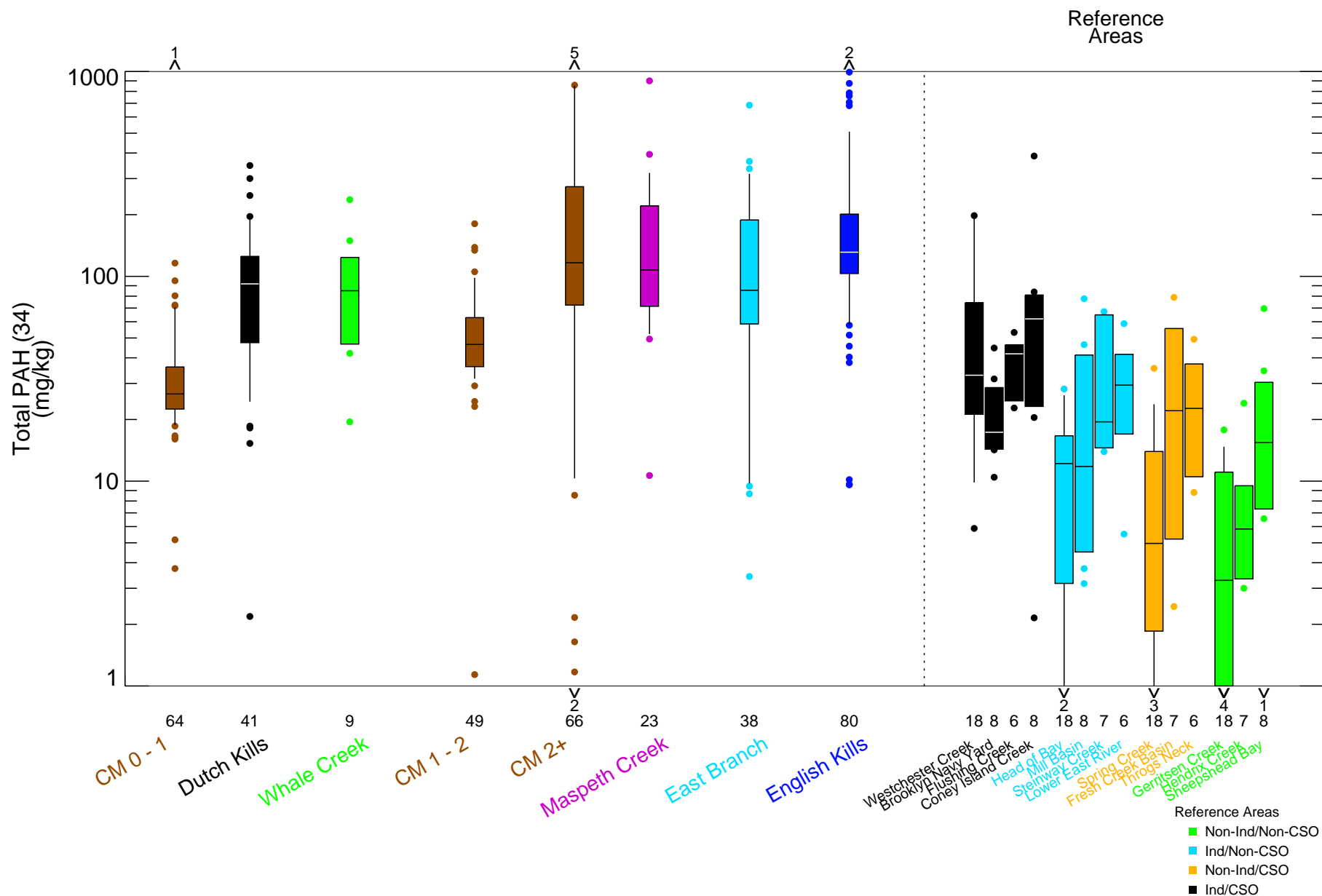
Figure 4-20 Total PAH (34) in Surface Sediment - Box Plots by Location Remedial Investigation Report Newtown Creek RI/FS
