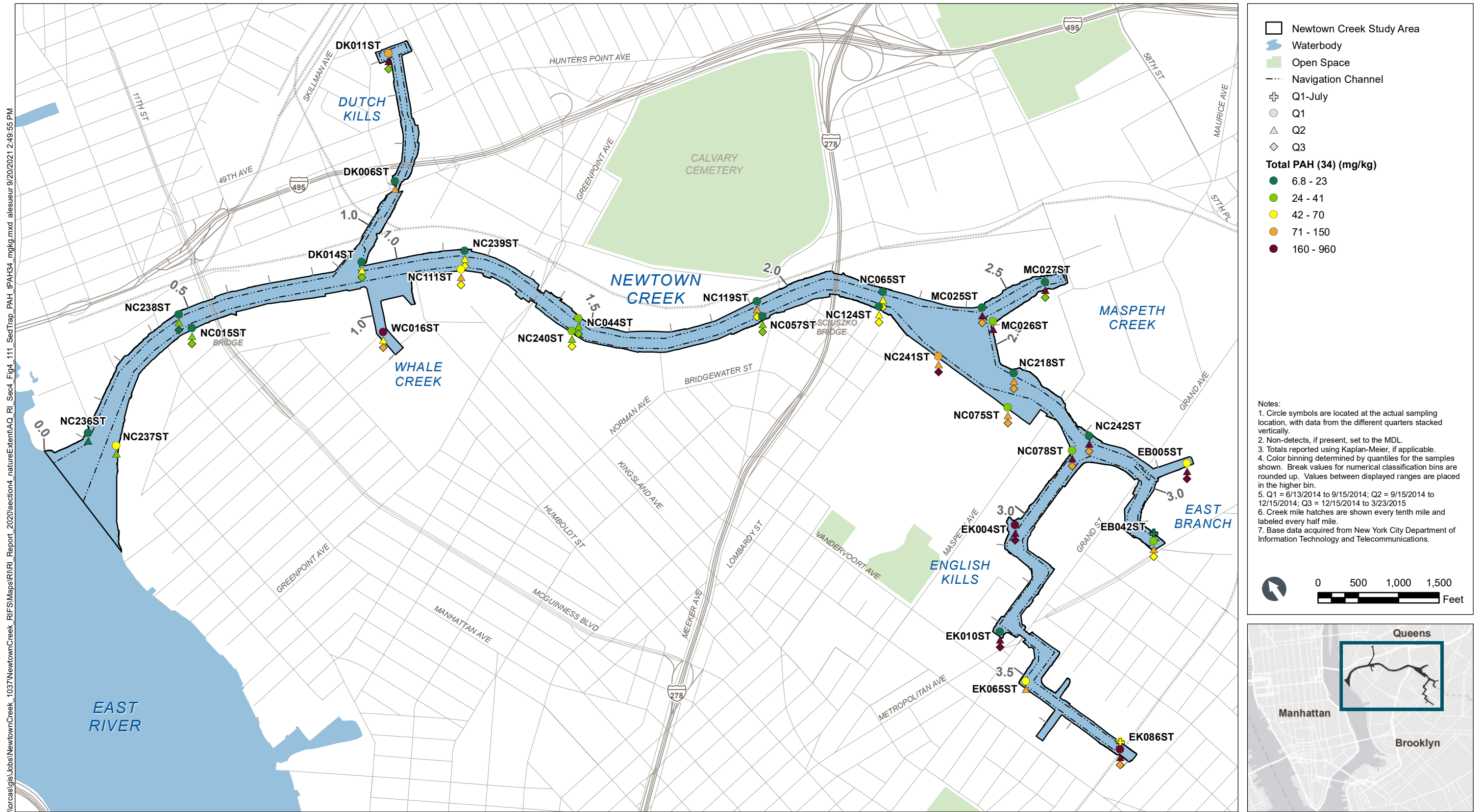
Figure 4-111 Spatial Patterns of Total PAH (34) in Sediment Traps – Plan View Remedial Investigation Report Newtown Creek RI/FS
