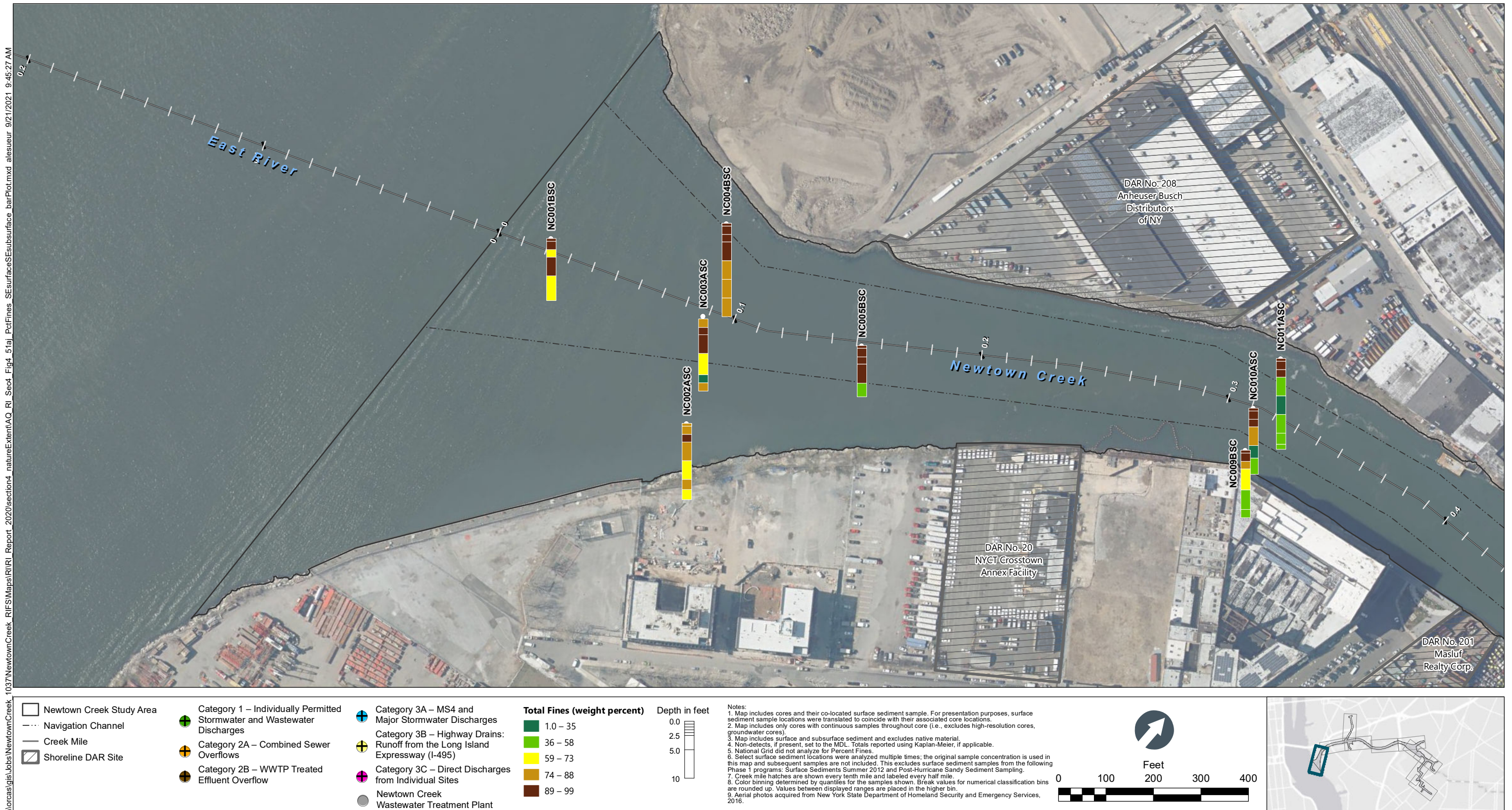
Figure 4-51a Total Percent Fines in Surface and Subsurface Sediment Bar Plots by Depth – Plan View of Newtown Creek CM 0 to 0.4 Remedial Investigation Report Newtown Creek RI/FS
