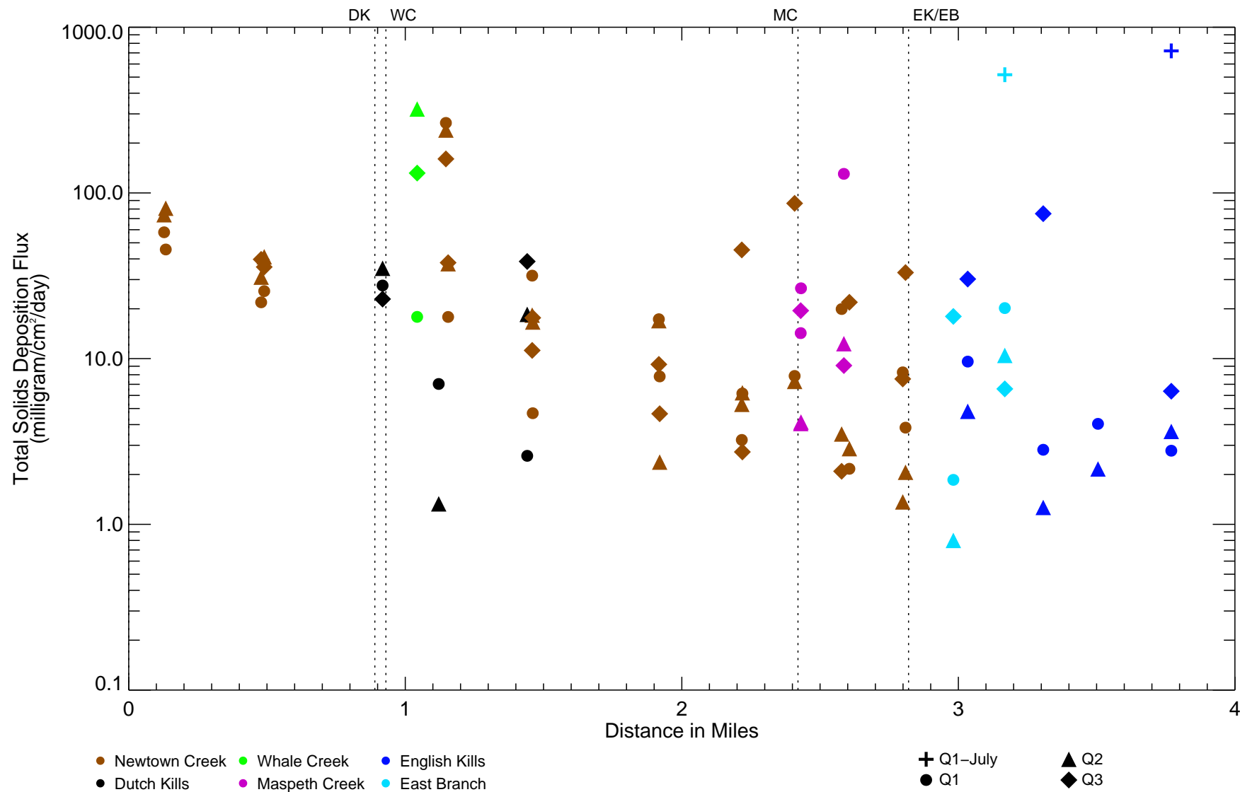
Figure 4-101 Spatial Pattern of Gross Solids Deposition (Mass) in Sediment Traps – Longitudinal Profile Remedial Investigation Report Newtown Creek RI/FS
