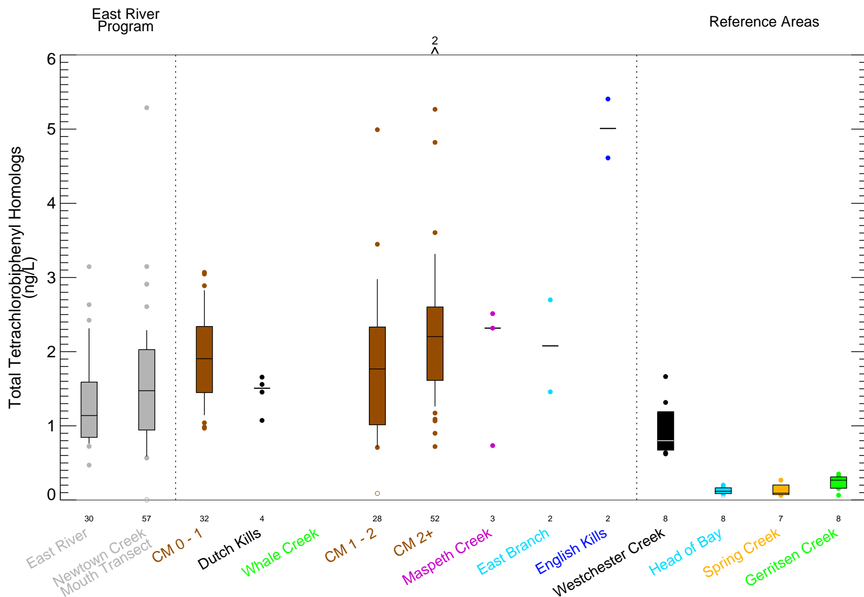
Figure 6-32c Total Tetrachlorobiphenyl Homologs in Surface Water During Dry Weather Sampling Events - Box Plots by Location Remedial Investigation Report Newtown Creek RI/FS
