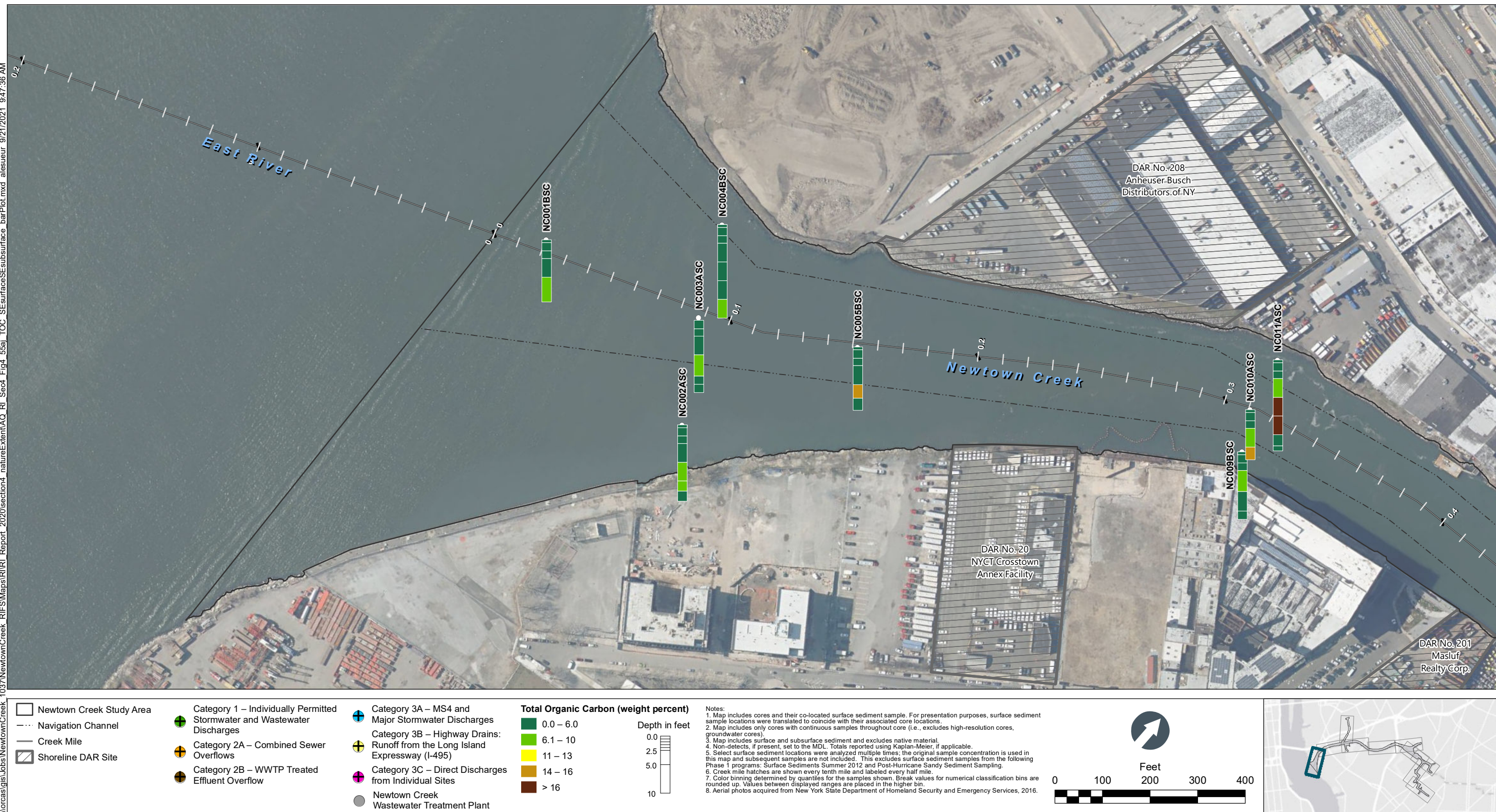
Figure 4-55a TOC in Surface and Subsurface Sediment Bar Plots by Depth – Plan View of Newtown Creek CM 0 to 0.4 Remedial Investigation Report Newtown Creek RI/FS
