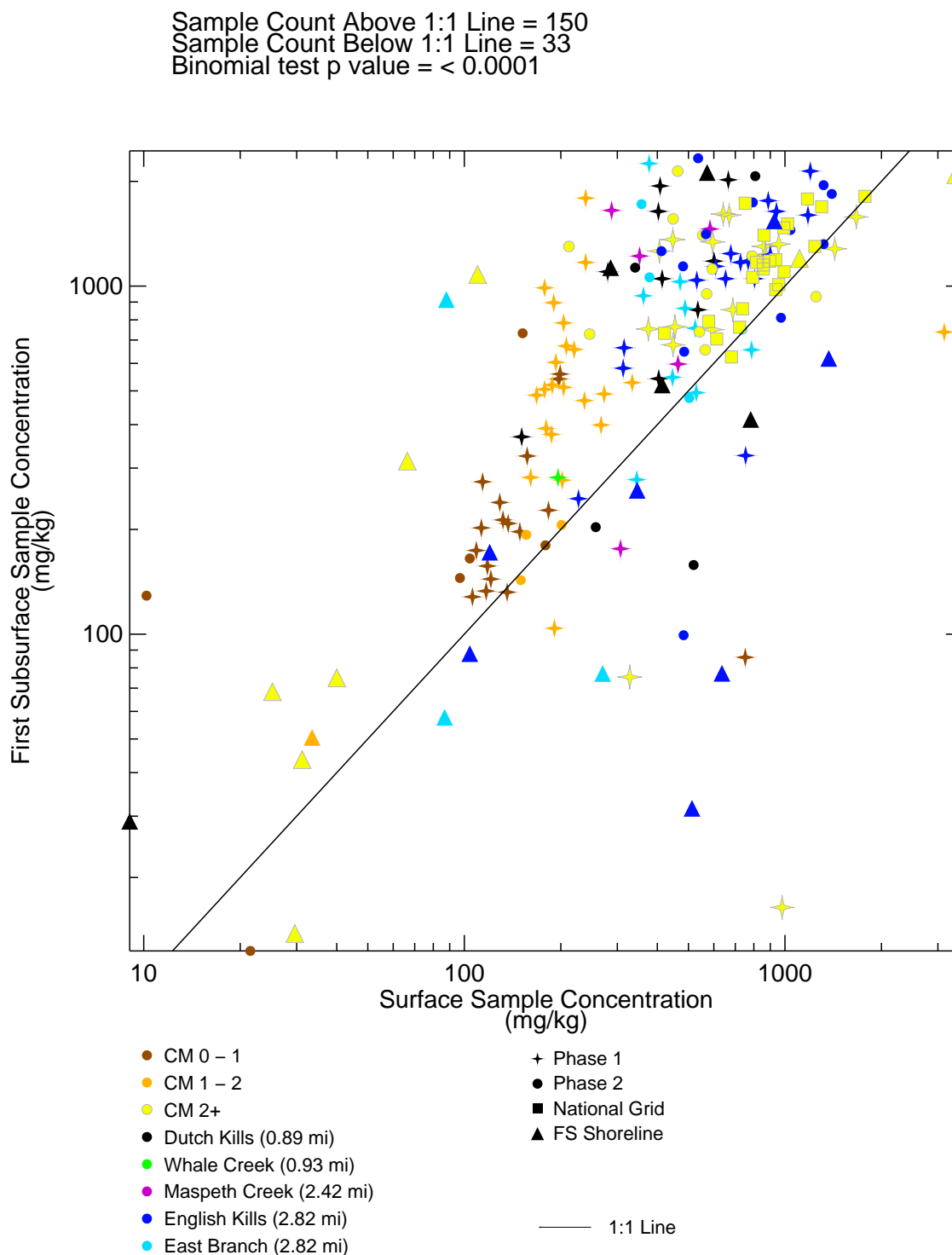
Figure 4–99 Lead in Surface Sediment versus Lead in First Subsurface Interval – Cross Plot Remedial Investigation Report Newtown Creek RI/FS
