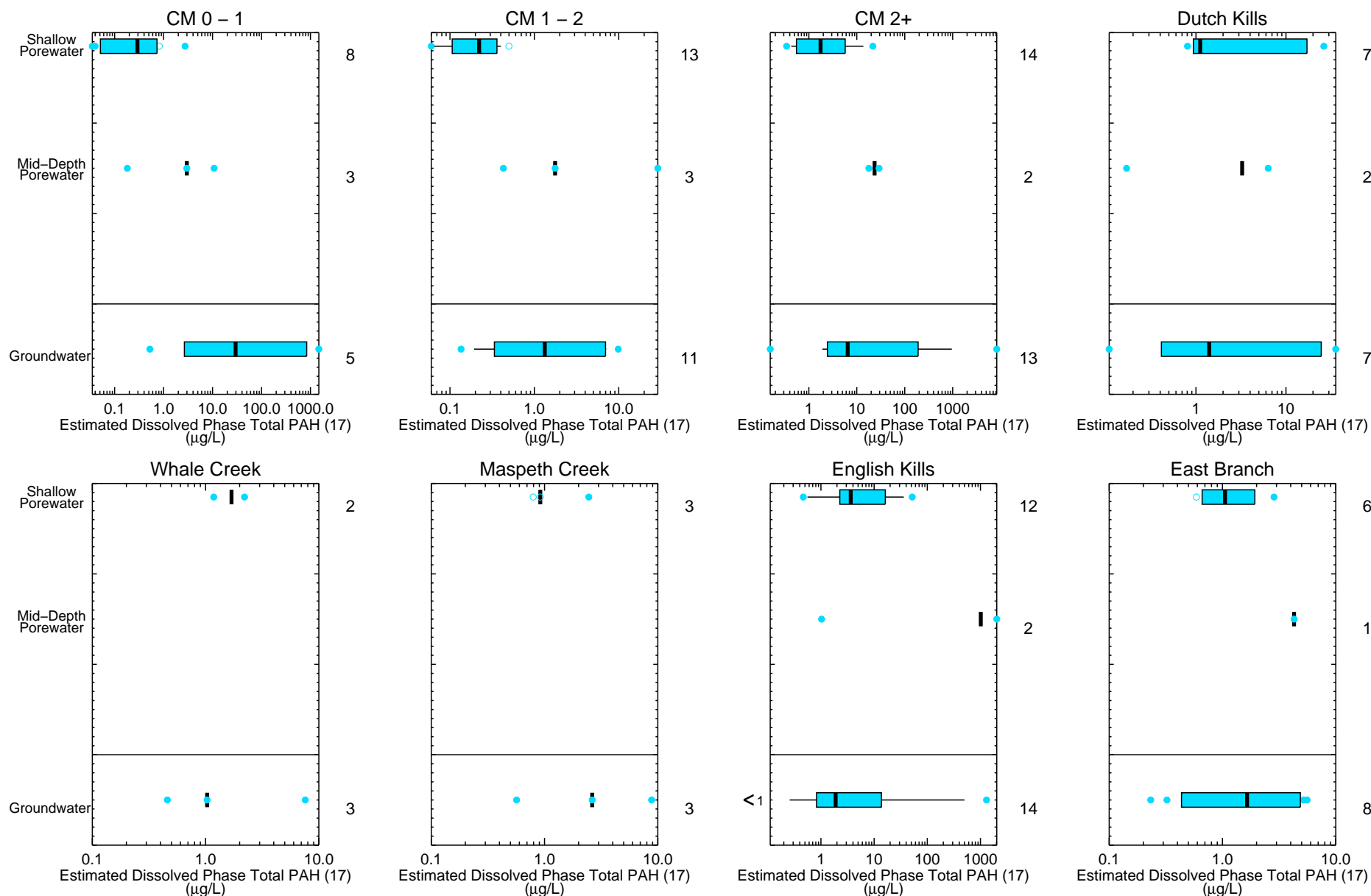
Figure 4-237a Estimated Dissolved Phase (Method 1) Total PAH (17) in Porewater and Groundwater – Box Plot Depth Profiles Remedial Investigation Report Newtown Creek RI/FS
