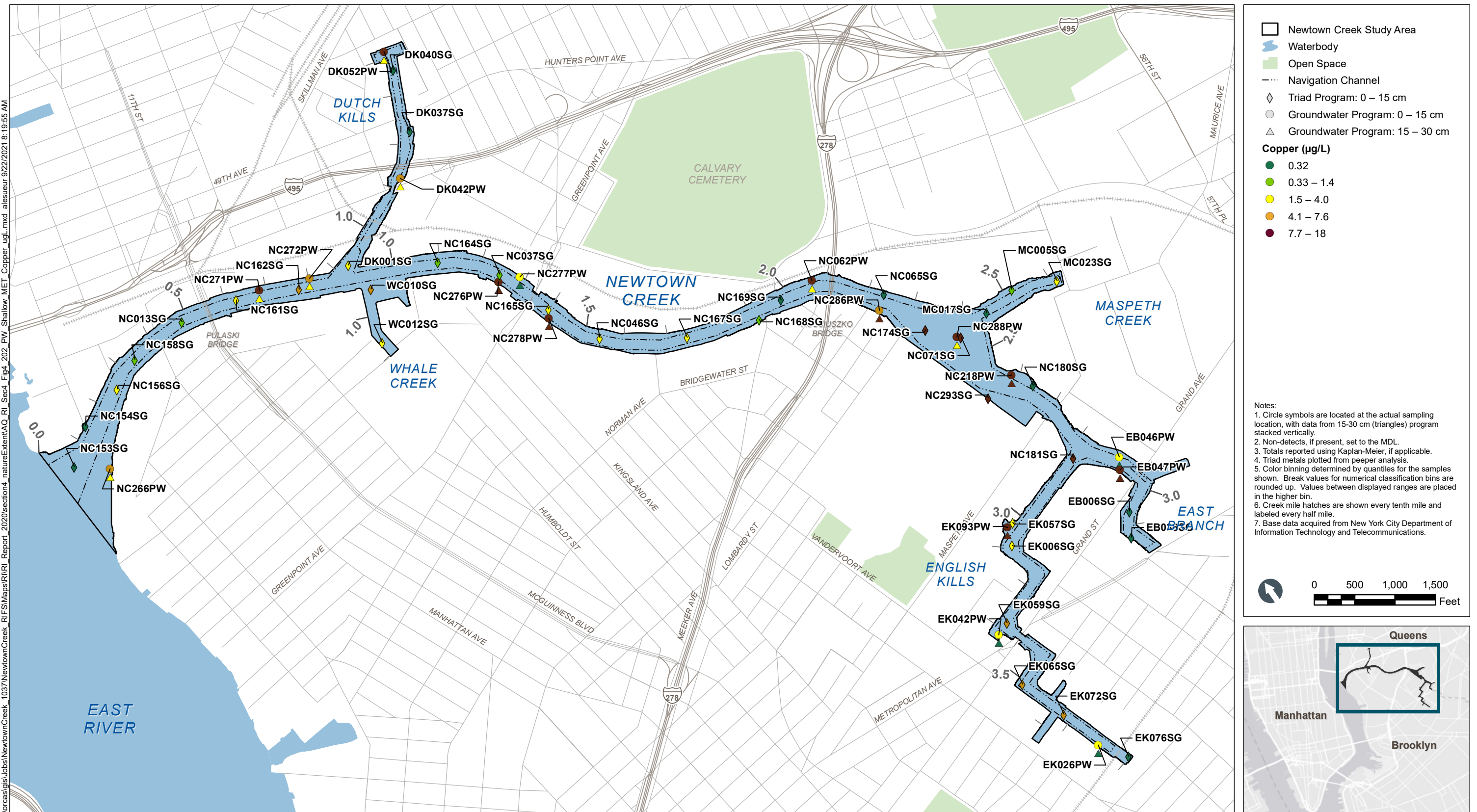
Figure 4-202 Copper in Shallow Porewater – Plan View Remedial Investigation Report Newtown Creek RI/FS
