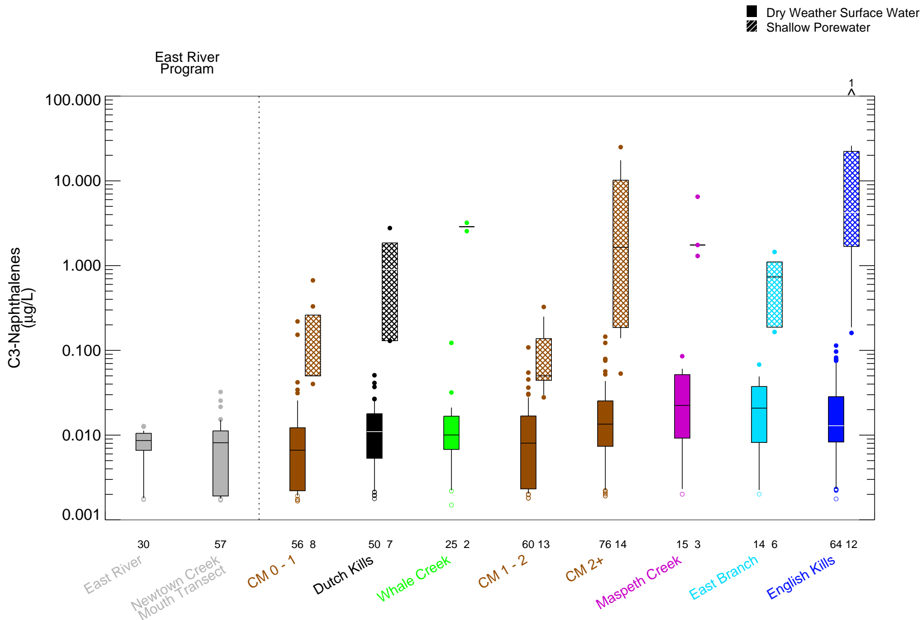
Figure 6-24c Dissolved Phase C3-Naphthalenes in Surface Water Dry Weather and Shallow Porewater - Box Plots Remedial Investigation Report Newtown Creek RI/FS
