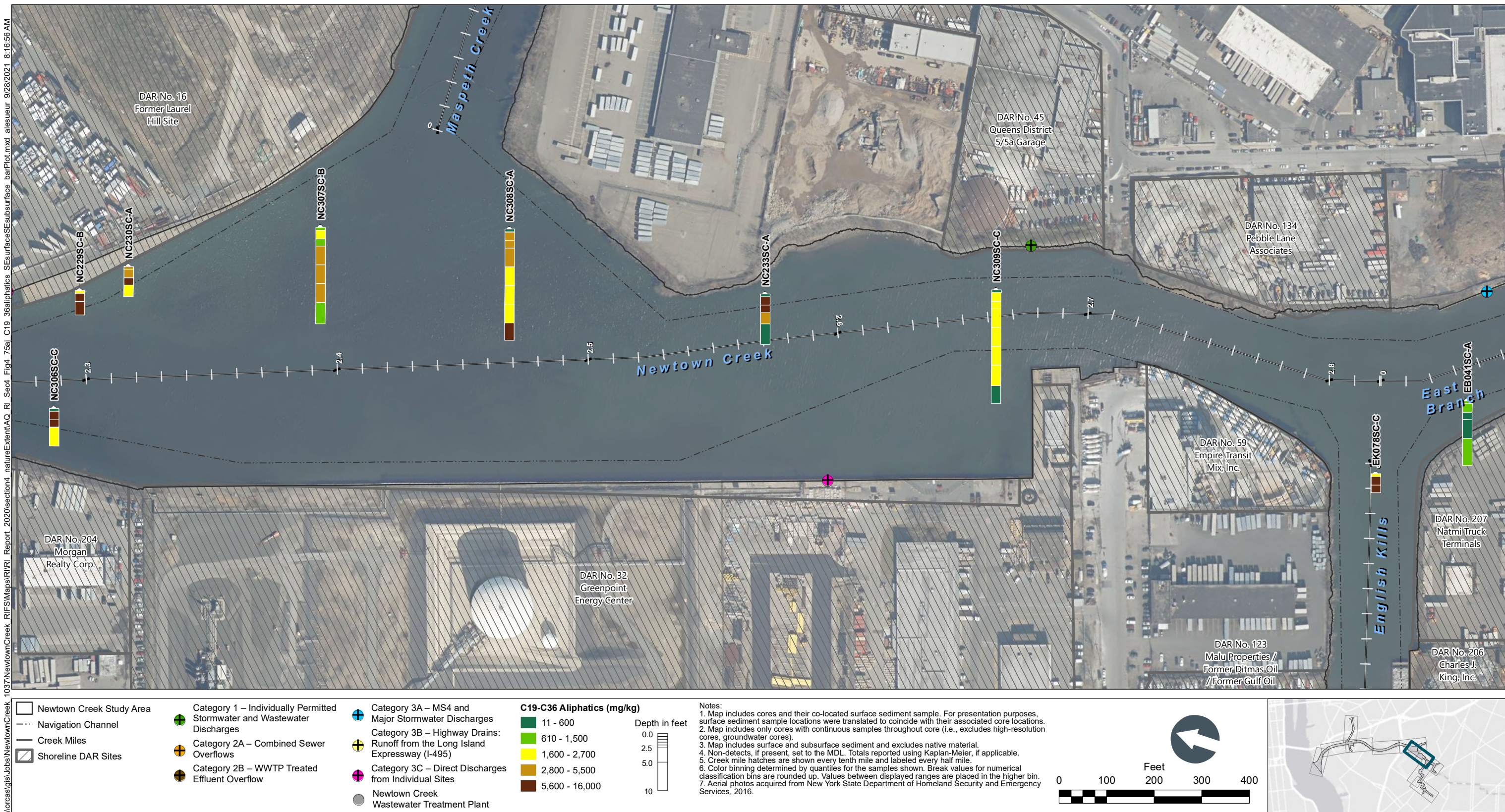
Figure 4-75g C19-C36 Aliphatics in Surface and Subsurface Sediment Bar Plots by Depth – Plan View of Newtown Creek CM 2.3 to 2.8 Remedial Investigation Report Newtown Creek RI/FS
