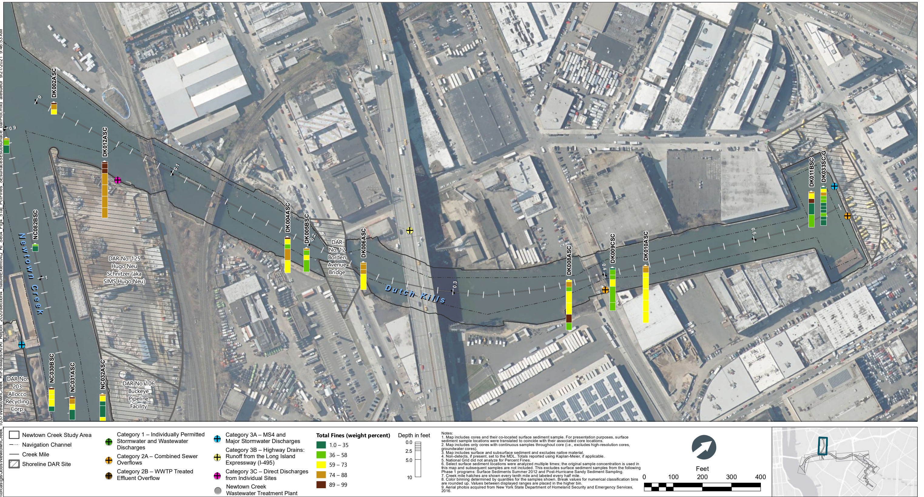
Figure 4-51d Total Percent Fines in Surface and Subsurface Sediment Bar Plots by Depth – Plan View of Dutch Kills CM 0 to 0.5 Remedial Investigation Report Newtown Creek RI/FS
