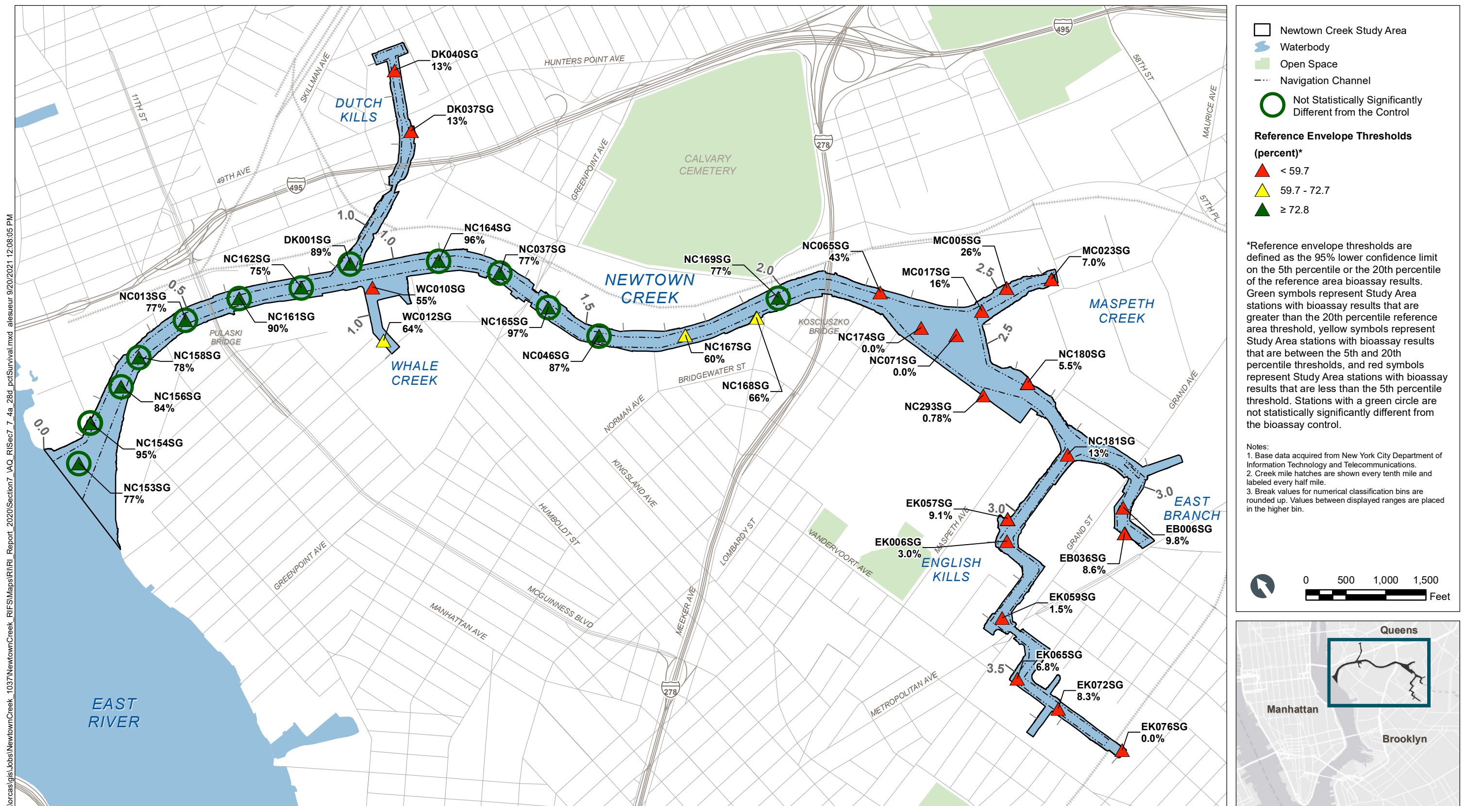
Figure 7-4a 28-Day Survival Reference Envelope (n = 48) Comparison by Study Area Creek Mile Remedial Investigation Report Newtown Creek RI/FS
