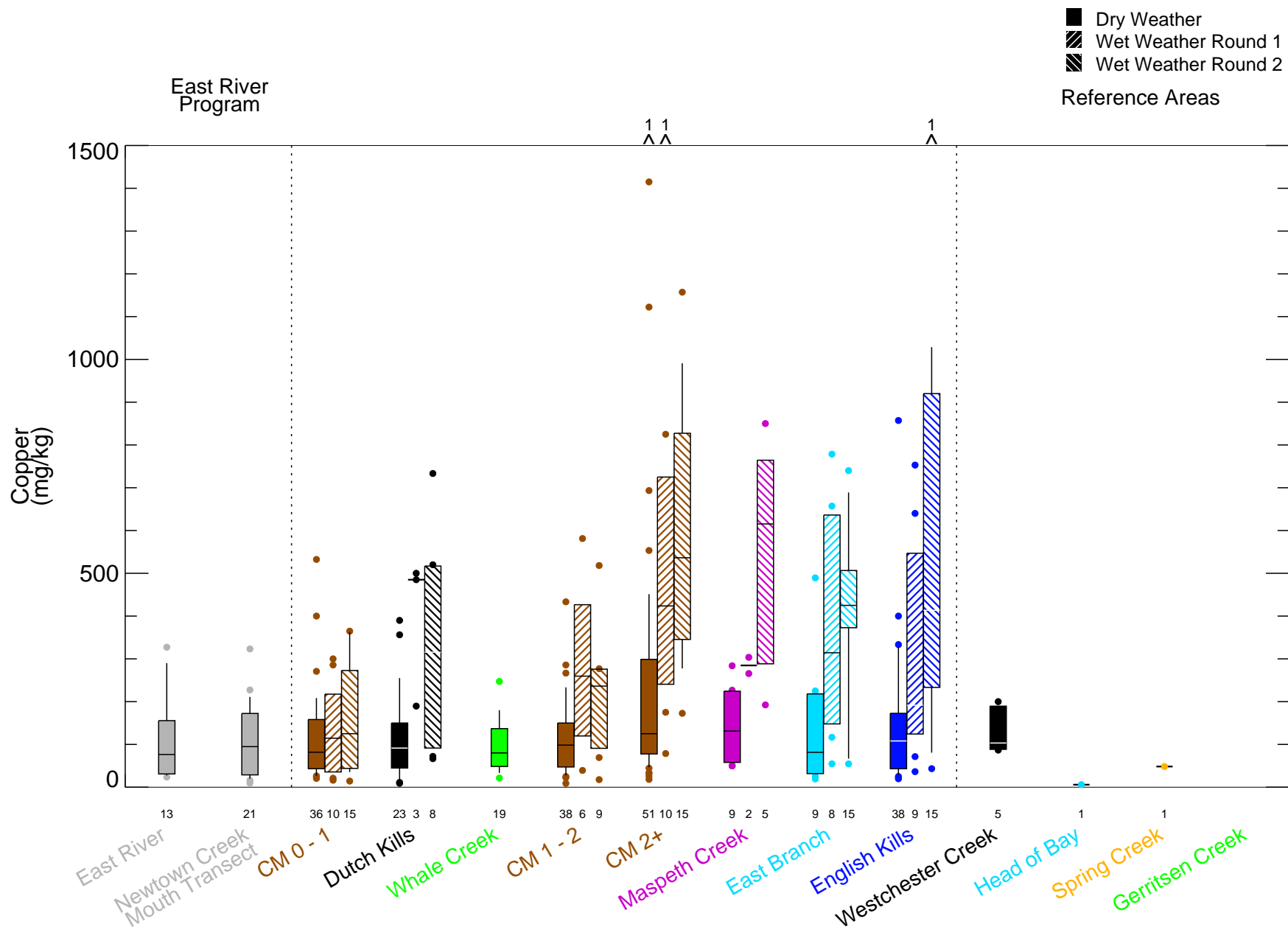
Figure 4-192 Calculated Particulate Phase Copper in Surface Water During Dry and Wet Weather Sampling Events - Box Plots Remedial Investigation Report Newtown Creek RI/FS
