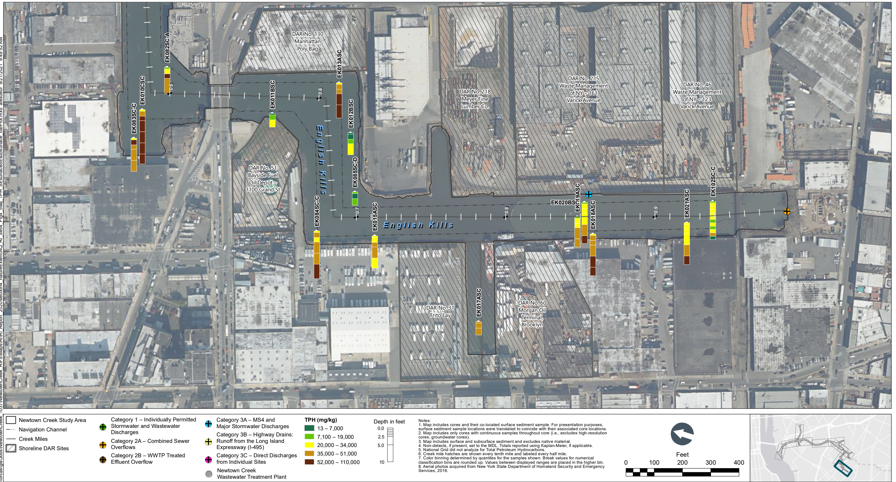
Figure 4-59j TPH in Surface and Subsurface Sediment Bar Plots by Depth – Plan View of English Kills CM 0.5 to 0.9 Remedial Investigation Report Newtown Creek RI/FS
