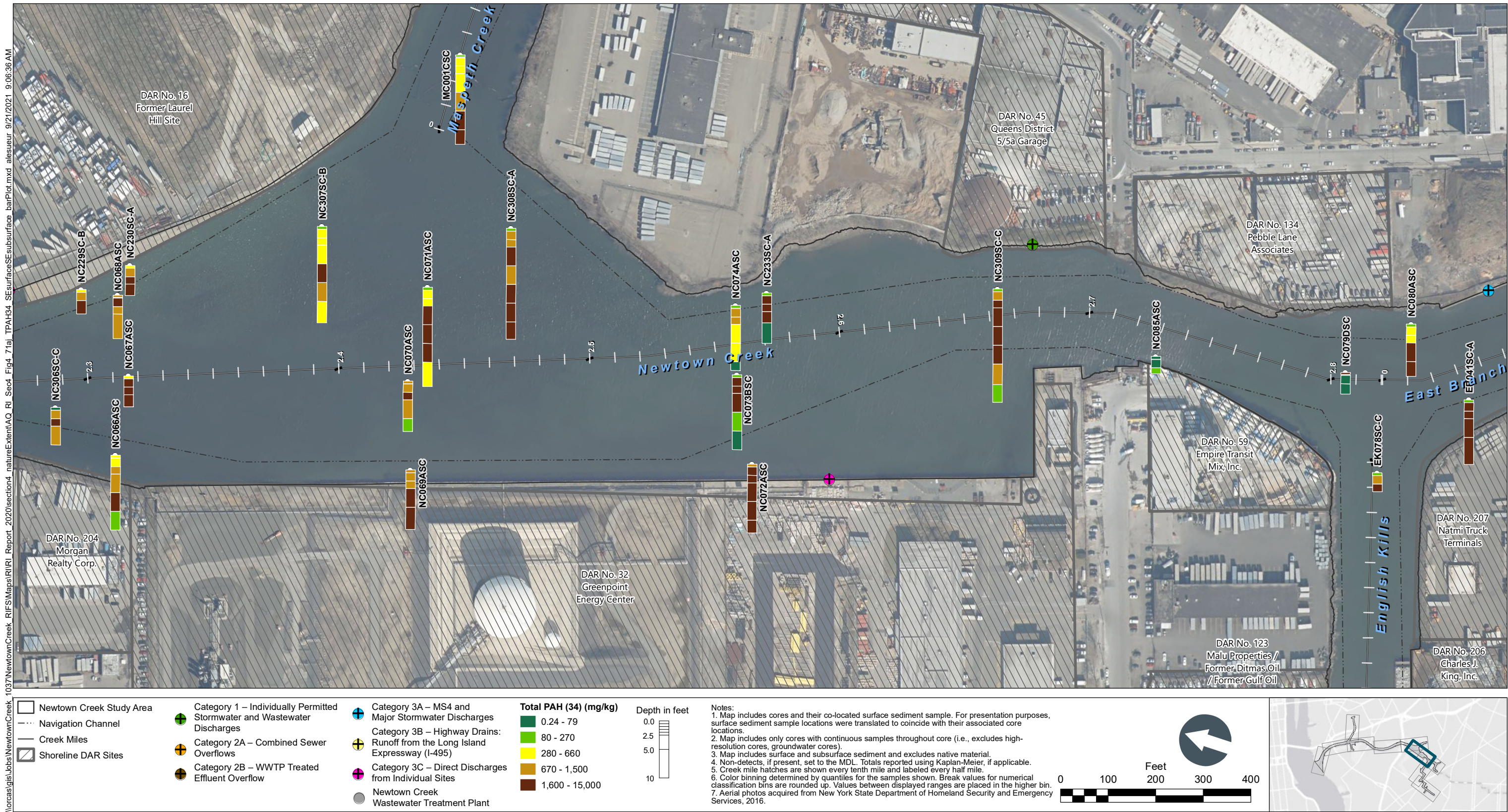
Figure 4-71g Total PAH (34) in Surface and Subsurface Sediment Bar Plots by Depth – Plan View of Newtown Creek CM 2.3 to 2.8 Remedial Investigation Report Newtown Creek RI/FS
