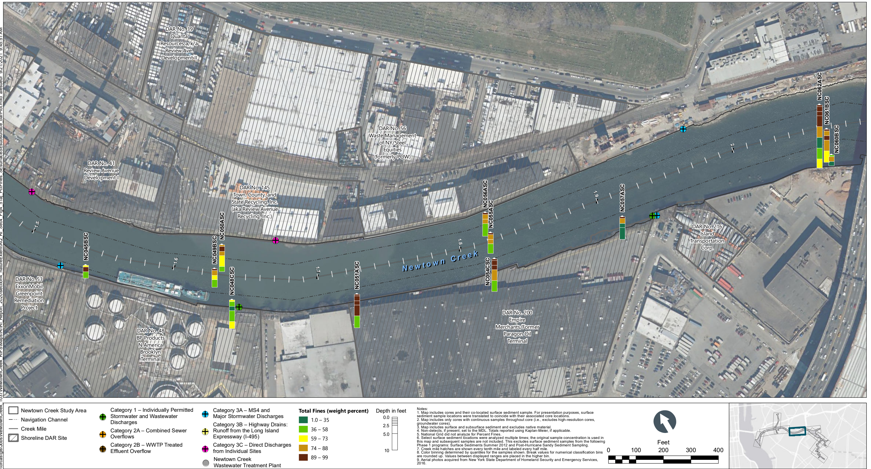
Figure 4-51e Total Percent Fines in Surface and Subsurface Sediment Bar Plots by Depth – Plan View of Newtown Creek CM 1.5 to 2.0 Remedial Investigation Report Newtown Creek RI/FS
