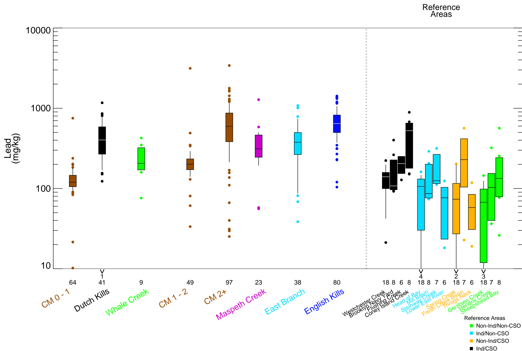
Figure 4-35 Lead in Surface Sediment - Box Plots by Location Remedial Investigation Report Newtown Creek RI/FS
