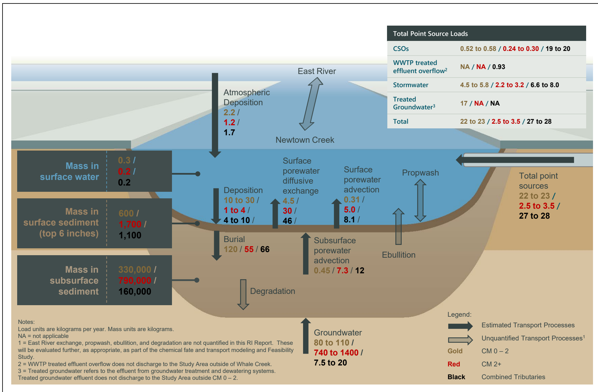
Figure 8-15 Estimated Total PAH (17) Mass and Loads Remedial Investigation Report Newtown Creek RI/FS
