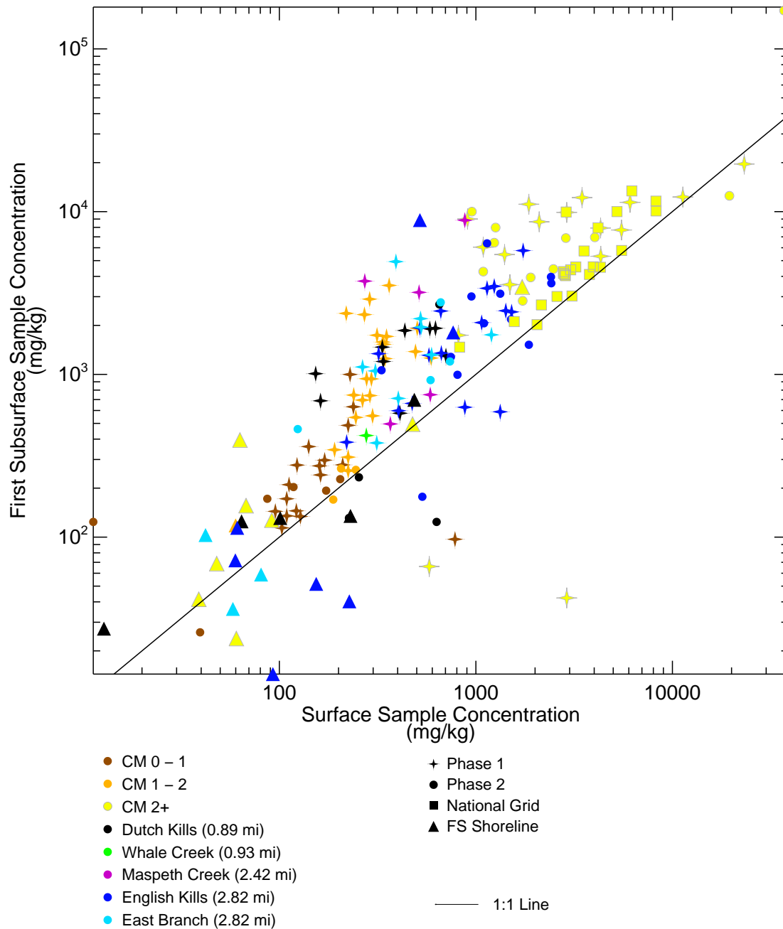
Figure 4-98 Copper in Surface Sediment versus Copper in First Subsurface Interval – Cross Plot Remedial Investigation Report Newtown Creek RI/FS
