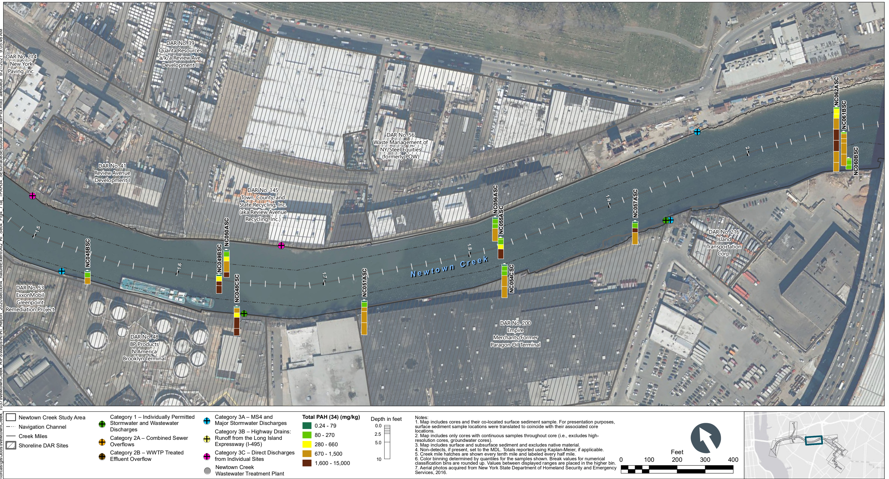
Figure 4-71e Total PAH (34) in Surface and Subsurface Sediment Bar Plots by Depth – Plan View of Newtown Creek CM 1.5 to 2.0 Remedial Investigation Report Newtown Creek RI/FS
