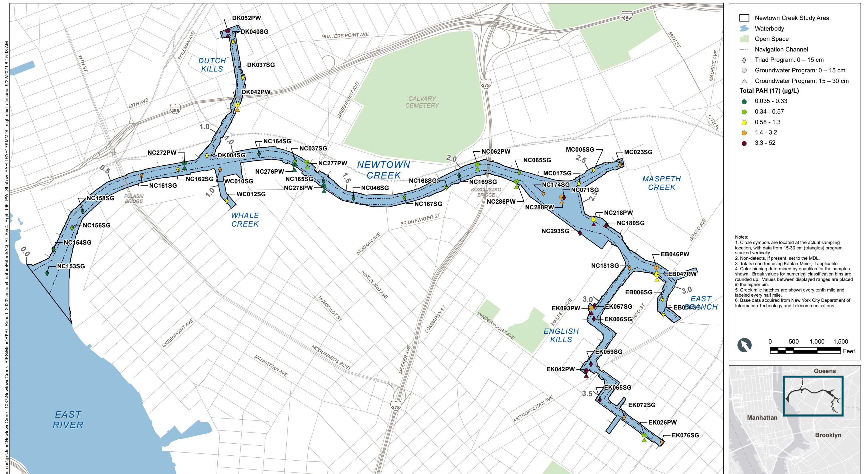
Figure 4-196 Total PAH (17) in Shallow Porewater – Plan View Remedial Investigation Report Newtown Creek RI/FS
