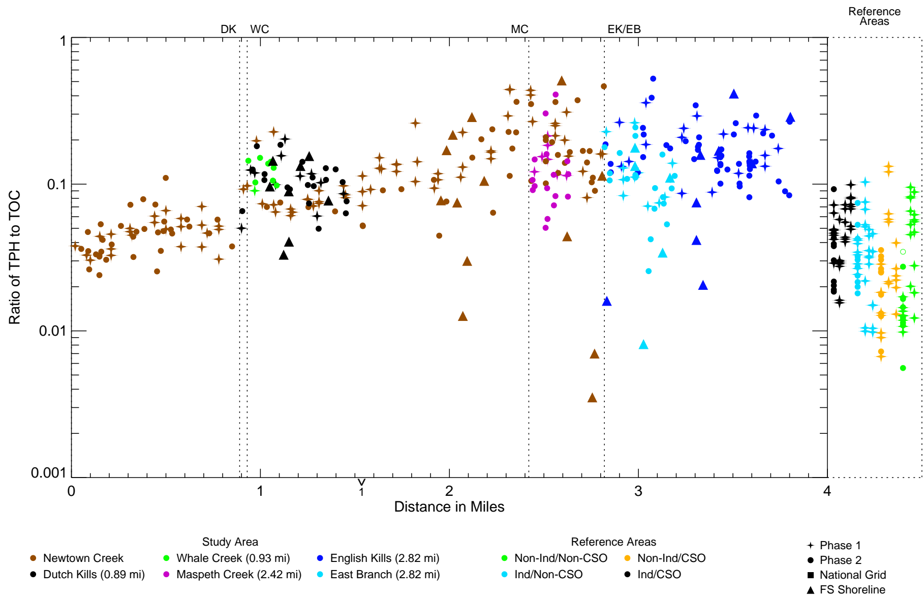
Figure 4-12 Ratio of TPH to TOC in Surface Sediment - Longitudinal Profile Remedial Investigation Report Newtown Creek RI/FS
