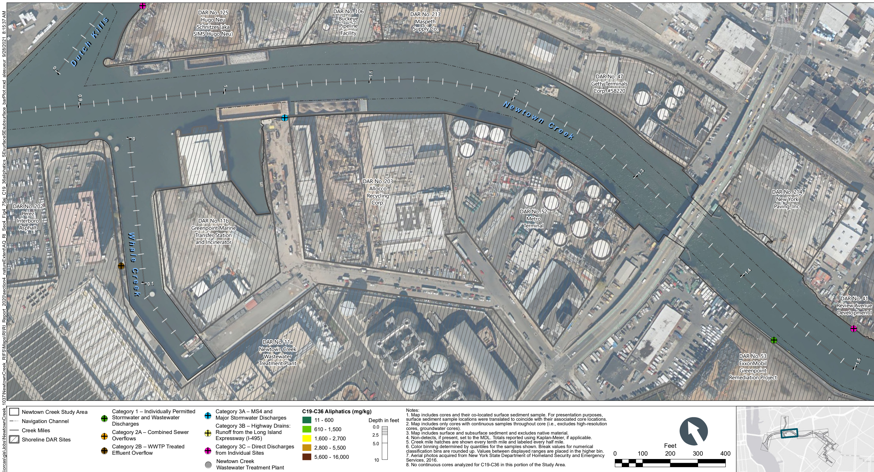
Figure 4-75c C19-C36 Aliphatics in Surface and Subsurface Sediment Bar Plots by Depth – Plan View of Whale Creek and Newtown Creek CM 0.9 to 1.5 Remedial Investigation Report Newtown Creek RI/FS
