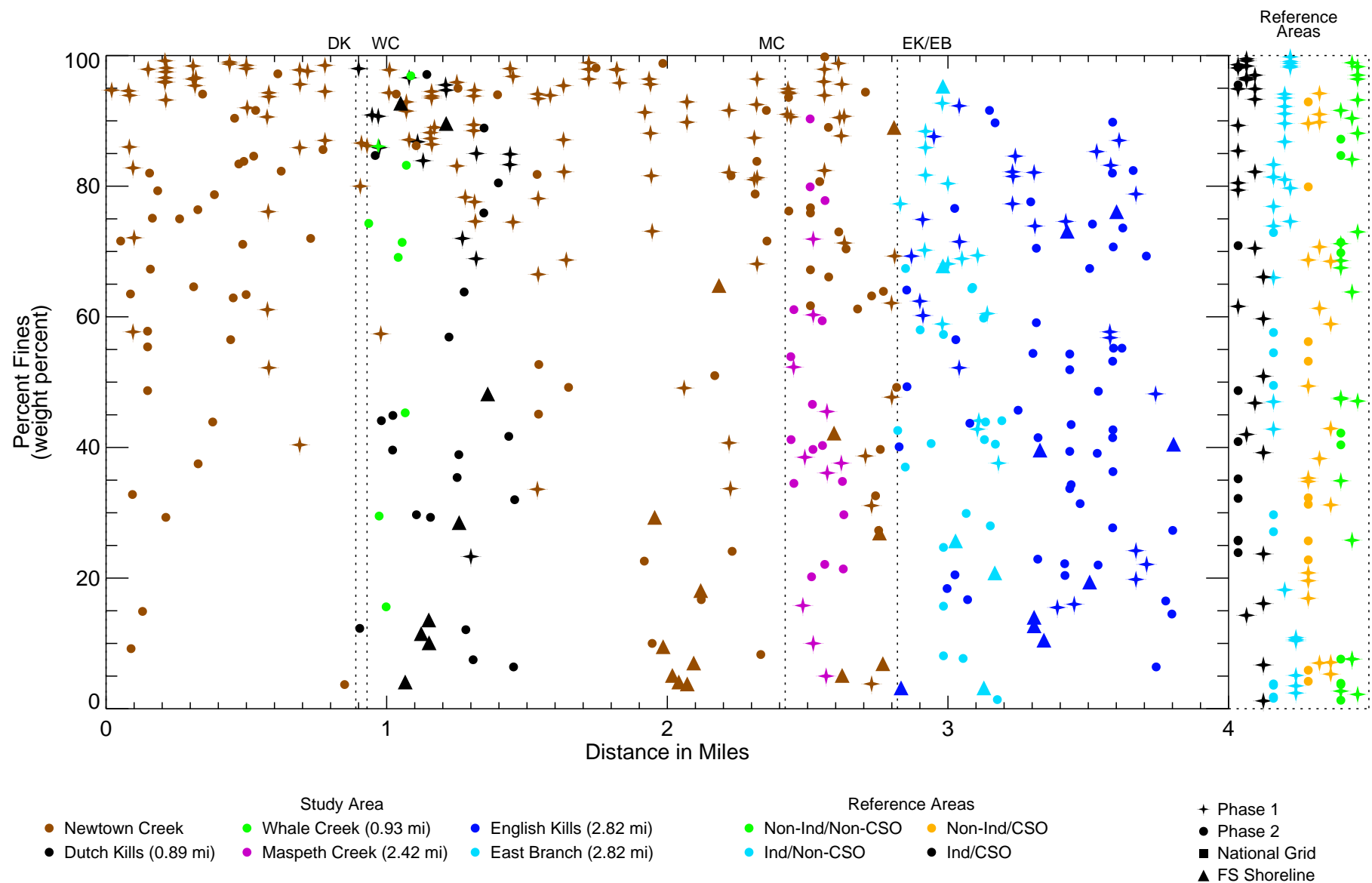
Figure 4-5 Percent Fines in Surface Sediment - Longitudinal Profile Remedial Investigation Report Newtown Creek RI/FS
