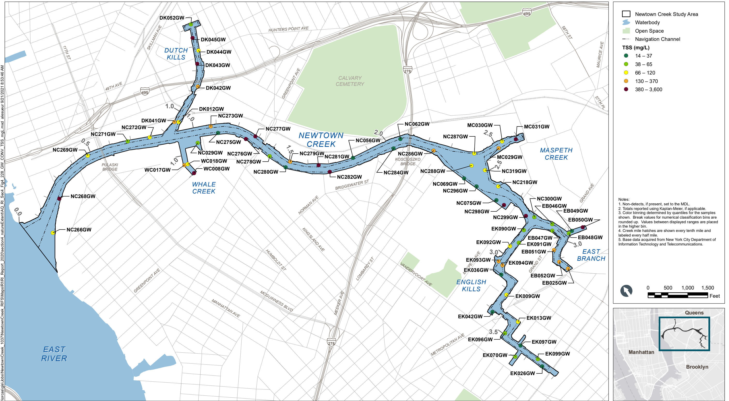
Figure 4-228 TSS in Groundwater – Plan View Remedial Investigation Report Newtown Creek RI/FS
