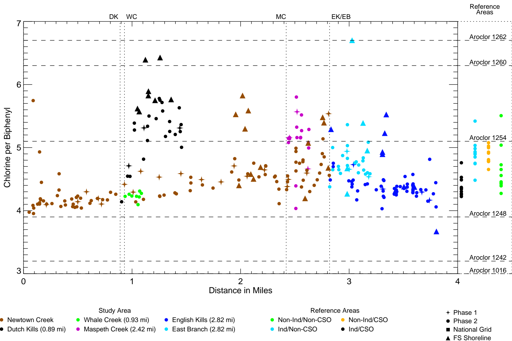
Figure 4-47 Chlorine per Biphenyl in Surface Sediment - Longitudinal Profile Remedial Investigation Report Newtown Creek RI/FS
