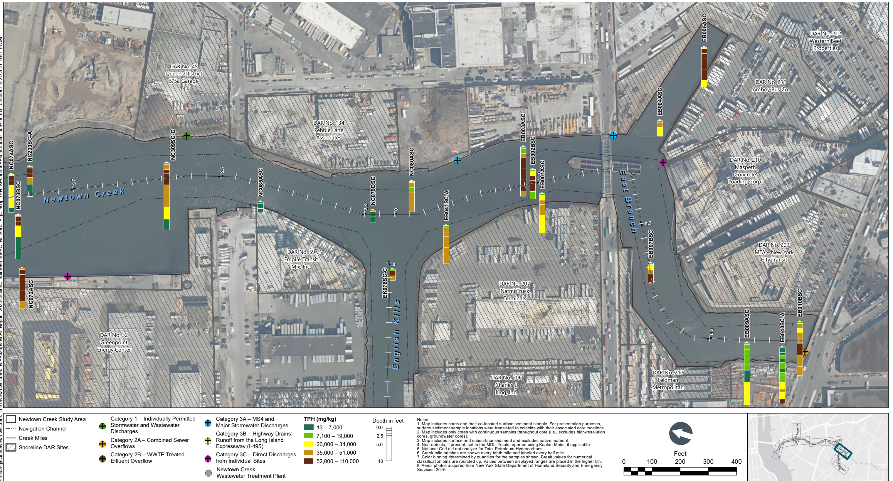
Figure 4-59h TPH in Surface and Subsurface Sediment Bar Plots by Depth – Plan View of East Branch and Newtown Creek CM 2.6 to 2.8 Remedial Investigation Report Newtown Creek RI/FS
