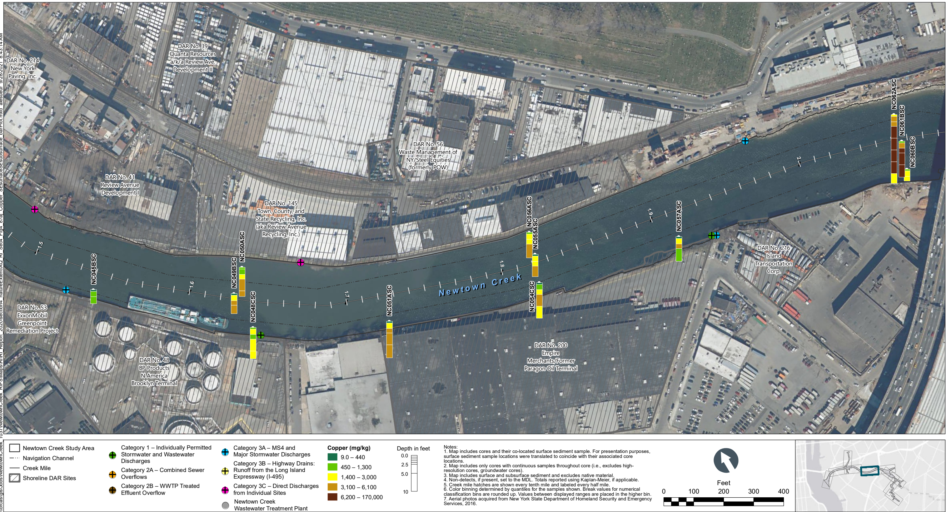
Figure 4-87e Copper in Surface and Subsurface Sediment Bar Plots by Depth – Plan View of Newtown Creek CM 1.5 to 2.0 Remedial Investigation Report Newtown Creek RI/FS
