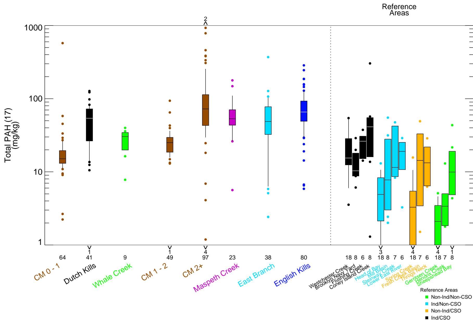
Figure 8-9 Total PAH (17) in Surface Sediment - Box Plots by Location Remedial Investigation Report Newtown Creek RI/FS
