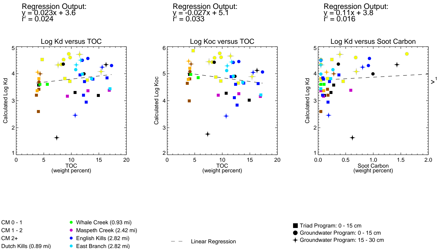
Figure 6-17b Calculated Partition Coefficient versus TOC and Soot Carbon for Naphthalene - Cross Plots Remedial Investigation Report Newtown Creek RI/FS
