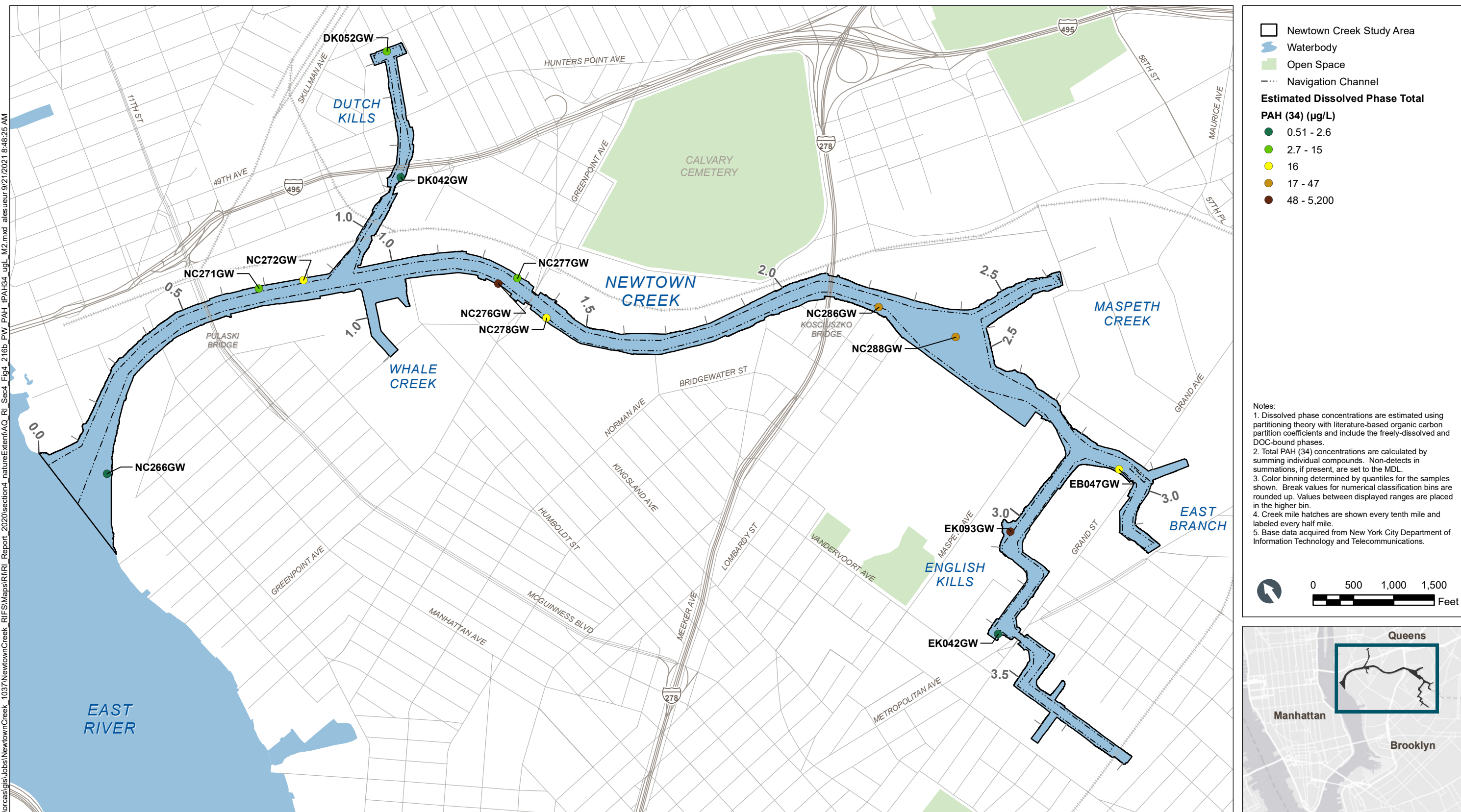
Figure 4-216b Estimated Dissolved Phase (Method 2) Total PAH (34) in Mid-Depth Porewater – Plan View Remedial Investigation Report Newtown Creek RI/FS
