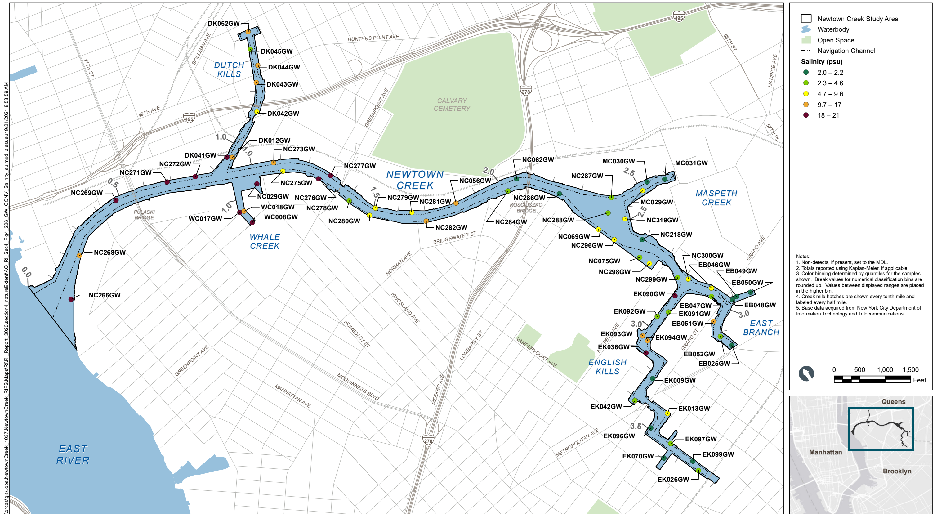
Figure 4-226 Salinity in Groundwater – Plan View Remedial Investigation Report Newtown Creek RI/FS
