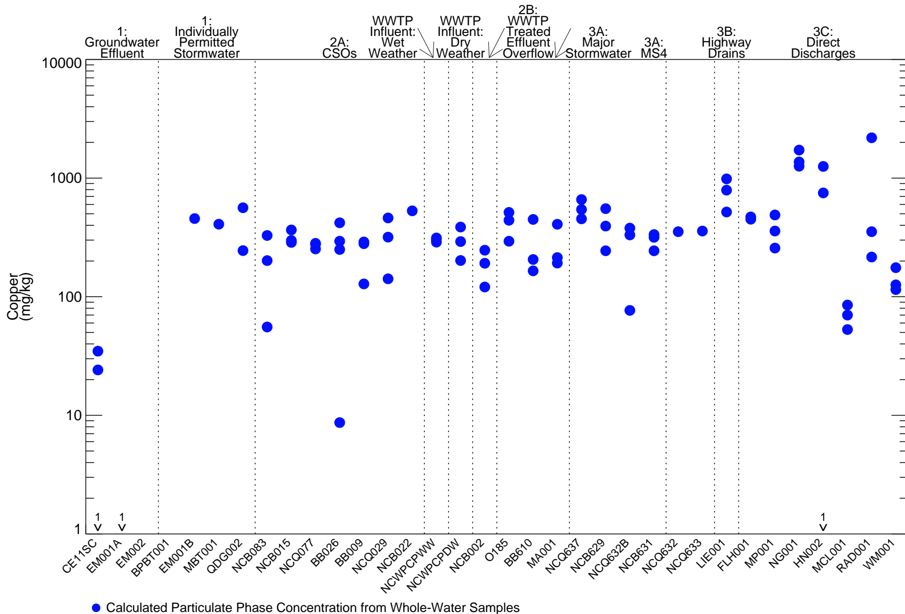
Figure 5-11 Particulate Phase Copper Concentrations in Point Sources Remedial Investigation Report Newtown Creek RI/FS
