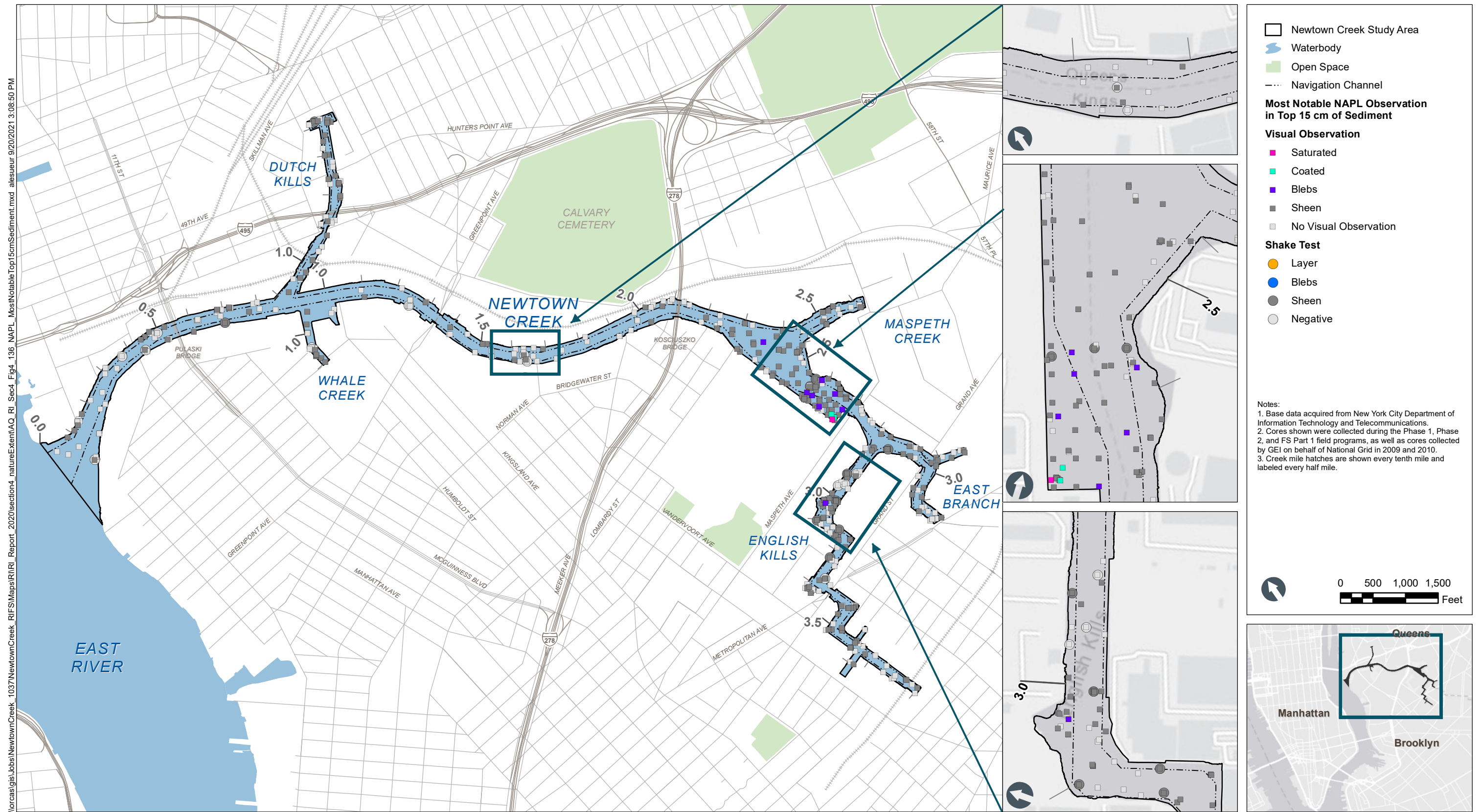
Figure 4-136 Most Notable NAPL Observations in Surface Sediment – Plan View Remedial Investigation Report Newtown Creek RI/FS
