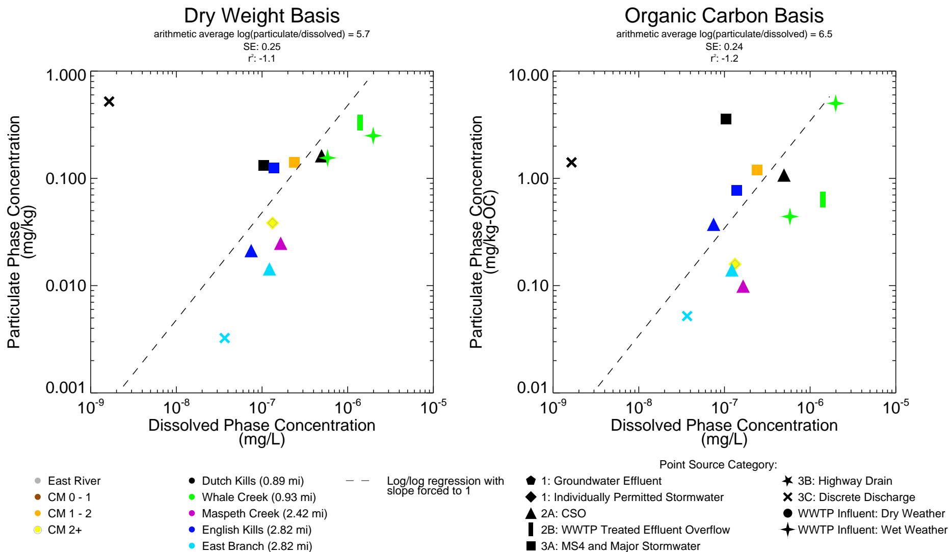
Figure 6-12g Point Source Particulate Phase versus Dissolved Phase for Total Heptachlorobiphenyl Homologs - Cross Plots Remedial Investigation Report Newtown Creek RI/FS
