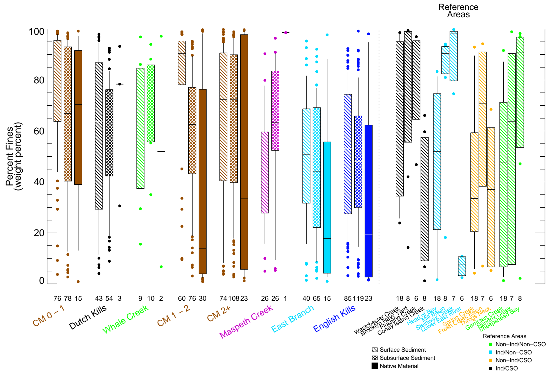
Figure 4-50 Percent Fines in Surface Sediment, Subsurface Sediment, and Native Material – Box Plots by Location Remedial Investigation Report Newtown Creek RI/FS
