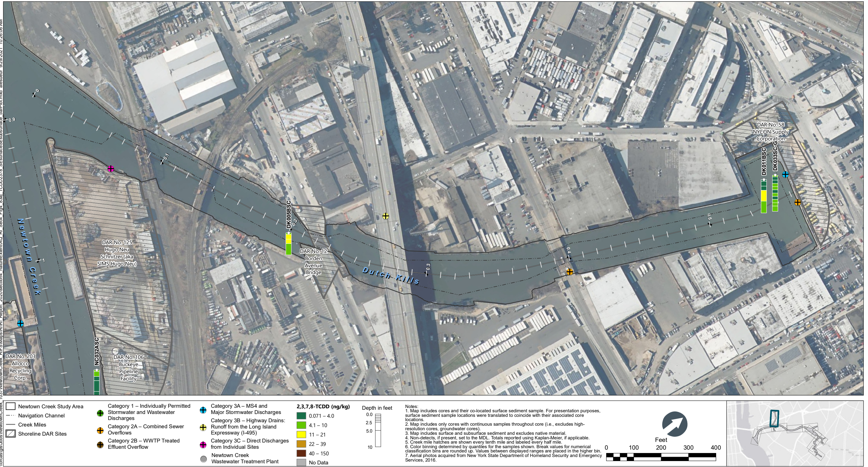
Figure 4-83d 2,3,7,8-TCDD in Surface and Subsurface Sediment Bar Plots by Depth – Plan View of Dutch Kills CM 0 to 0.5 Remedial Investigation Report Newtown Creek RI/FS
