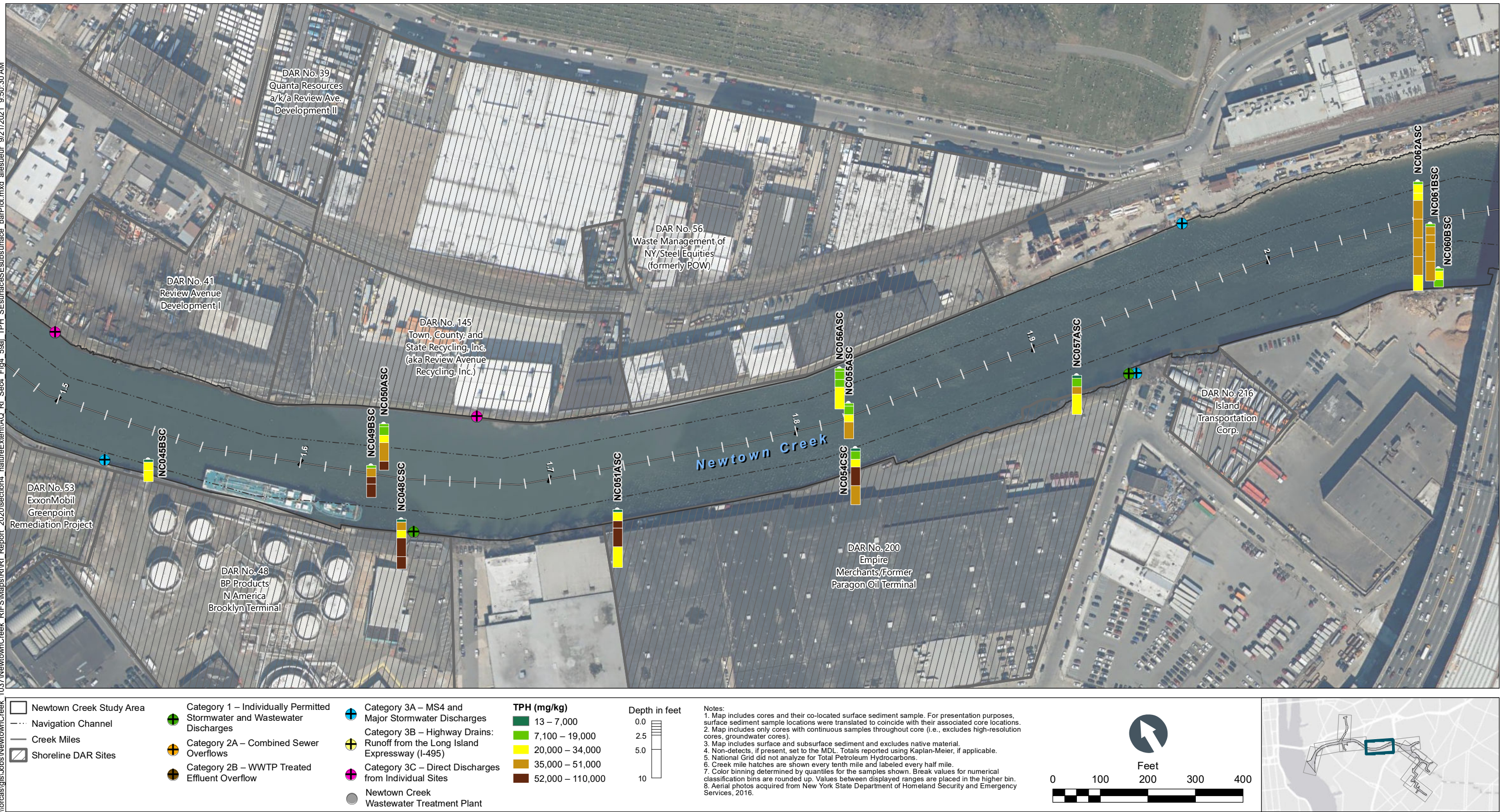
Figure 4-59e TPH in Surface and Subsurface Sediment Bar Plots by Depth – Plan View of Newtown Creek CM 1.5 to 2.0 Remedial Investigation Report Newtown Creek RI/FS
