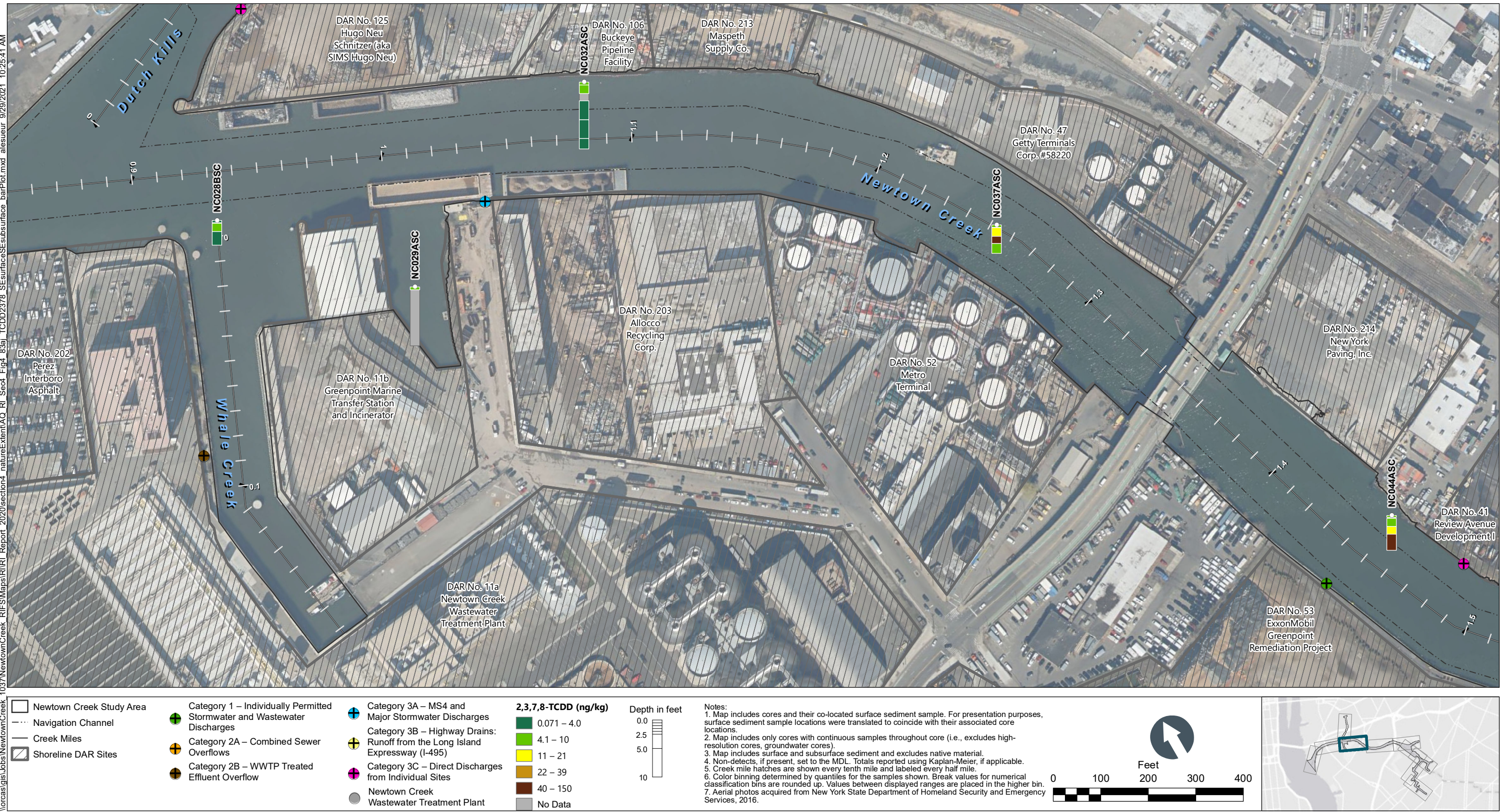
Figure 4-83c 2,3,7,8-TCDD in Surface and Subsurface Sediment Bar Plots by Depth – Plan View of Whale Creek and Newtown Creek CM 0.9 to 1.5 Remedial Investigation Report Newtown Creek RI/FS
