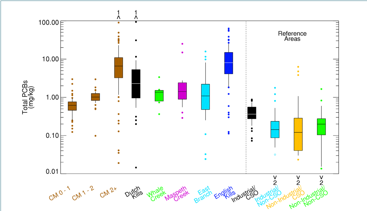
Graphic ES-5. TPCB in Surface Sediment
