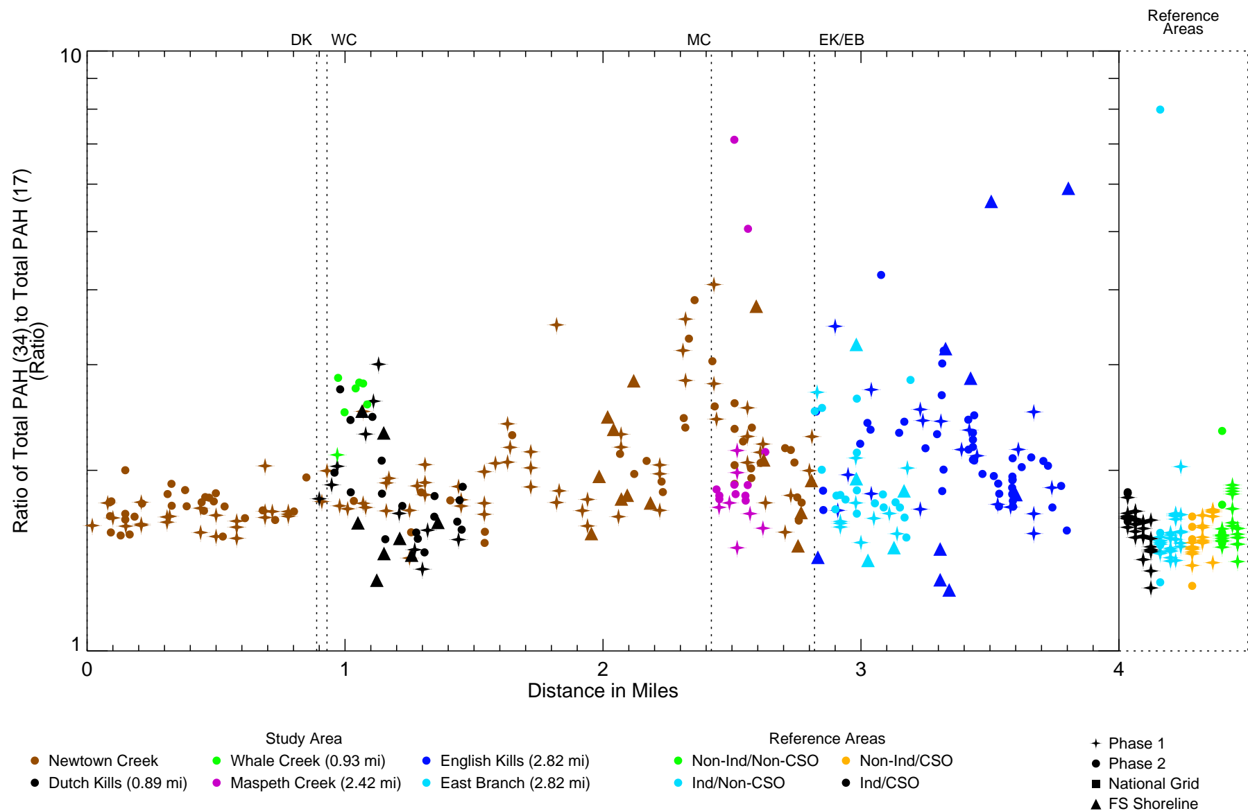
Figure 4-43 Ratio of Total PAH (34) to Total PAH (17) in Surface Sediment - Longitudinal Profile Remedial Investigation Report Newtown Creek RI/FS
