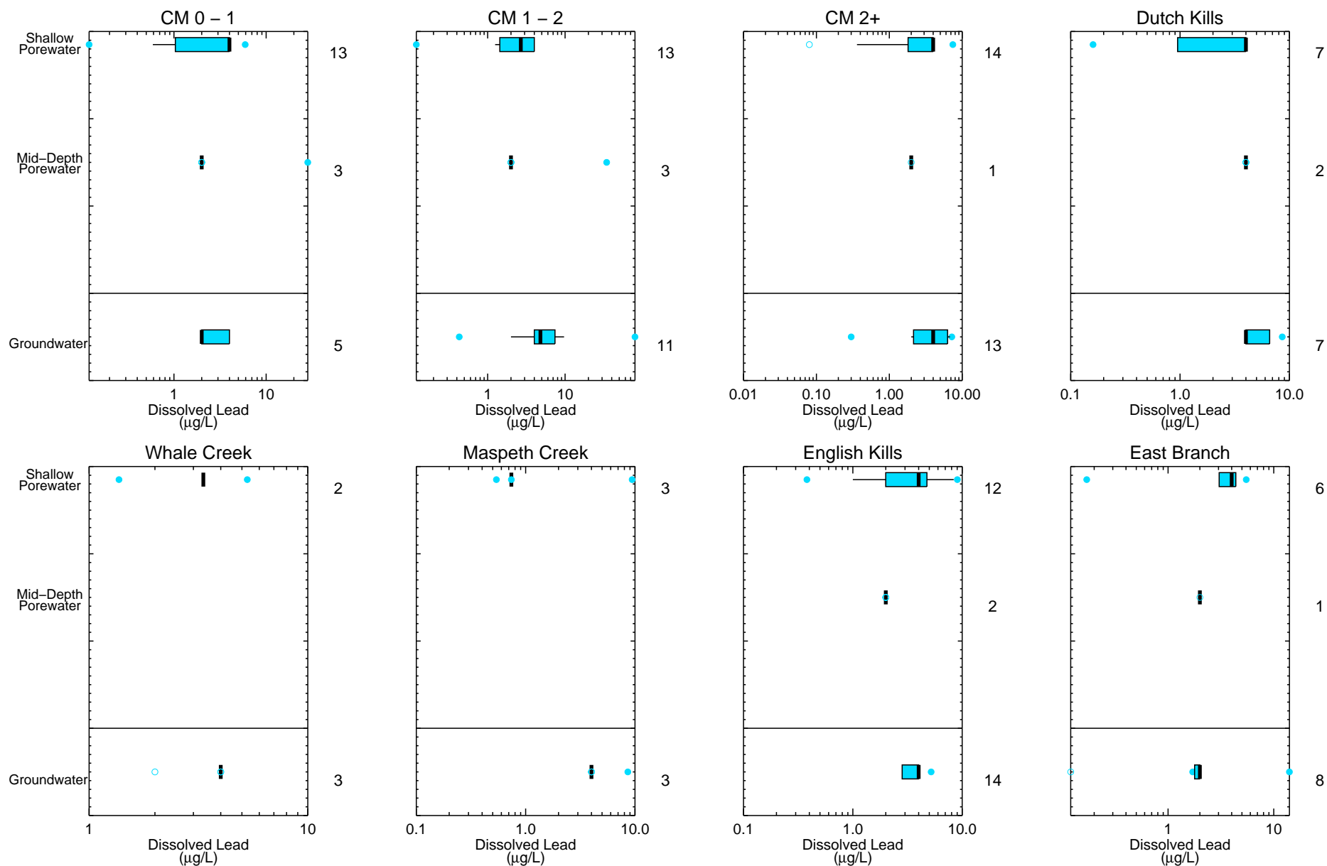
Figure 4-262 Dissolved Lead in Porewater and Groundwater – Box Plot Depth Profiles Remedial Investigation Report Newtown Creek RI/FS
