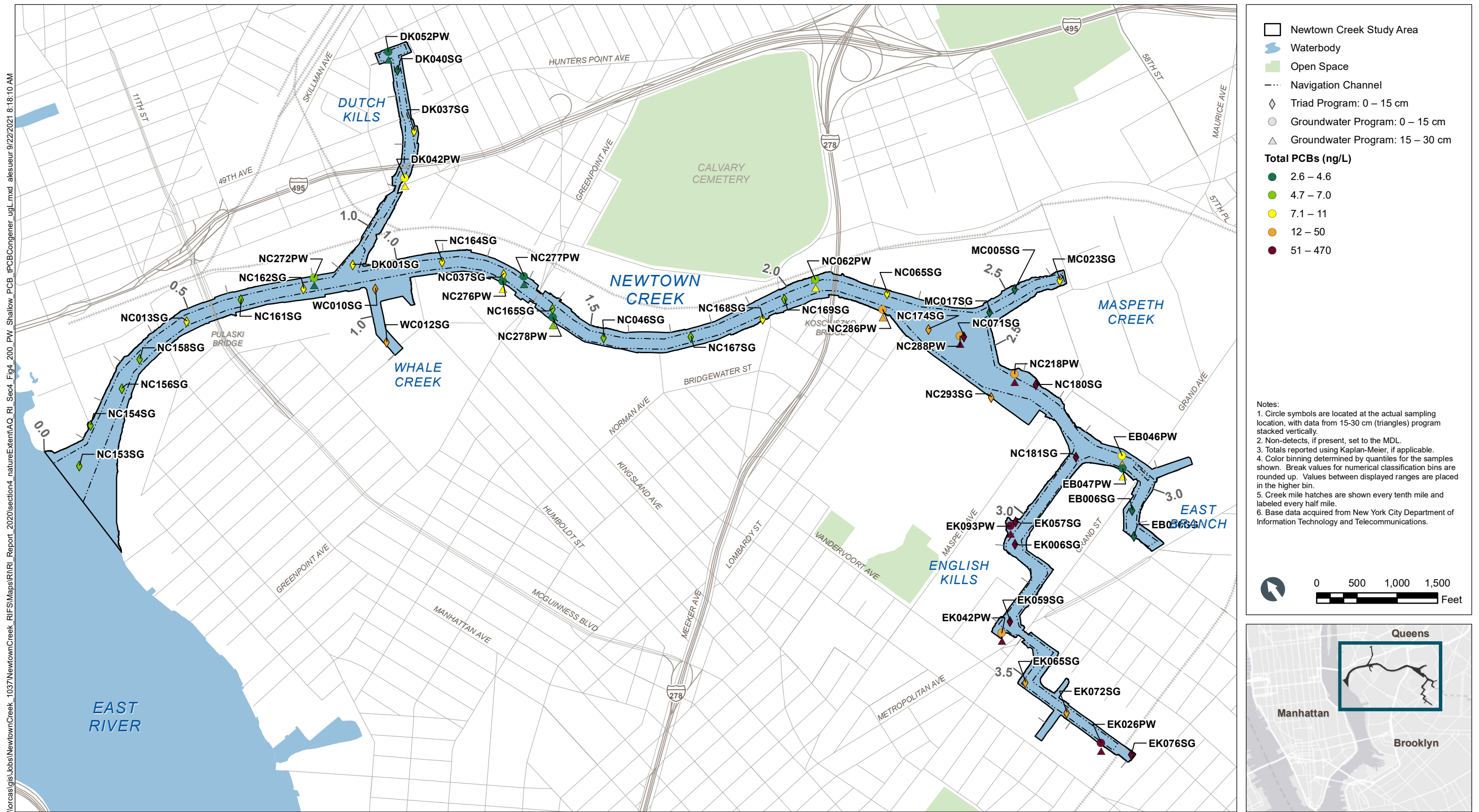
Figure 4-200 Total PCBs in Shallow Porewater – Plan View Remedial Investigation Report Newtown Creek RI/FS
