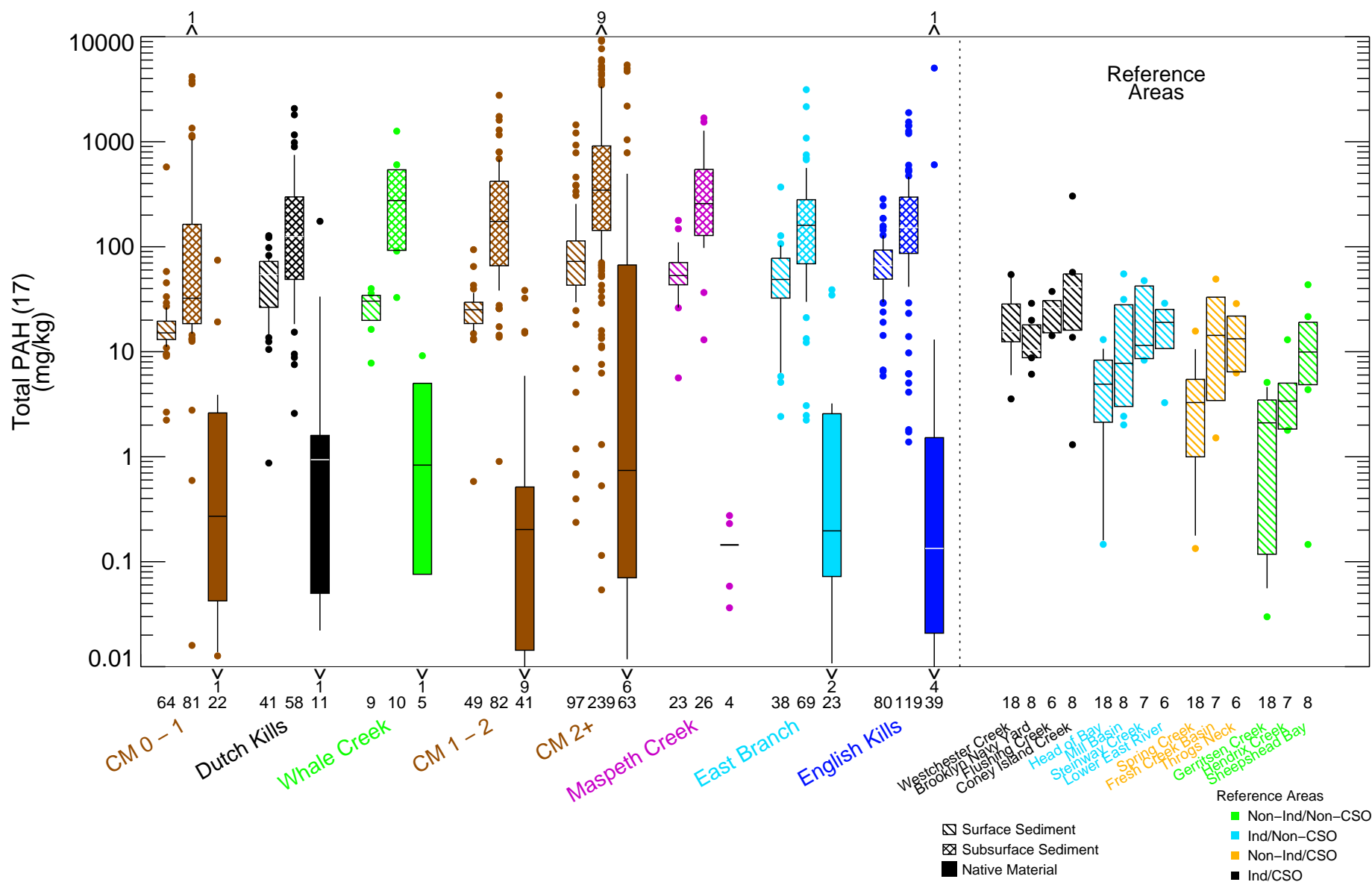
Figure 4-64 Total PAH (17) in Surface Sediment, Subsurface Sediment, and Native Material – Box Plots by Location Remedial Investigation Report Newtown Creek RI/FS
