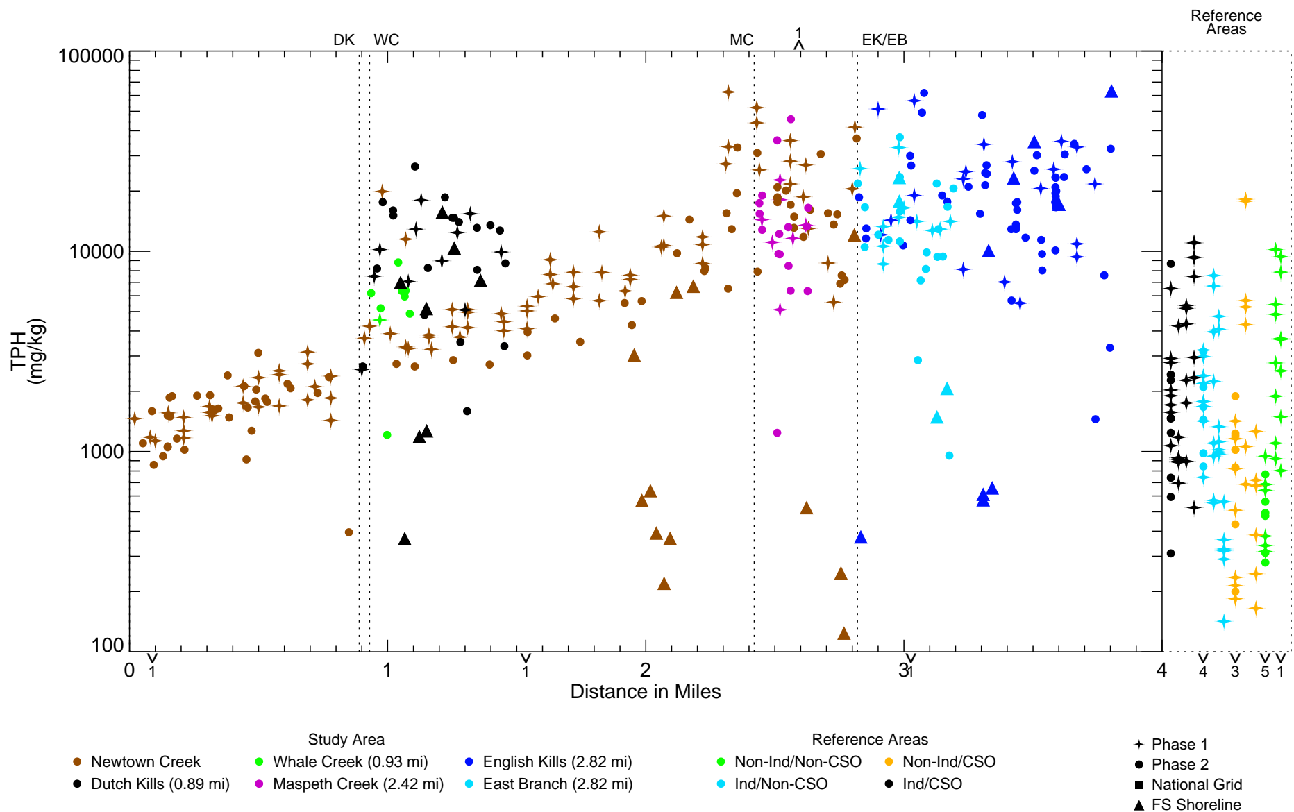
Figure 4-11 TPH in Surface Sediment - Longitudinal Profile Remedial Investigation Report Newtown Creek RI/FS
