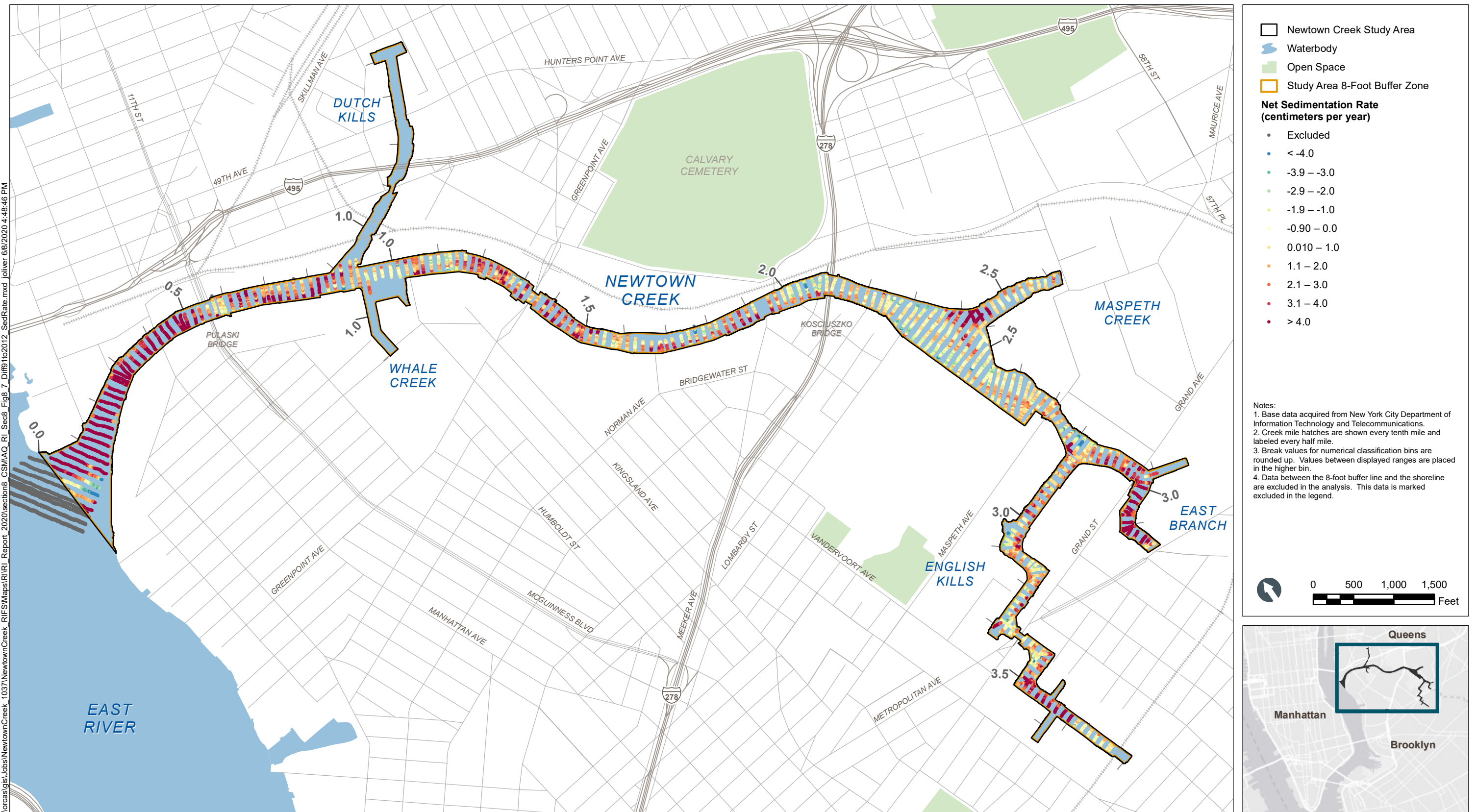
Figure 8-7 1991 to 2012 Differential Bathymetry Analysis Results: Spatial Variation in Net Sedimentation Rates Remedial Investigation Report Newtown Creek RI/FS
