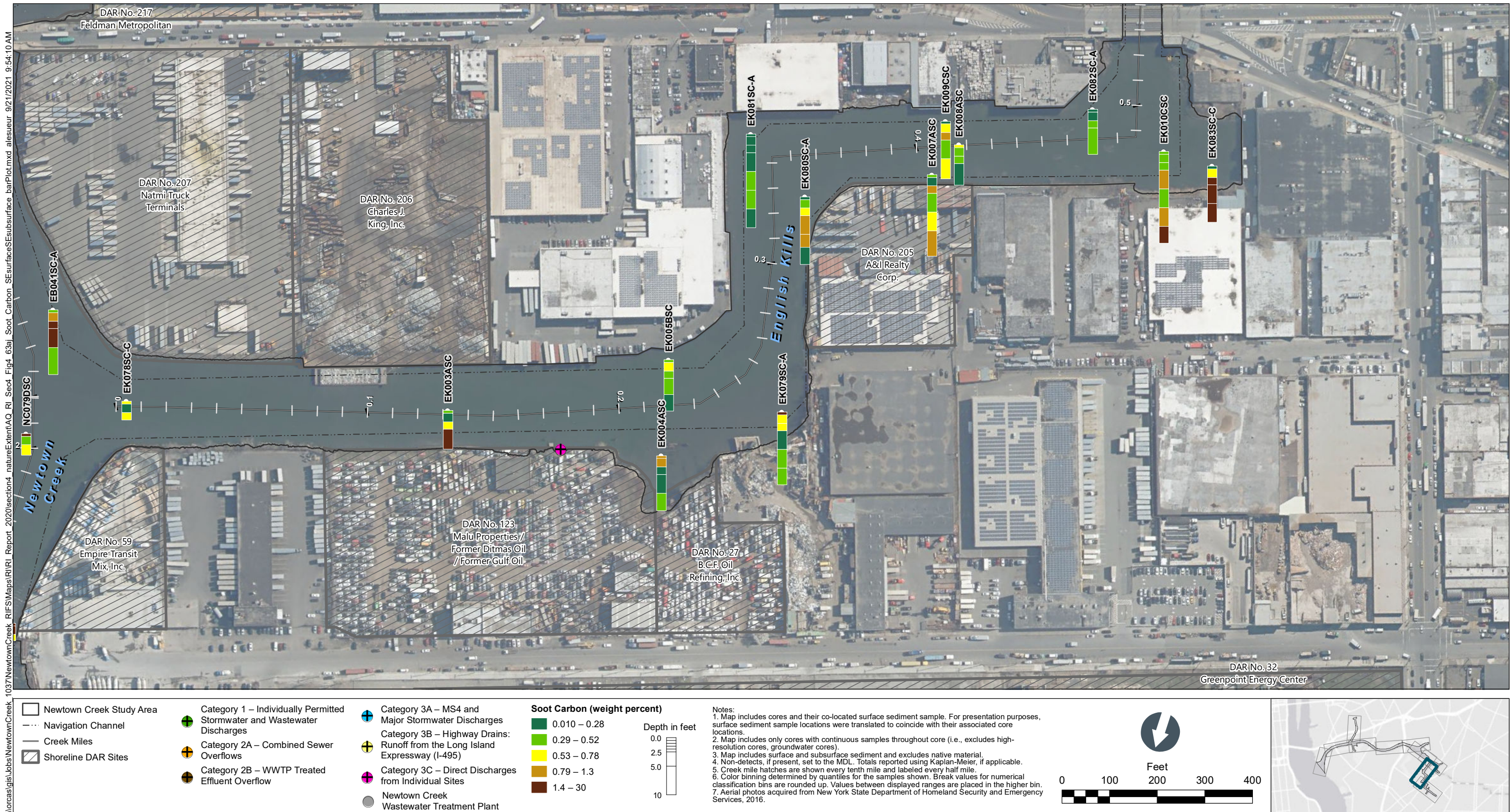
Figure 4-63i Percent Soot Carbon in Surface and Subsurface Sediment Bar Plots by Depth – Plan View of English Kills CM 0 to 0.5 Remedial Investigation Report Newtown Creek RI/FS
