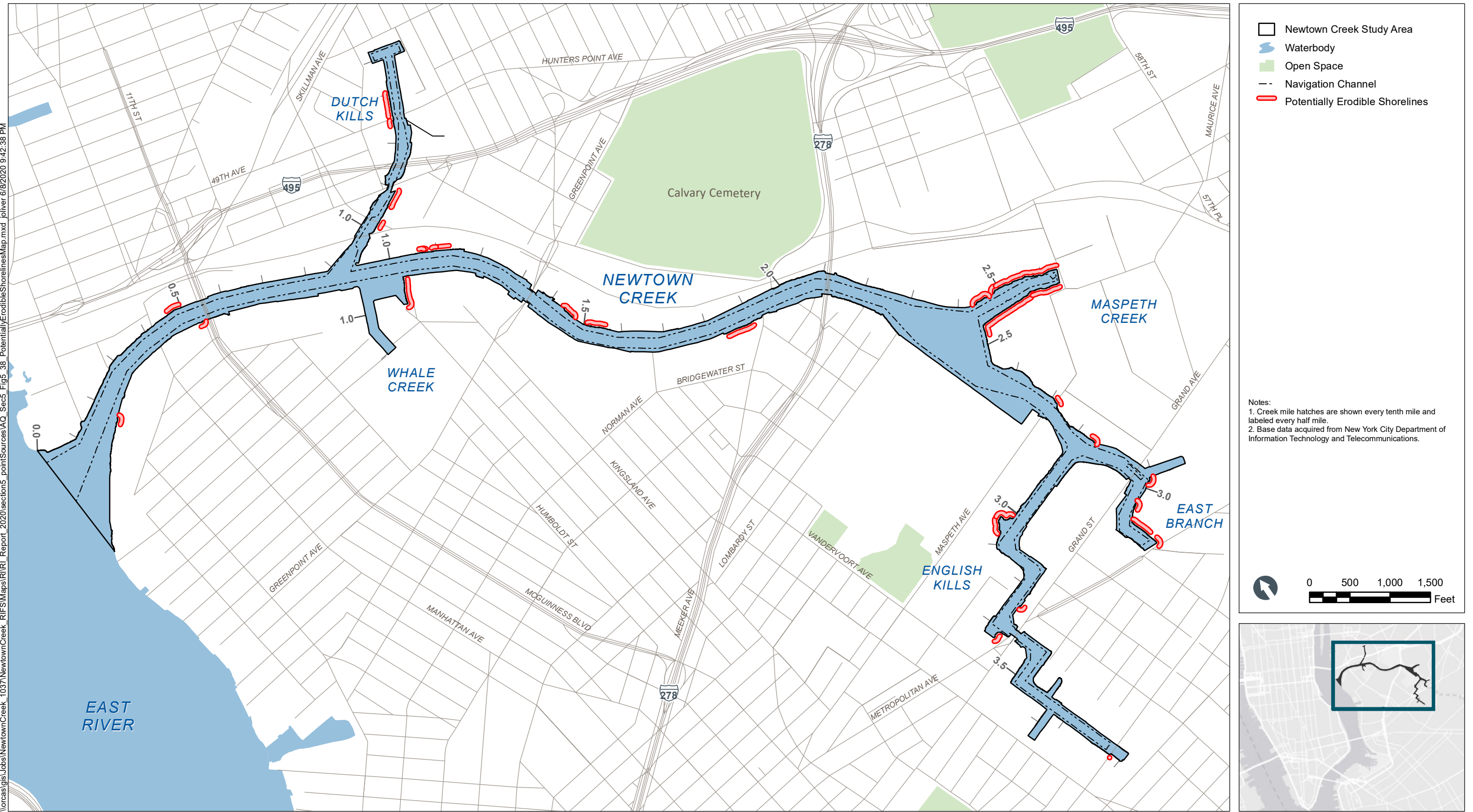
Figure 5-38 Potentially Erodible Shorelines Within the Study Area Remedial Investigation Report Newtown Creek RI/FS
