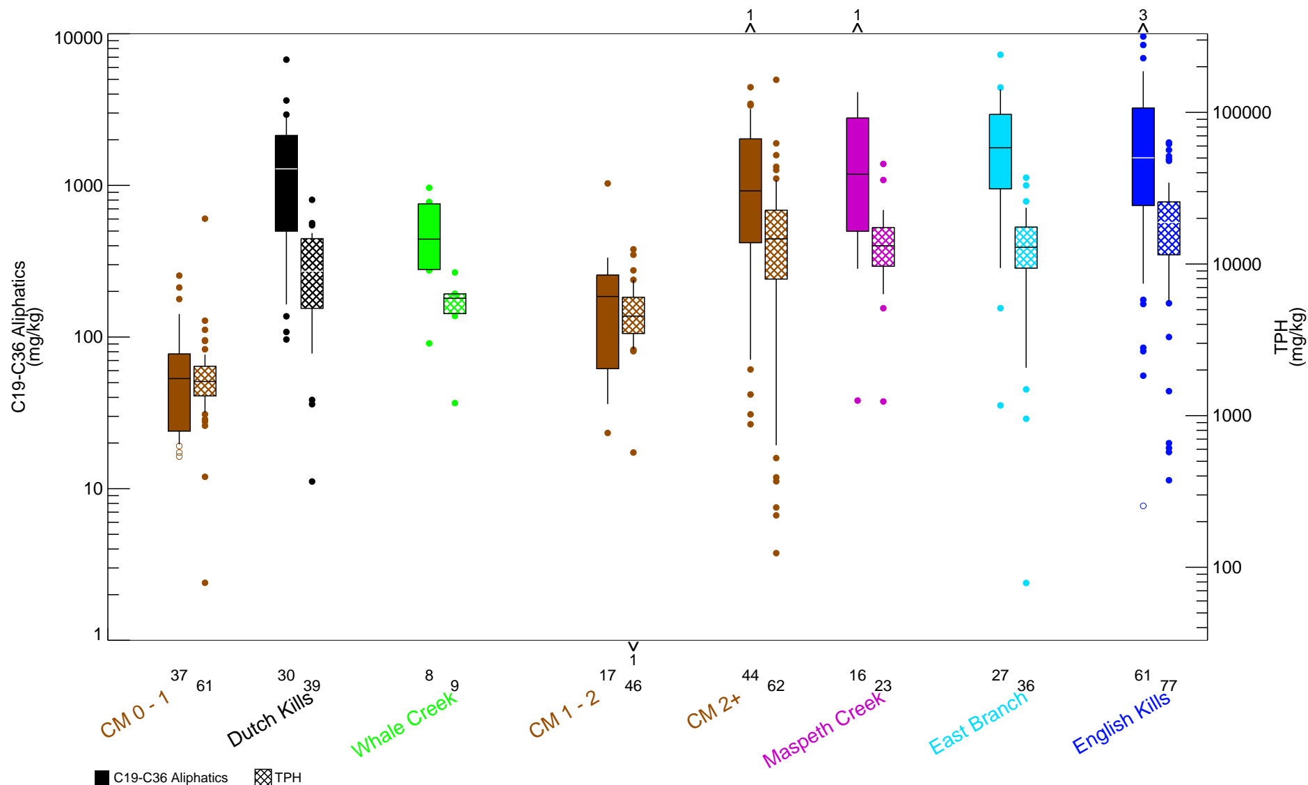
Figure 4-327 Comparison of C19-C36 Aliphatics and TPH in Surface Sediment - Box Plots by Location Remedial Investigation Report Newtown Creek RI/FS
