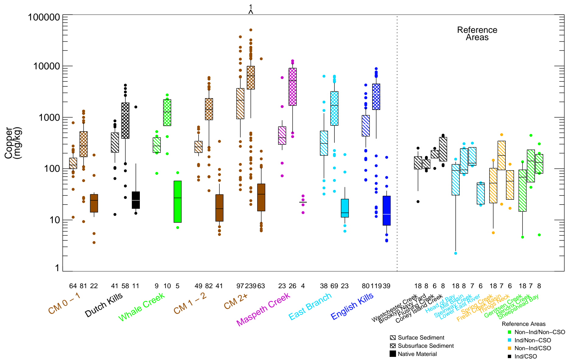
Figure 4-84 Copper in Surface Sediment, Subsurface Sediment, and Native Material – Box Plots by Location Remedial Investigation Report Newtown Creek RI/FS
