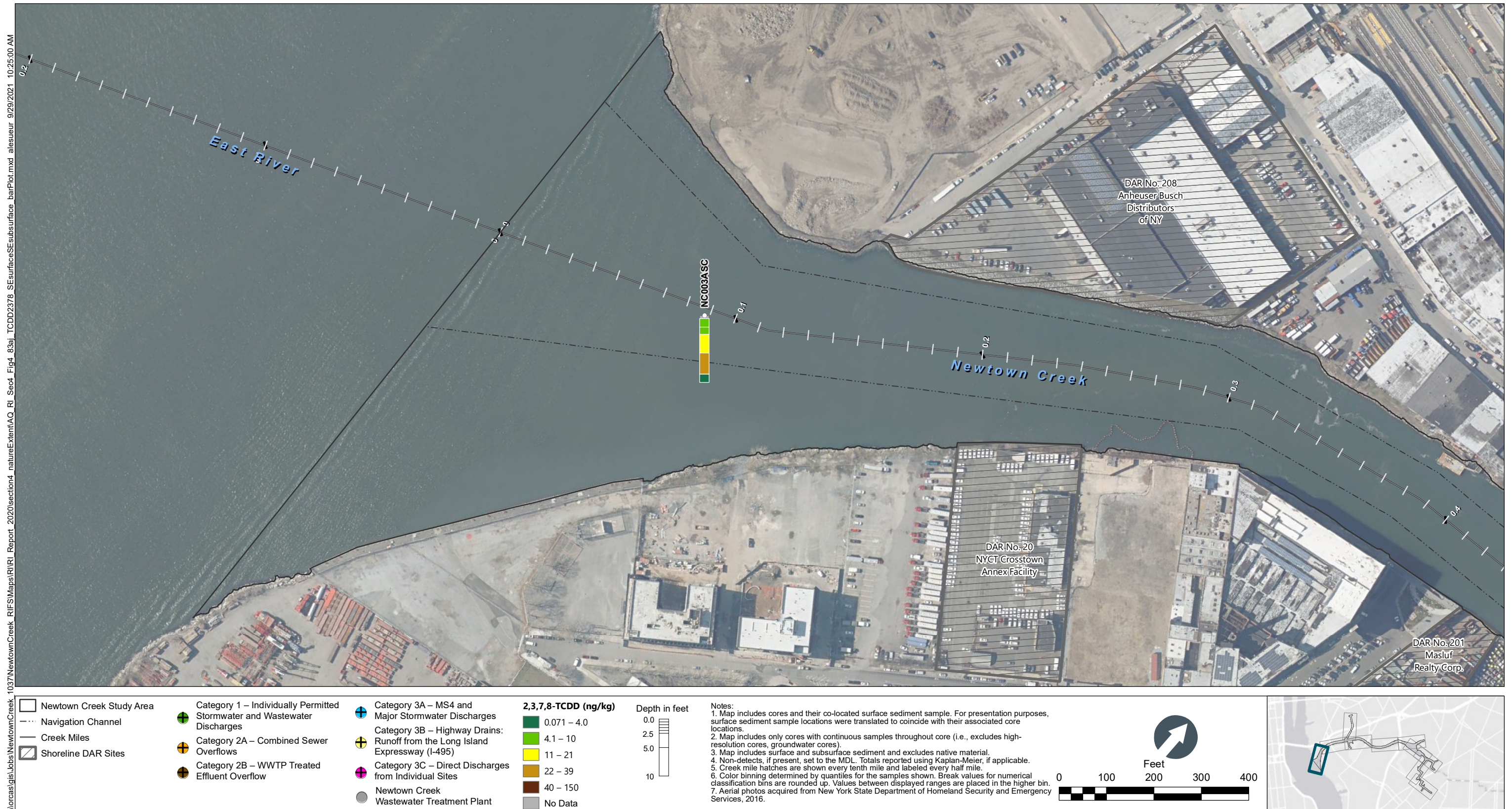
Figure 4-83a 2,3,7,8-TCDD in Surface and Subsurface Sediment Bar Plots by Depth – Plan View of Newtown Creek CM 0 to 0.4 Remedial Investigation Report Newtown Creek RI/FS
