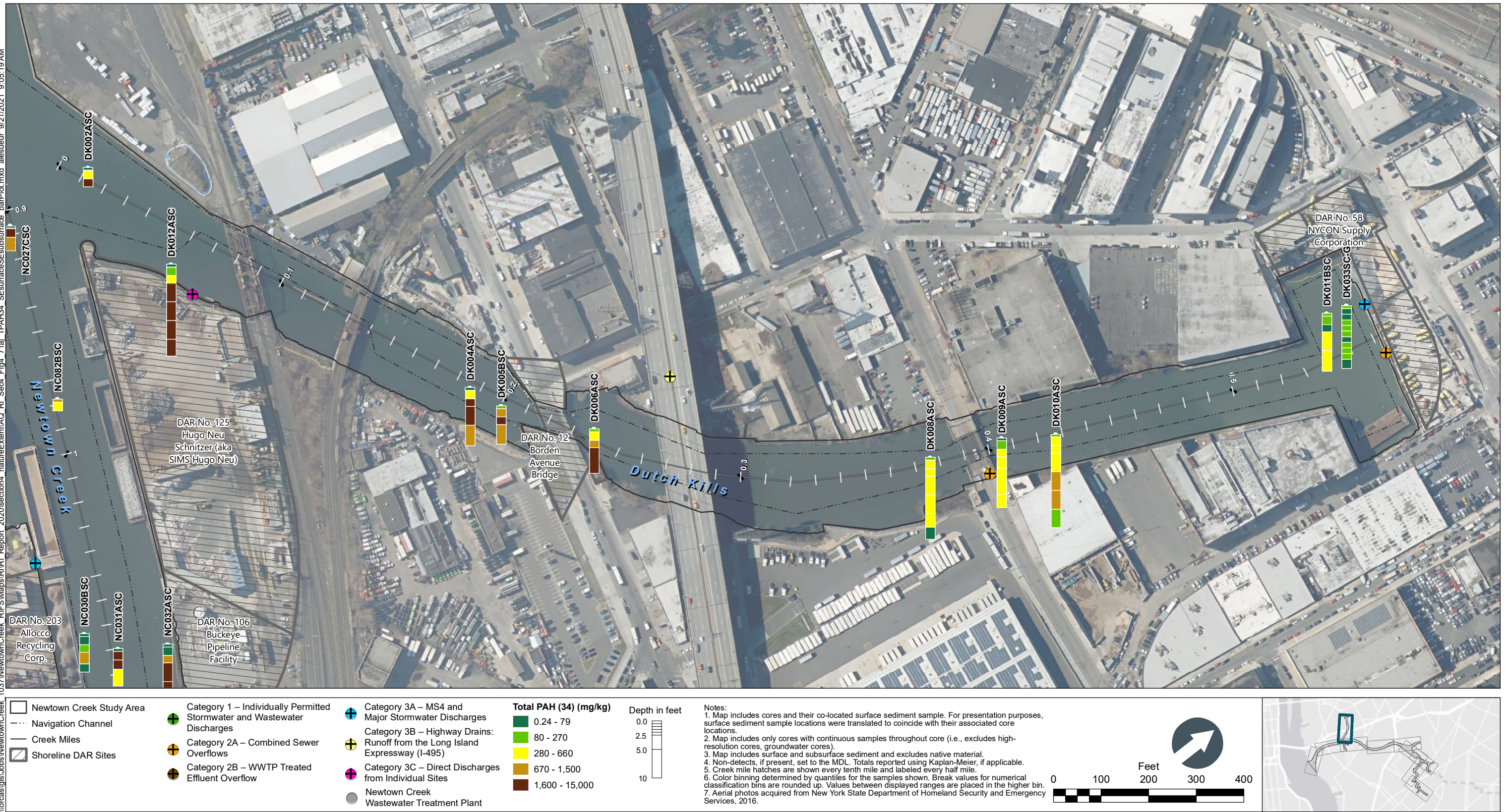
Figure 4-71d Total PAH (34) in Surface and Subsurface Sediment Bar Plots by Depth – Plan View of Dutch Kills CM 0 to 0.5 Remedial Investigation Report Newtown Creek RI/FS
