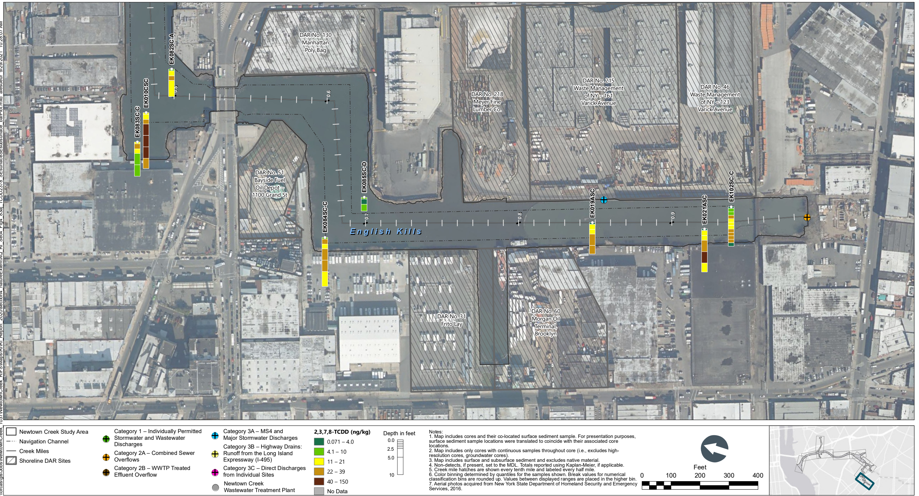
Figure 4-83j 2,3,7,8-TCDD in Surface and Subsurface Sediment Bar Plots by Depth – Plan View of English Kills CM 0.5 to 0.9 Remedial Investigation Report Newtown Creek RI/FS
