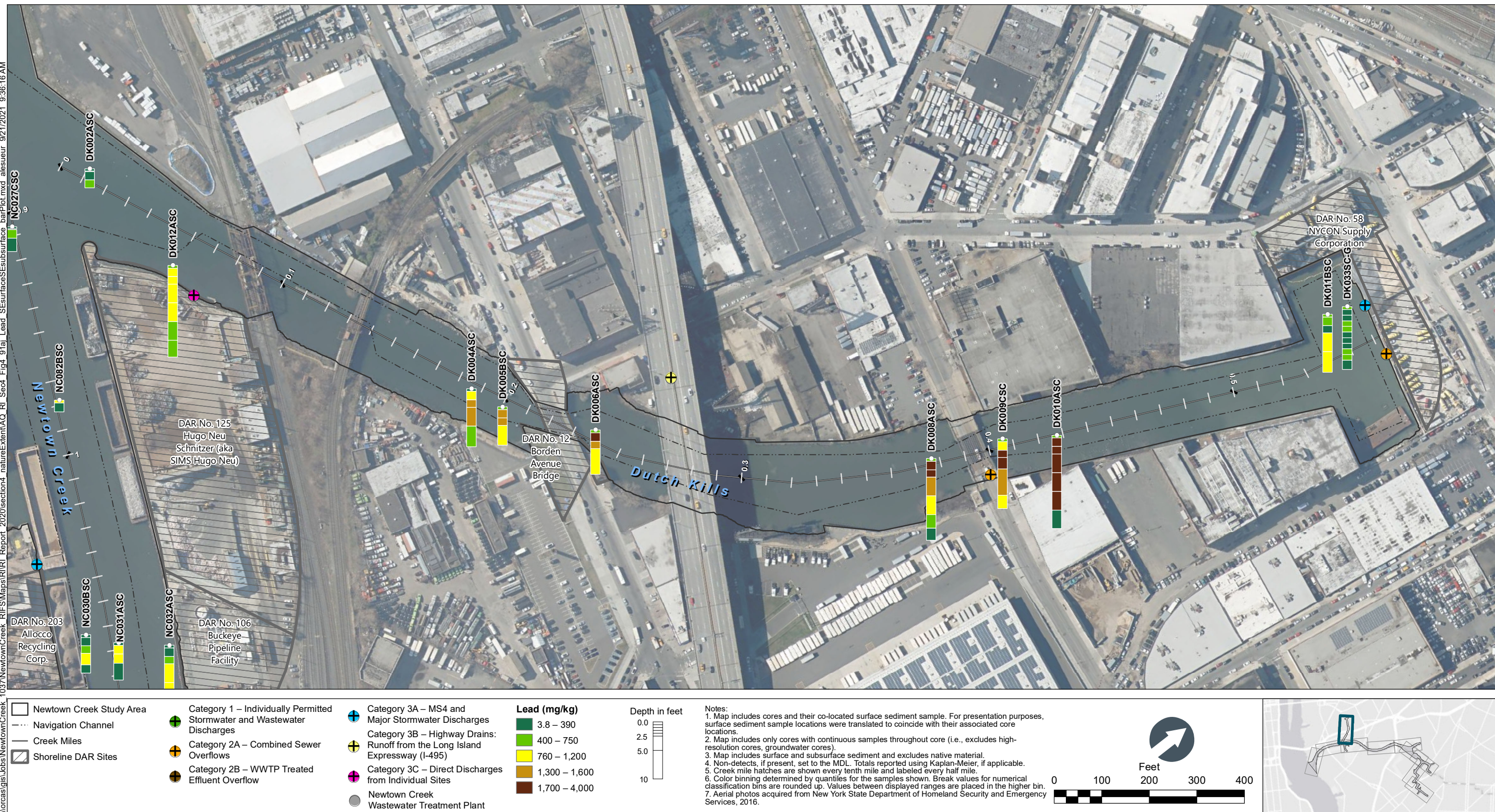
Figure 4-91d Lead in Surface and Subsurface Sediment Bar Plots by Depth – Plan View of Dutch Kills CM 0 to 0.5 Remedial Investigation Report Newtown Creek RI/FS
