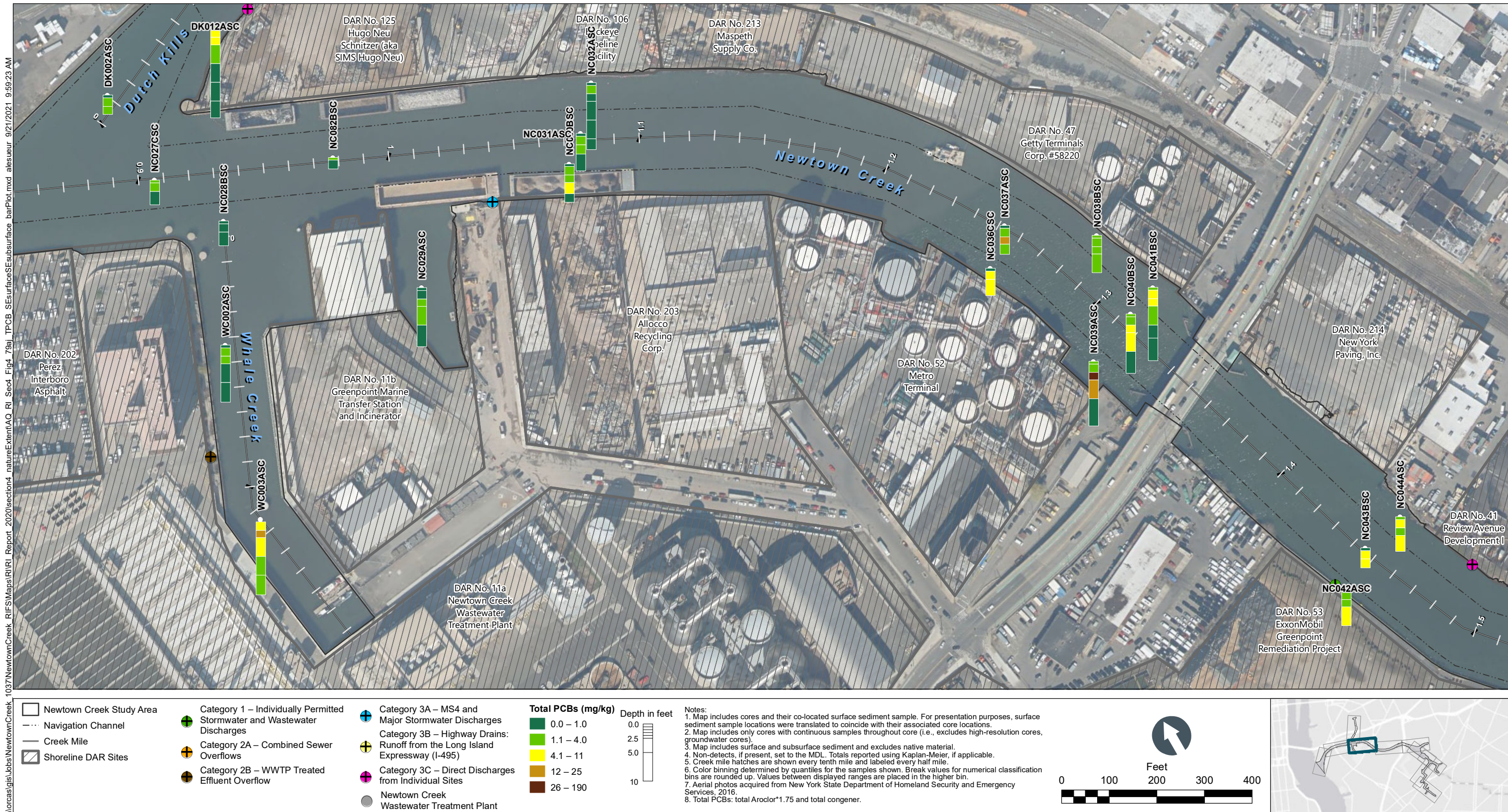
Figure 4-79c Total PCBs in Surface and Subsurface Sediment Bar Plots by Depth – Plan View of Whale Creek and Newtown Creek CM 0.9 to 1.5 Remedial Investigation Report Newtown Creek RI/FS
