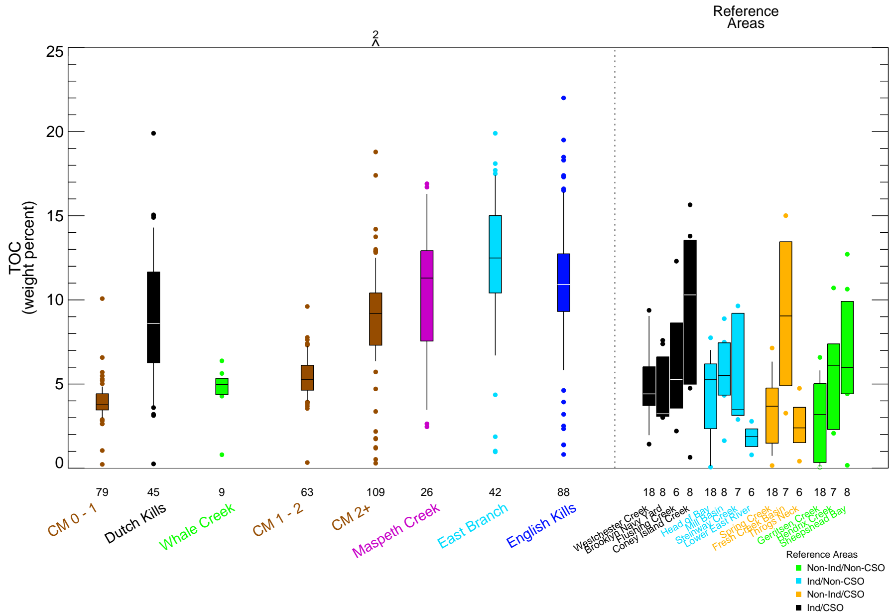
Figure 4-9 TOC in Surface Sediment - Box Plots by Location Remedial Investigation Report Newtown Creek RI/FS
