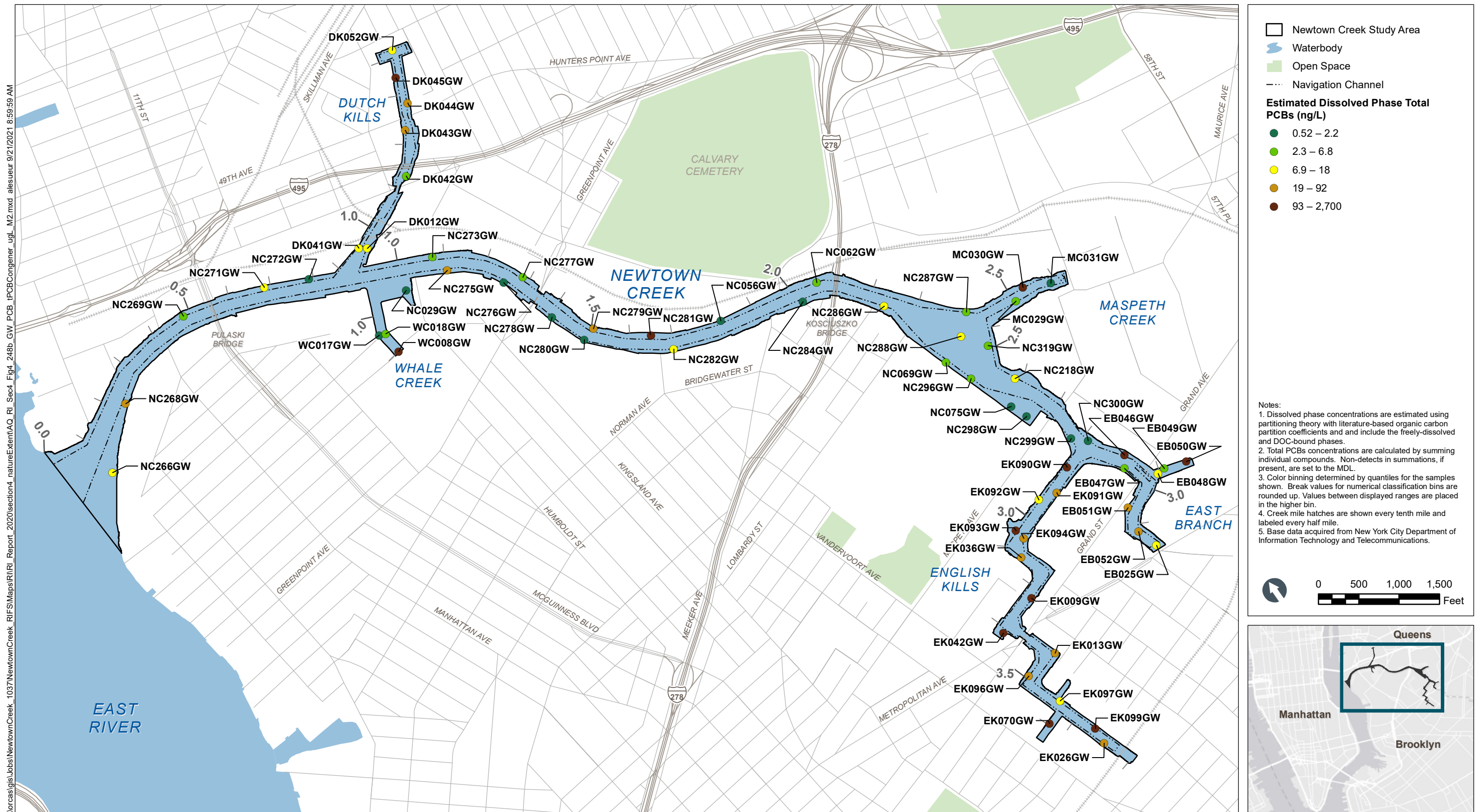
Figure 4-248b Estimated Dissolved Phase (Method 2) Total PCBs in Groundwater – Plan View Remedial Investigation Report Newtown Creek RI/FS
