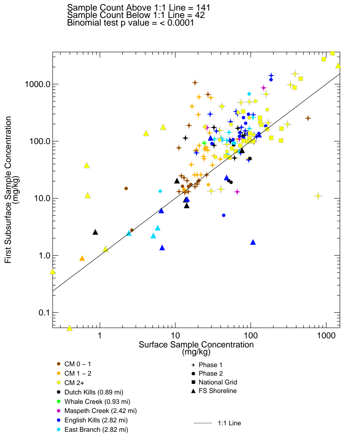
Figure 4–93 Total PAH (17) in Surface Sediment versus Total PAH (17) in First Subsurface Interval – Cross Plot Remedial Investigation Report Newtown Creek RI/FS
