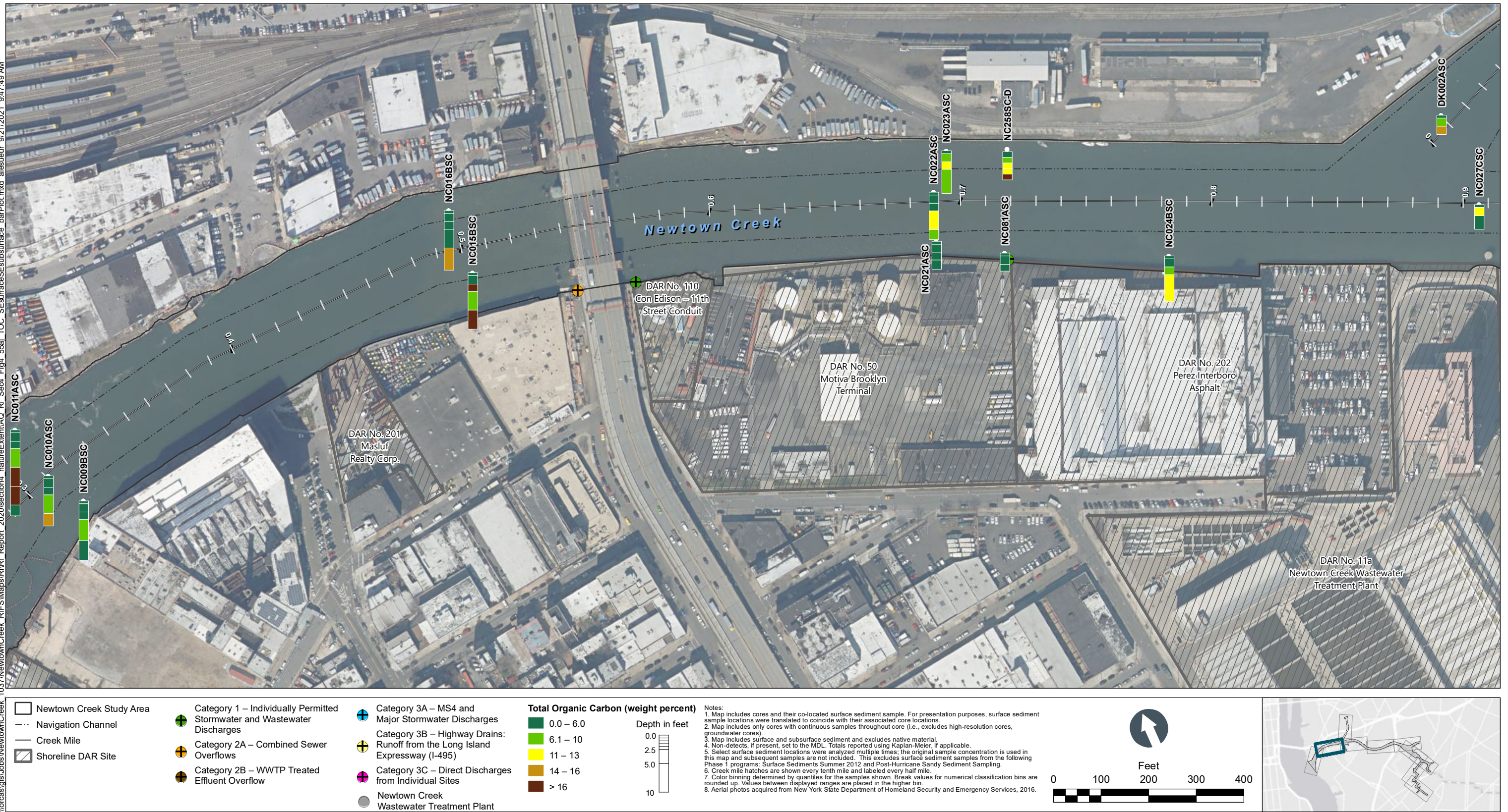
Figure 4-55b TOC in Surface and Subsurface Sediment Bar Plots by Depth – Plan View of Newtown Creek CM 0.3 to 0.9 Remedial Investigation Report Newtown Creek RI/FS
