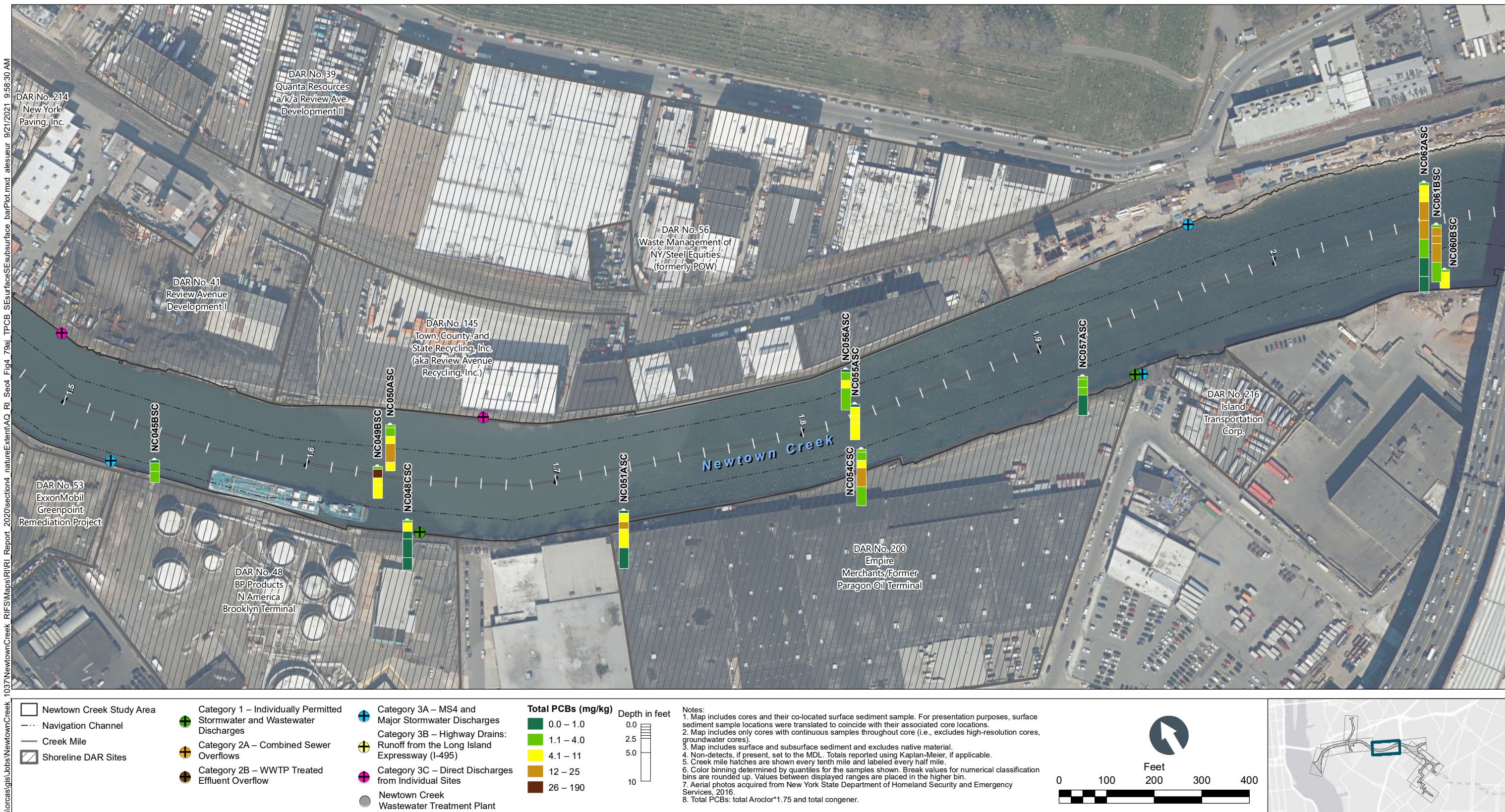
Figure 4-79e Total PCBs in Surface and Subsurface Sediment Bar Plots by Depth – Plan View of Newtown Creek CM 1.5 to 2.0 Remedial Investigation Report Newtown Creek RI/FS
