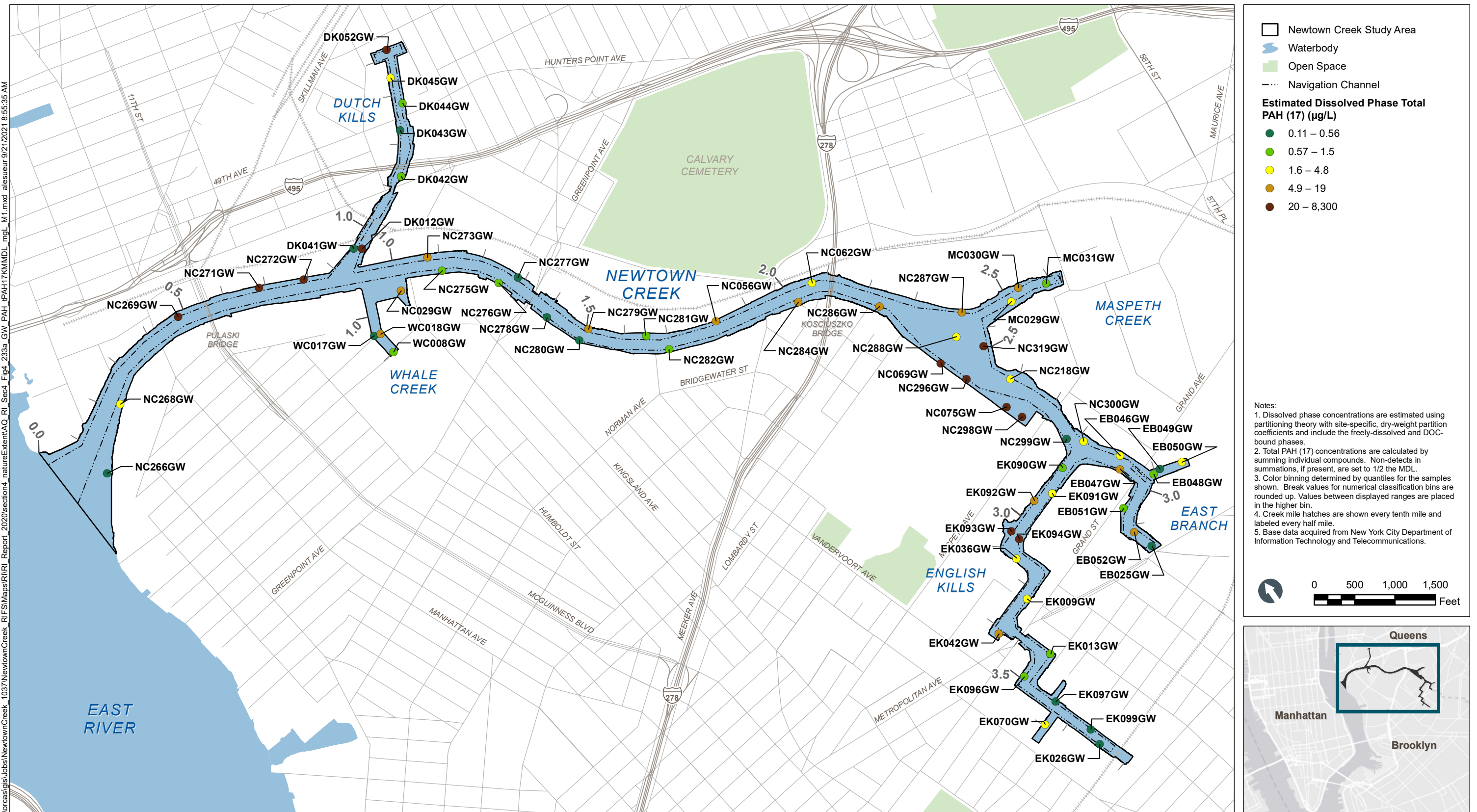
Figure 4-233a Estimated Dissolved Phase (Method 1) Total PAH (17) in Groundwater – Plan View Remedial Investigation Report Newtown Creek RI/FS
