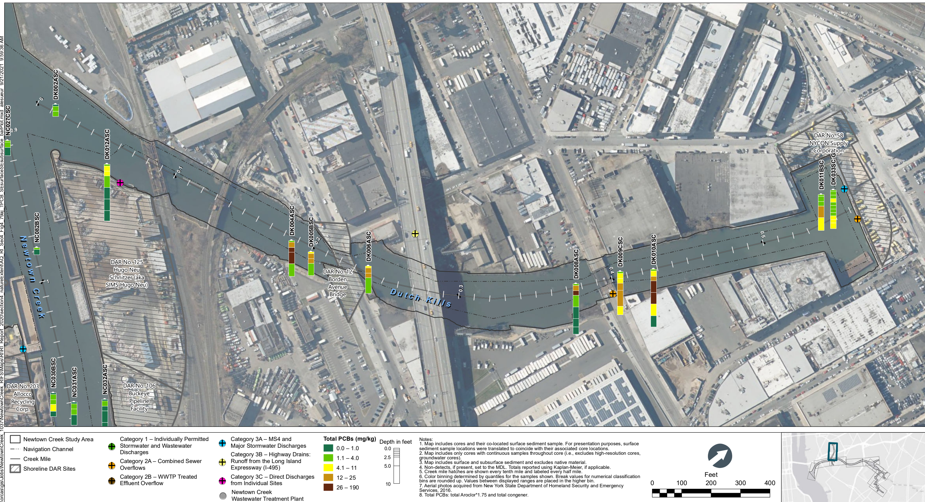
Figure 4-79d Total PCBs in Surface and Subsurface Sediment Bar Plots by Depth – Plan View of Dutch Kills CM 0 to 0.5 Remedial Investigation Report Newtown Creek RI/FS
