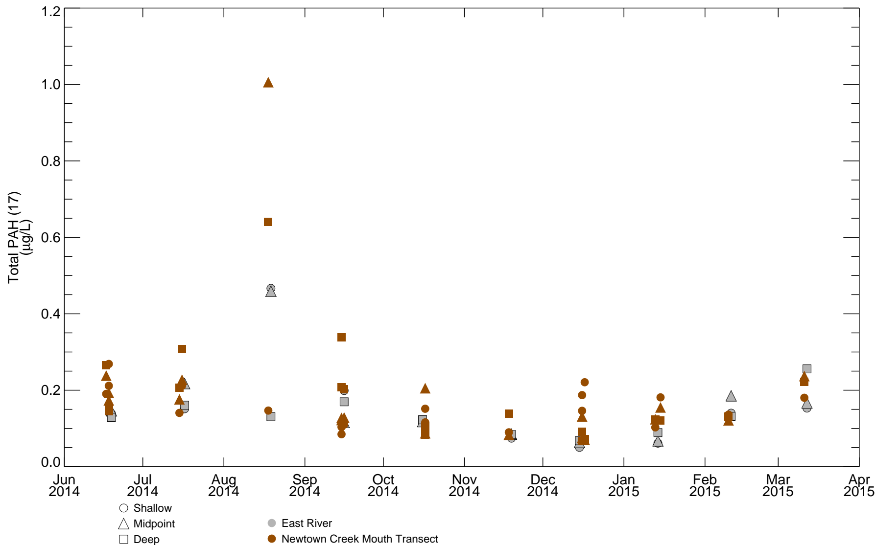
Figure 5-32 Total PAH (17) in East River Surface Water - Temporal Remedial Investigation Report Newtown Creek RI/FS
