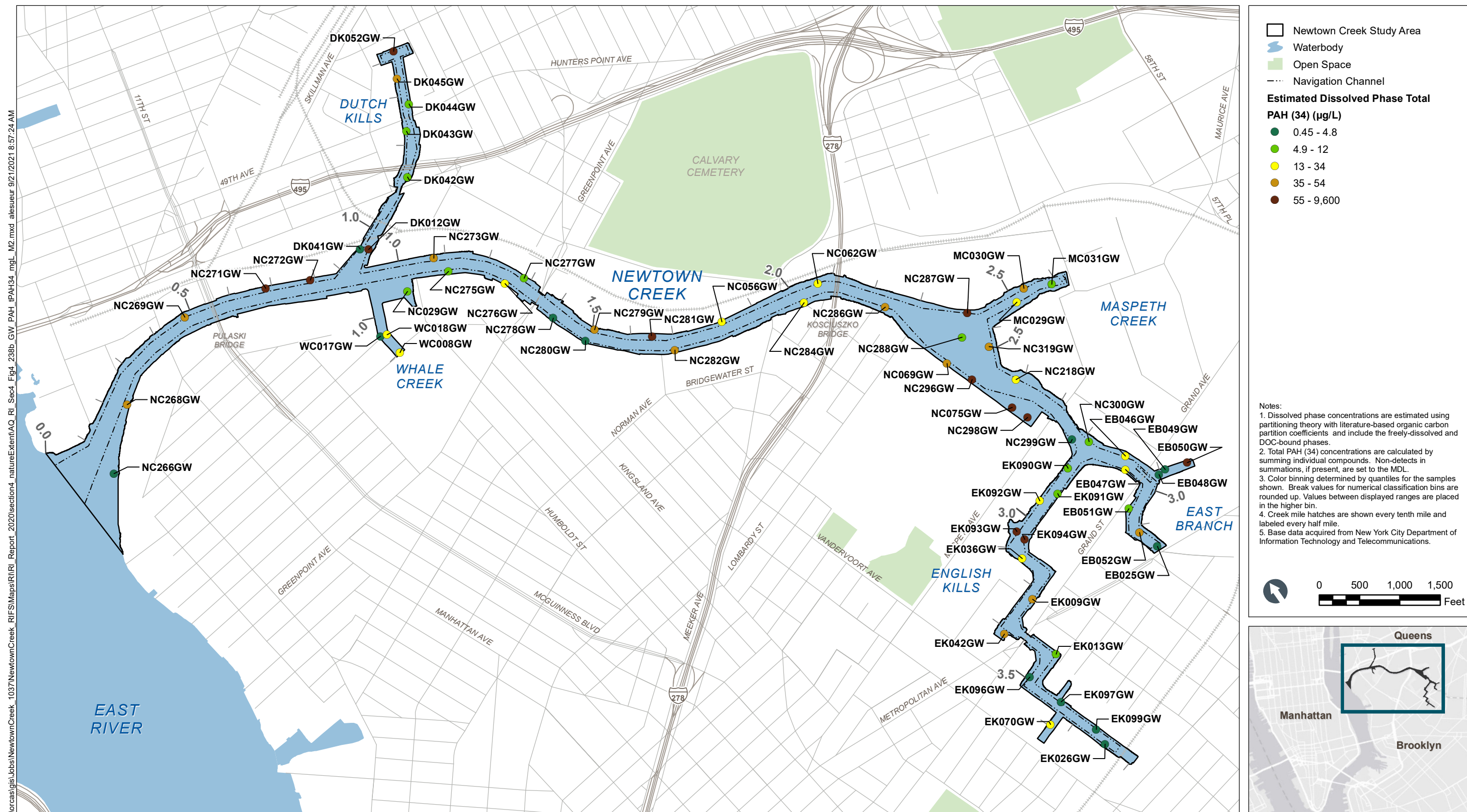
Figure 4-238b Estimated Dissolved Phase (Method 2) Total PAH (34) in Groundwater – Plan View Remedial Investigation Report Newtown Creek RI/FS
