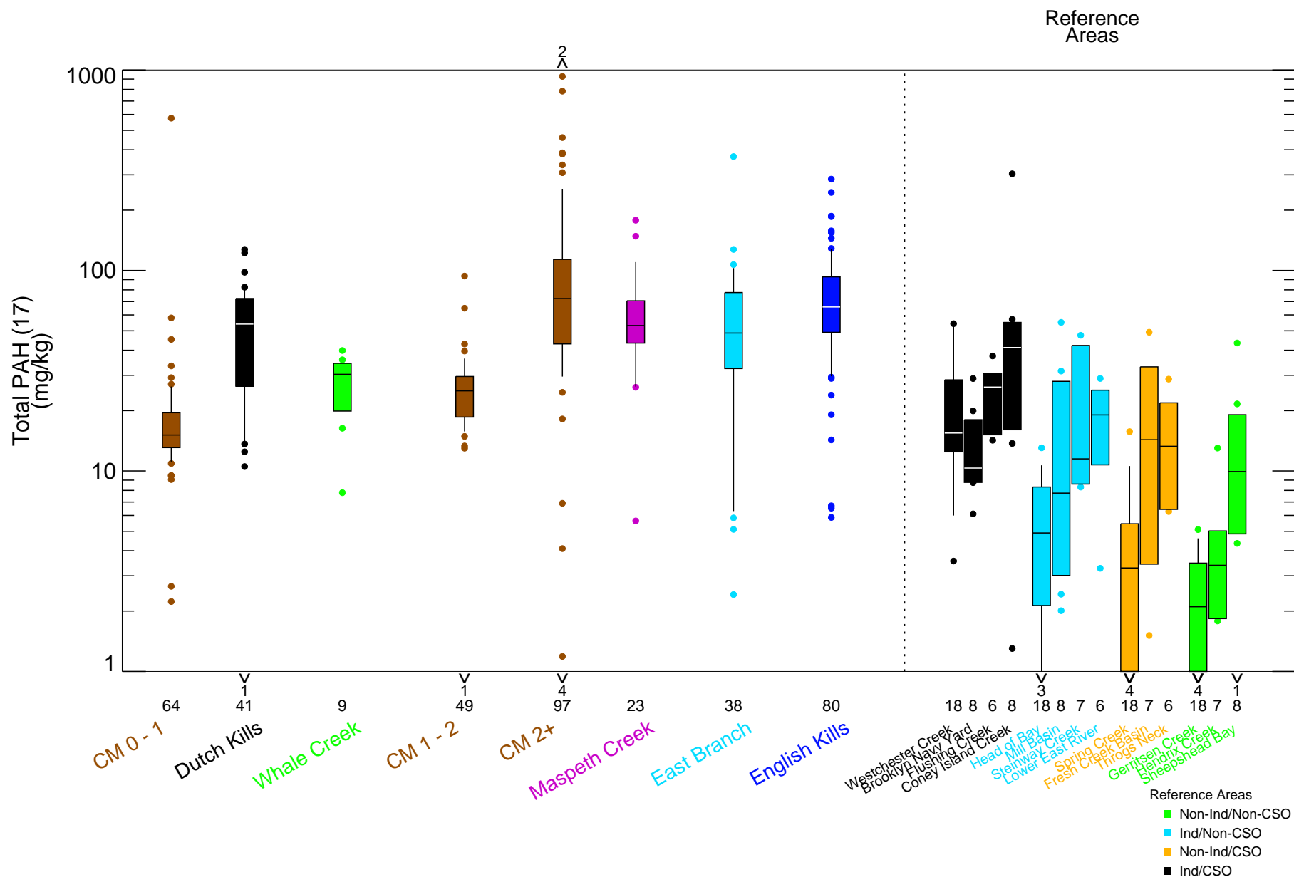
Figure 4-17 Total PAH (17) in Surface Sediment - Box Plots by Location Remedial Investigation Report Newtown Creek RI/FS
