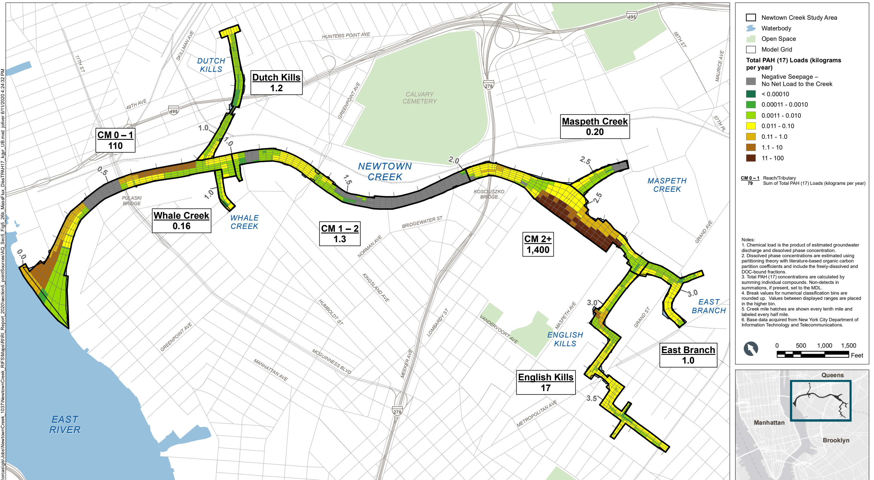
Figure 5-26b Total PAH (17) Loads to Subsurface Sediment from Groundwater – Base Case – Upper Bound (Method 2) Remedial Investigation Report Newtown Creek RI/FS
