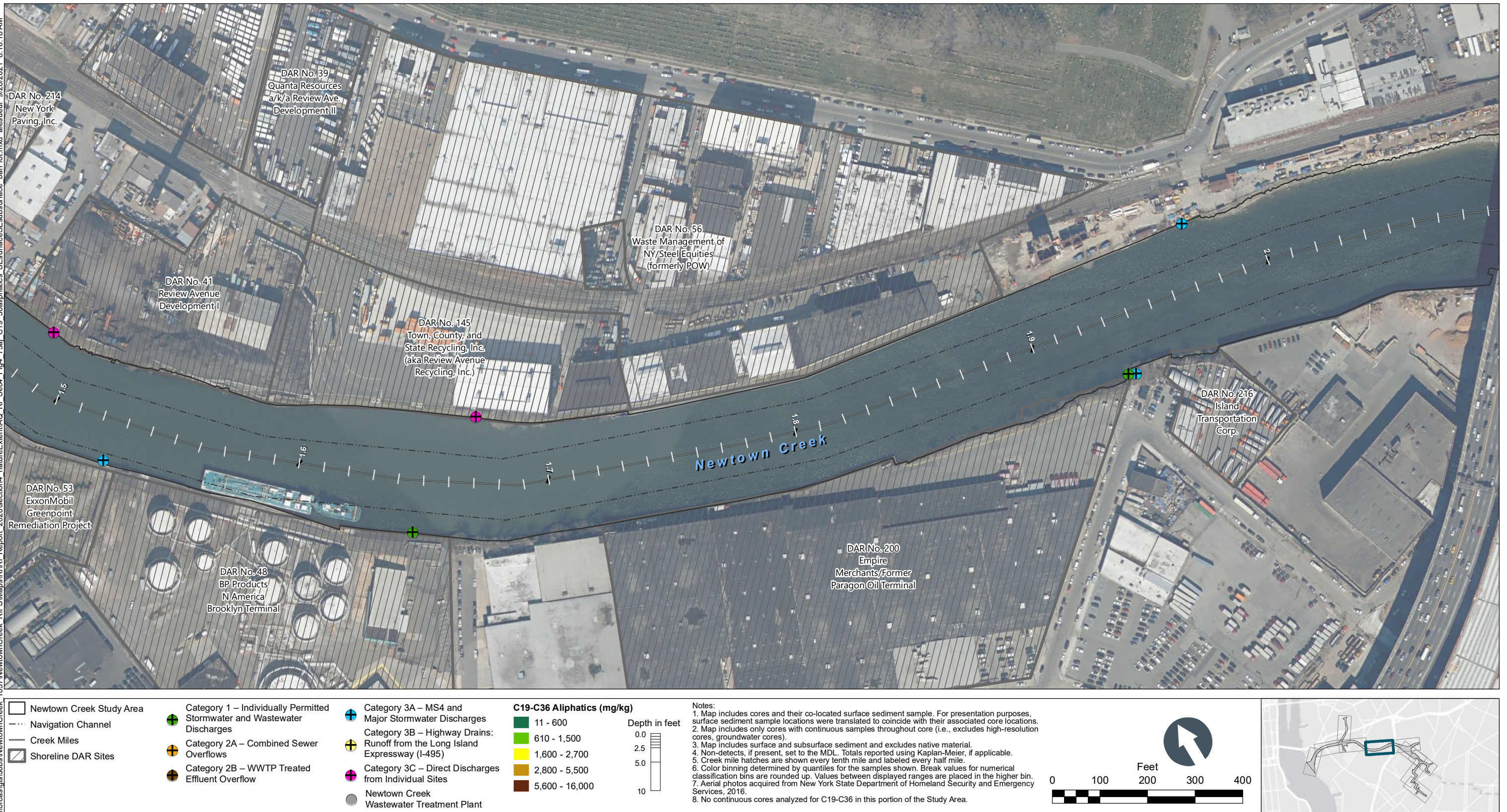
Figure 4-75e C19-C36 Aliphatics in Surface and Subsurface Sediment Bar Plots by Depth – Plan View of Newtown Creek CM 1.5 to 2.0 Remedial Investigation Report Newtown Creek RI/FS
