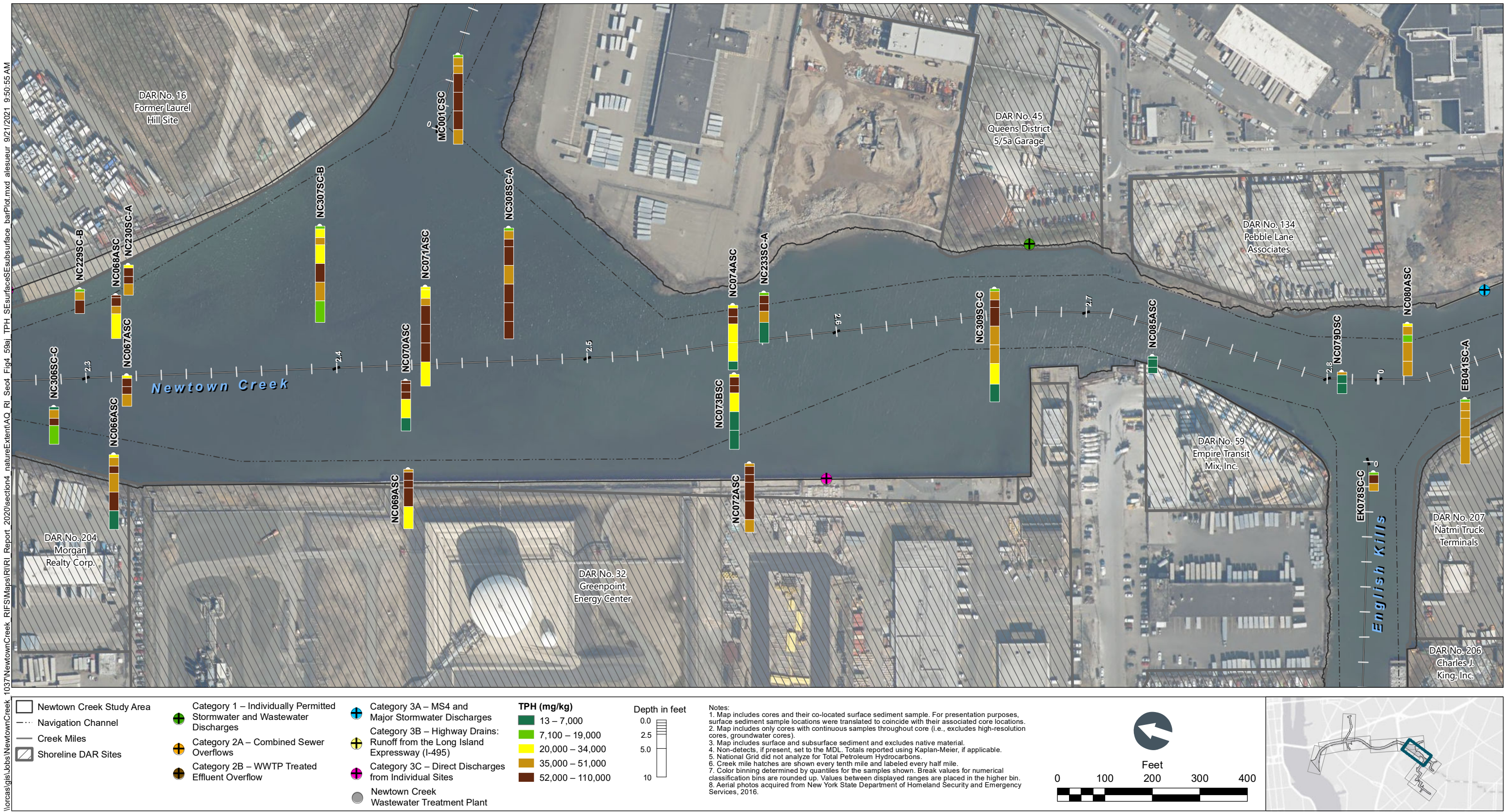
Figure 4-59g TPH in Surface and Subsurface Sediment Bar Plots by Depth – Plan View of Newtown Creek CM 2.3 to 2.8 Remedial Investigation Report Newtown Creek RI/FS
