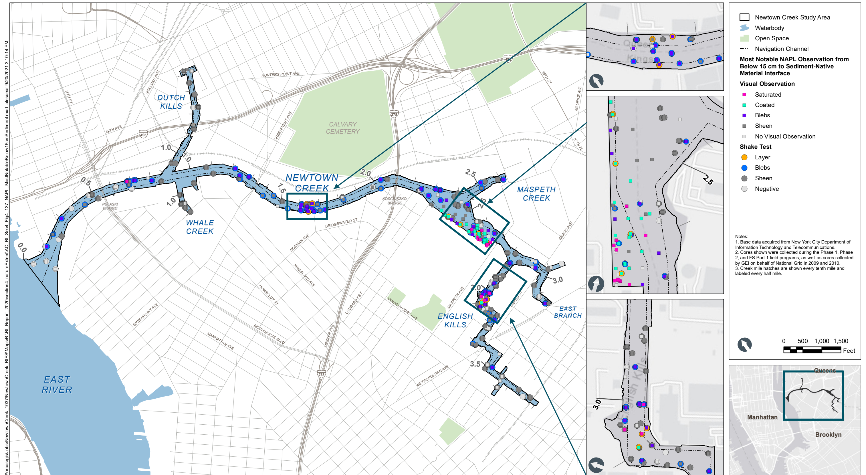
Figure 4-137 Most Notable NAPL Observations in Subsurface Sediment – Plan View Remedial Investigation Report Newtown Creek RI/FS
