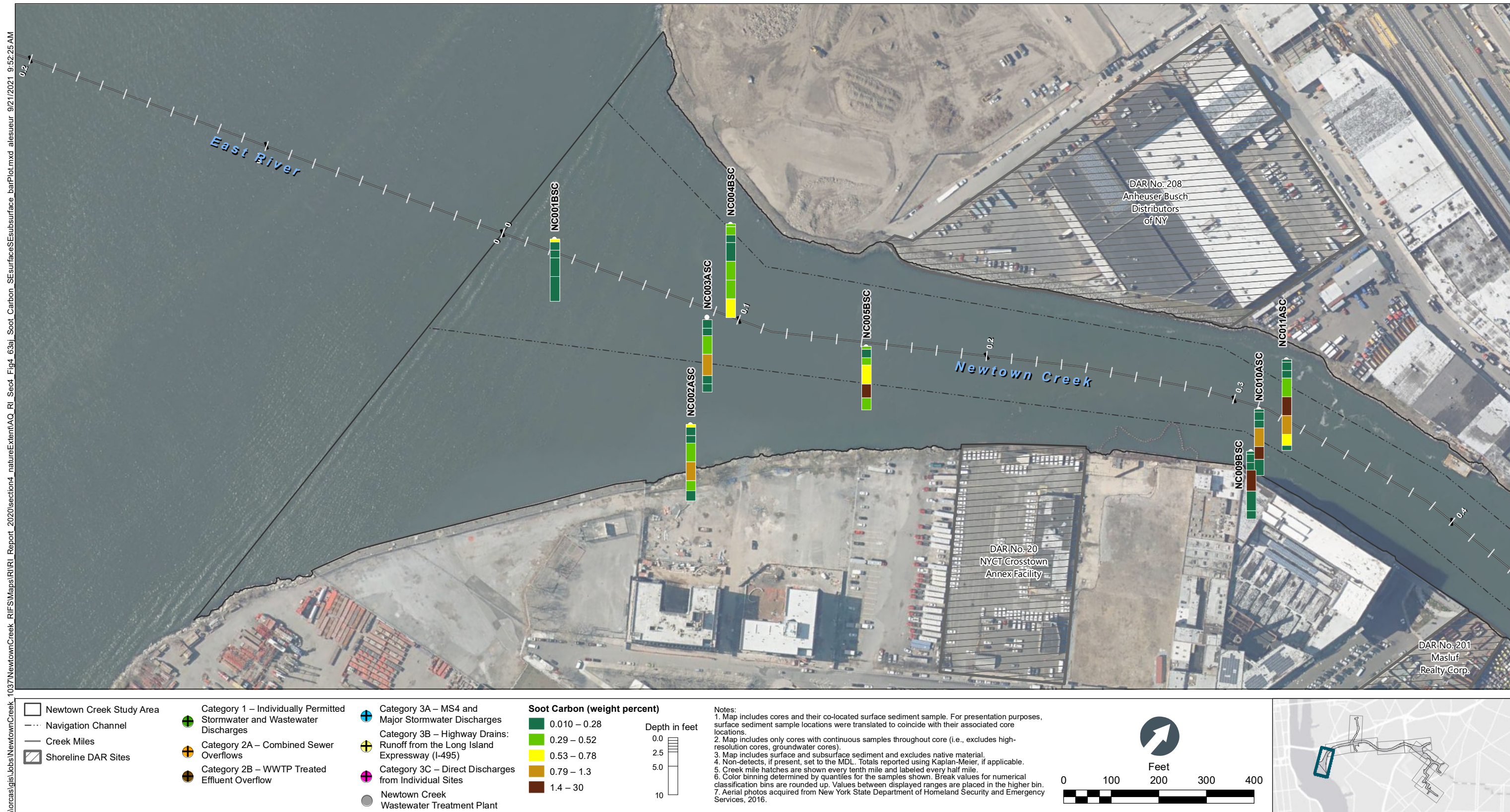
Figure 4-63a Percent Soot Carbon in Surface and Subsurface Sediment Bar Plots by Depth – Plan View of Newtown Creek CM 0 to 0.4 Remedial Investigation Report Newtown Creek RI/FS
