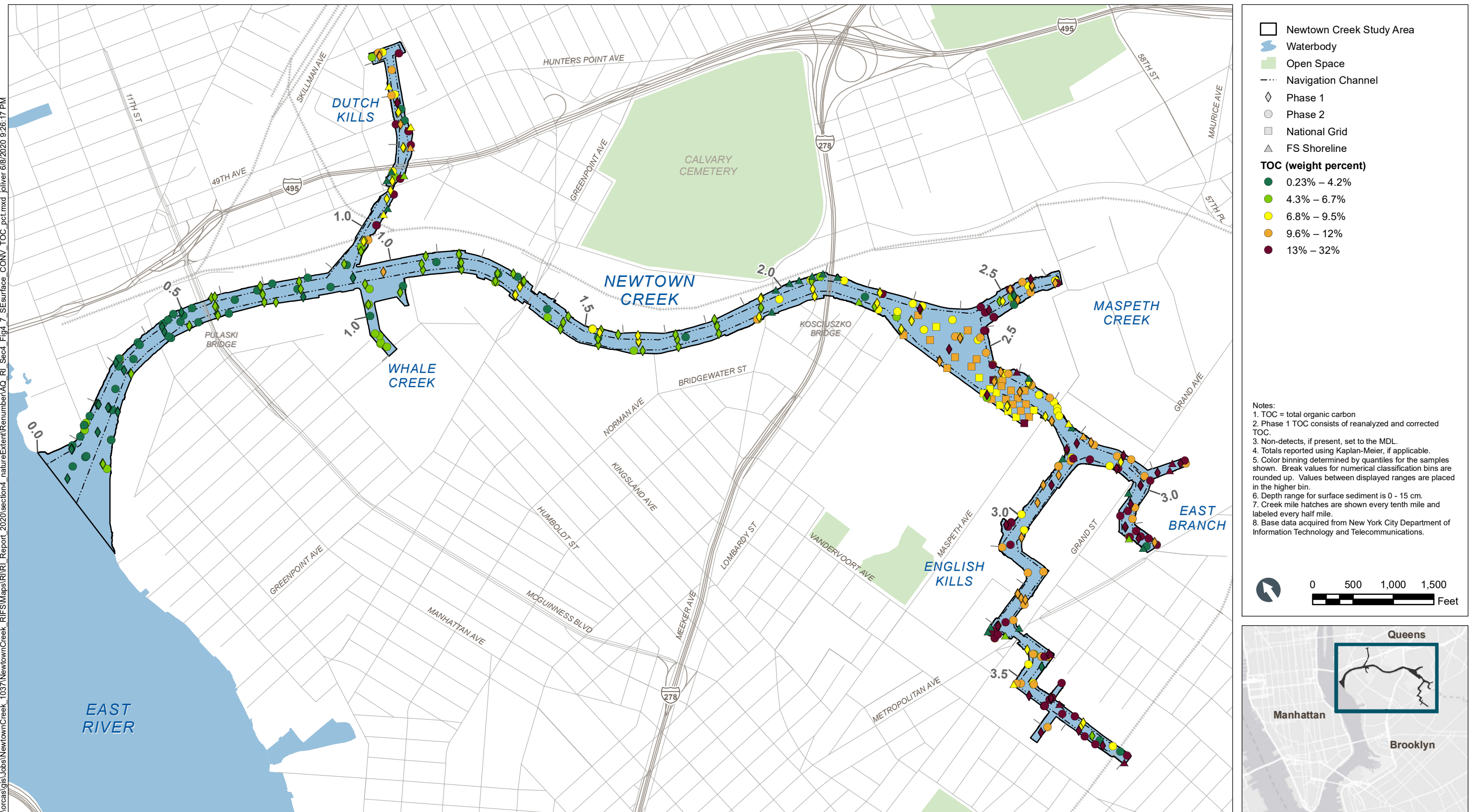
Figure 4-7 TOC in Surface Sediment – Plan View Remedial Investigation Report Newtown Creek RI/FS
