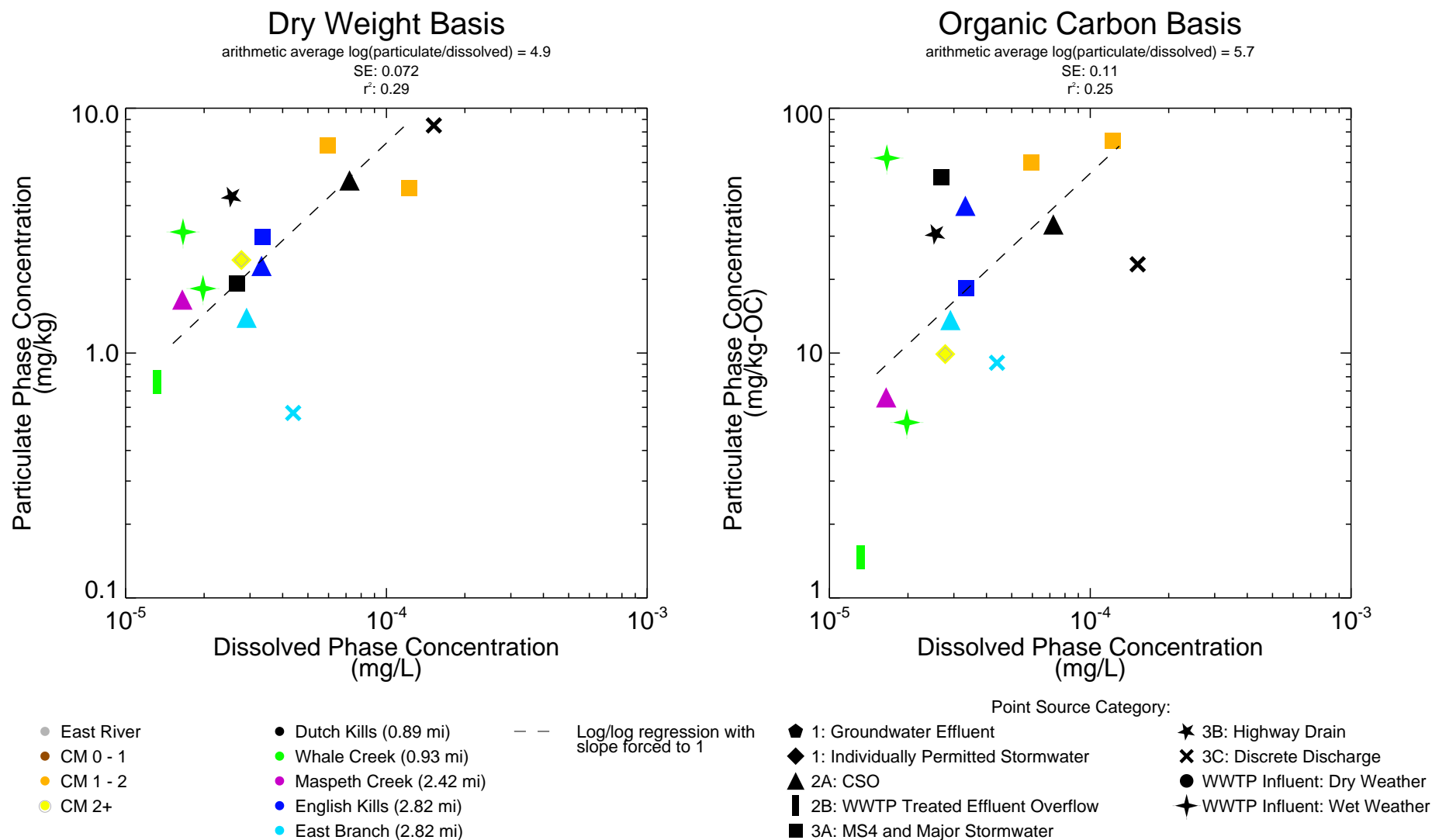
Figure 6-11e Point Source Particulate Phase versus Dissolved Phase for Pyrene - Cross Plots Remedial Investigation Report Newtown Creek RI/FS
