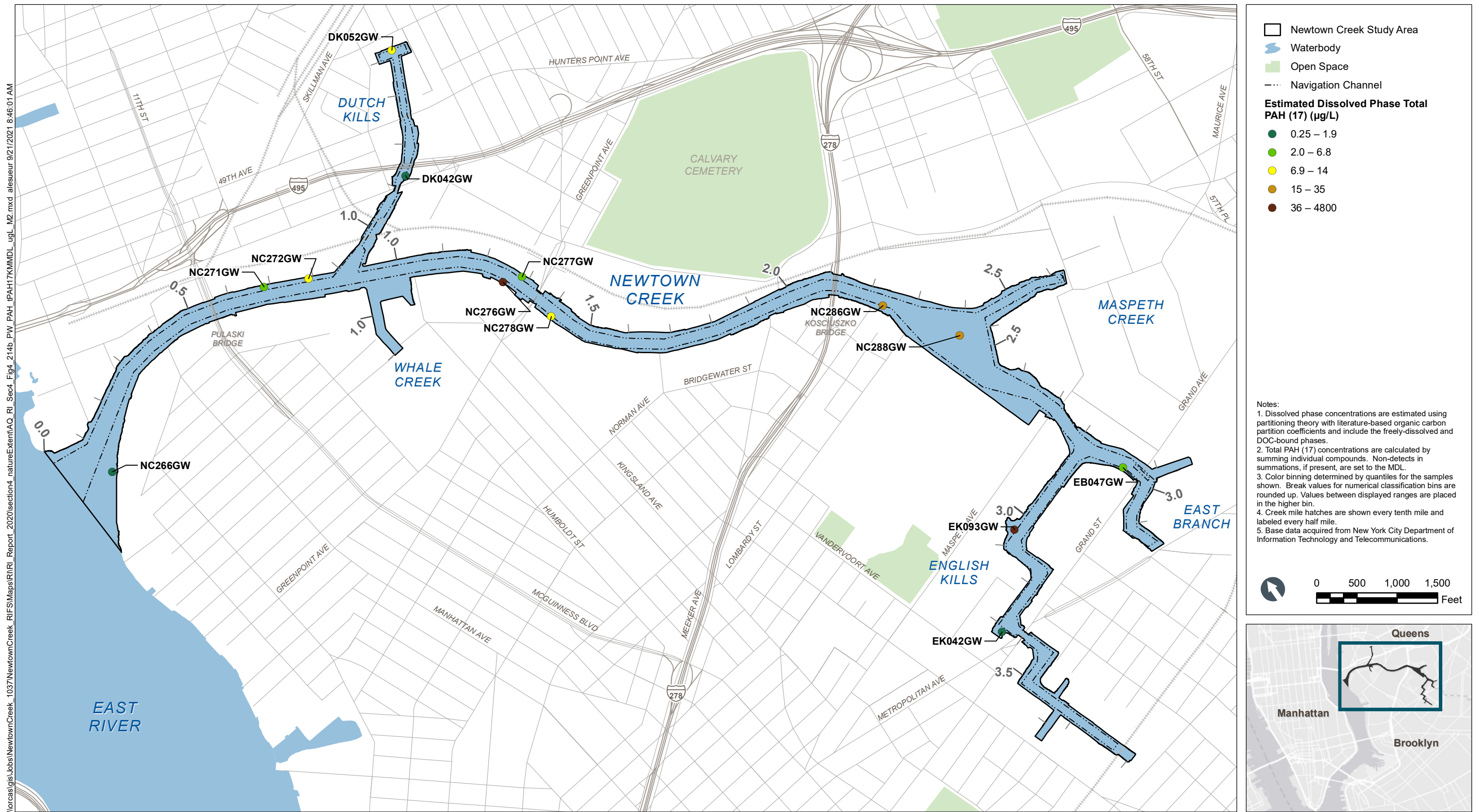
Figure 4-214b Estimated Dissolved Phase (Method 2) Total PAH (17) in Mid-Depth Porewater – Plan View Remedial Investigation Report Newtown Creek RI/FS
