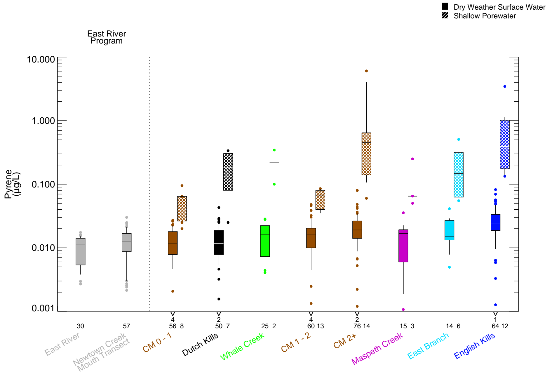
Figure 6-24e Dissolved Phase Pyrene in Surface Water Dry Weather and Shallow Porewater - Box Plots Remedial Investigation Report Newtown Creek RI/FS
