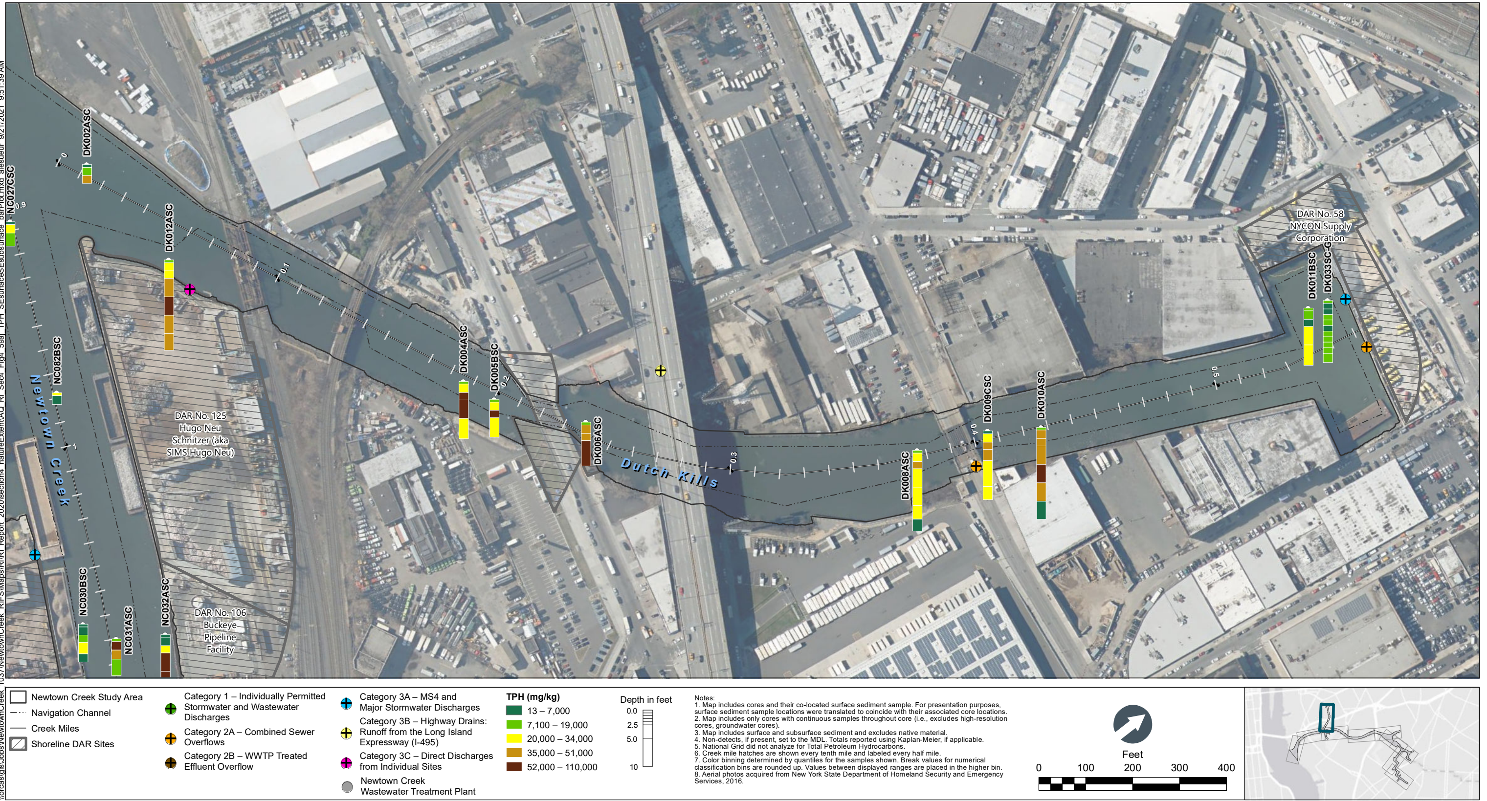
Figure 4-59d TPH in Surface and Subsurface Sediment Bar Plots by Depth – Plan View of Dutch Kills CM 0 to 0.5 Remedial Investigation Report Newtown Creek RI/FS
