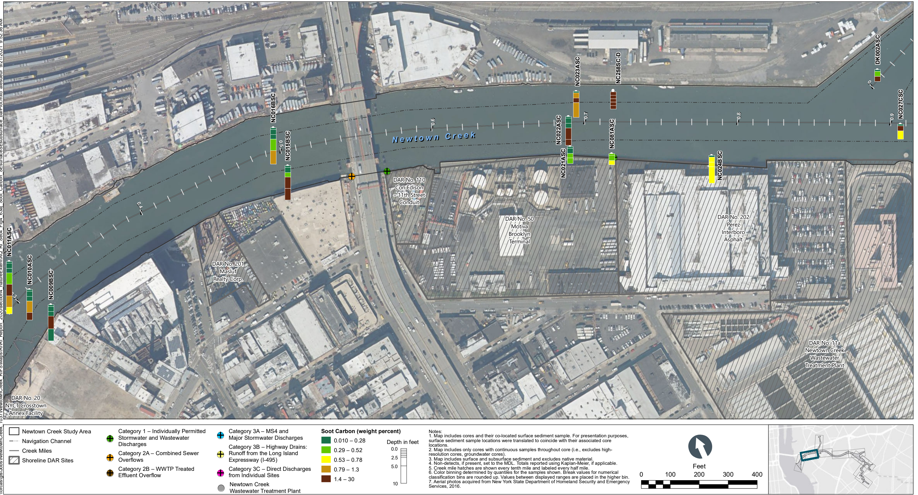
Figure 4-63b Percent Soot Carbon in Surface and Subsurface Sediment Bar Plots by Depth – Plan View of Newtown Creek CM 0.3 to 0.9 Remedial Investigation Report Newtown Creek RI/FS
