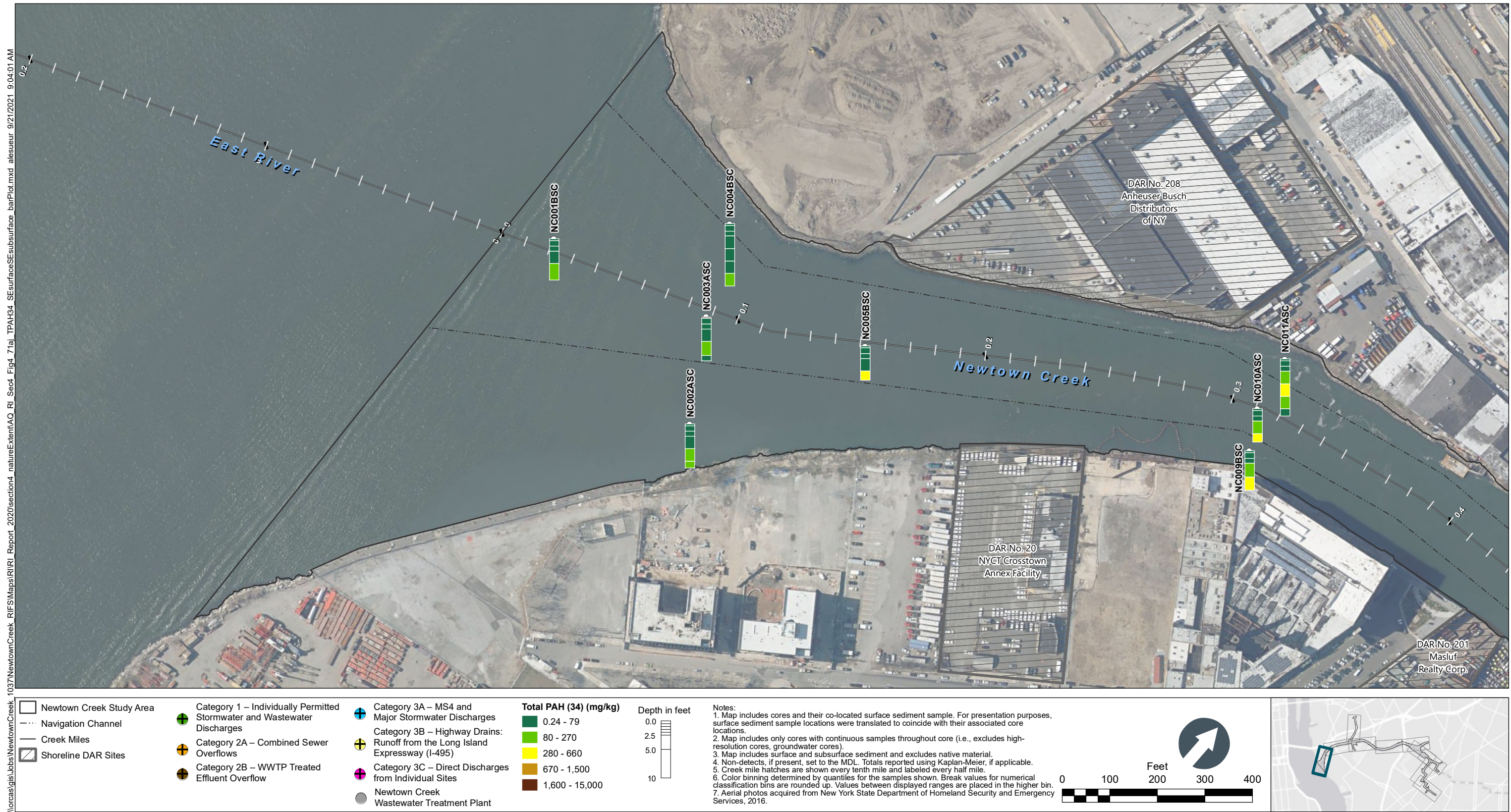
Figure 4-71a Total PAH (34) in Surface and Subsurface Sediment Bar Plots by Depth – Plan View of Newtown Creek CM 0 to 0.4 Remedial Investigation Report Newtown Creek RI/FS
