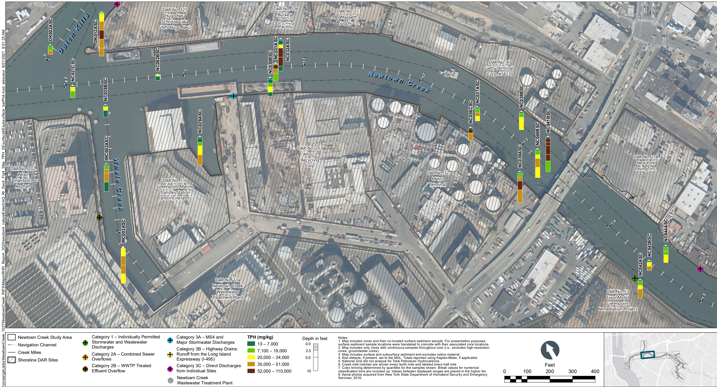
Figure 4-59c TPH in Surface and Subsurface Sediment Bar Plots by Depth – Plan View of Whale Creek and Newtown Creek CM 0.9 to 1.5 Remedial Investigation Report Newtown Creek RI/FS
