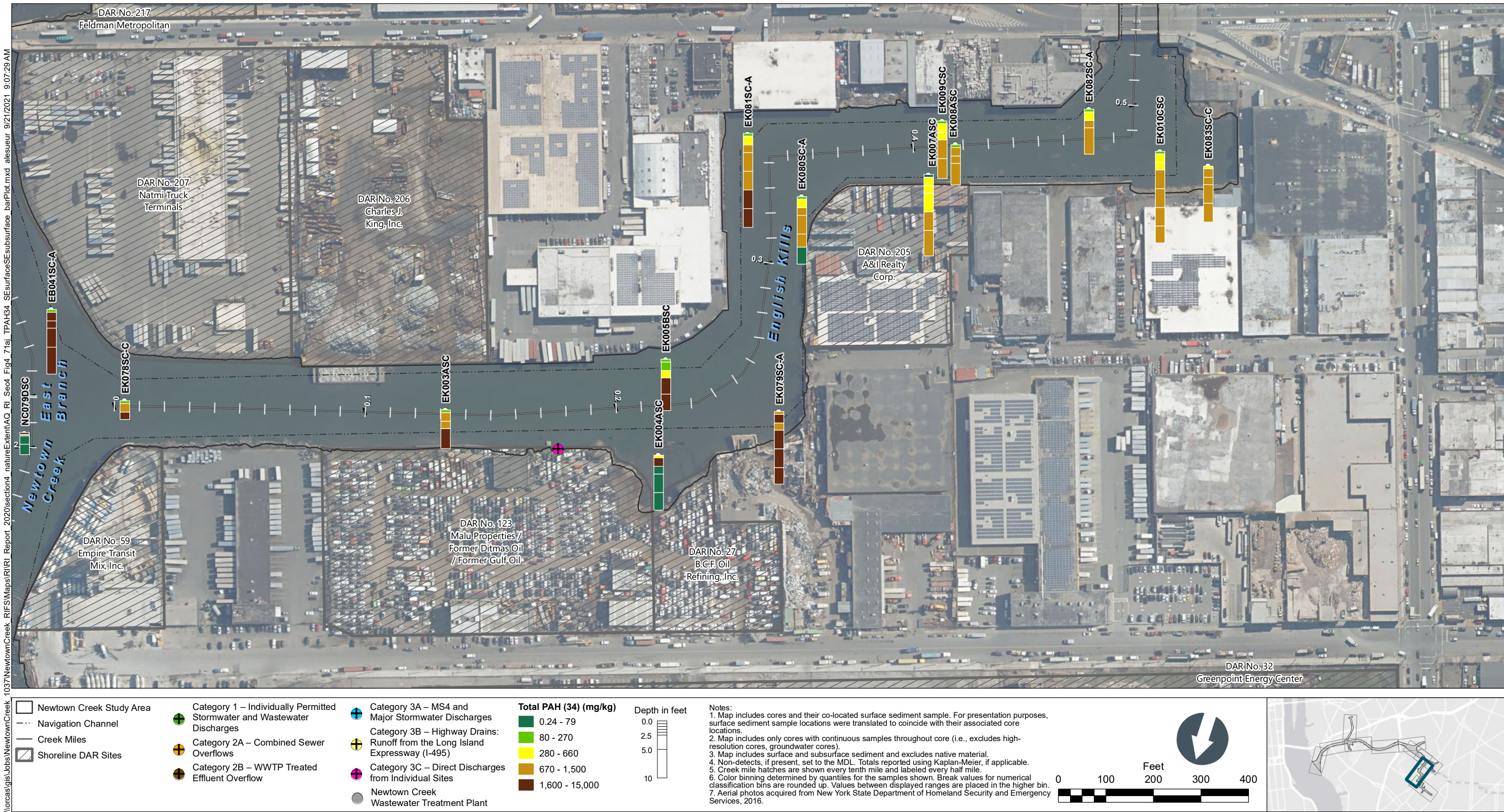
Figure 4-71i Total PAH (34) in Surface and Subsurface Sediment Bar Plots by Depth – Plan View of English Kills CM 0 to 0.5 Remedial Investigation Report Newtown Creek RI/FS
