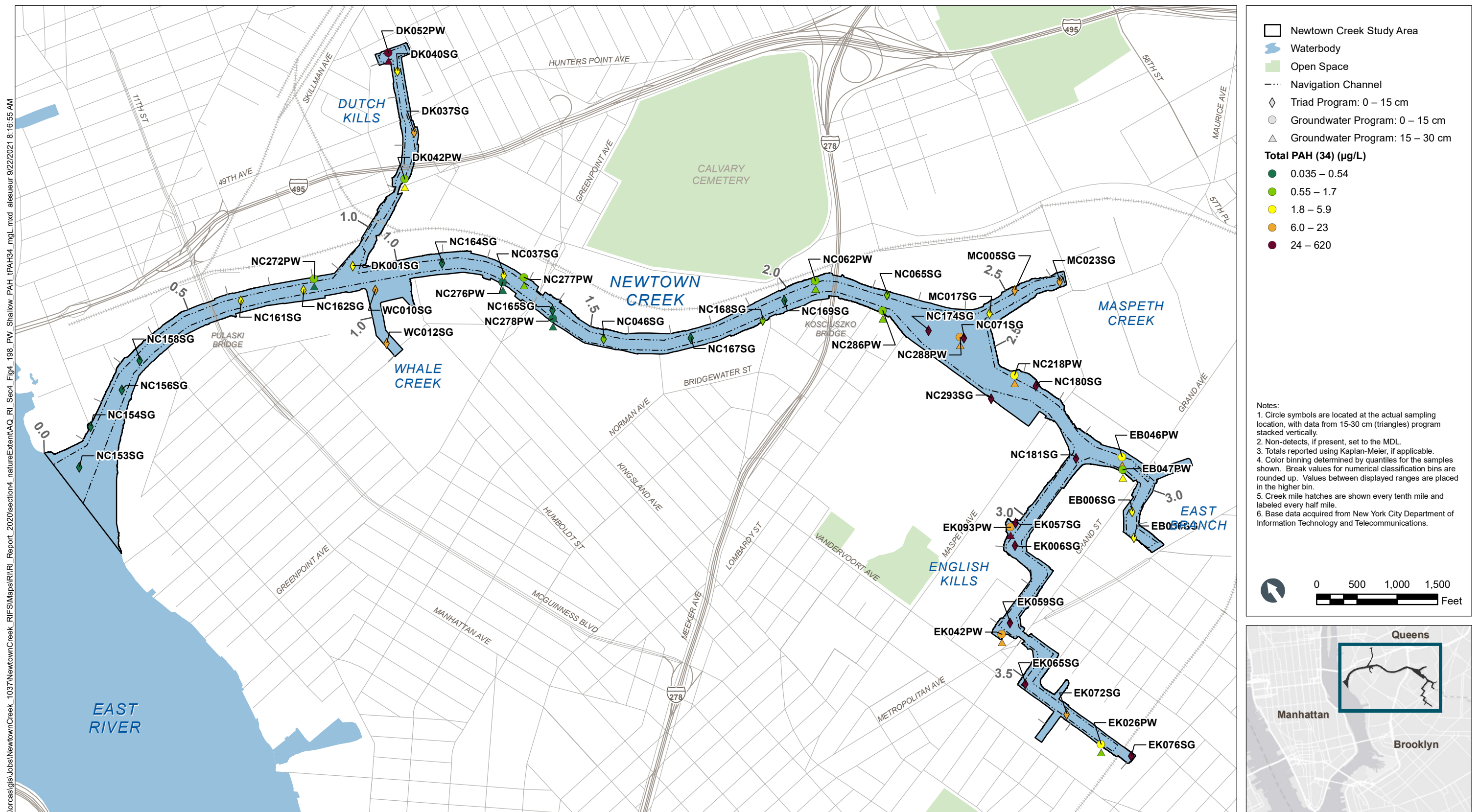
Figure 4-198 Total PAH (34) in Shallow Porewater – Plan View Remedial Investigation Report Newtown Creek RI/FS
