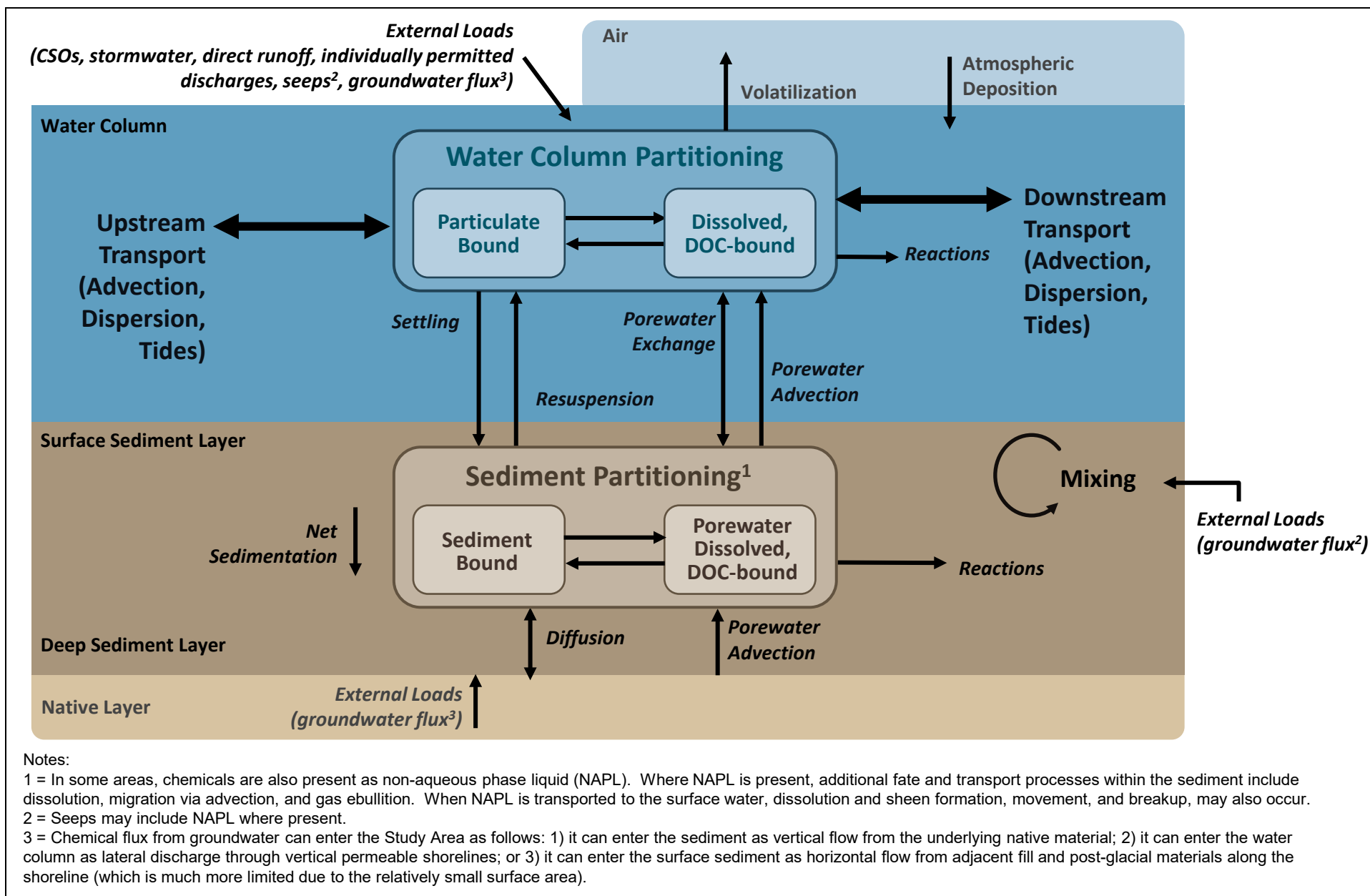
Figure 6-1 Chemical Fate and Transport Processes Remedial Investigation Report Newtown Creek RI/FS
