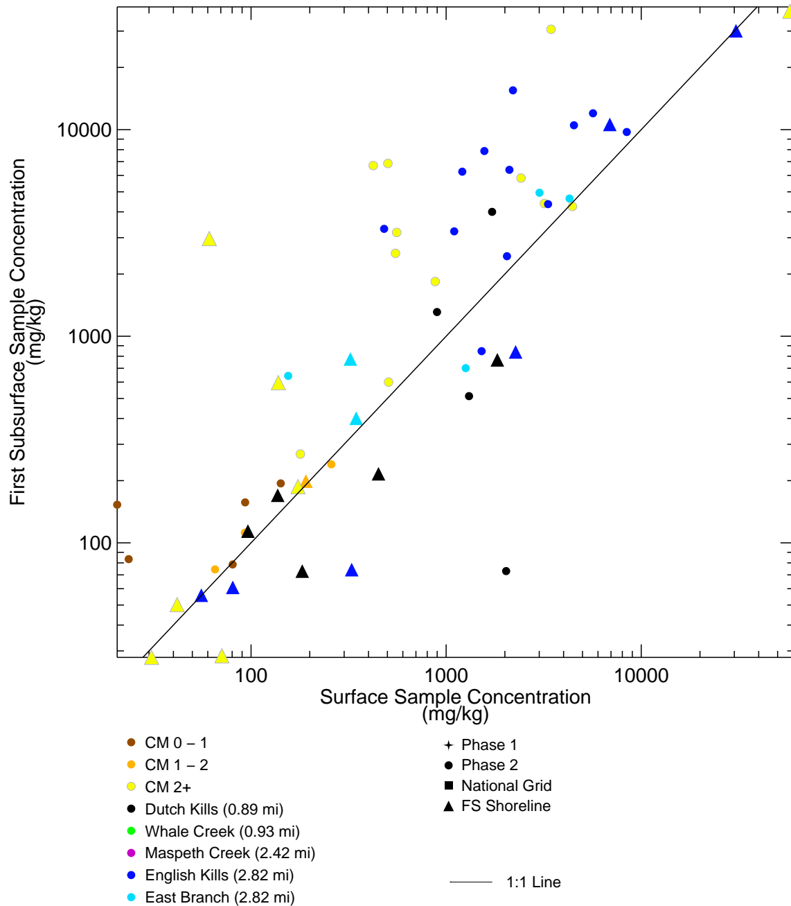
Figure 4-95 C19–C36 Aliphatics in Surface Sediment versus C19–C36 Aliphatics in First Subsurface Interval – Cross Plot Remedial Investigation Report Newtown Creek RI/FS
