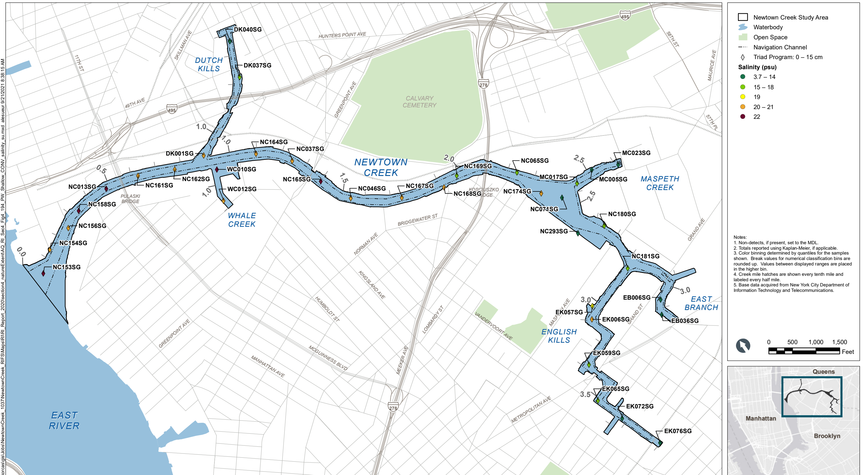
Figure 4-194 Salinity in Shallow Porewater – Plan View Remedial Investigation Report Newtown Creek RI/FS
