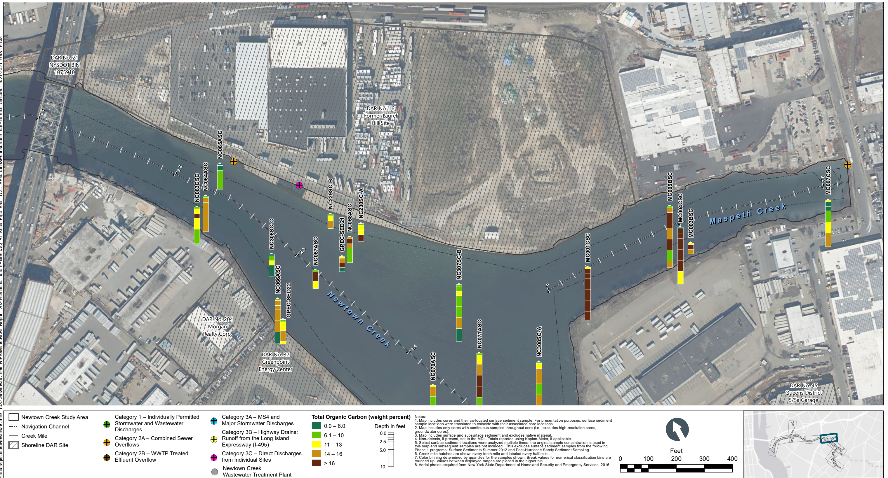
Figure 4-55f TOC in Surface and Subsurface Sediment Bar Plots by Depth – Plan View of Maspeth Creek and Newtown Creek CM 2.1 to 2.4 Remedial Investigation Report Newtown Creek RI/FS
