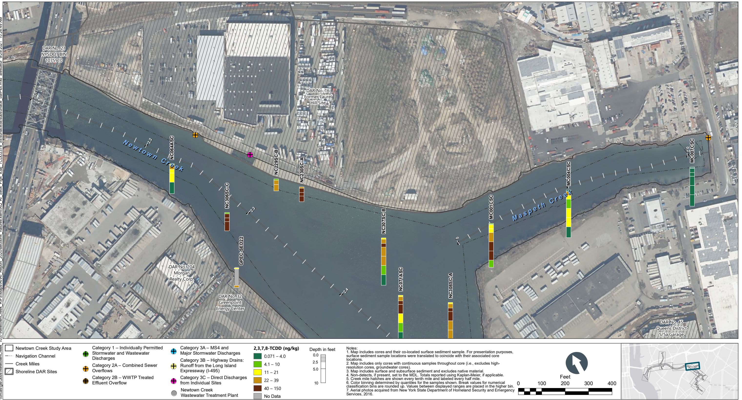
Figure 4-83f 2,3,7,8-TCDD in Surface and Subsurface Sediment Bar Plots by Depth – Plan View of Maspeth Creek and Newtown Creek CM 2.1 to 2.4 Remedial Investigation Report Newtown Creek RI/FS
