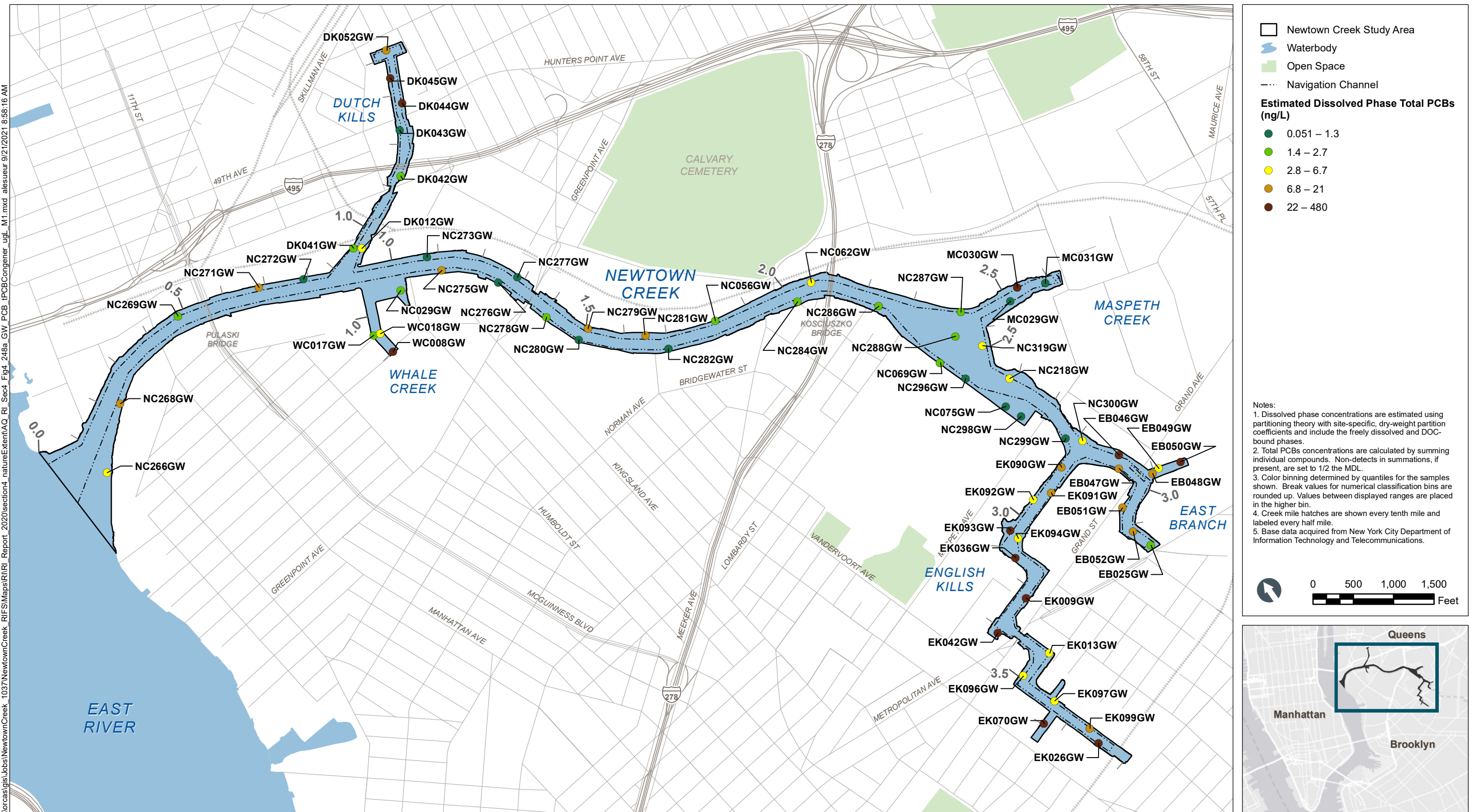
Figure 4-248a Estimated Dissolved Phase (Method 1) Total PCBs in Groundwater – Plan View Remedial Investigation Report Newtown Creek RI/FS
