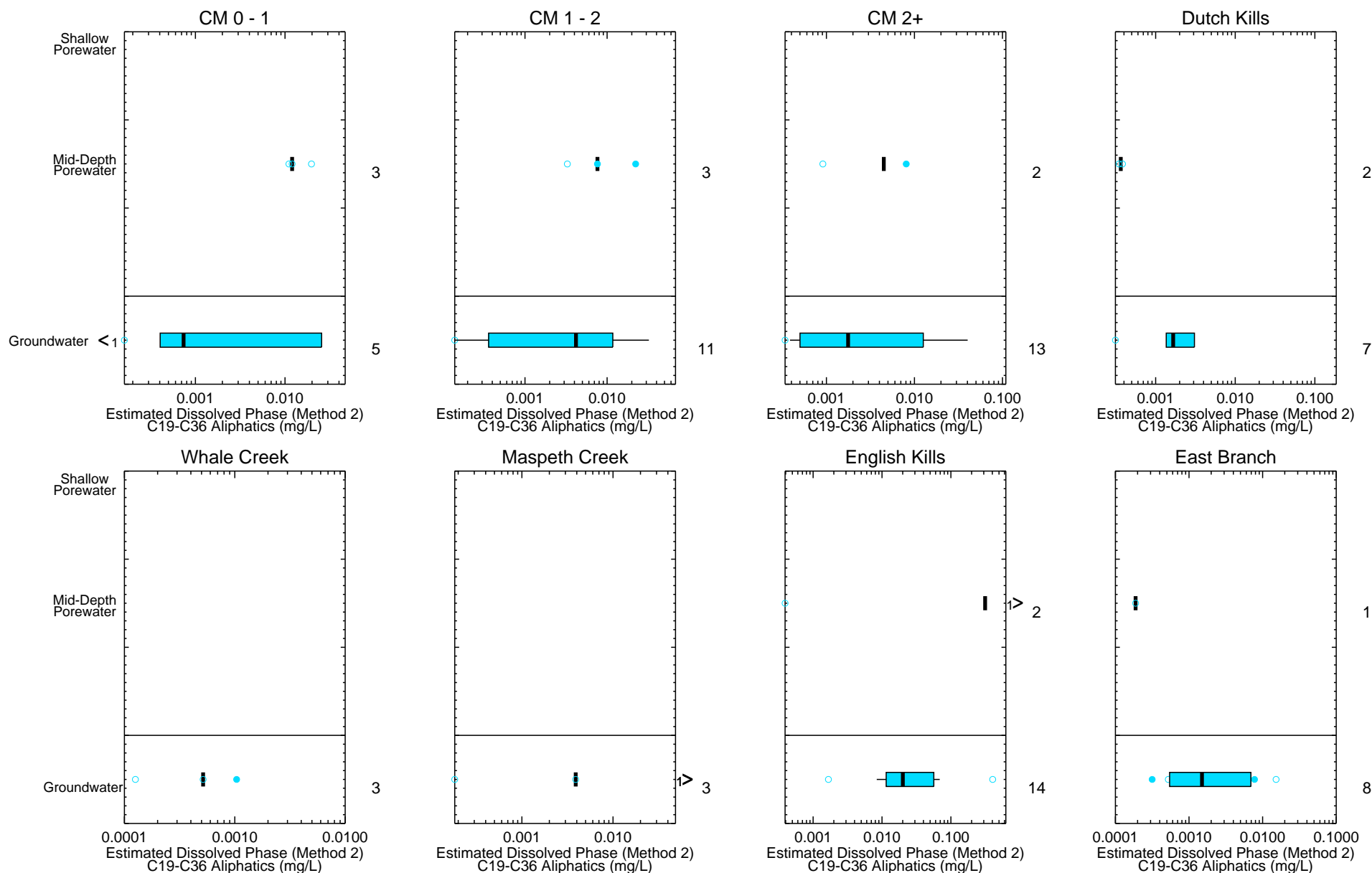
Figure 4-247 Estimated Dissolved Phase (Method 2) C19-C36 Aliphatics in Porewater and Groundwater - Box Plot Depth Profiles Remedial Investigation Report Newtown Creek RI/FS
