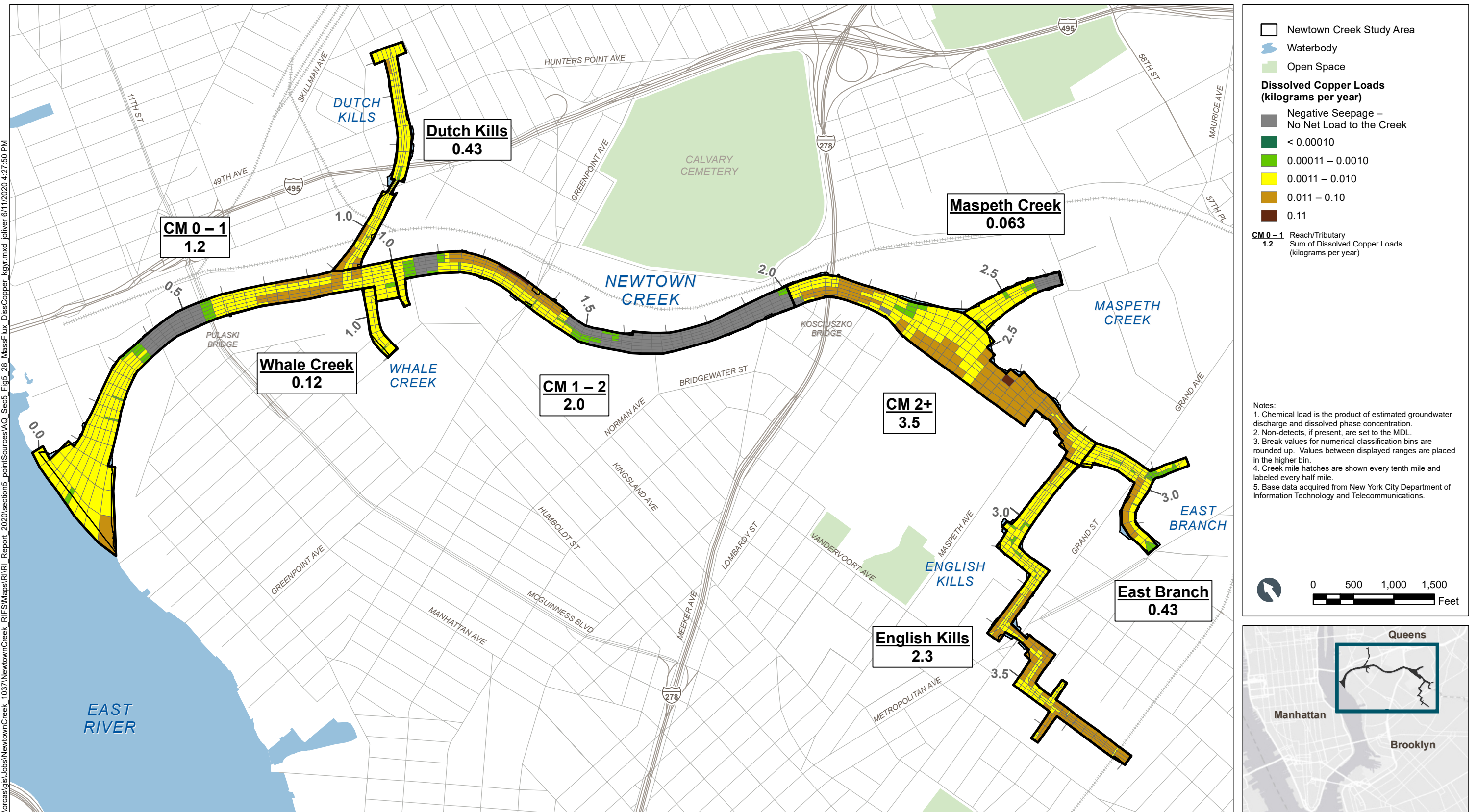
Figure 5-28 Dissolved Copper Loads to Subsurface Sediment from Groundwater Remedial Investigation Report Newtown Creek RI/FS
