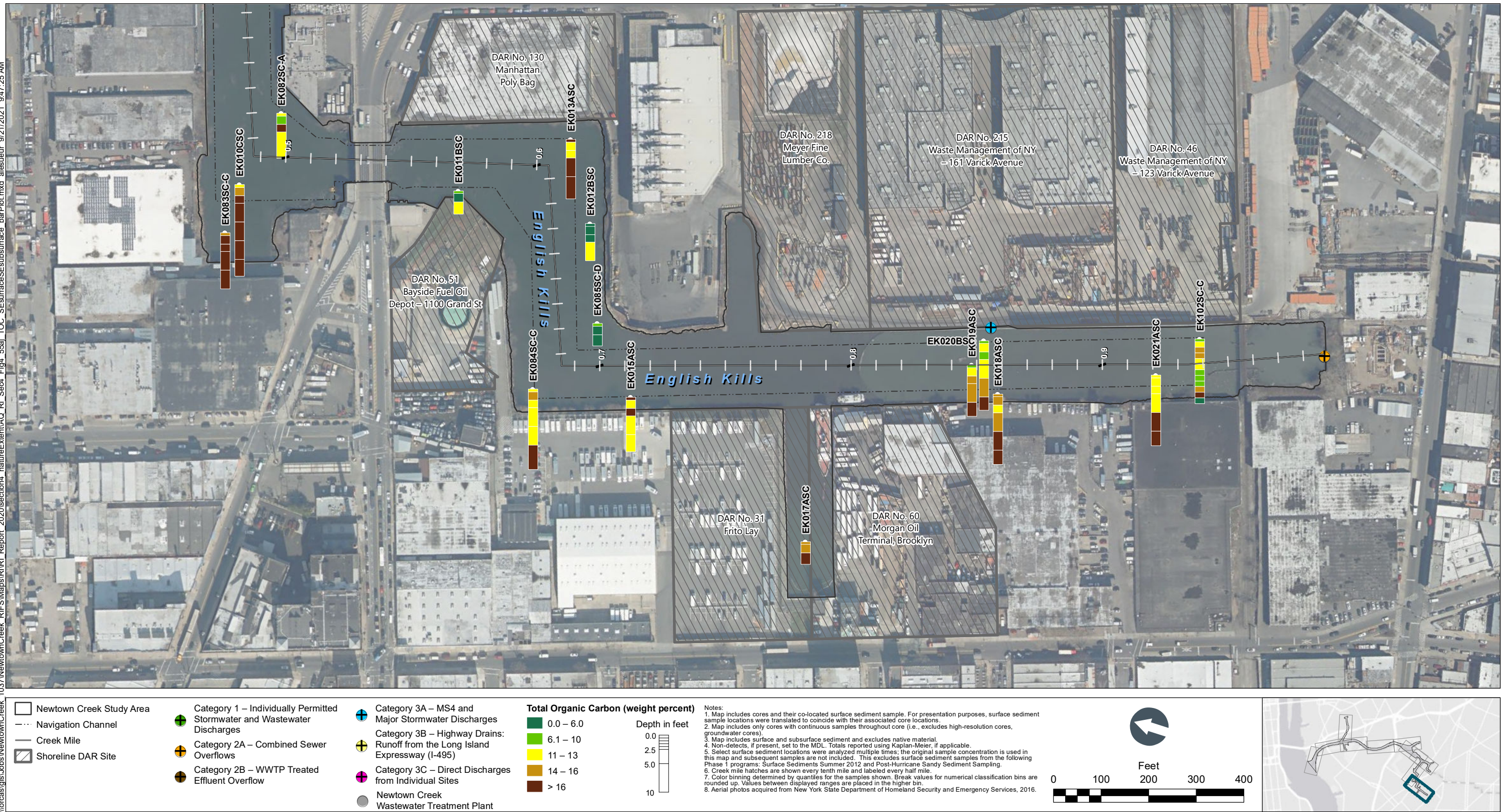
Figure 4-55j TOC in Surface and Subsurface Sediment Bar Plots by Depth – Plan View of English Kills CM 0.5 to 0.9 Remedial Investigation Report Newtown Creek RI/FS
