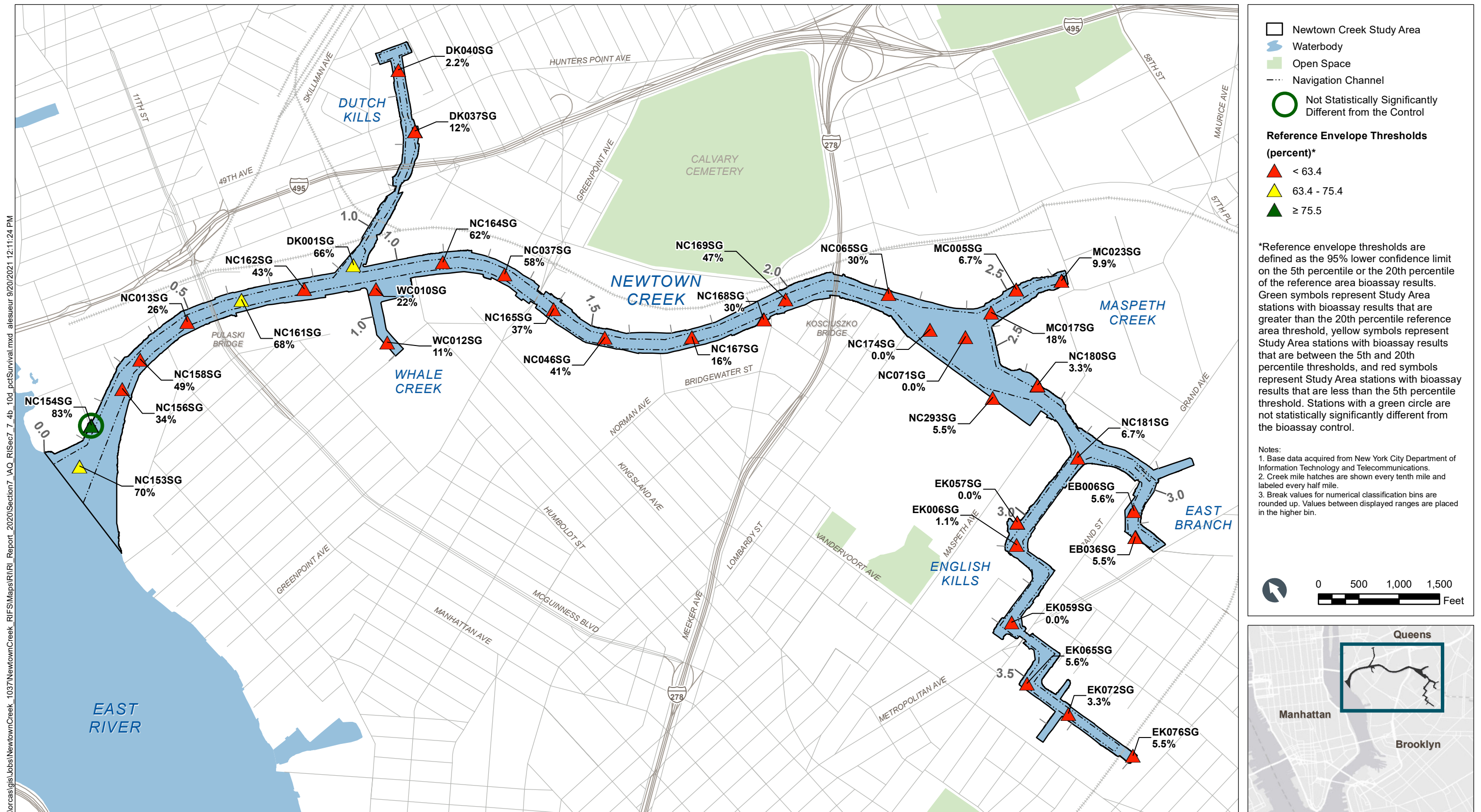
Figure 7-4b 10-Day Survival Reference Envelope (n = 48) Comparison by Study Area Creek Mile Remedial Investigation Report Newtown Creek RI/FS
