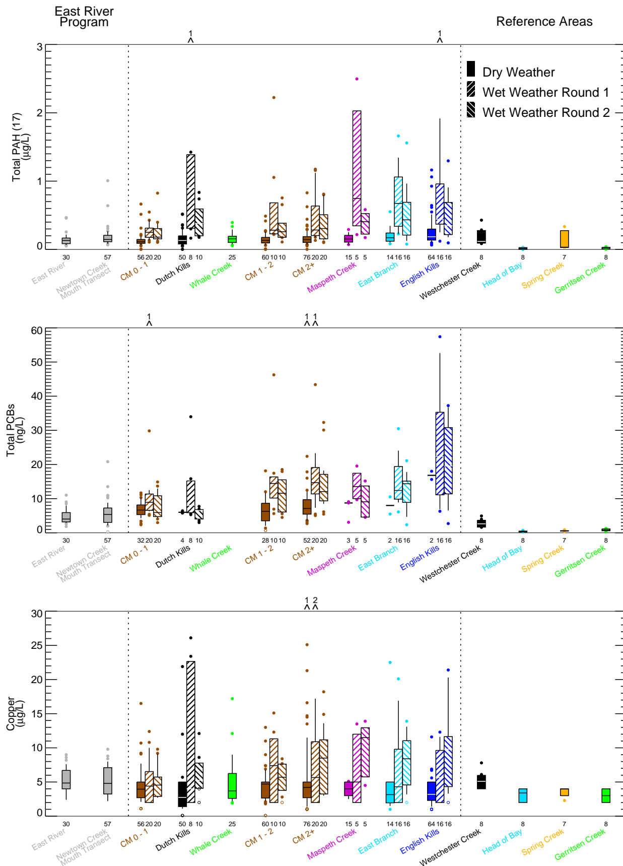
Figure 8-13 Surface Water Concentrations During Dry and Wet Weather Remedial Investigation Report Newtown Creek RI/FS
