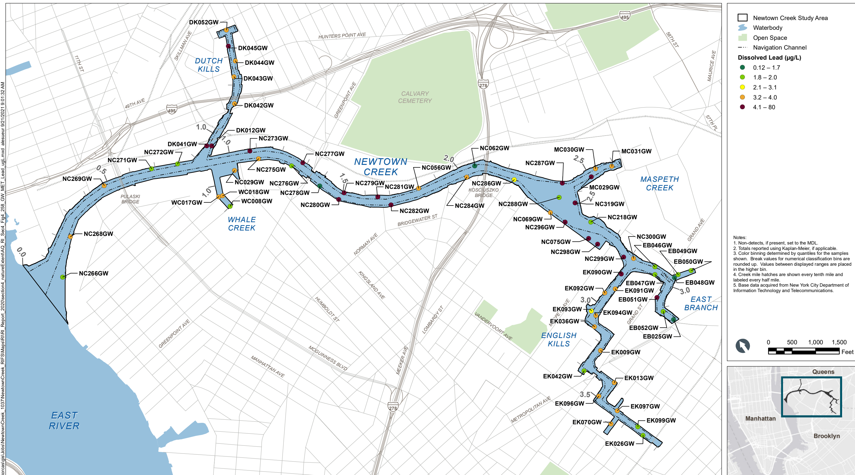
Figure 4-258 Dissolved Lead in Groundwater – Plan View Remedial Investigation Report Newtown Creek RI/FS
