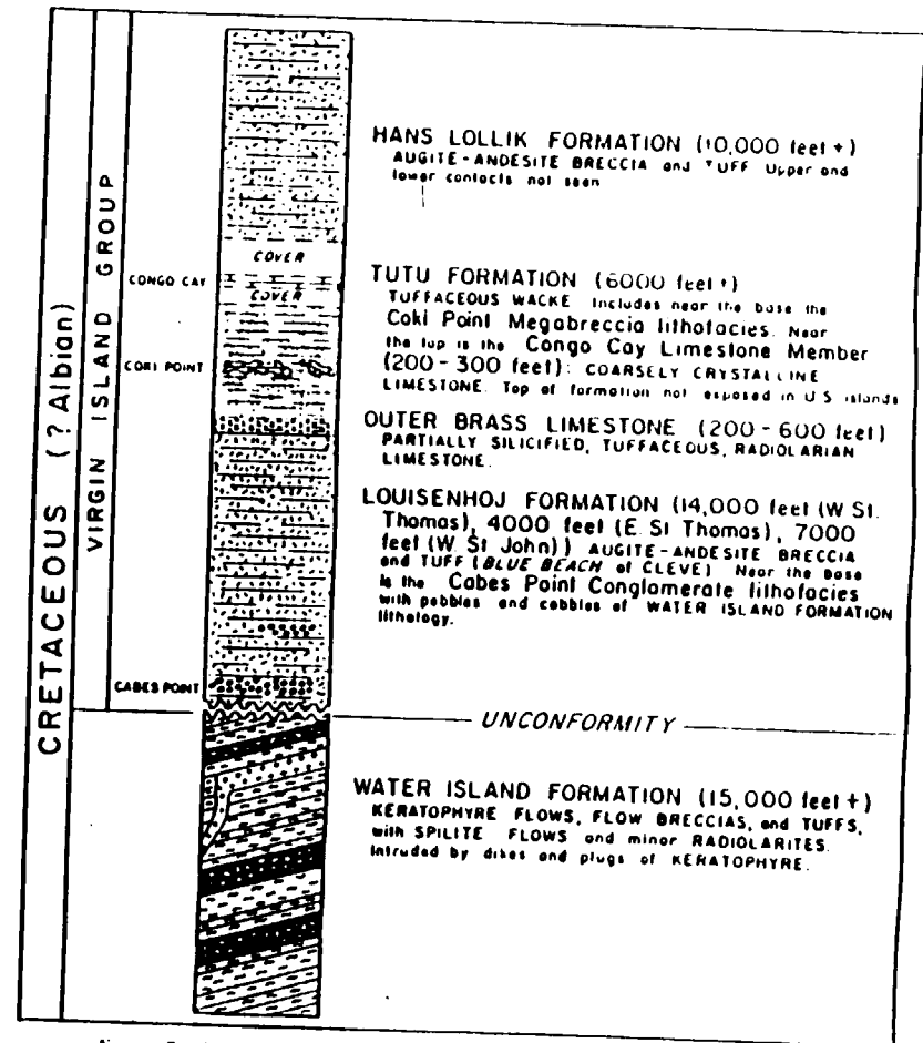
FIGURE 2. Stratigraphic section for St. Thomas and St. John, Virgin Islands.
