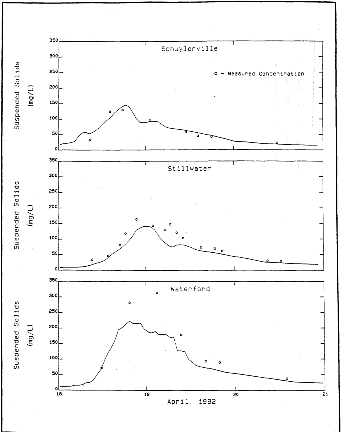
Figure 3-5. Model-Predicted and Observed TSS Concentrations at Schuylerville, Stillwater, and Waterford.
