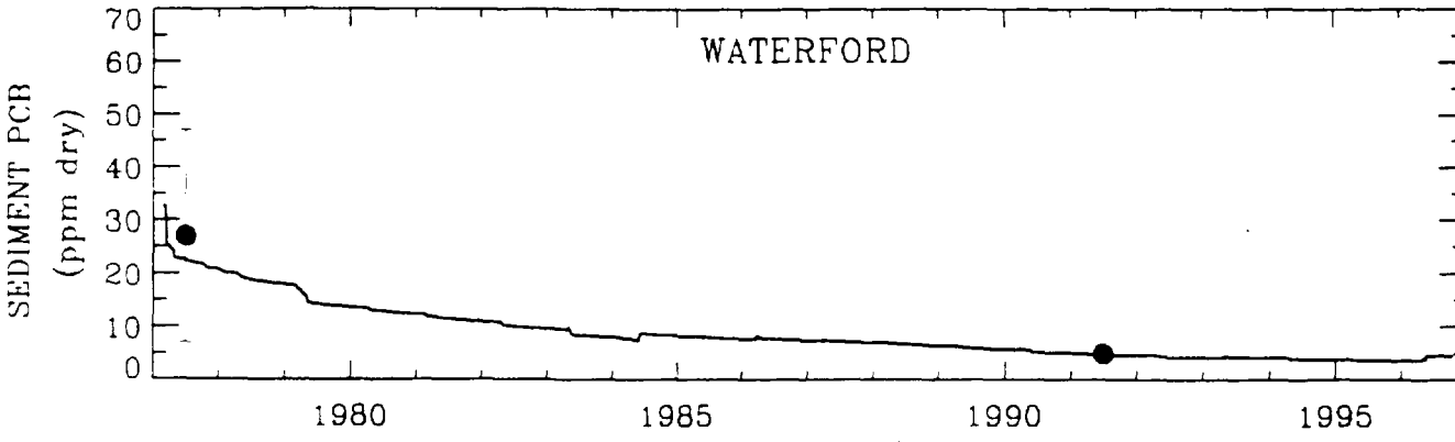
Figure 3-6. Comparison of Computed and Observed Surface (0-5 cm) Sediment PCB Levels in Four Areas of the Upper Hudson River.
