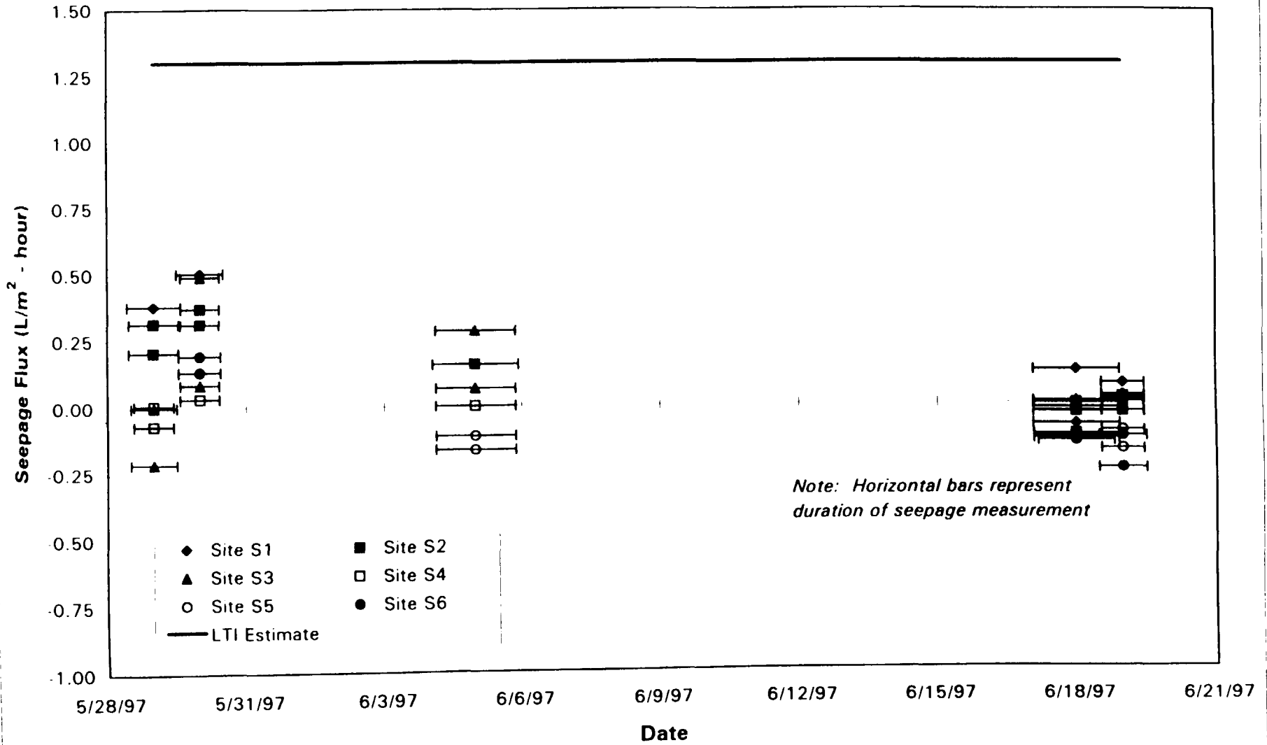
Figure 4-3. Temporal Trends in Measured Groundwater Seepage into Thompson Island Pool.
