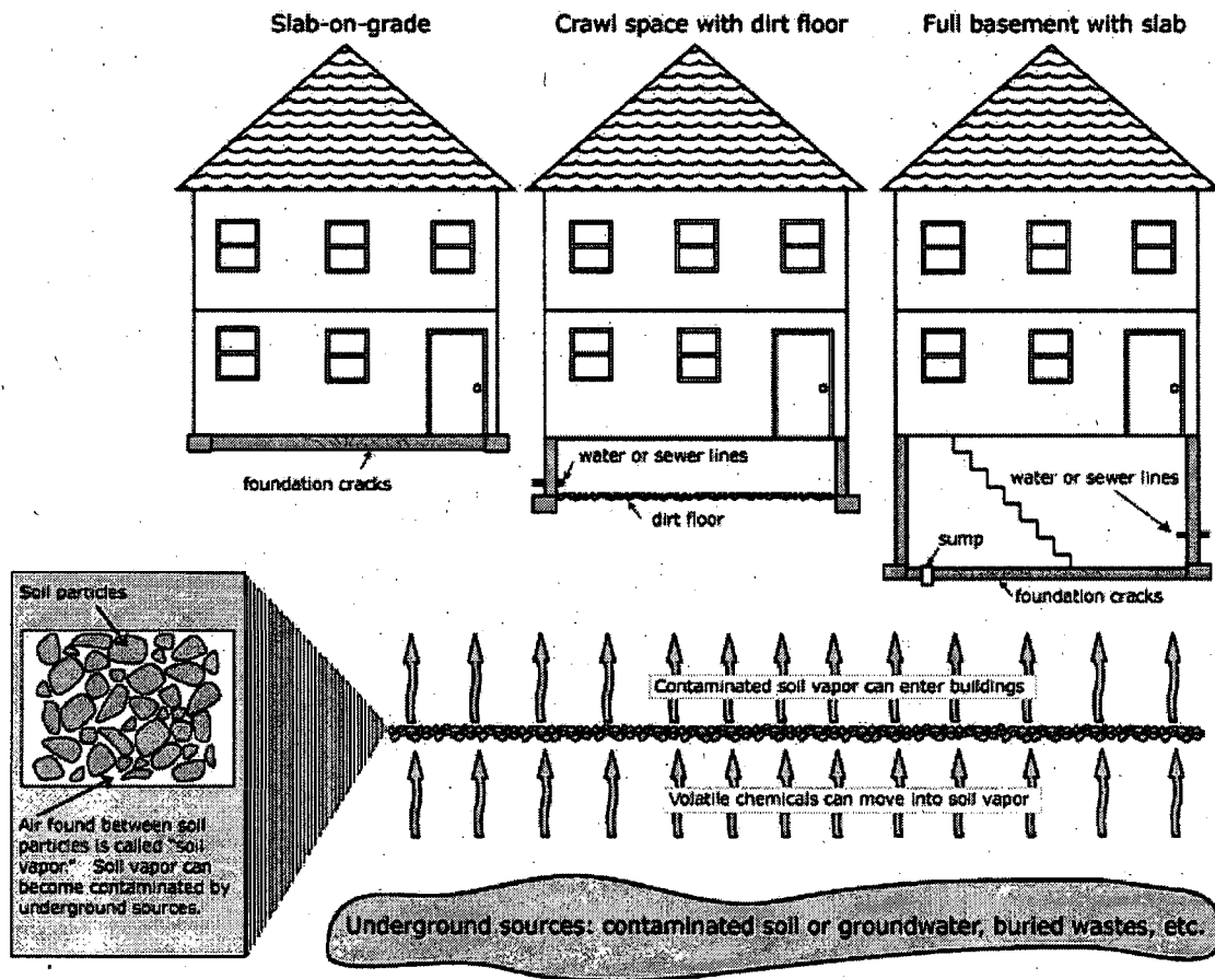
Figure 1.1 Generalized diagram of soil vapor intrusion
