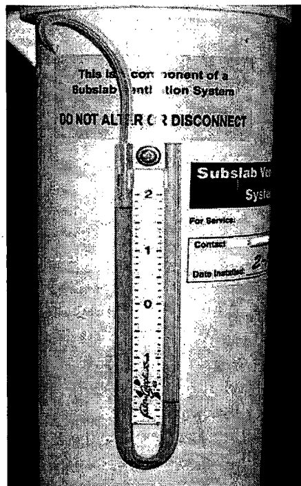
Figure 5.1 Manometer indicating the SSD system is operating properly.
