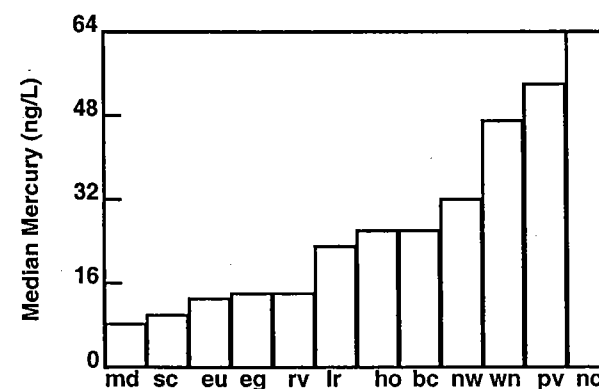
Figure 3-10b. Measured median STP effluent concentrations in New Jersey.
