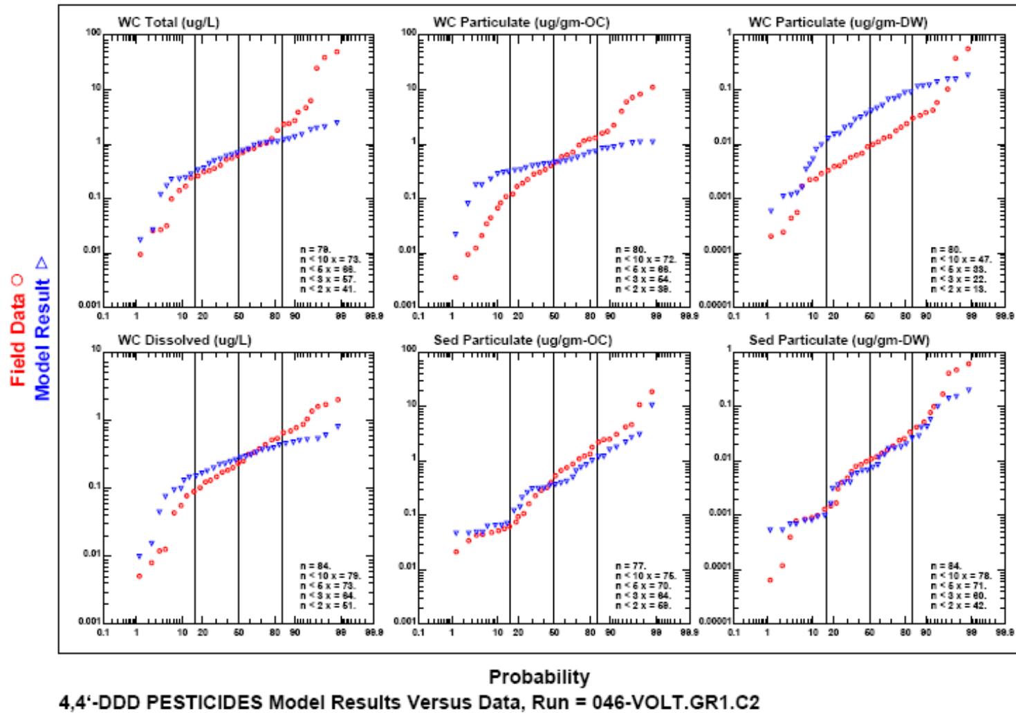
Figure 7-6. Example probability model and data comparisons for 4,4'-DDD
