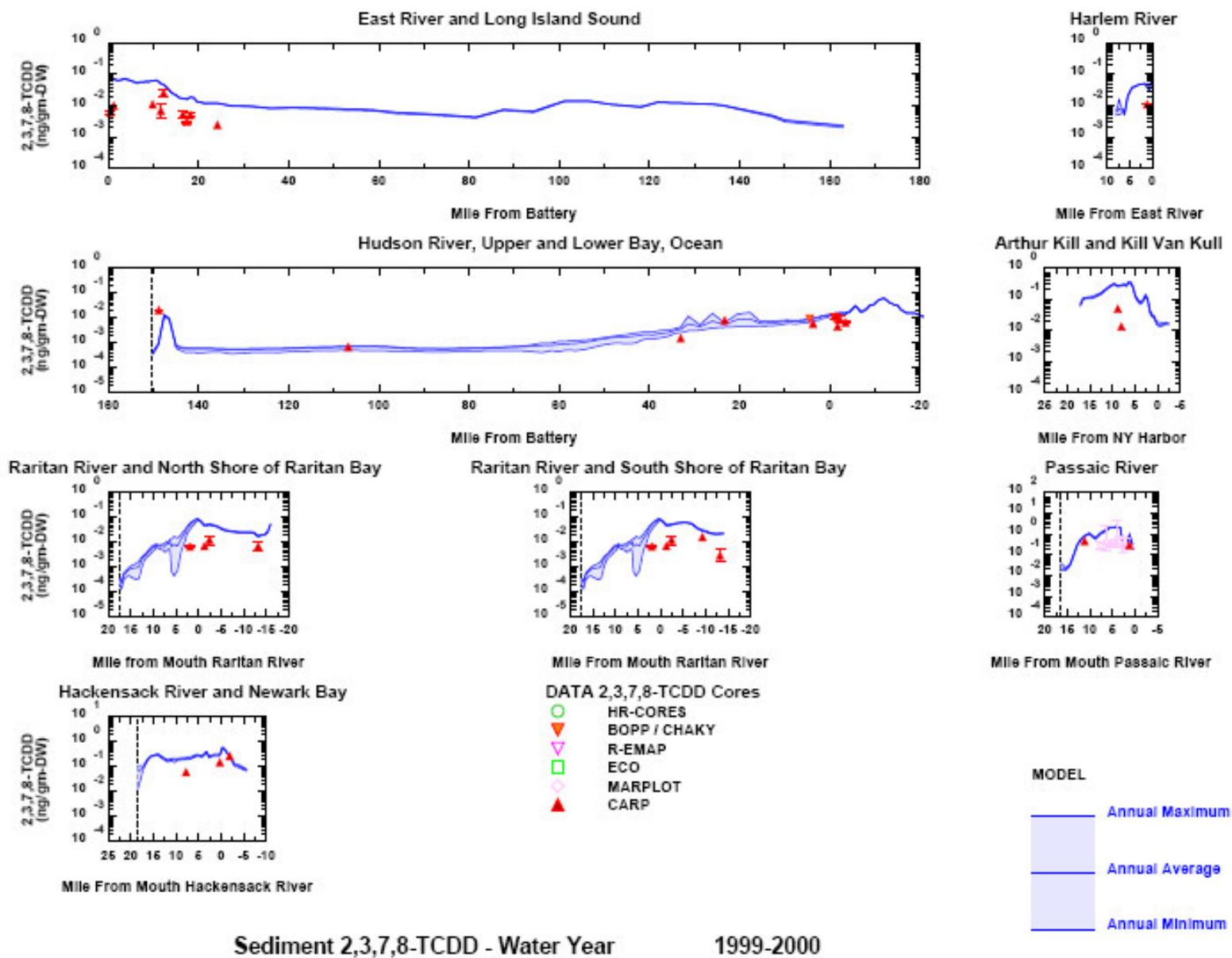
Figure 6-16. Example spatial transect model and data comparisons for CARP 2,3,7,8-TCDD hindcast – 1999-2000.
