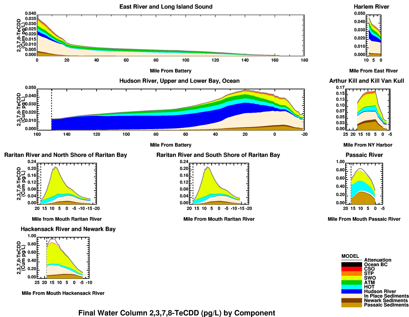
Figure 12-5. Example water column loading component responses along spatial transects for simulation years 29-32 for 2,3,7,8-TCDD.
