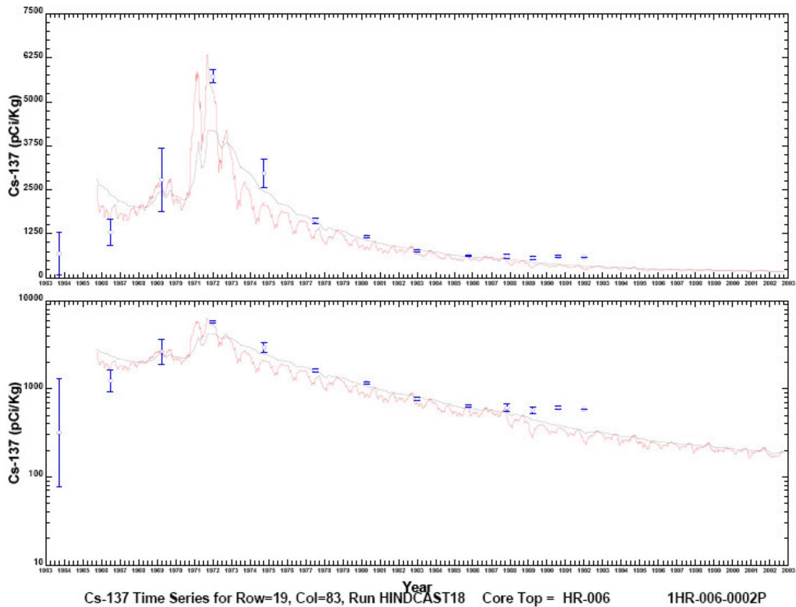
Figure 6-10. Example sediment chronology model and data comparisons for core HR-006.
