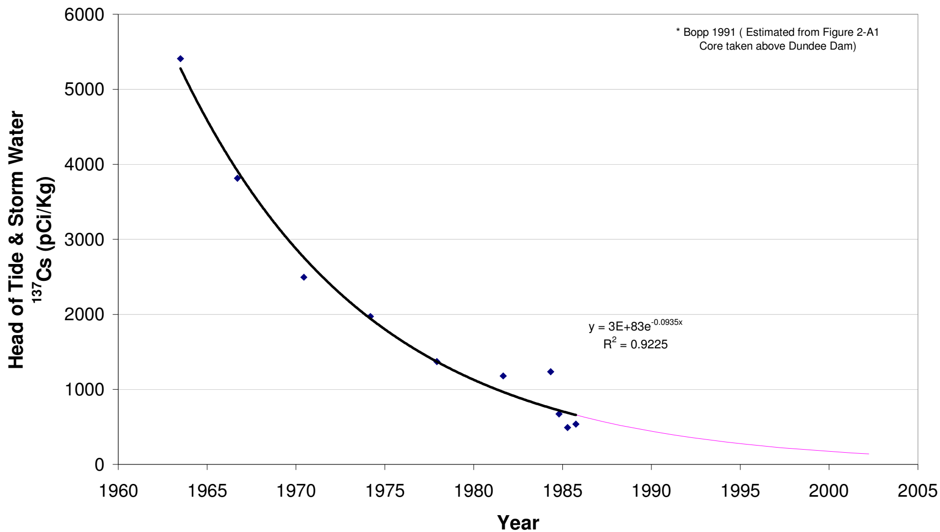
Figure 6-5. Time trend, inferred from dated sediment core data, of head of tide and storm water ^{137}\text{Cs} inputs used in CARP model hindcast simulations.
