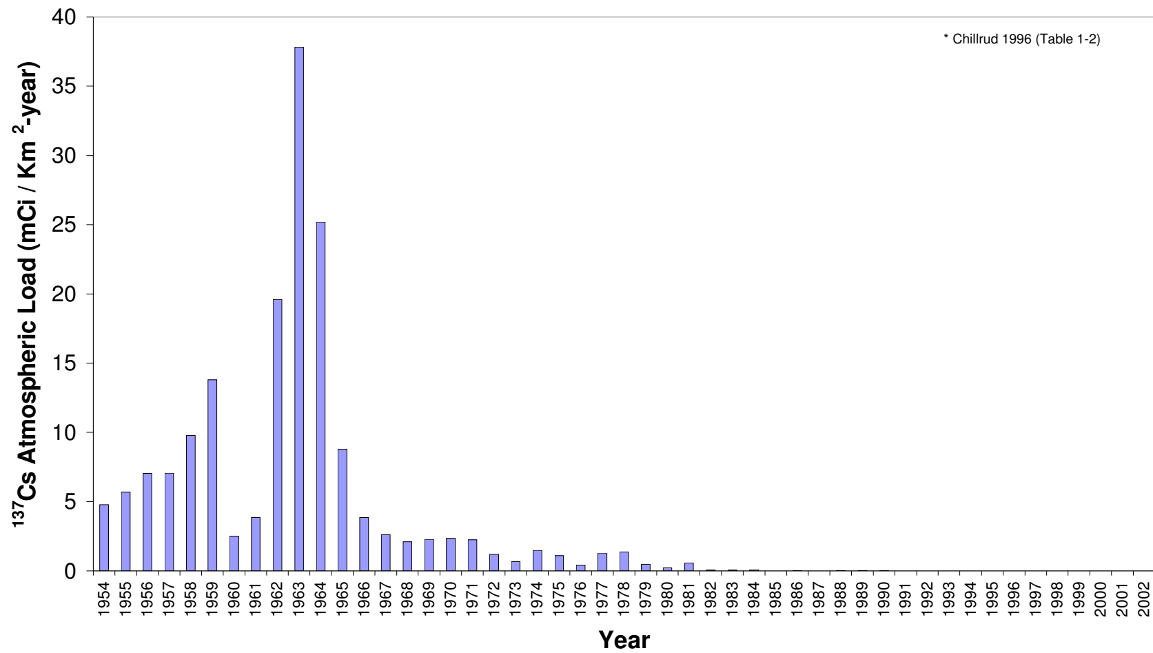
Figure 6-3. Annual release of ^{137}\text{Cs} from atmospheric deposition as reported by Chillrud 1996.
