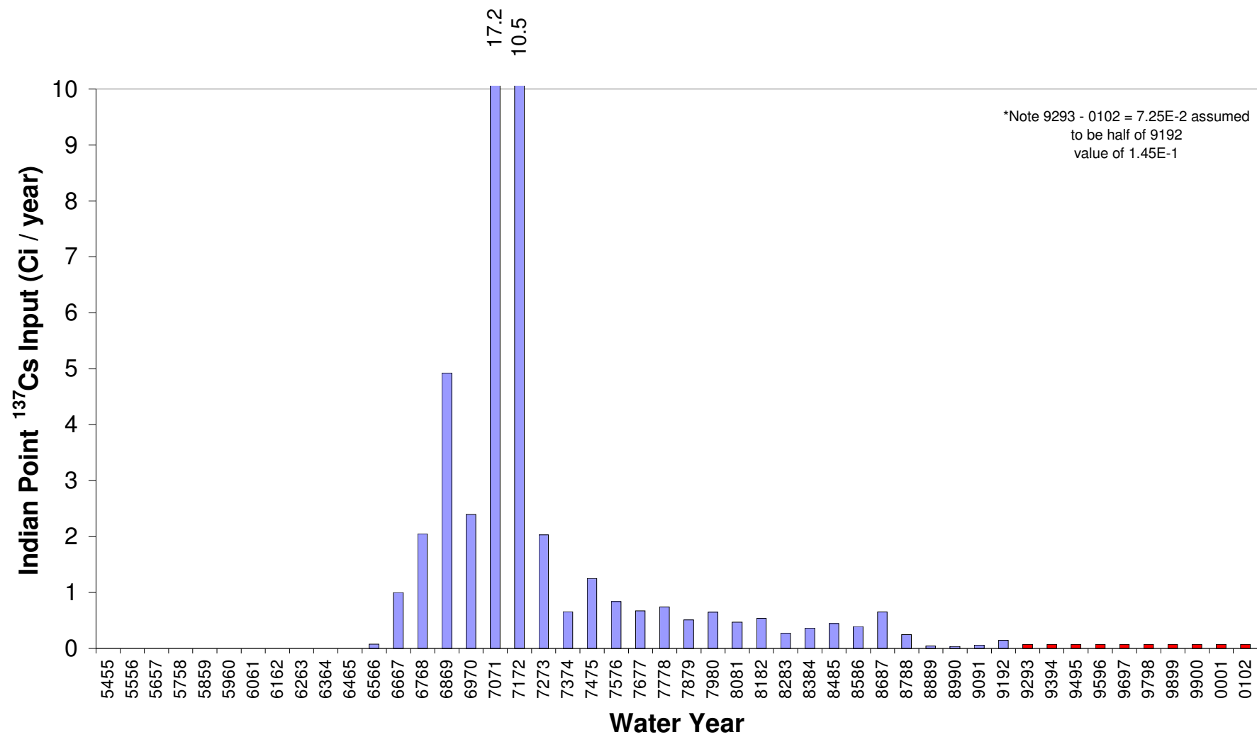
Figure 6-2. Indian Point release of ^{137}\text{Cs} per water year applied in CARP model hindcast simulations.
