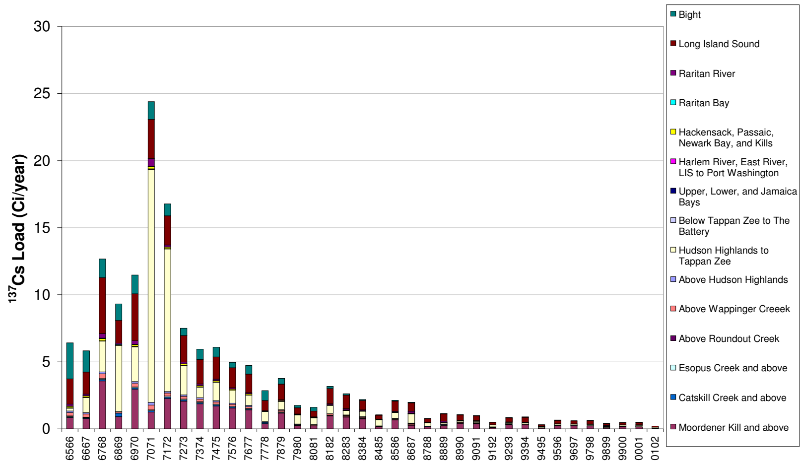
Figure 6-7. All CARP model hindcast simulation loads for ^{137}\text{Cs} by source location.
