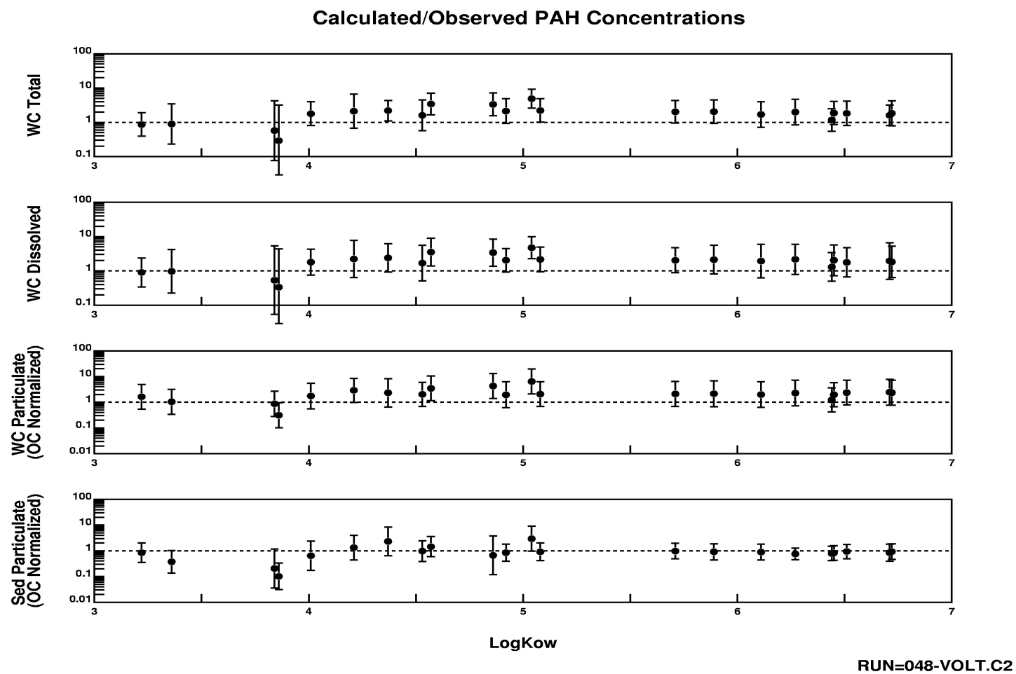
Figure 7-4. Calibration summary for 22 PAH compounds.
