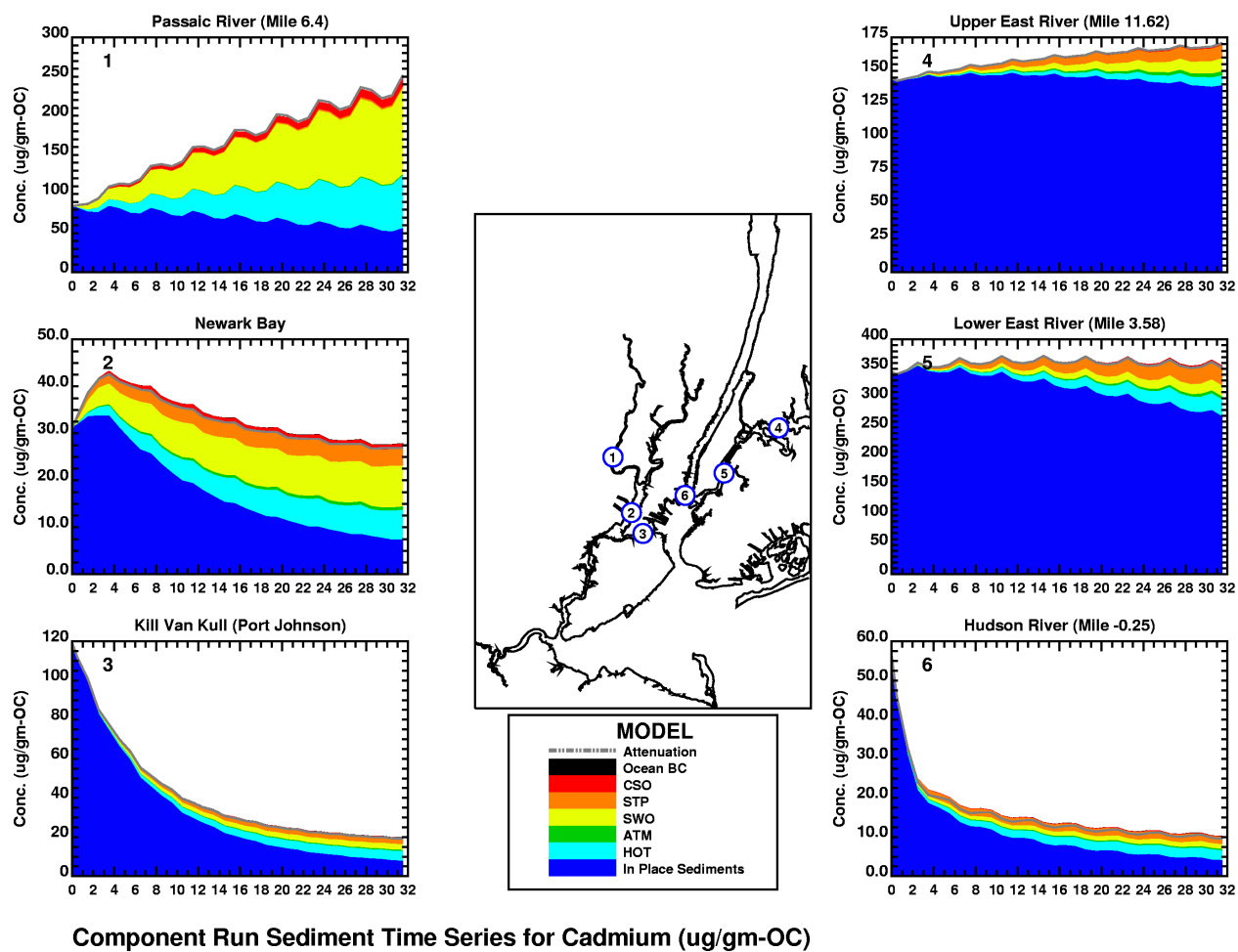
Figure 12-4. Time series component results for sediments at six selected locations - Cadmium Example.
