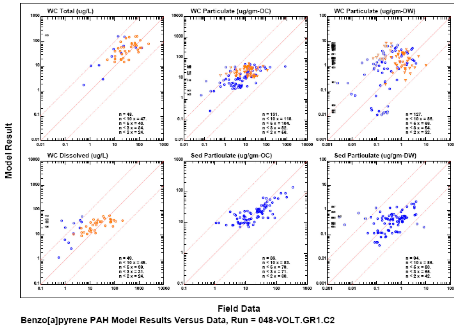
Figure 7-1. Example X-Y model and data comparison plots for benzo[a]pyrene
