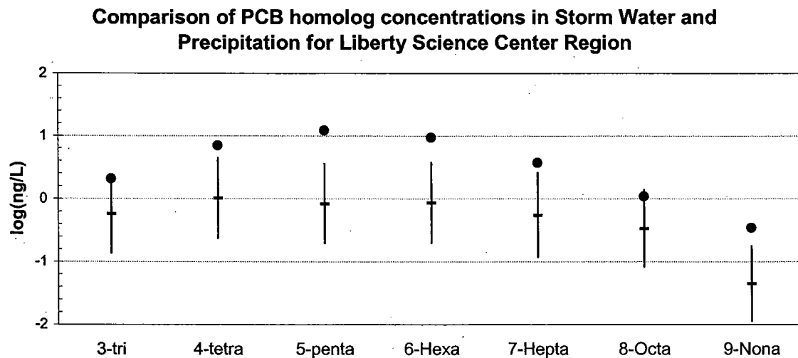
Figure 3-14. Comparison between PCB concentrations measured in precipitation and stormwater runoff.
