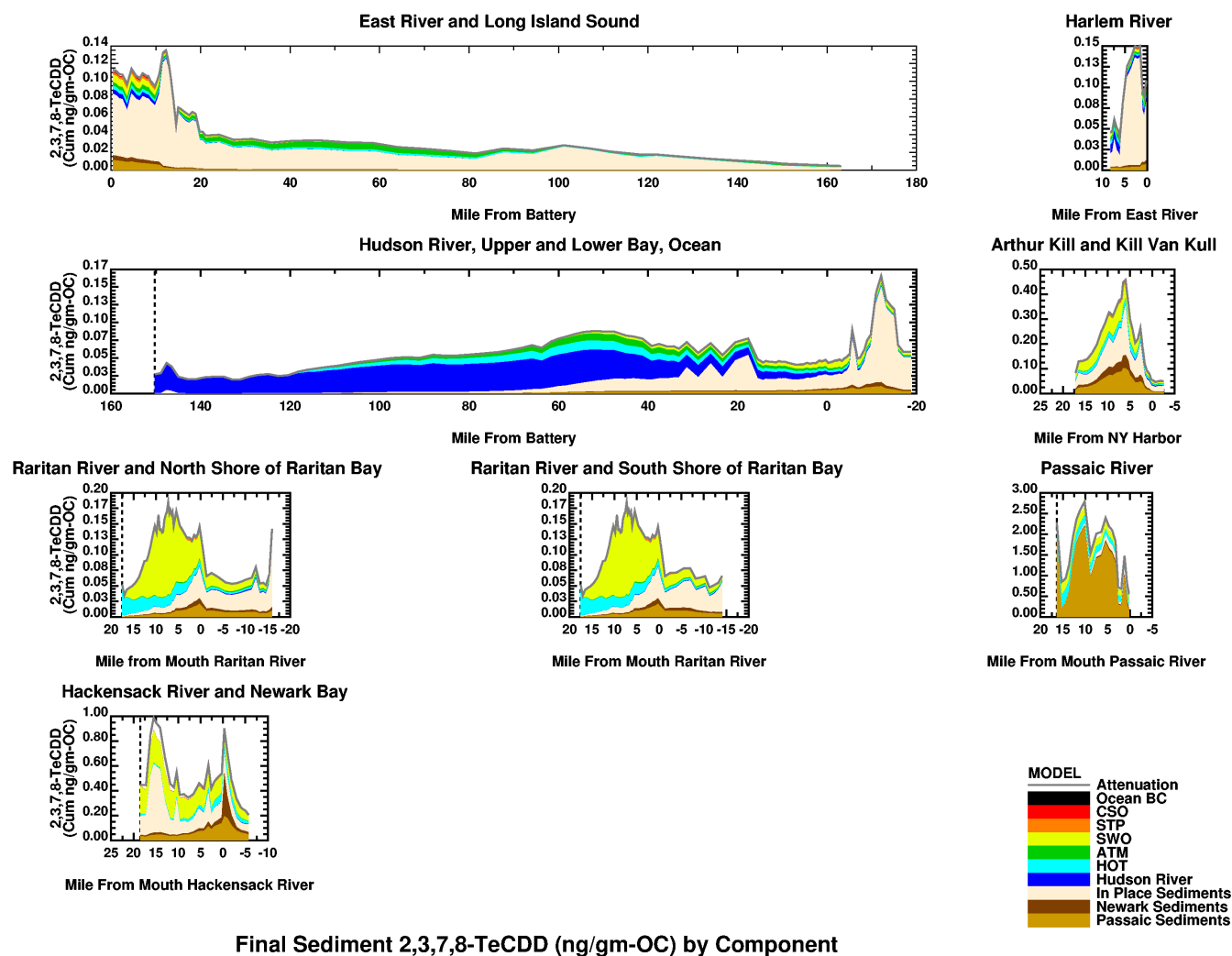
Figure 12-6. Example sediment bed loading component responses along spatial transects for simulation years 29-32 for 2,3,7,8-TCDD.
