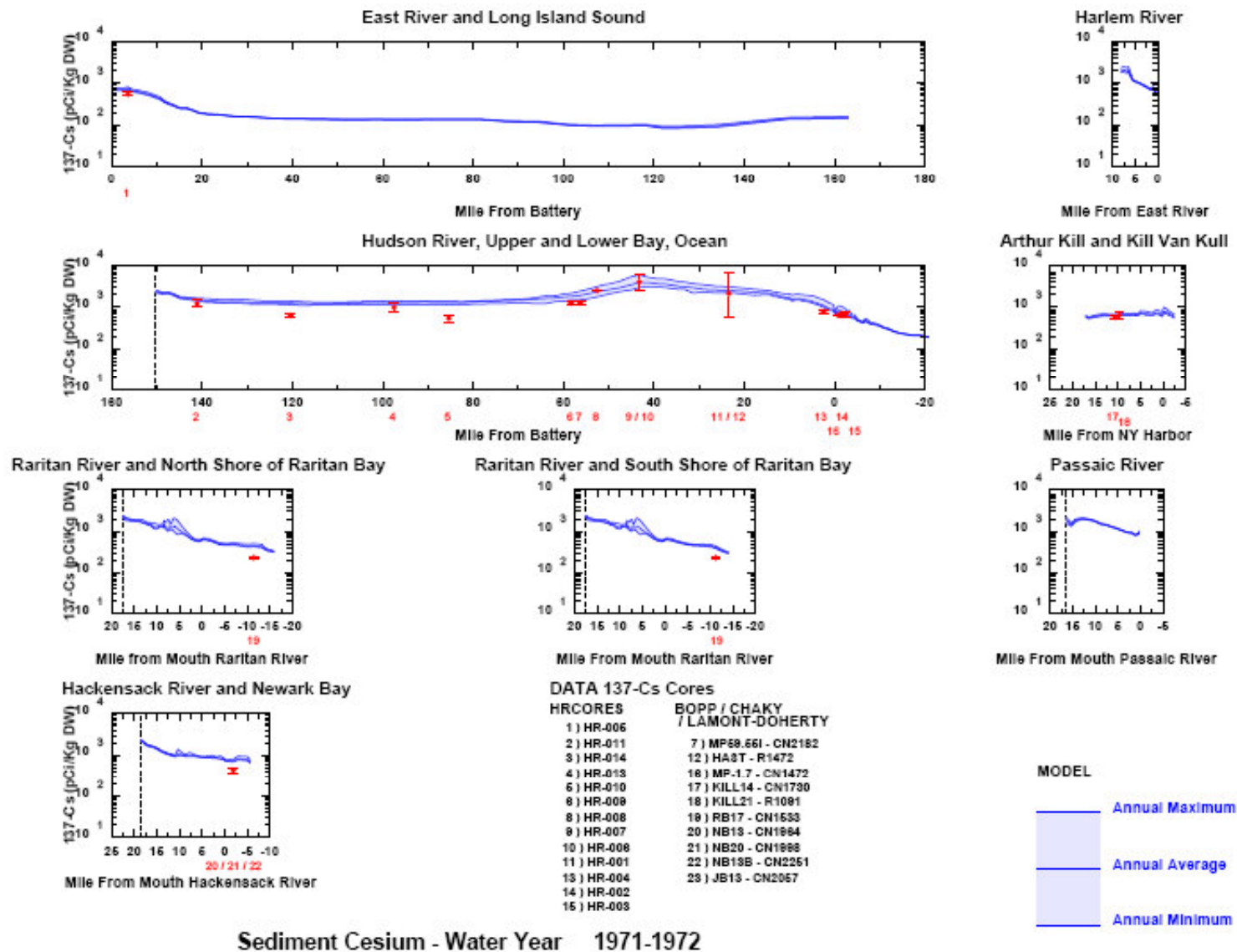
Figure 6-8. Example sediment spatial transect model and data comparisons for CARP ^{137}\text{Cs} hindcast – 1971-72.
