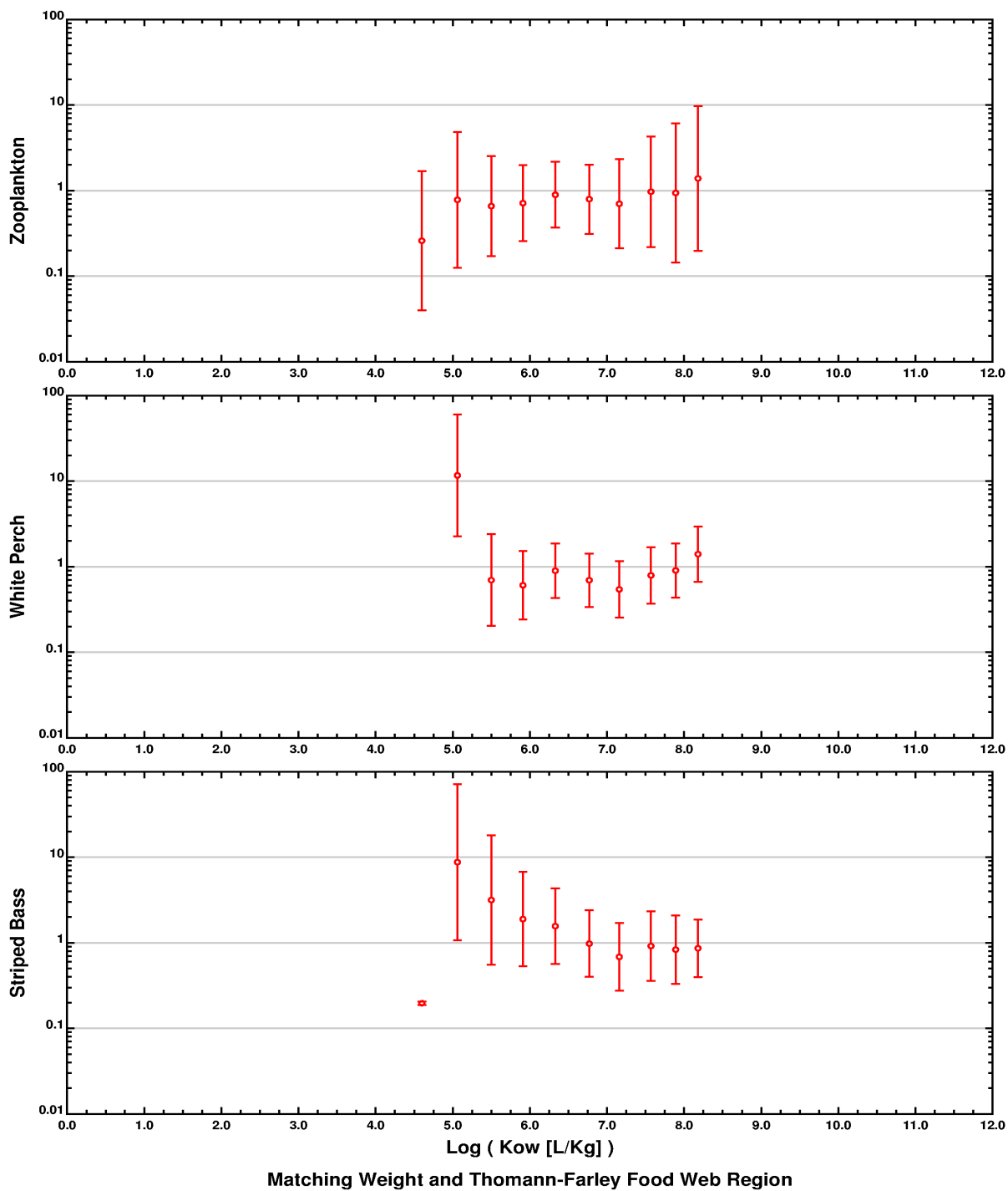
Figure 11-1. Summary comparison between field observed and model calculated PCB concentrations in organisms - base case
