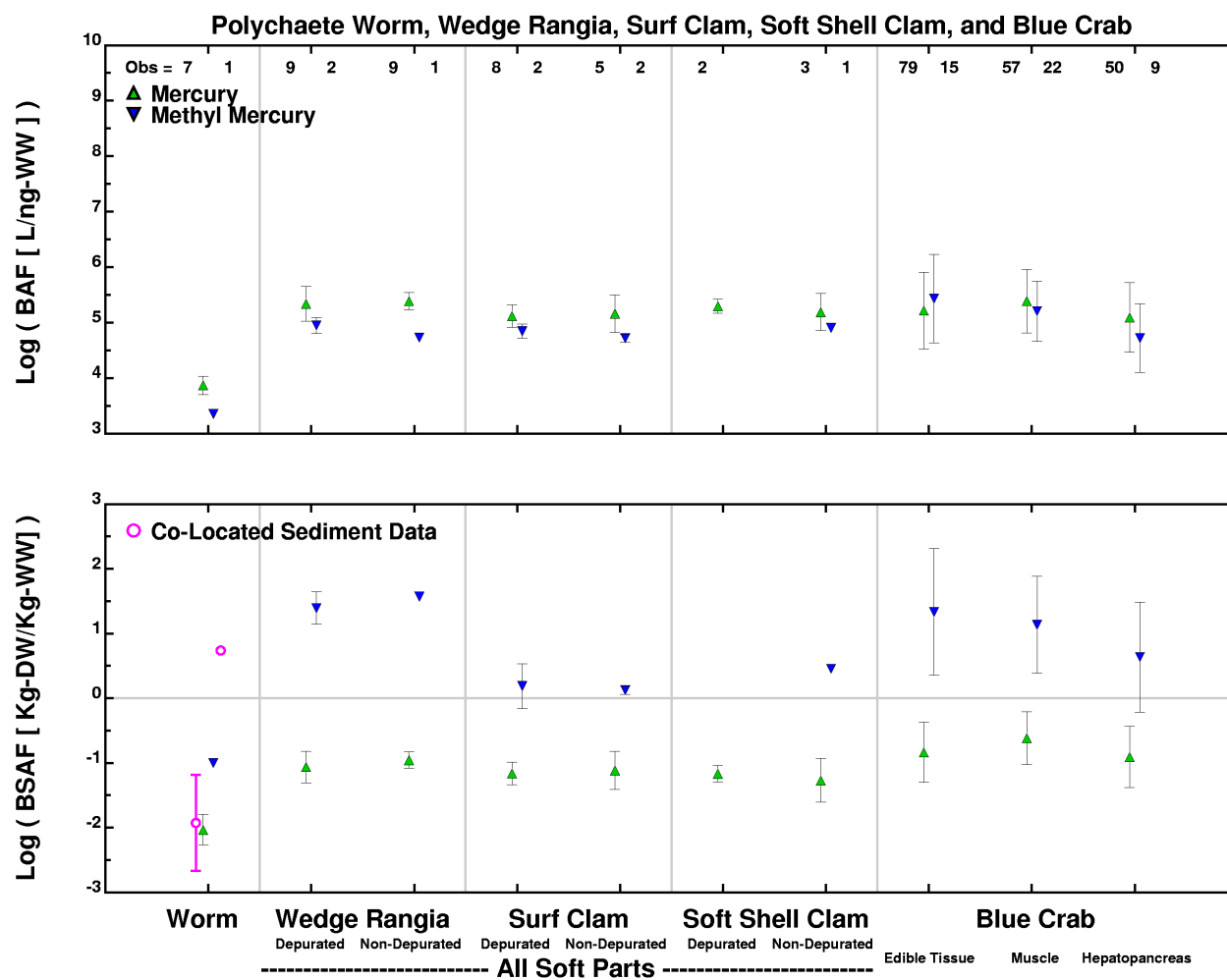
Mercury Bioaccumulation in Benthic Species Derived from Measured Body Burden and Model Calculated Dissolved and Sediment Concentrations
