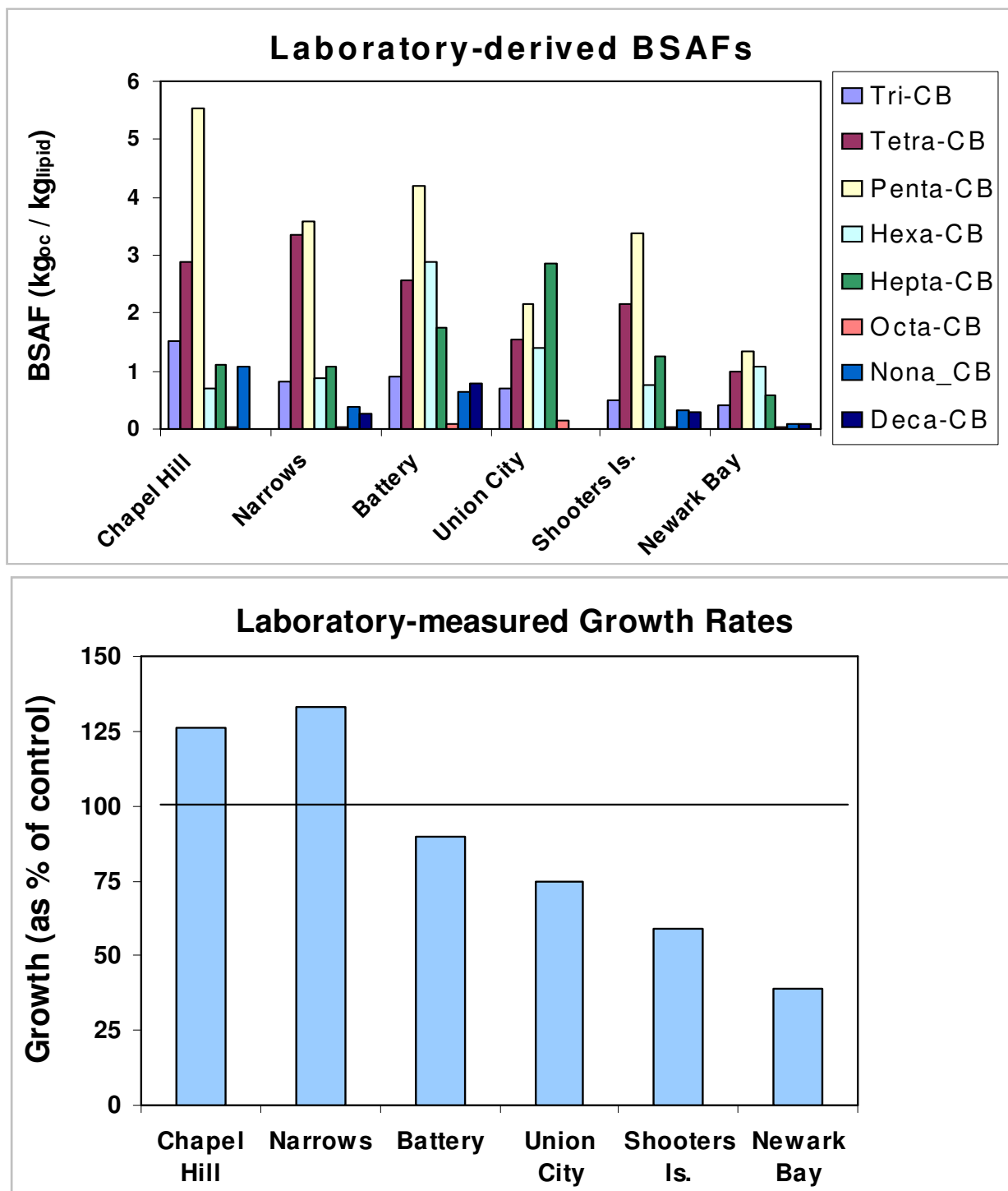
Figure 11-11. Laboratory derived BSAFs (top) and growth rates for Armandia . Based on bioaccumulation studies (Meador et al., 1997) and effects testing (Rice et al., 1995).
