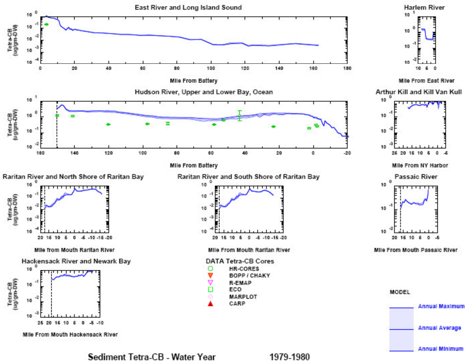
Figure 6-28. Example tetra-CB hindcast model and data comparisons along spatial transects – 1979-80.
