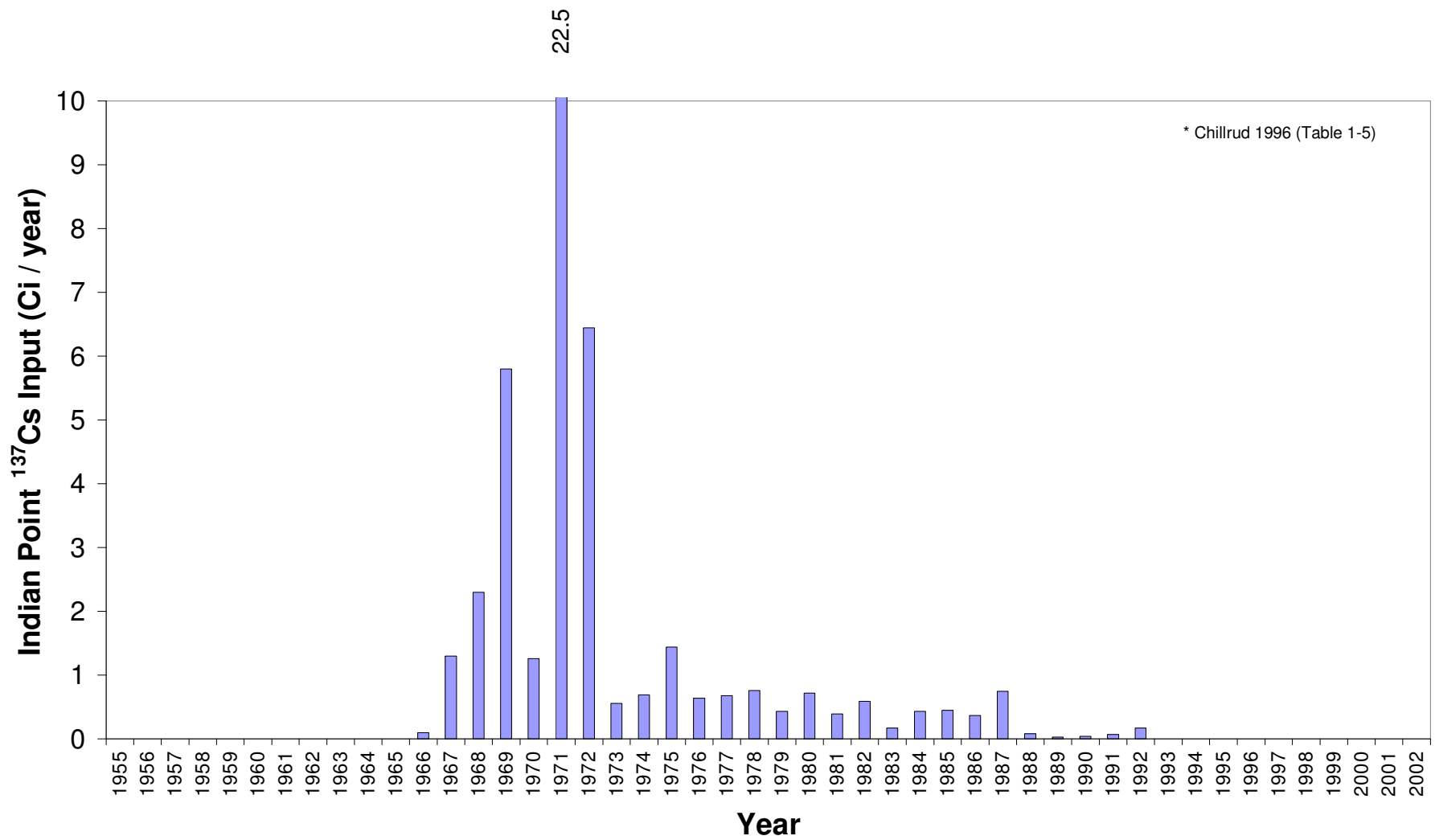
Figure 6-1. Annual releases of ^{137}\text{Cs} from Indian Point as reported by Chillrud 1996.
