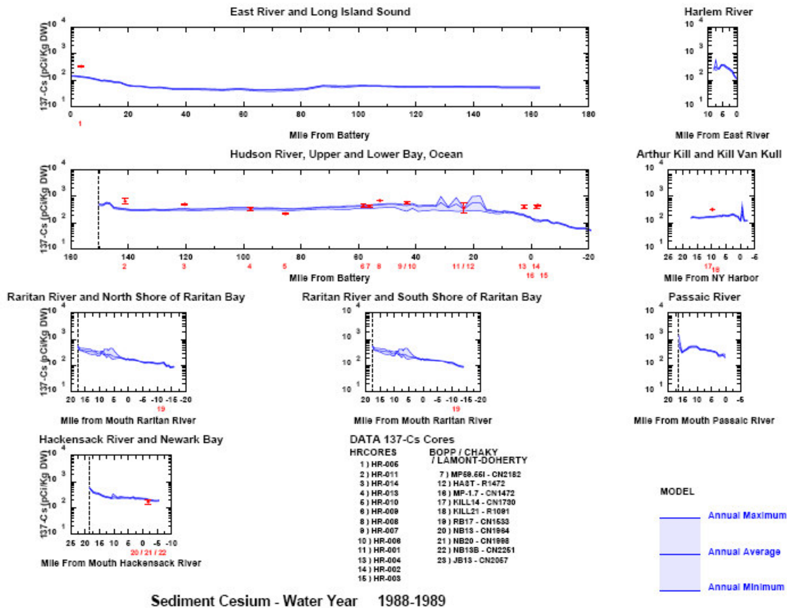
Figure 6-9. Example sediment spatial transect model and data comparisons for CARP ^{137}\text{Cs} hindcast – 1988-89.
