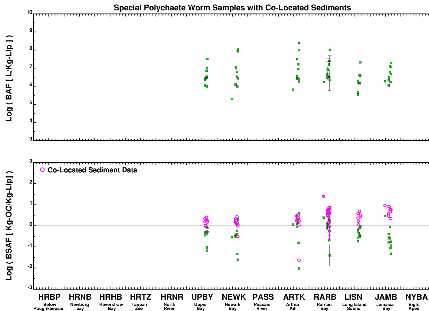
Pesticide Bioaccumulation in Worms Derived from Measured Worm and Model Calculated Dissolved and Sediment Concentrations
