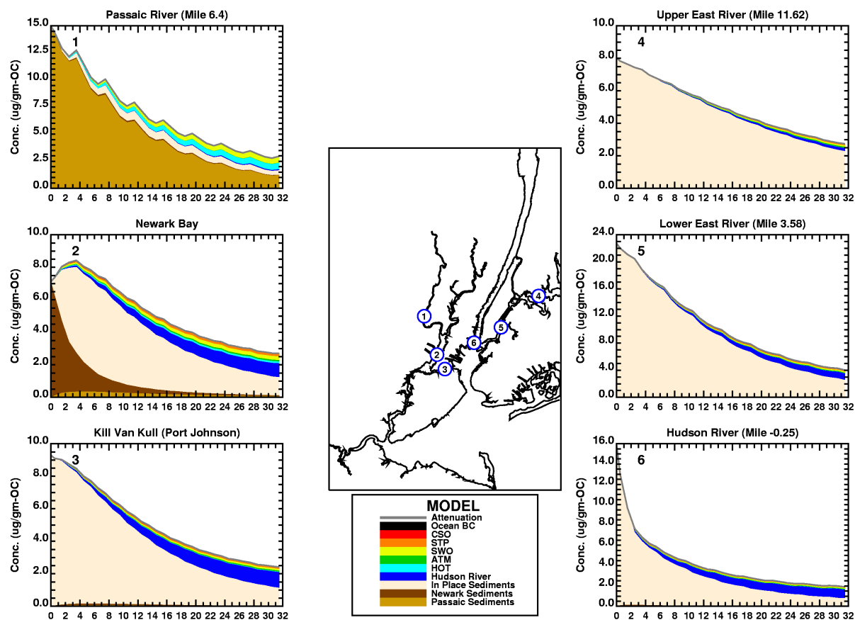
Component Run Sediment Time Series for Tetra-CB PCB (ug/gm-OC)
