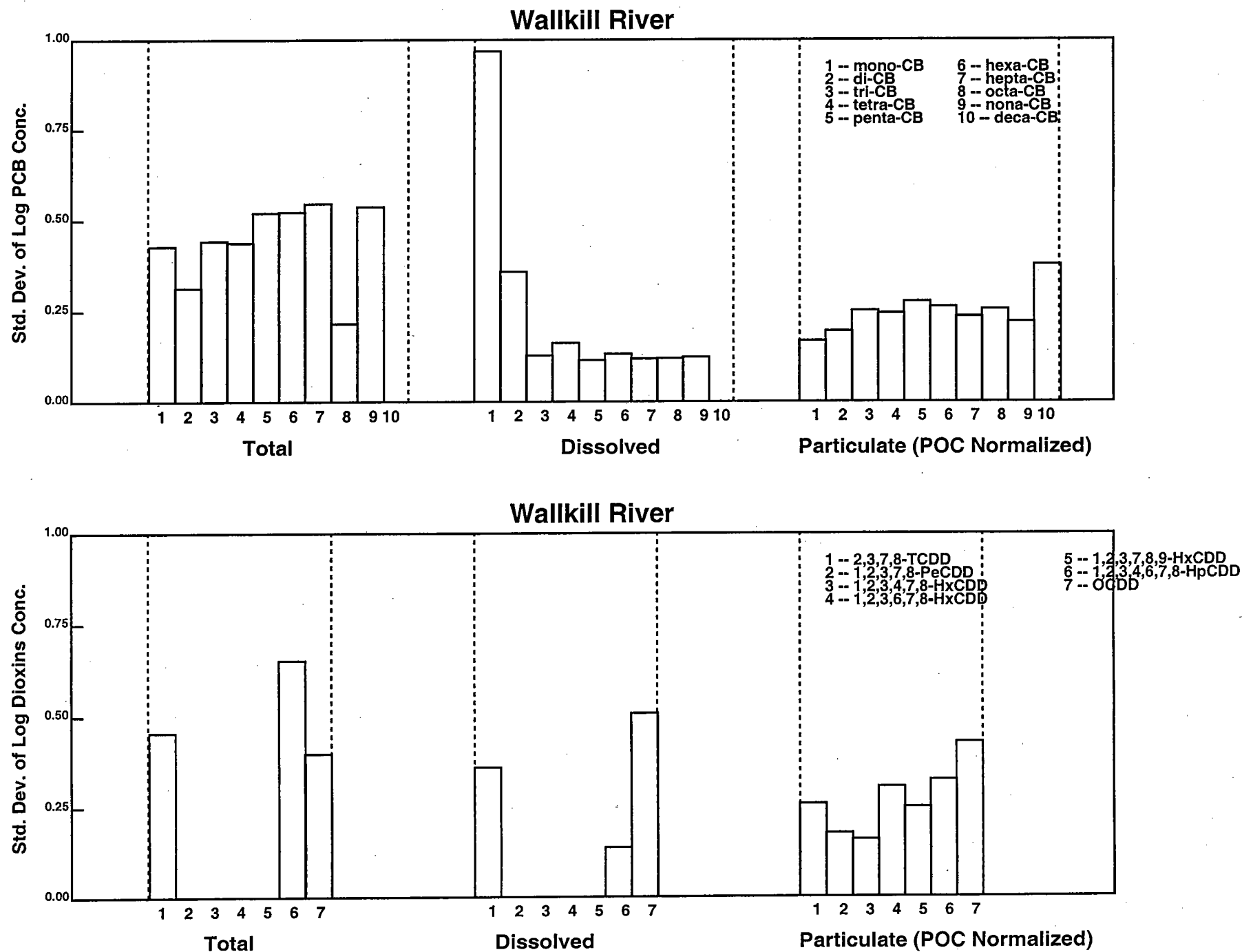
Figure 3-3a. Comparisons of standard deviations across same tributary measurements for various fractions for PCB homologs and dioxin congeners.
