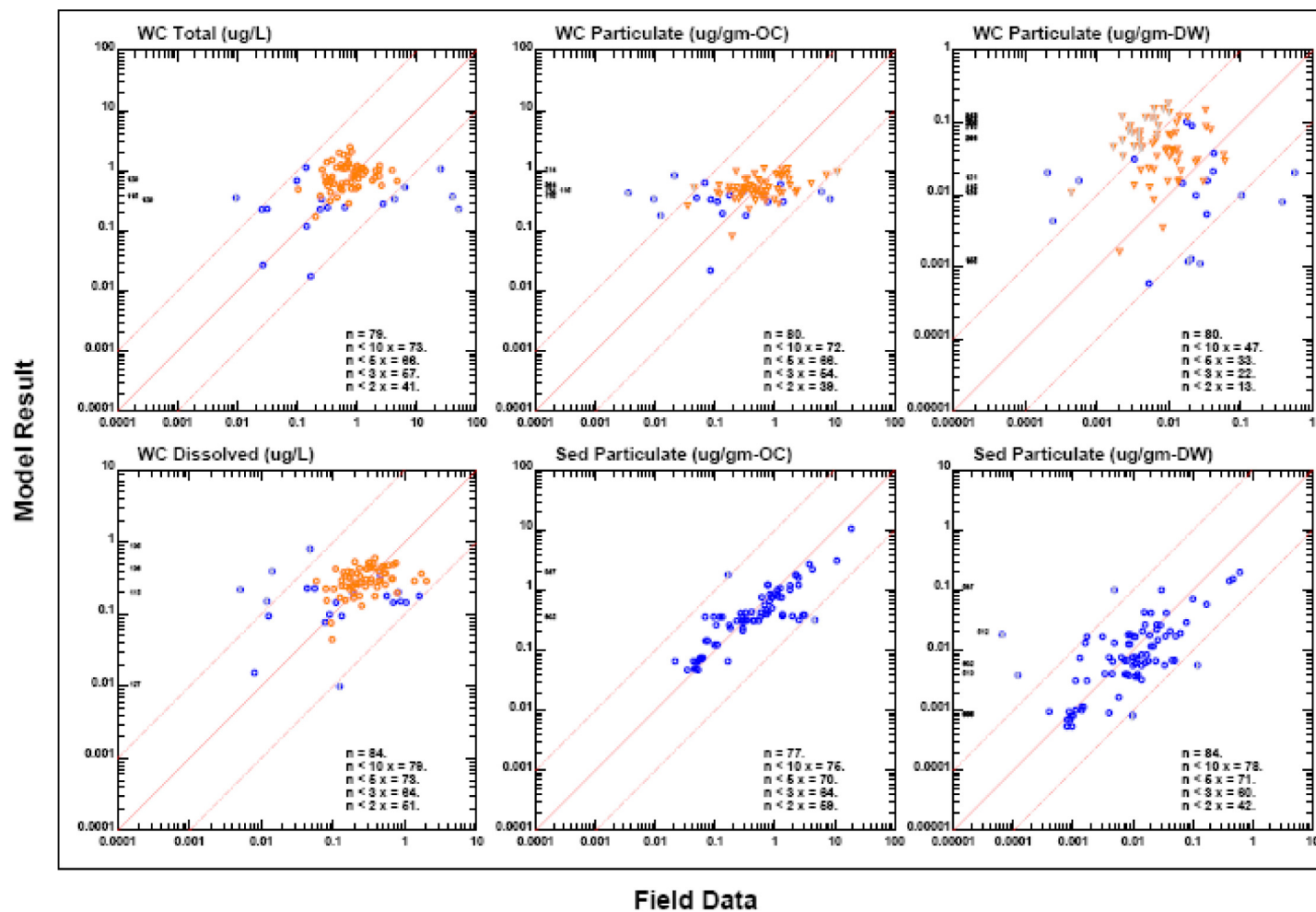
4,4'-DDD PESTICIDES Model Results Versus Data, Run = 046-VOLT.GR1.C2
