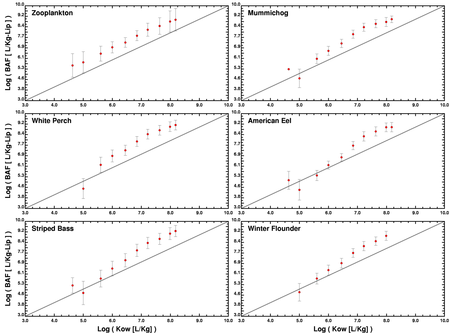
PCB BAFs Derived From Measured Fish and Model Dissolved Concentrations
