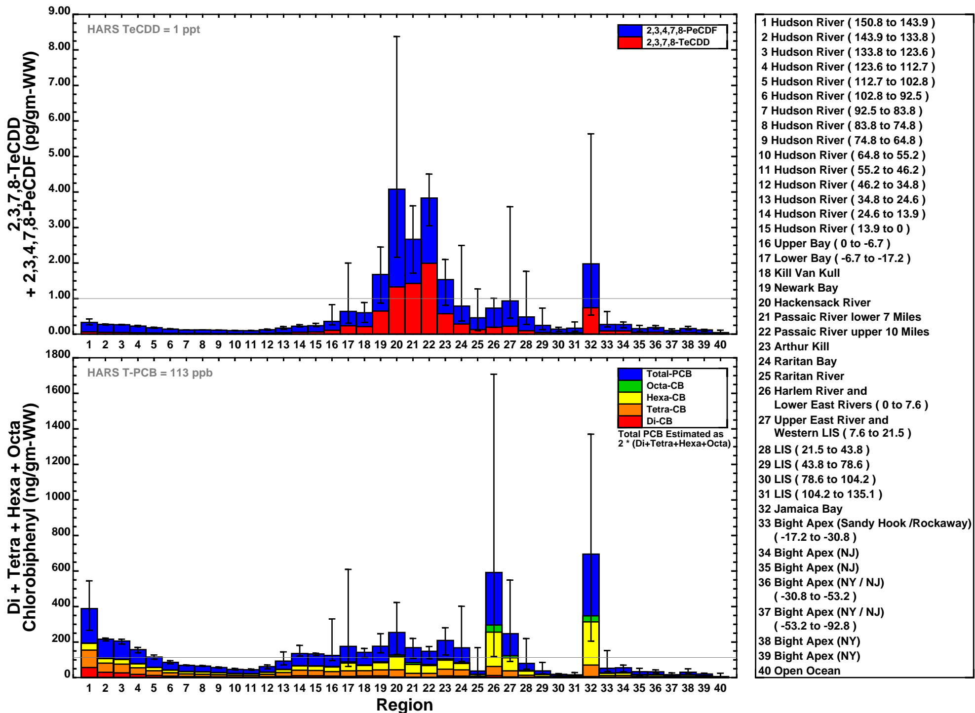
Future with Current Loads Projection, Year 37 Polychaete Worm Concentration Calculated Using CARP Data BSAFs
