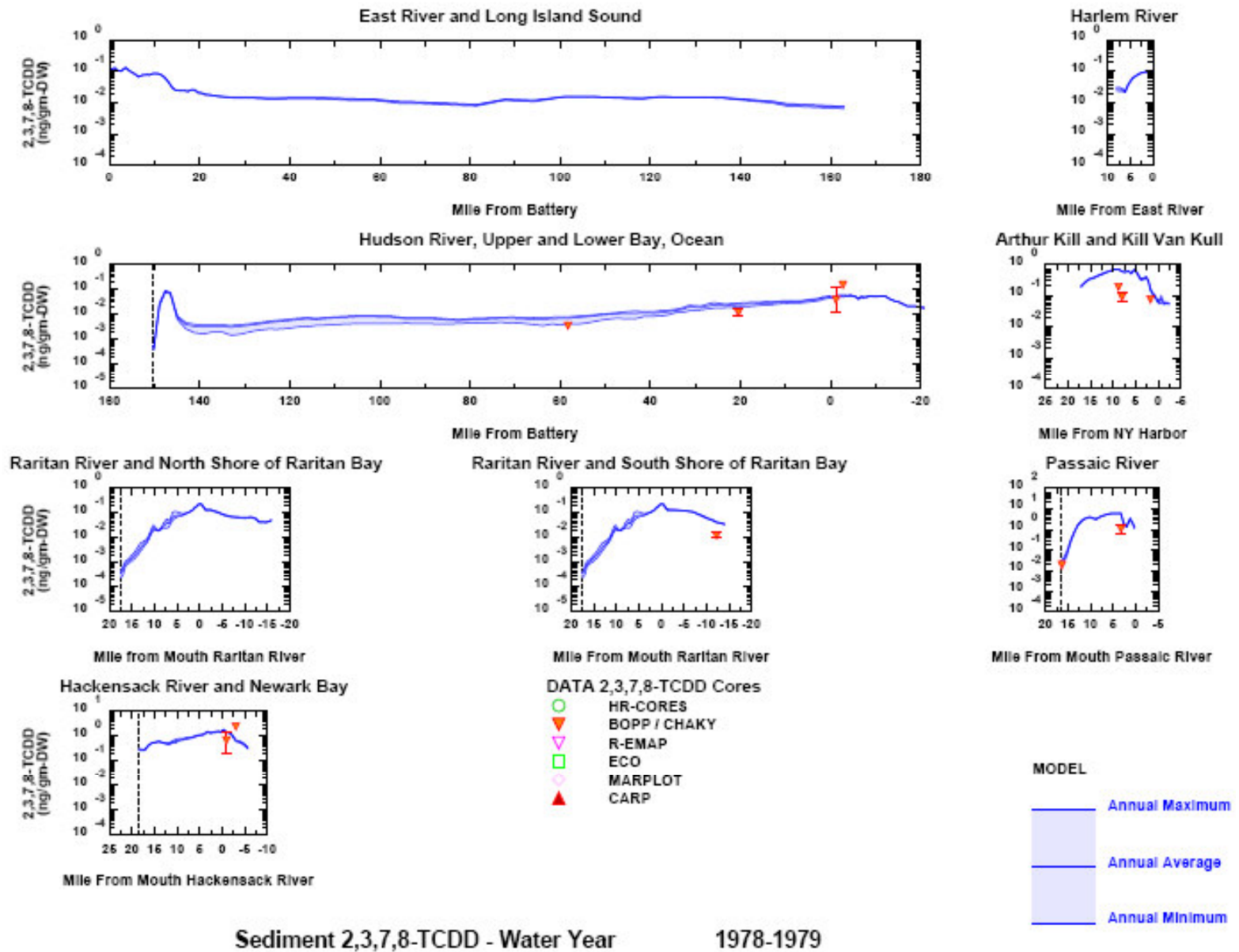
Figure 6-15. Example spatial transect model and data comparisons for CARP 2,3,7,8-TCDD hindcast – 1978-79.
