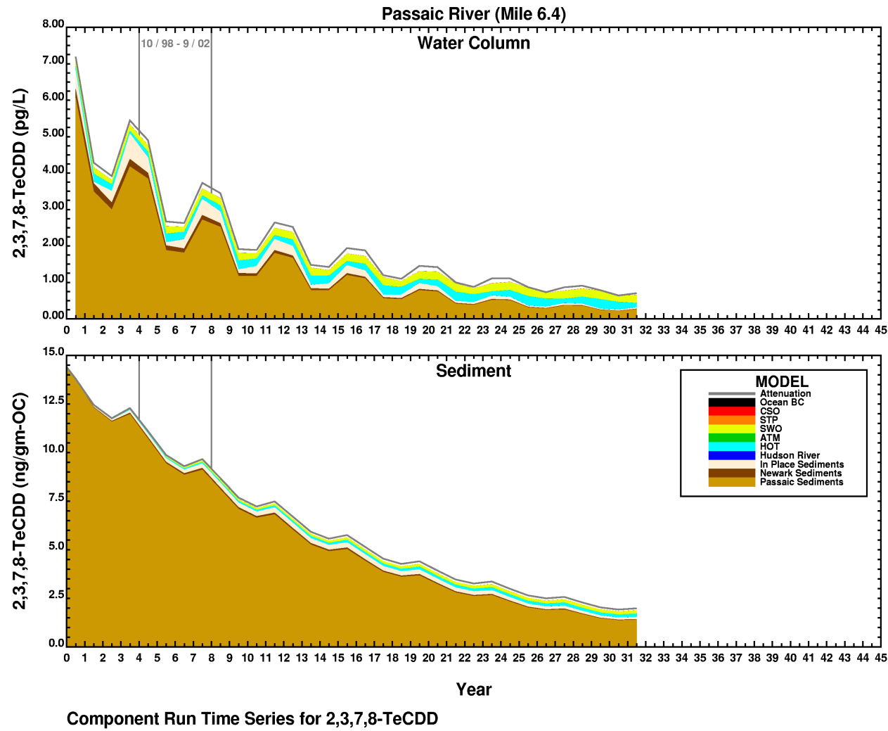
Figure 12-1. Example loading component responses for 32 simulation years
