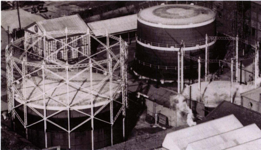
Figure 7. Evolution of gasholders on a former gasworks, Bottom right – Column guided, Bottom Left – Guide framed and Top – Spiral guided.
