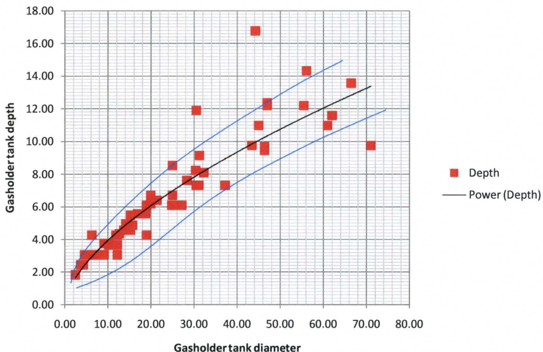
Figure 16. A plot of the Gasholder tank diameter against depth for brick, stone, concrete and composite tanks
