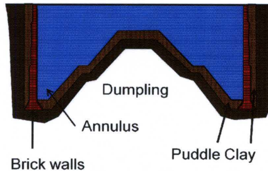
Figure 10. Schematic of a gasholder tank with a dumpling and annulus.
