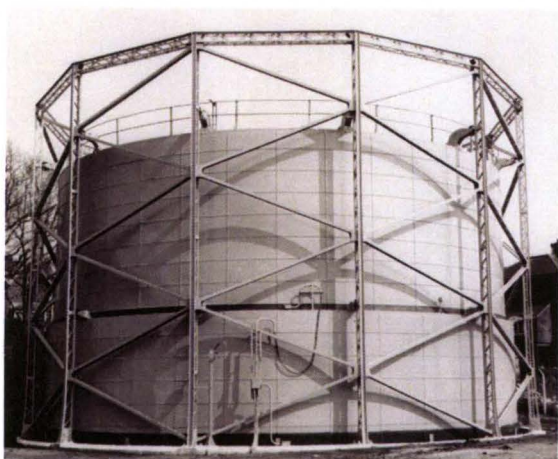
Figure 2. A two lift frame guided gasholder with concrete tank, Southern England
