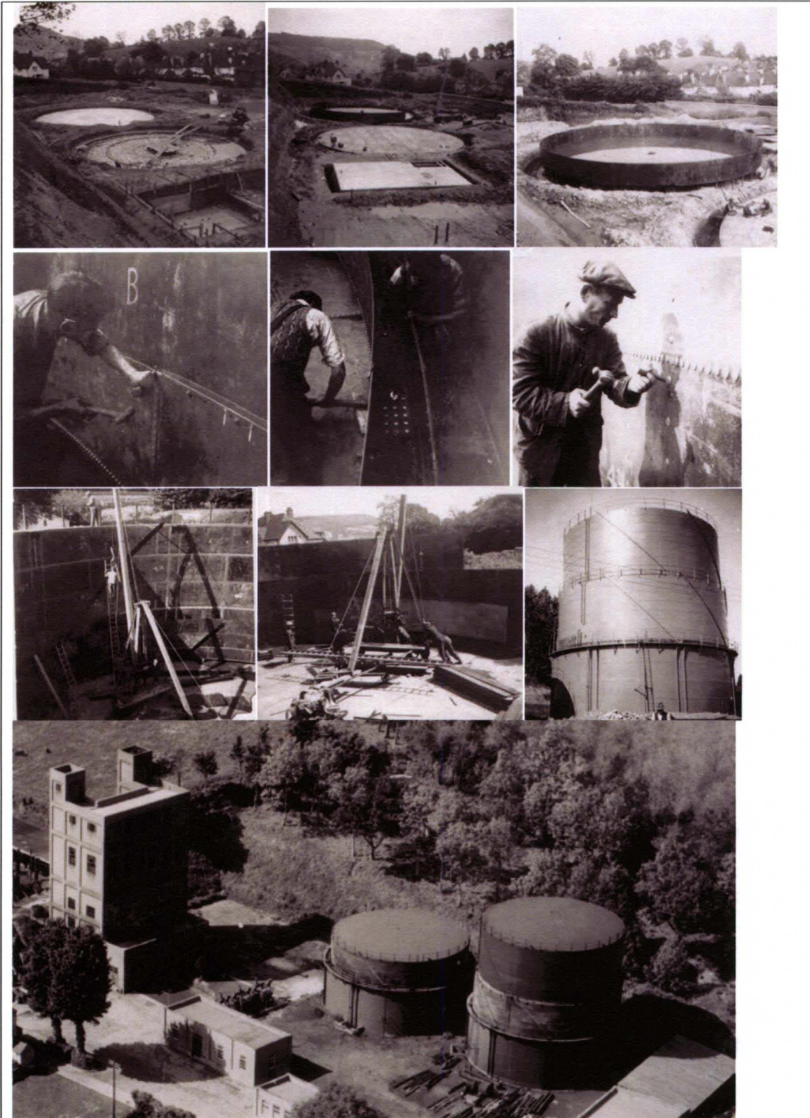
Figure 15. Construction of two above ground spiral guided gasholder at a former gasworks in South West England.
