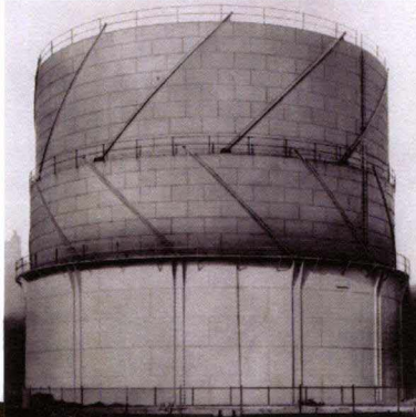
Figure 8b. Multiple Roller Carriage which guide the upwards and downwards movement of the gasholder.
