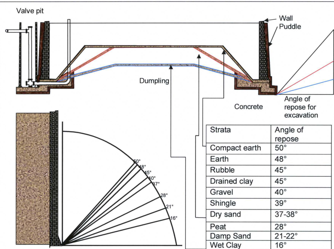
Figure 12. The effect of ground conditions on the angle of repose when constructing an underground gasholder tank. Showing angles of repose for different Strata.
