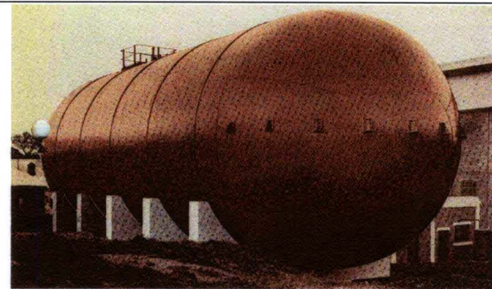
Figure 5. A high pressure bullet tank.
