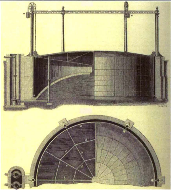
Figure 6. A drawing of an early single lift gasholder with counterweights and a brick tank. From "A Practical Treatise on the manufacture and distribution of coal gas. Richards Williams 1877.
