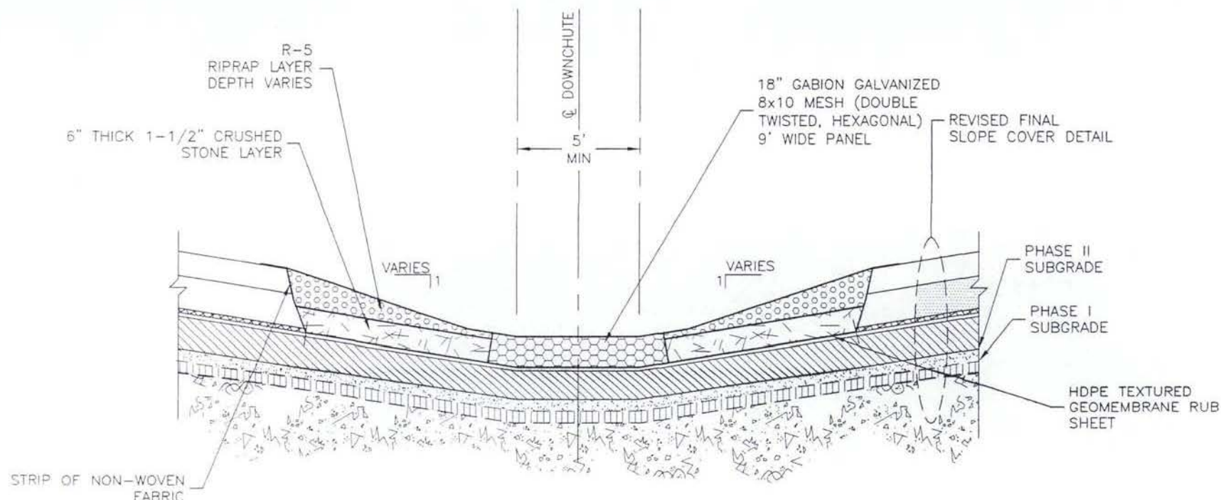
DOWNCHUTE CROSS SECTION (REVISED)
