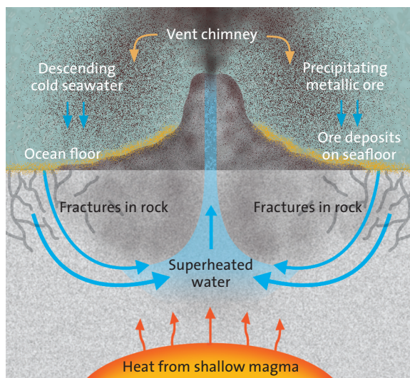
Cross-section of a typical seafloor hydrothermal vent. Source: Ron Toelke.
