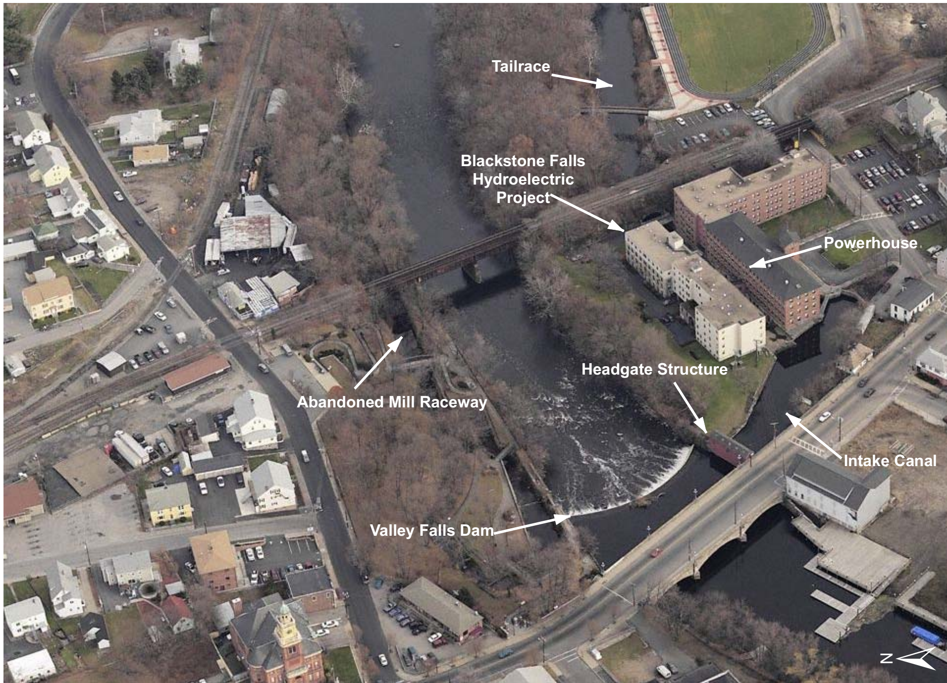
FIGURE 10: BLACKSTONE FALLS HYDROELECTRIC
