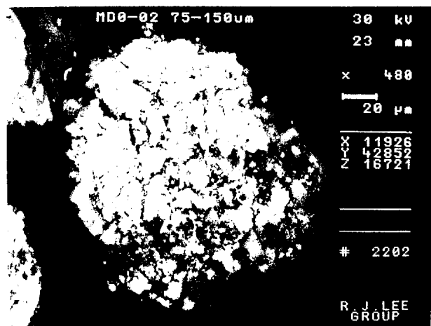
Photomicrograph of a single tailings particle. White flakes are amorphous iron-oxide coatings, many containing trace metals such as As, Zn, and Cu (note 20 micrometer scale above right-center).
