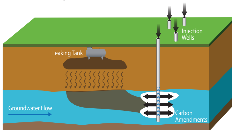
Carbon amendments can be injected underground to treat fuel from leaking tanks.
