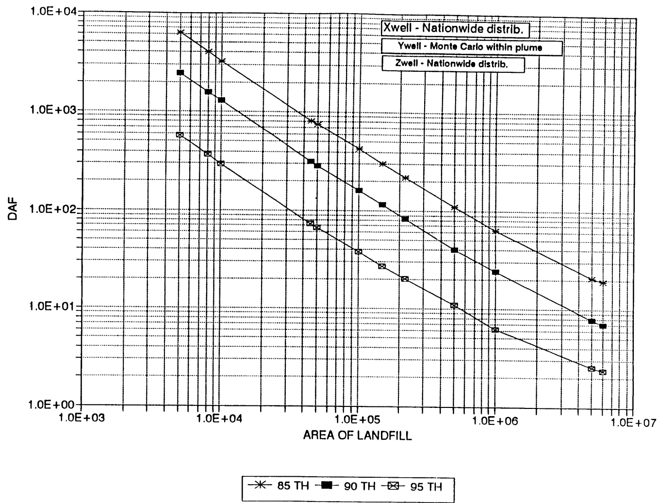
Figure 6 Variation Of DAF With Size Of Source Area For The Default Nationwide Scenario (Scenario 2: x=nationwide distribution, y=uniform in plume, z=nationwide distribution)
