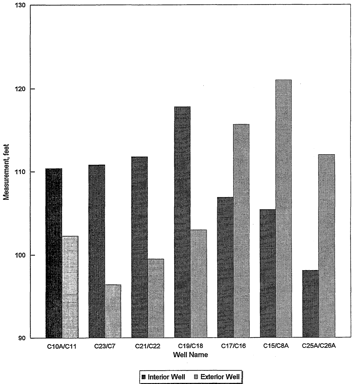
Site 13 FIGURE 3 MAX HEAD DIFFERENCES ACROSS BARRIER Tetra Tech EM Inc.
