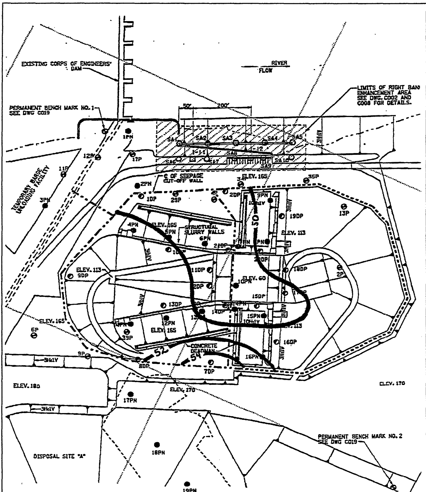
Site 35 FIGURE 3 GROUNDWATER CONTOURS INSIDE THE PERIMETER SEEPAGE CUT-OFF WALL (4/5/96) Tetra Tech EM Inc.
