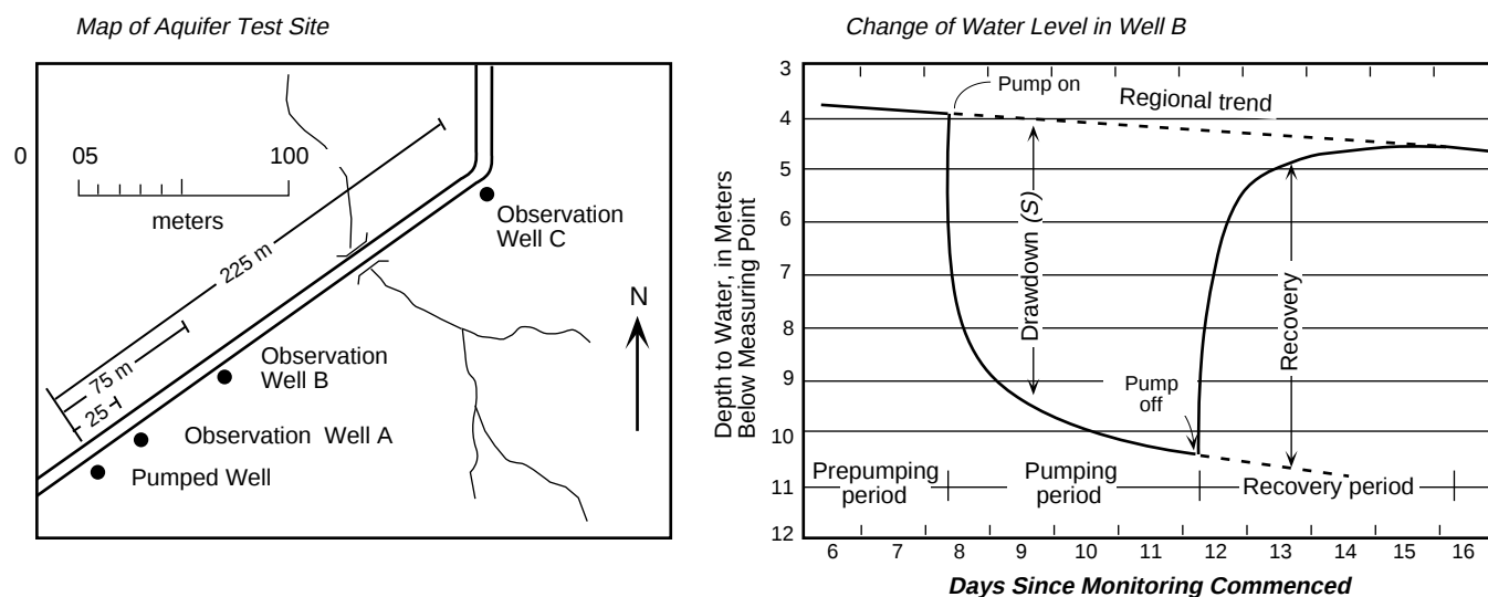
Figure 3. Example test site showing baseline, pumping test, and recovery water level measurements in one of the wells.
