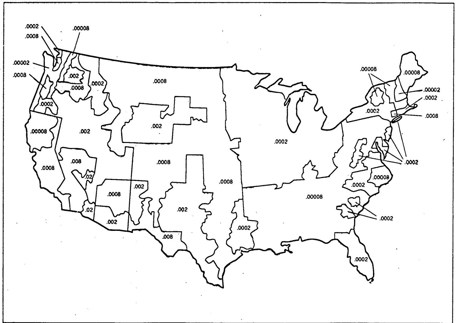
FIGURE 6-3 PARTICULATE MOBILITY FACTOR VALUES a
